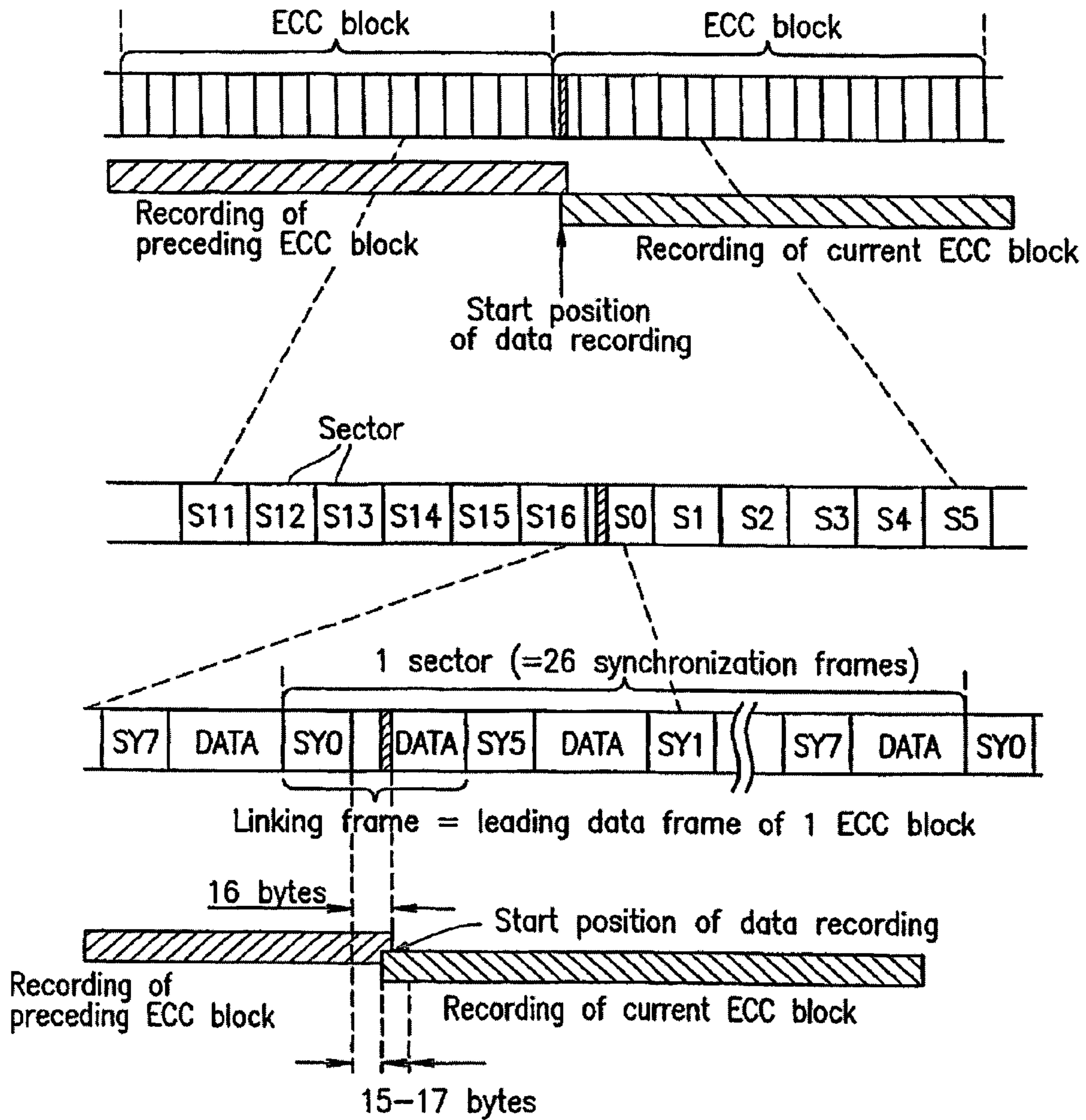
FIG. 44 CONVENTIONAL ART
