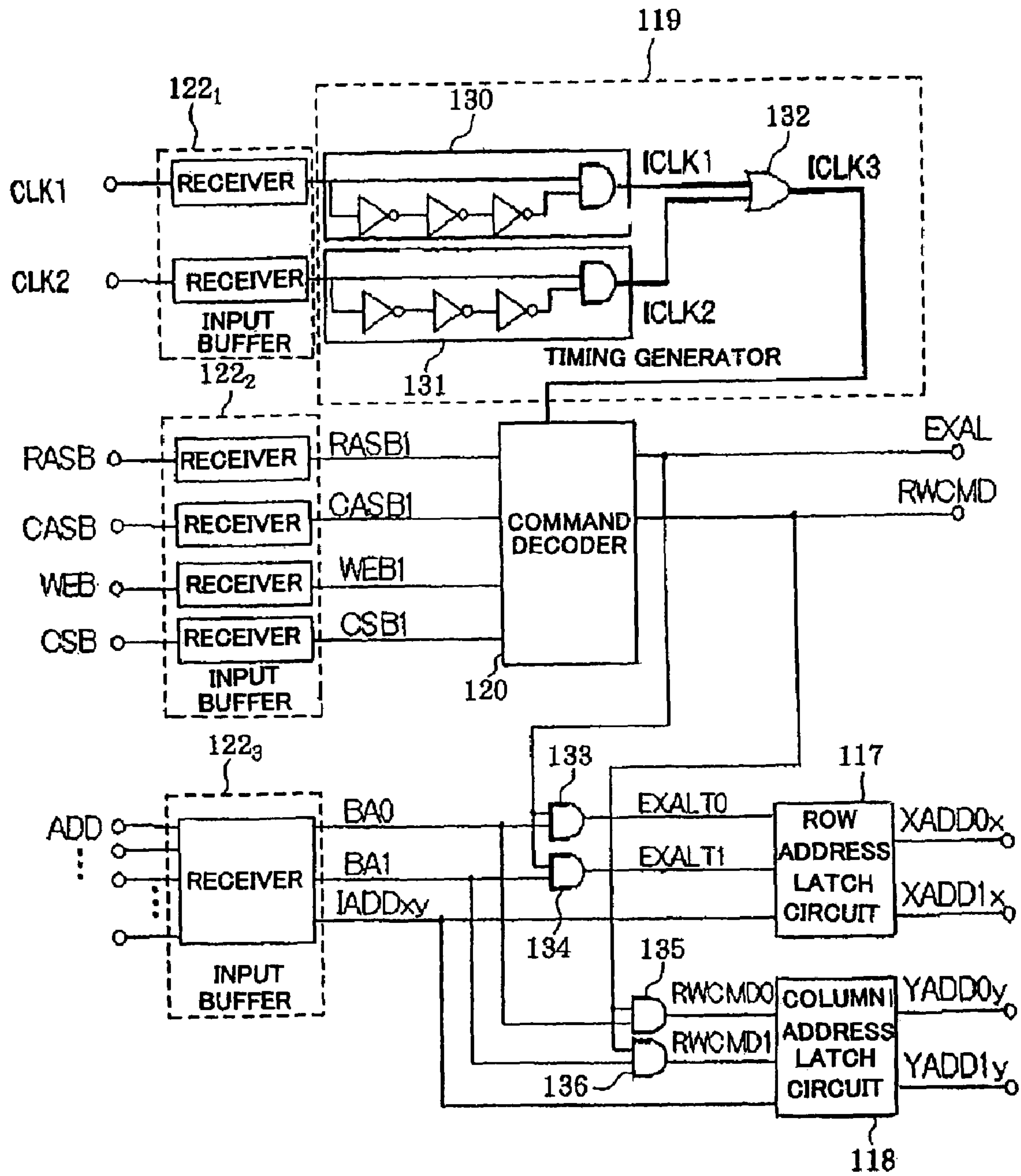
FIG. 2 (PRIOR ART)
