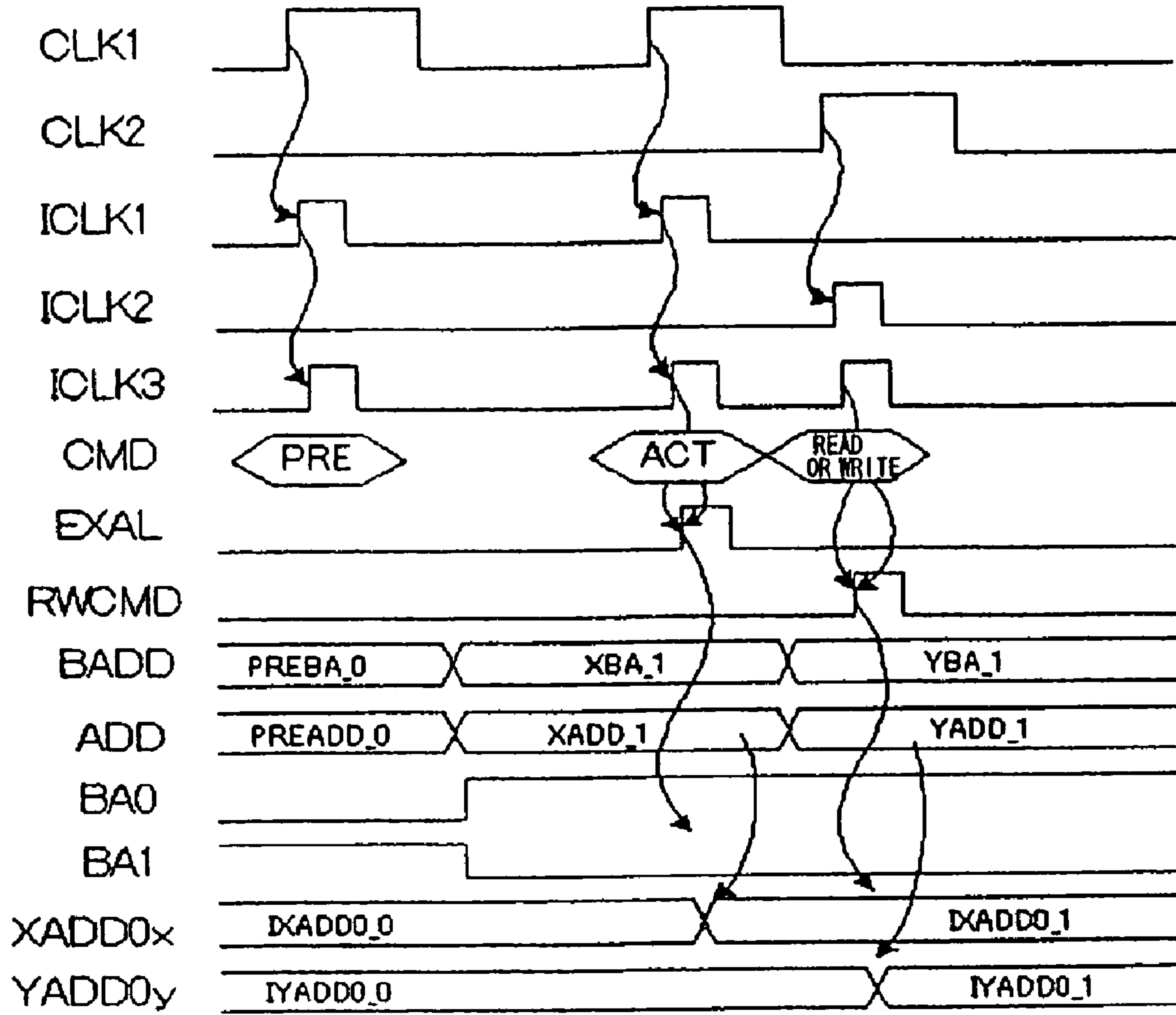
FIG. 3 (PRIOR ART)
