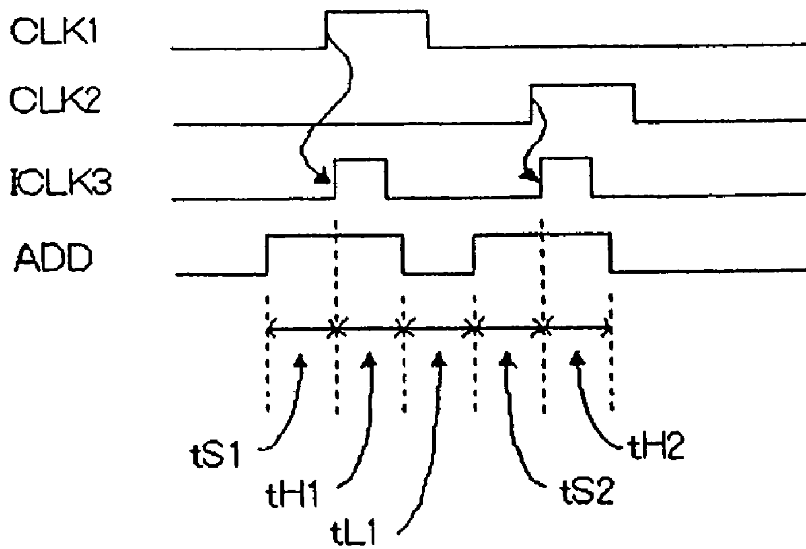
FIG. 4 (PRIOR ART)
