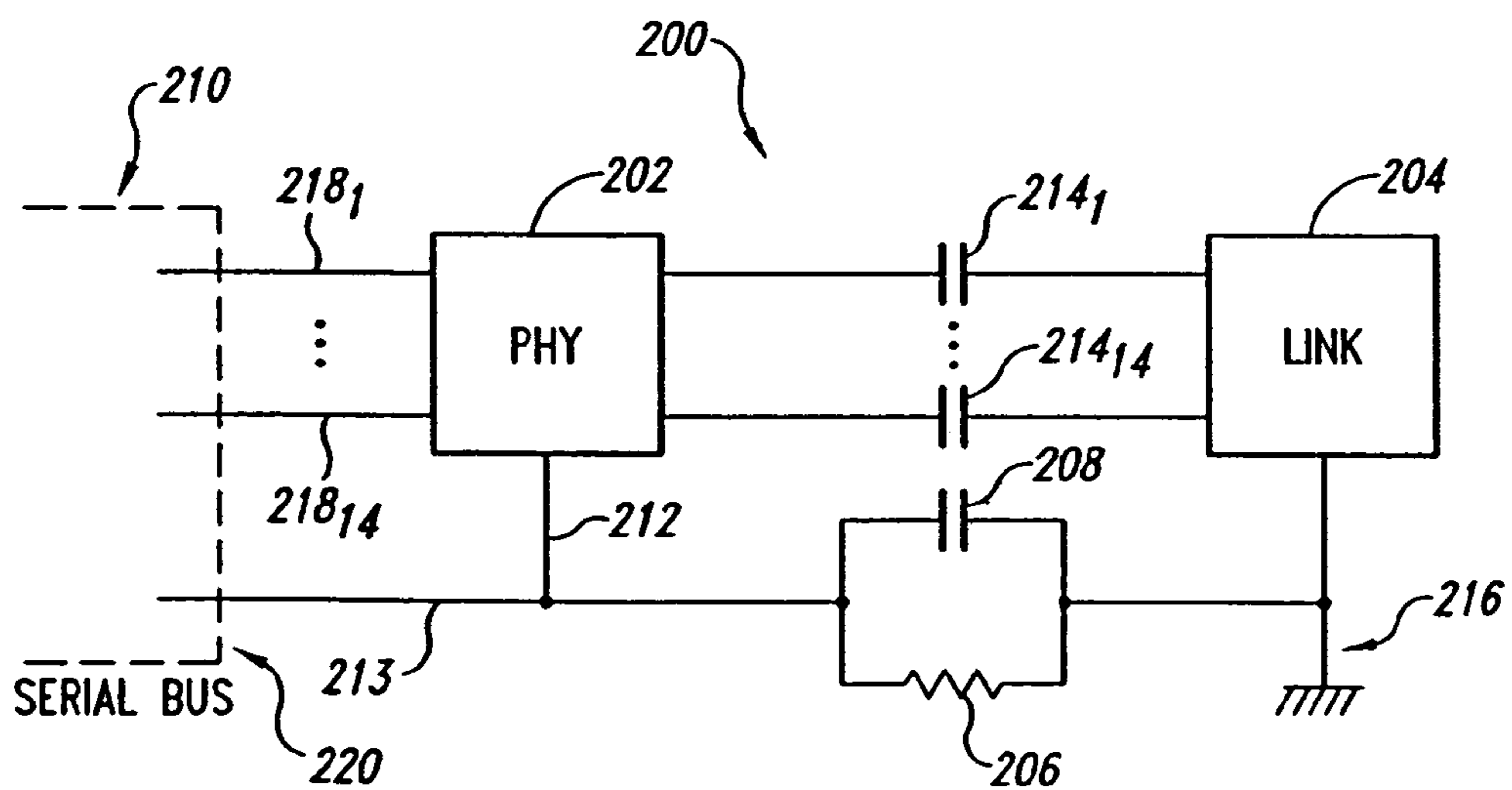
Fig. 2 (Prior Art)
