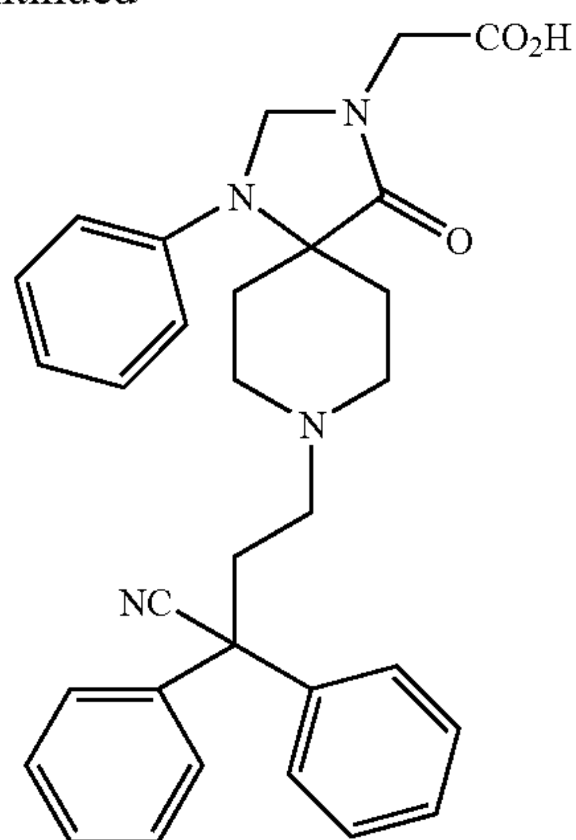
Compound AD
