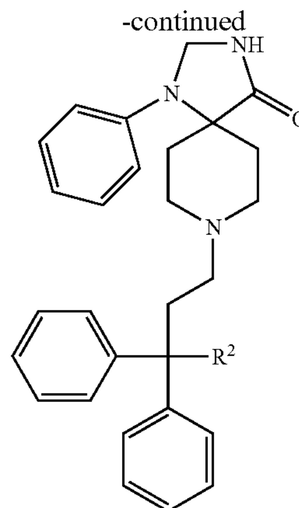
Compound C
