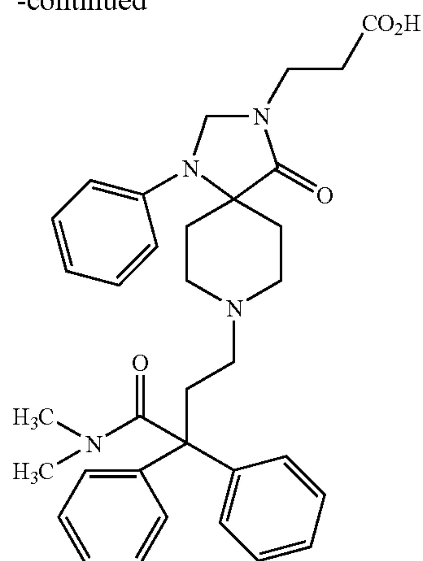
Compound AT
