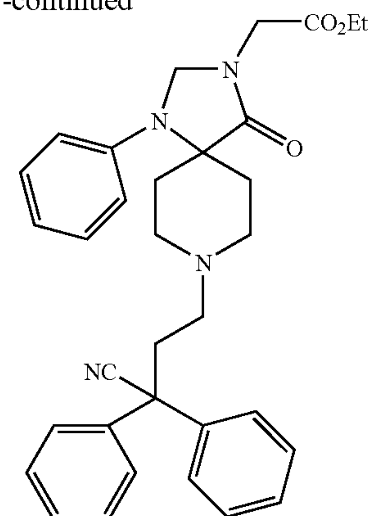
Compound AH
