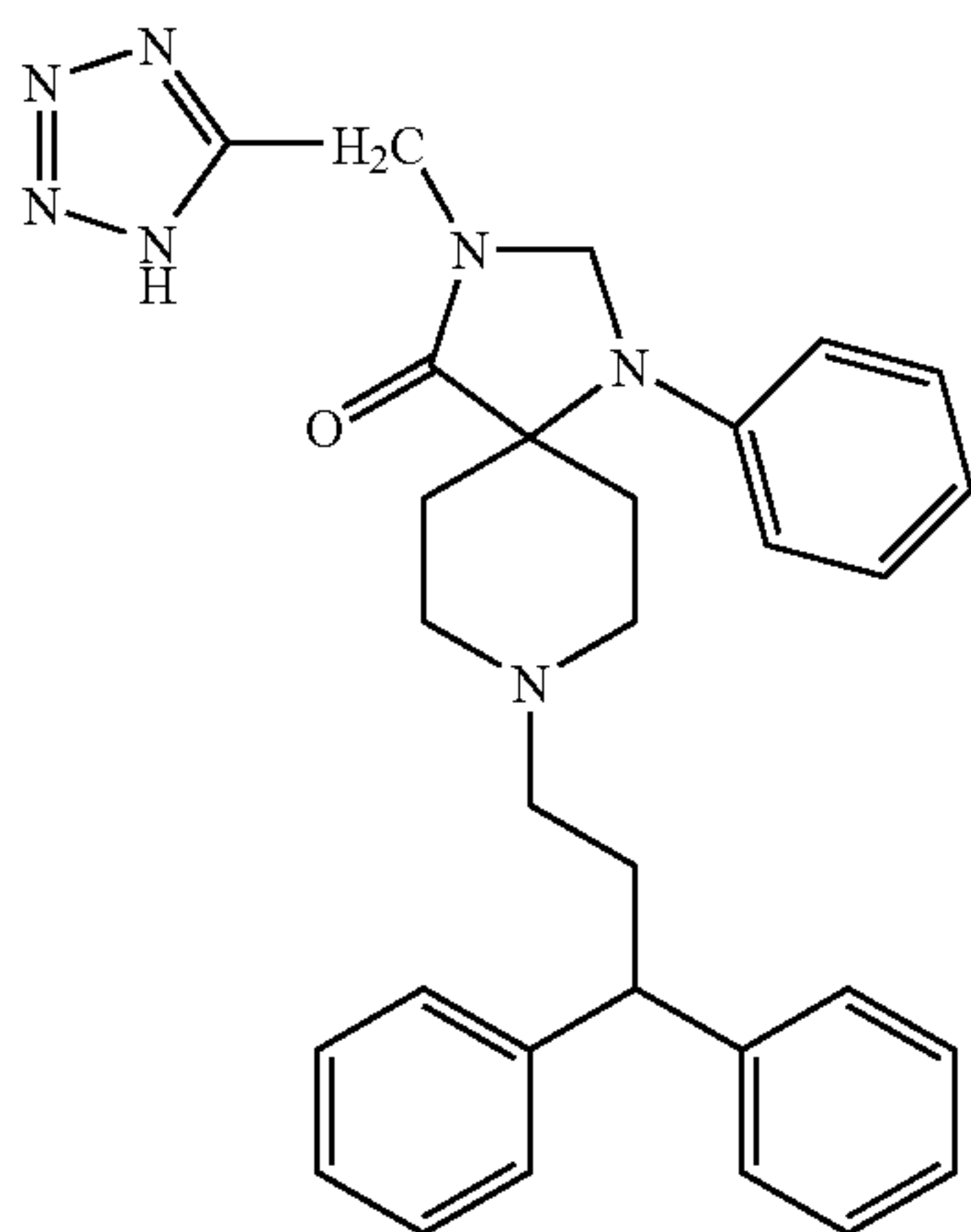
8-(3,3-diphenyl-propyl)-1-phenyl-3-(1H-tetrazol-5-ylmethyl)-1,3,8-triaza-spiro[4.5]decan-4-one;
