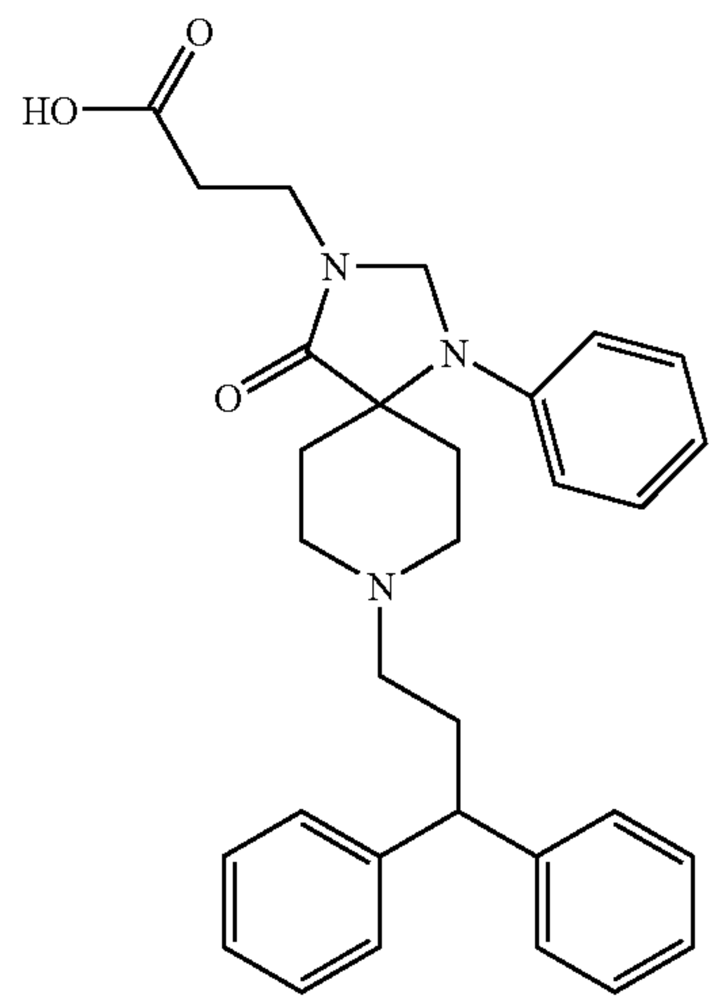
3-[8-(3,3-Diphenyl-propyl)-4-oxo-1-phenyl-1,3,8-triazaspiro[4.5]dec-3-yl]-propionic acid;
