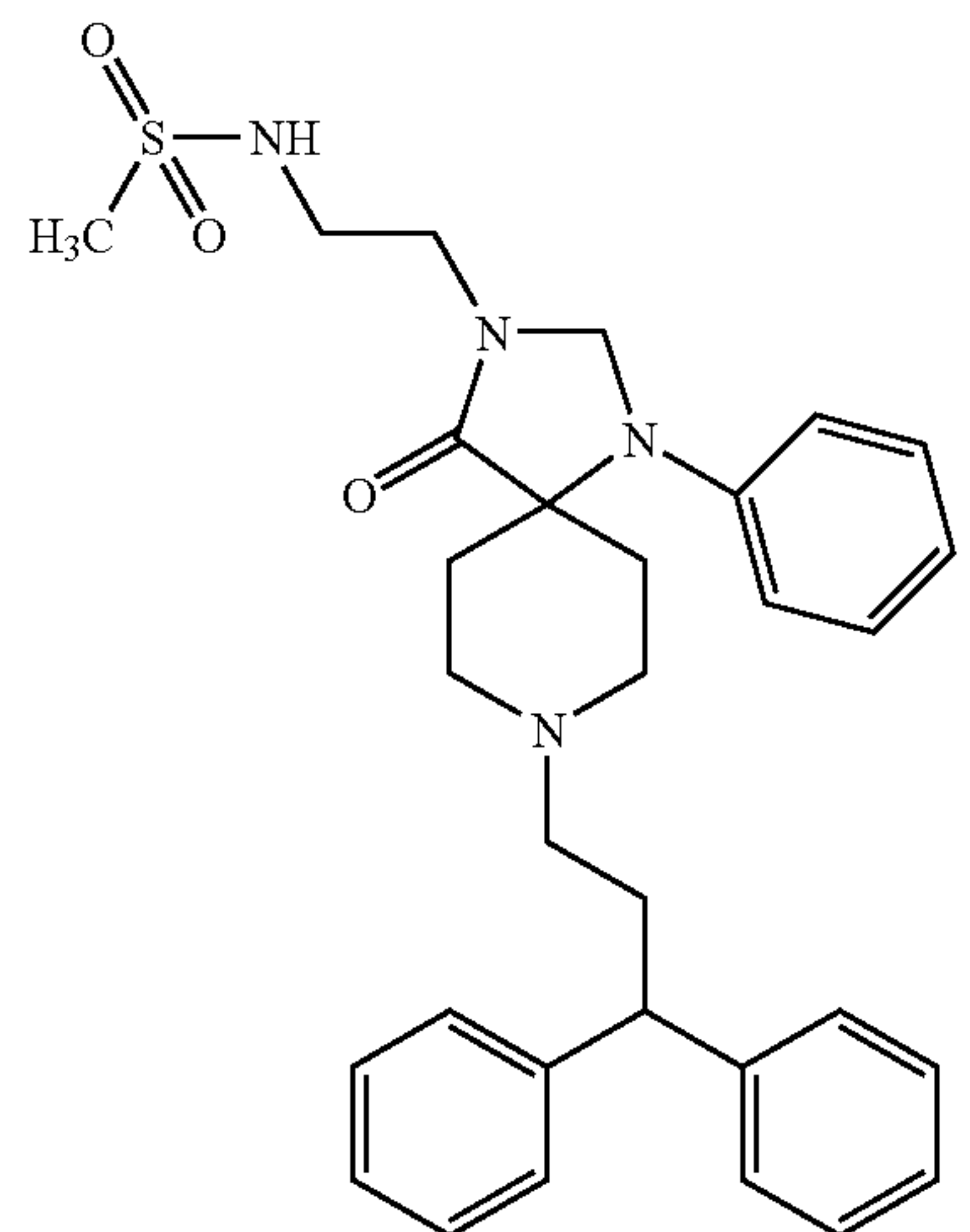
N-{2-[8-(3,3-Diphenyl-propyl)-4-oxo-1-phenyl-1,3,8-triazaspiro[4.5]dec-3-yl]-ethyl}-methanesulfonamide;
