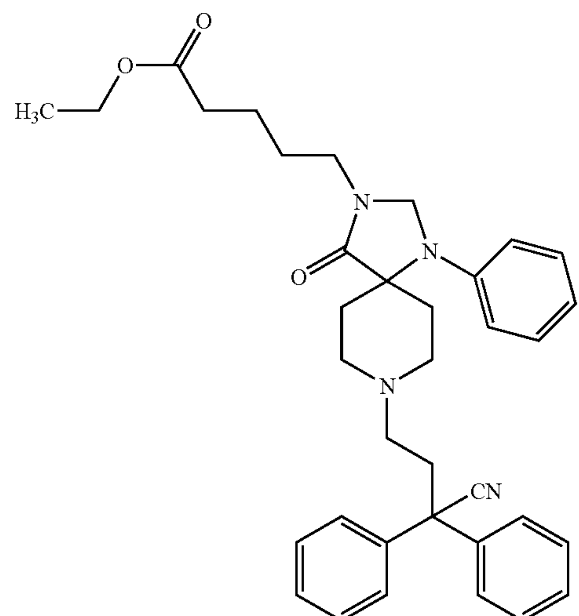
5-[8-(3-Cyano-3,3-diphenyl-propyl)-4-oxo-1-phenyl-1,3,8-triaza-spiro[4.5]dec-3-yl]-pentanoic acid ethyl ester;
