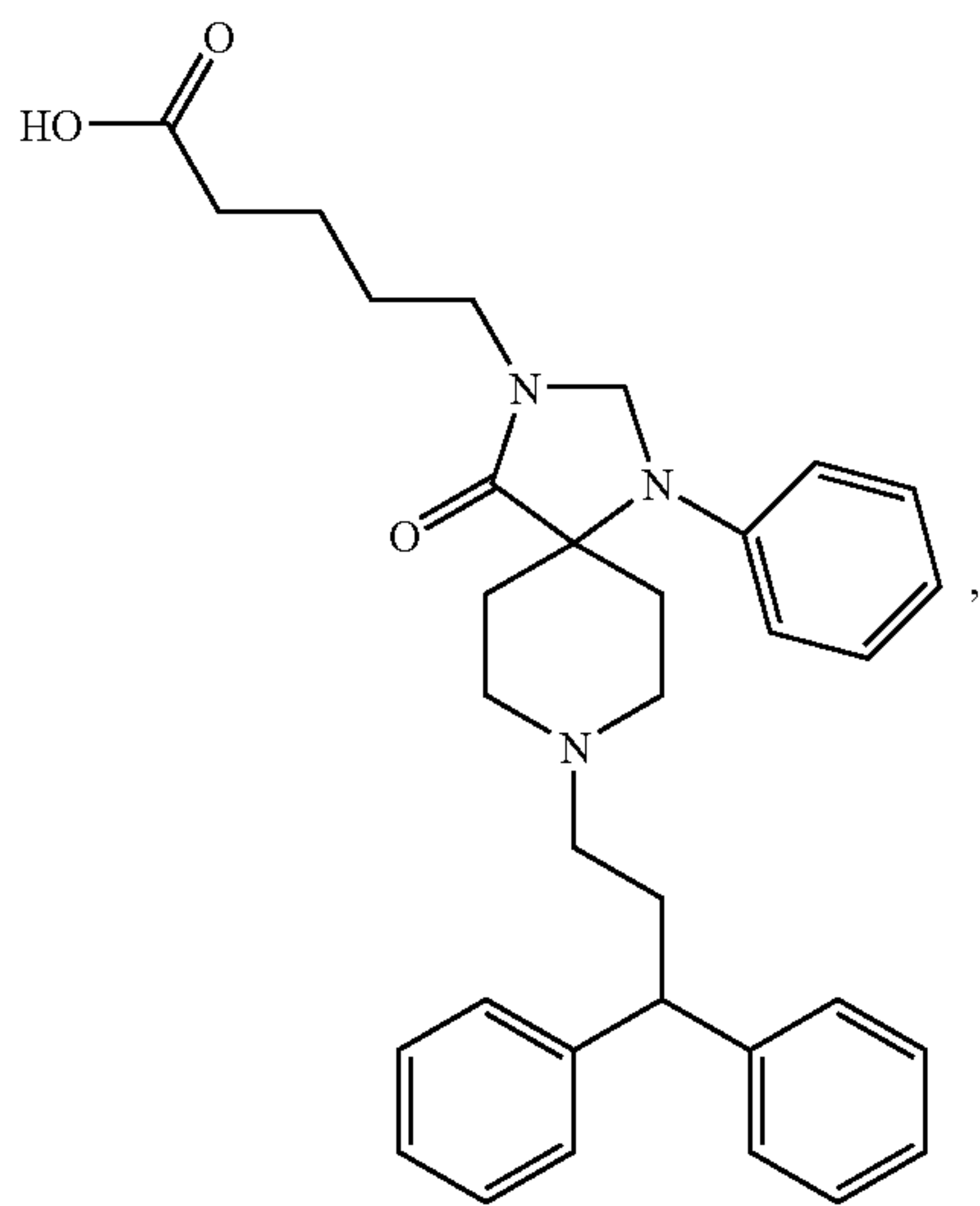
5-[8-(3,3-Diphenyl-propyl)-4-oxo-1-phenyl-1,3,8-triaza-spiro[4.5]dec-3-yl]-pentanoic acid;
