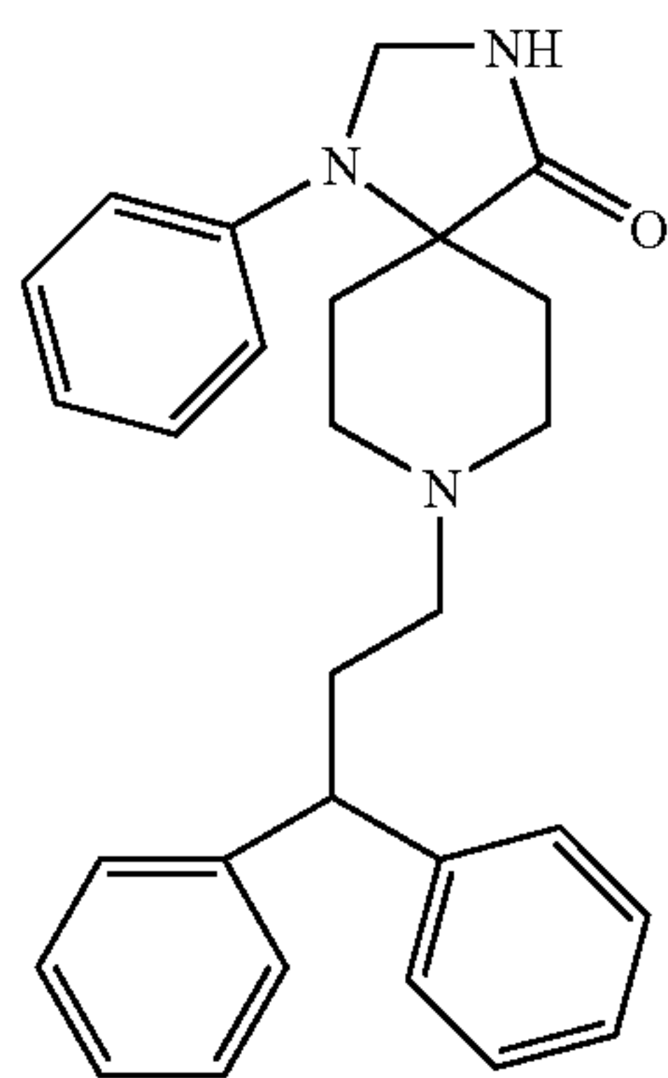
Compound F
