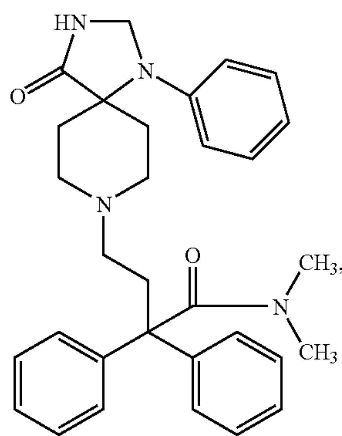
N,N-Dimethyl-4-(4-oxo-1-phenyl-1,3,8-triaza-spiro[4.5]dec-8-yl)-2,2-diphenyl-butryamide;
