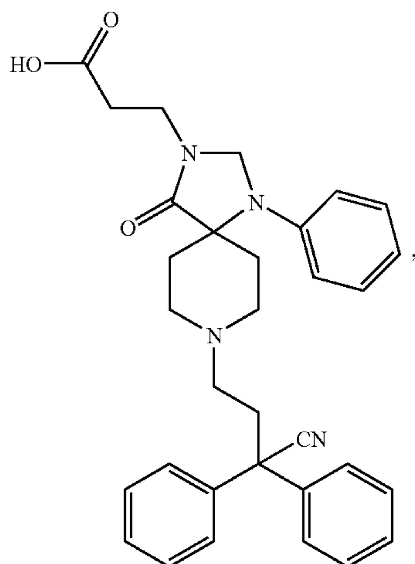
3-[8-(3-Cyano-3,3-diphenyl-propyl)-4-oxo-1-phenyl-1,3,8-triaza-spiro[4.5]dec-3-yl]-propionic acid;
