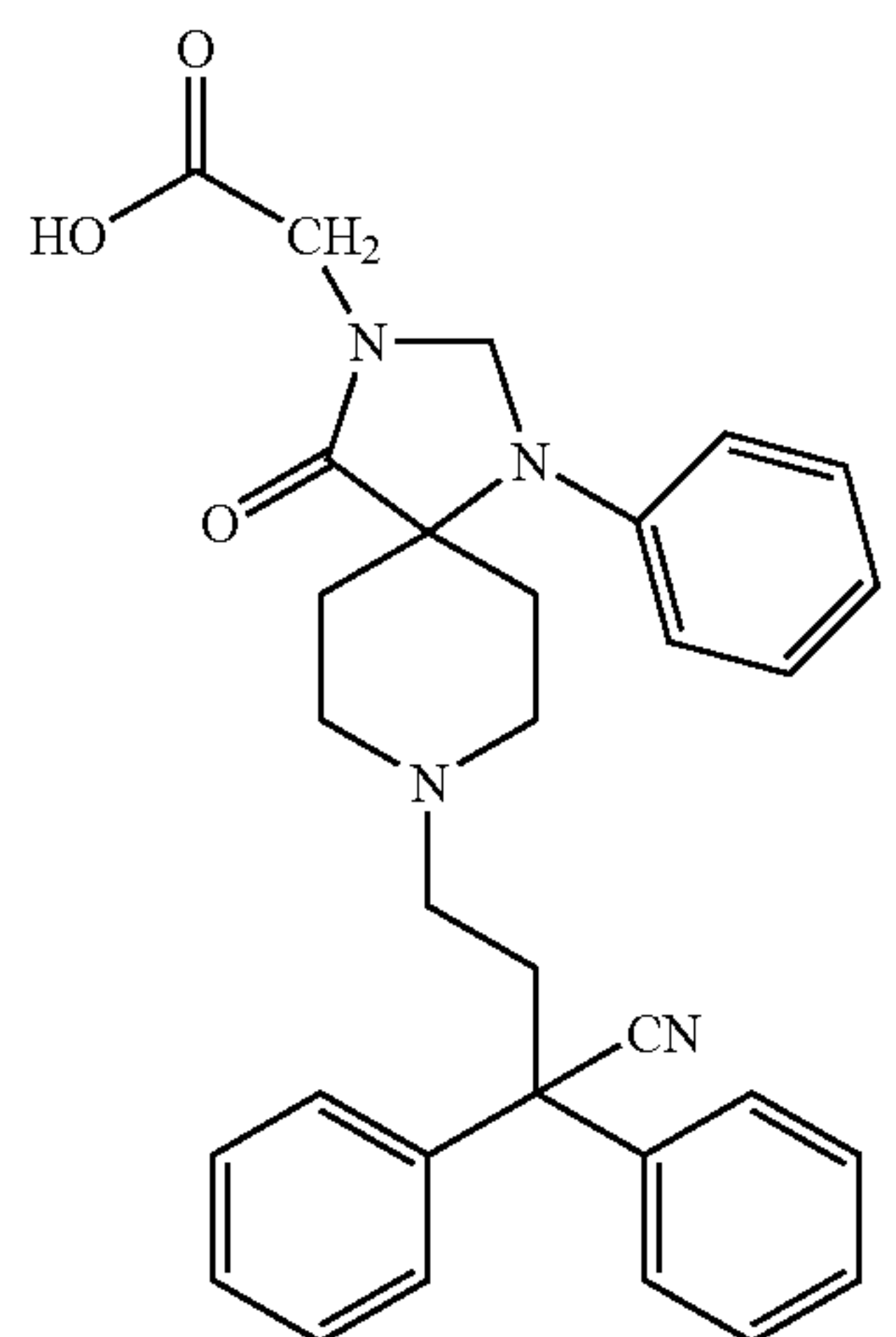
[8-(3-Cyano-3,3-diphenyl-propyl)-4-oxo-1-phenyl-1,3,8-triaza-spiro[4.5]dec-3-yl]-acetic acid;
