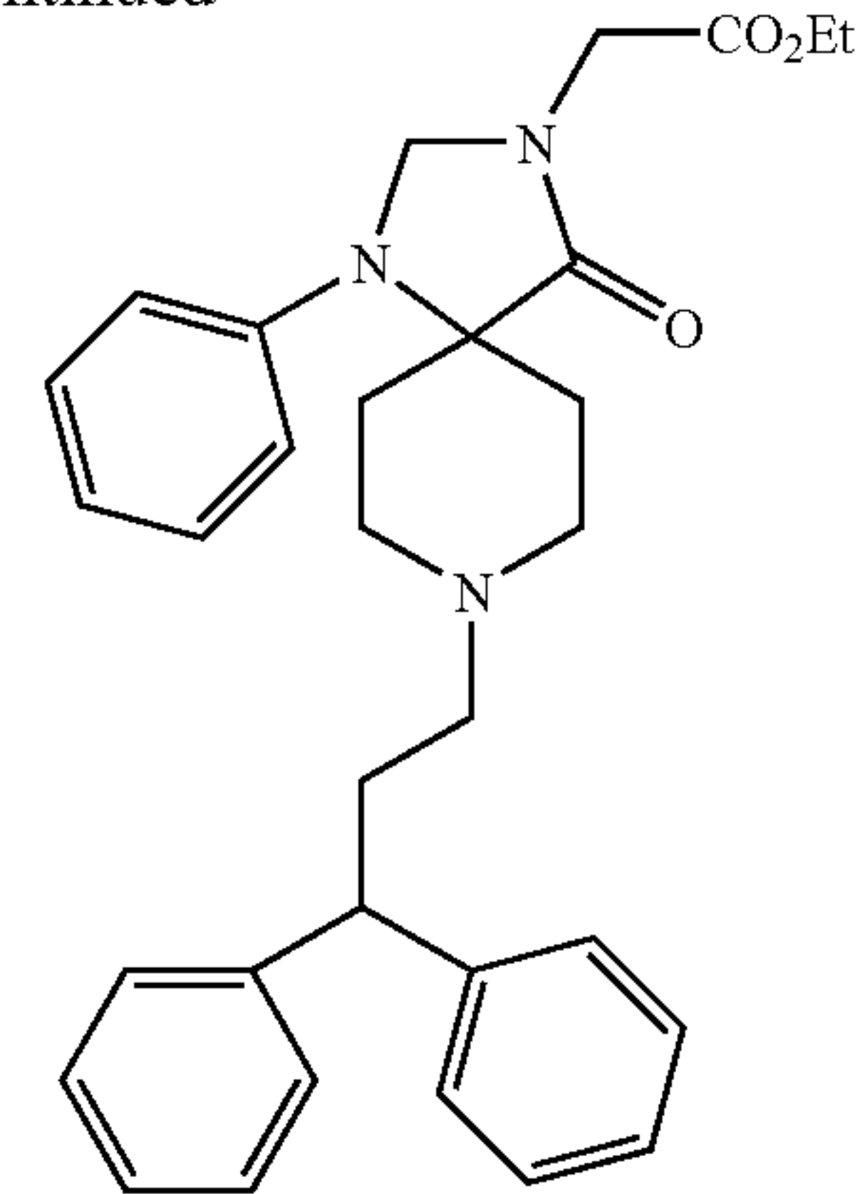
Compound AG
