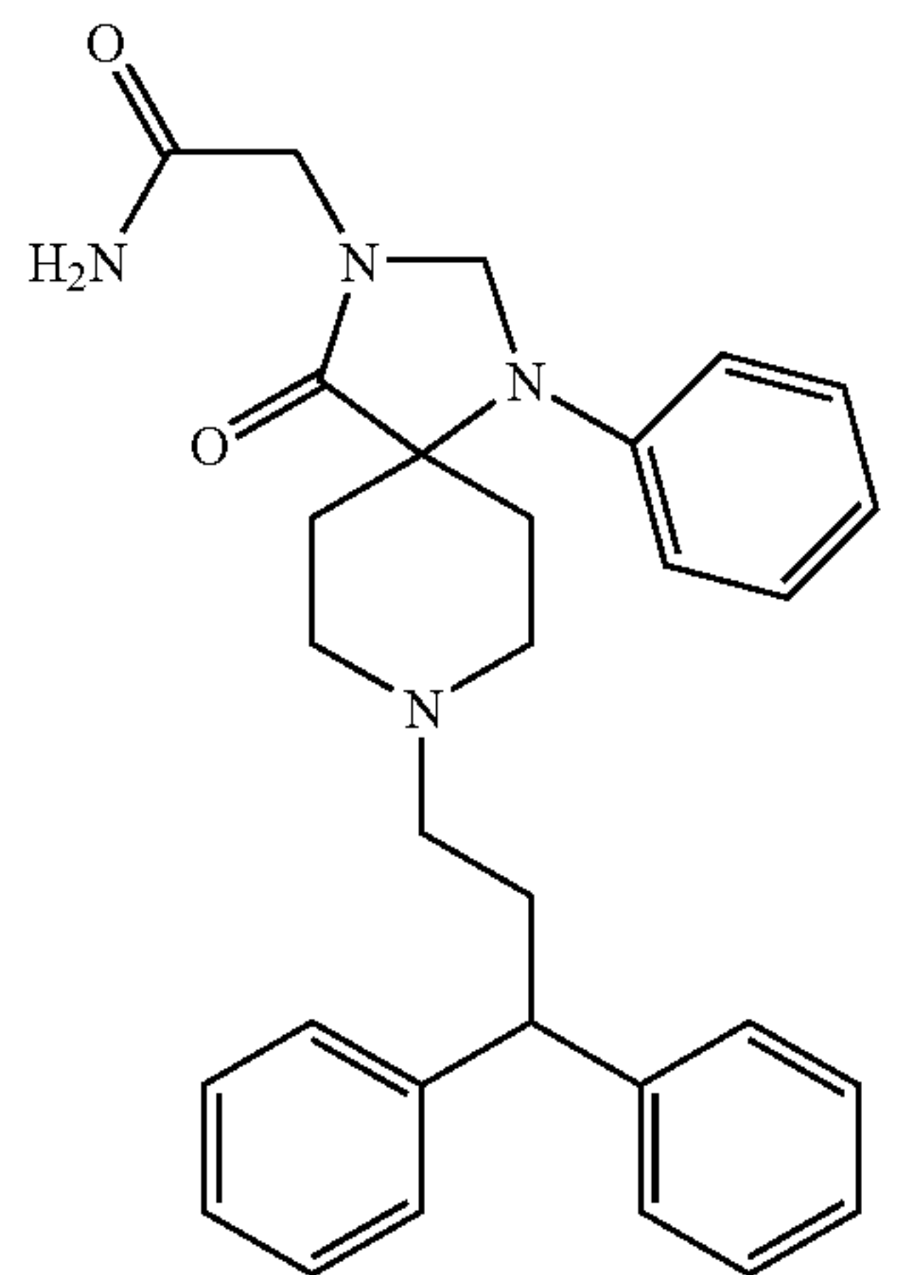
2-[8-(3,3-Diphenyl-propyl)-4-oxo-1-phenyl-1,3,8-triazaspiro[4.5]dec-3-yl]-acetamide
