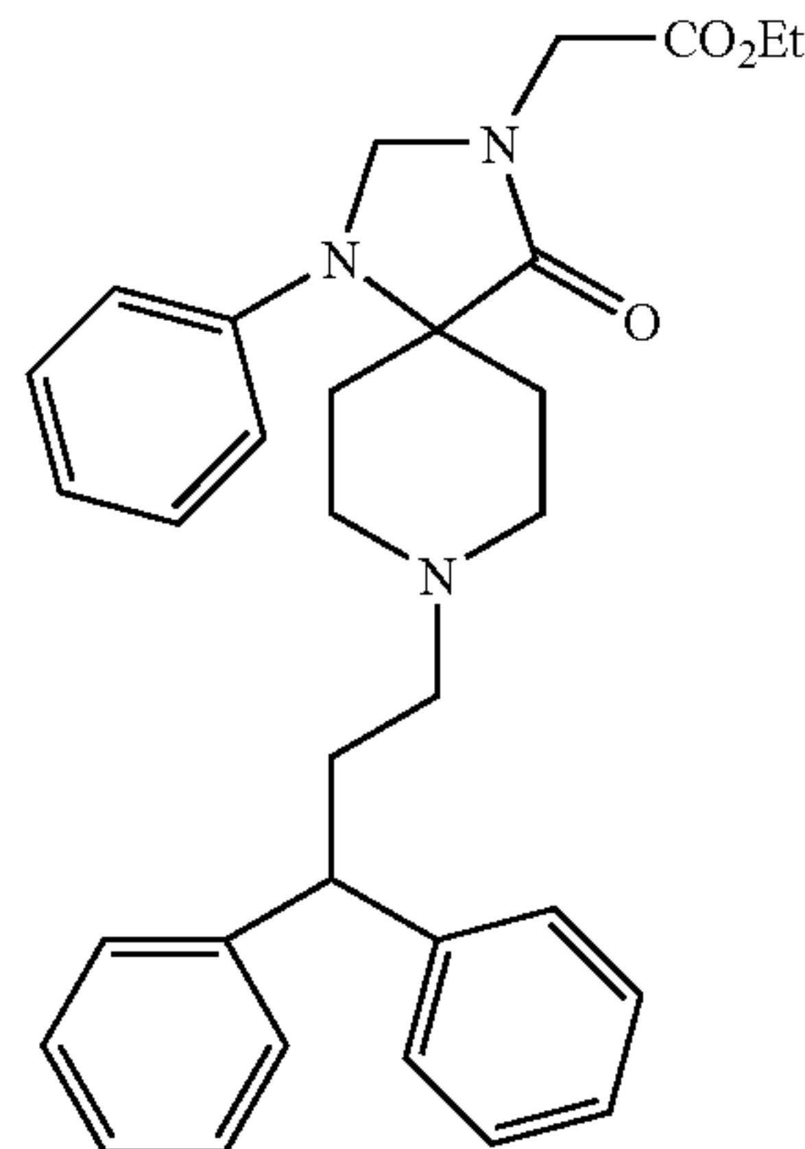
Compound AG
