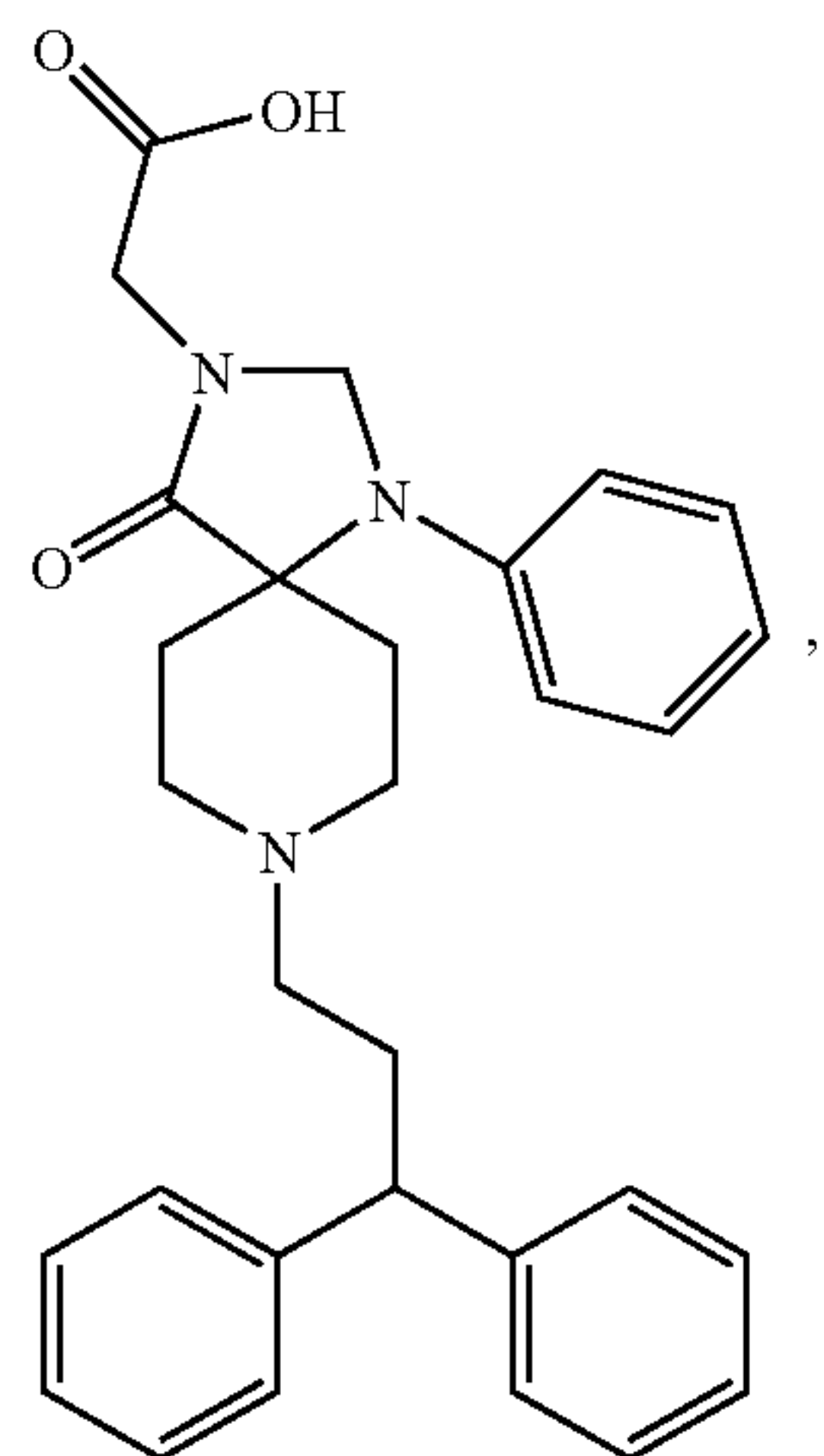
[8-(3,3-Diphenyl-propyl)-4-oxo-1-phenyl-1,3,8-triazaspiro[4.5]dec-3-yl]-acetic acid;
