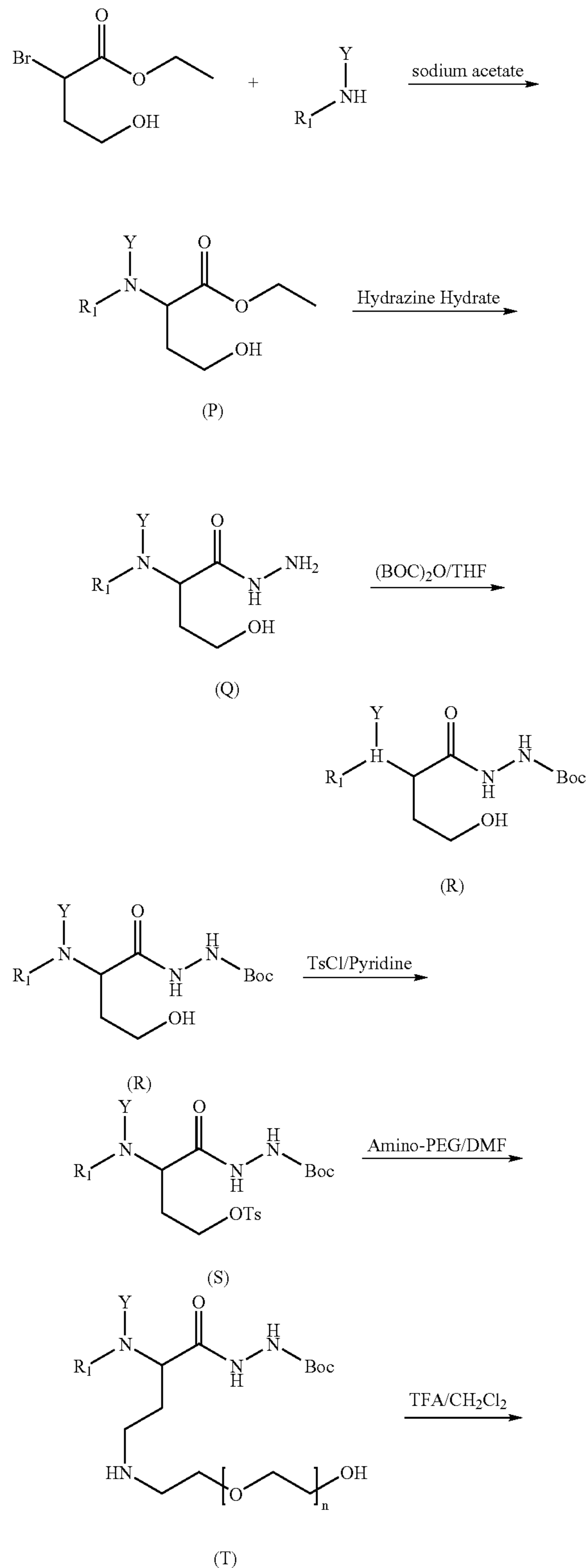
REACTION SCHEME 9
