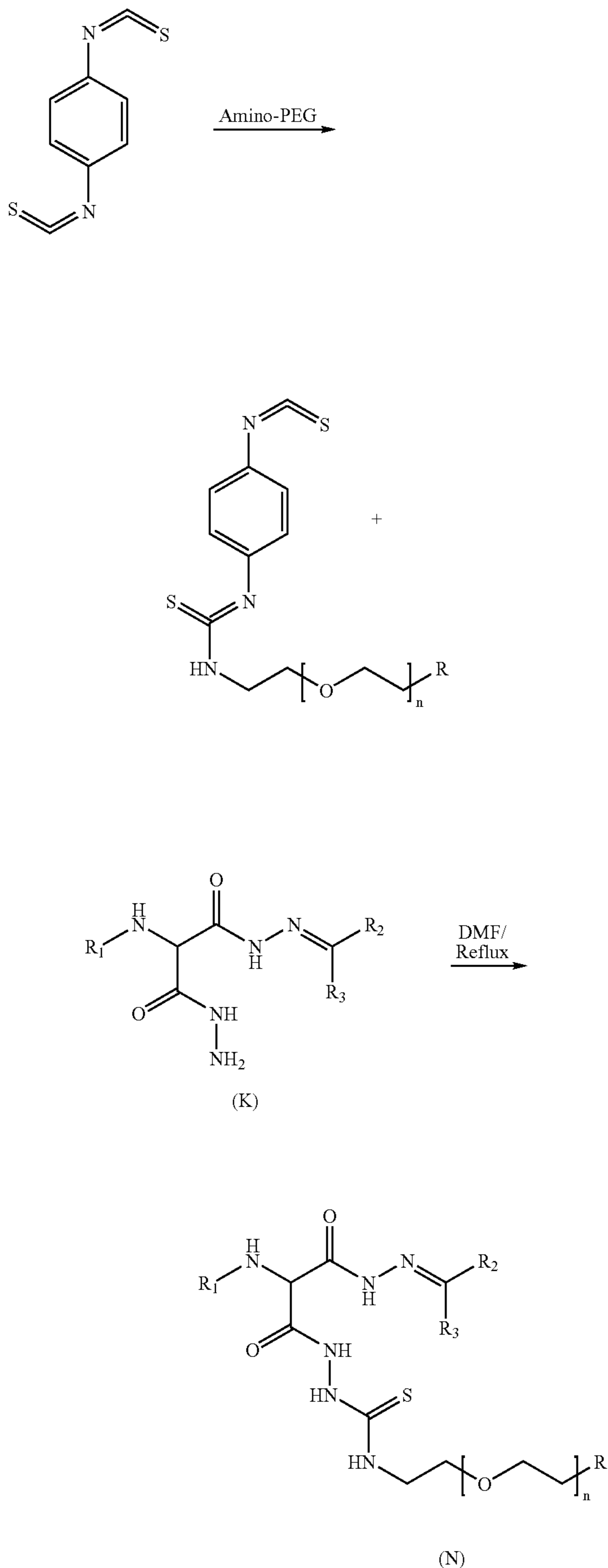
REACTION SCHEME 7
