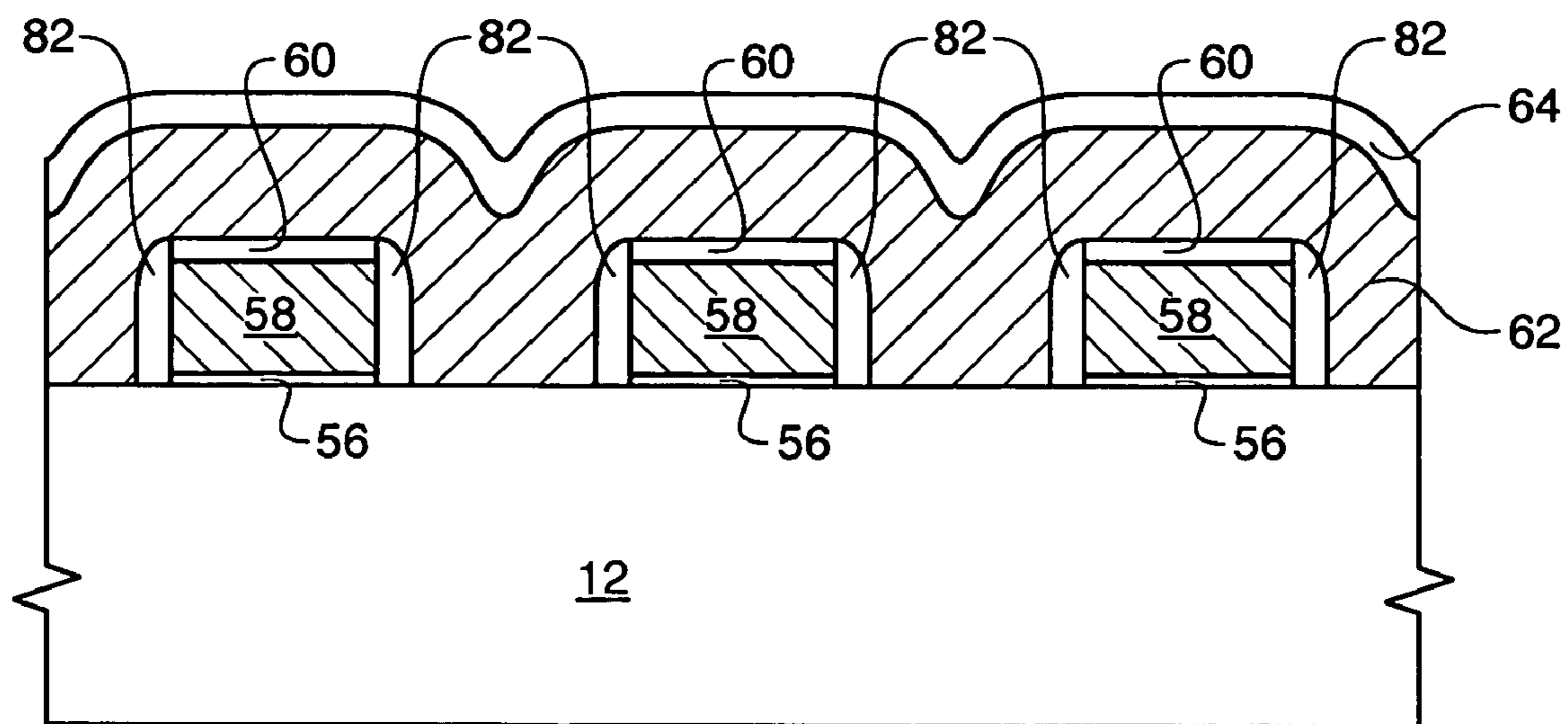
FIG. 7 (RELATED ART)
