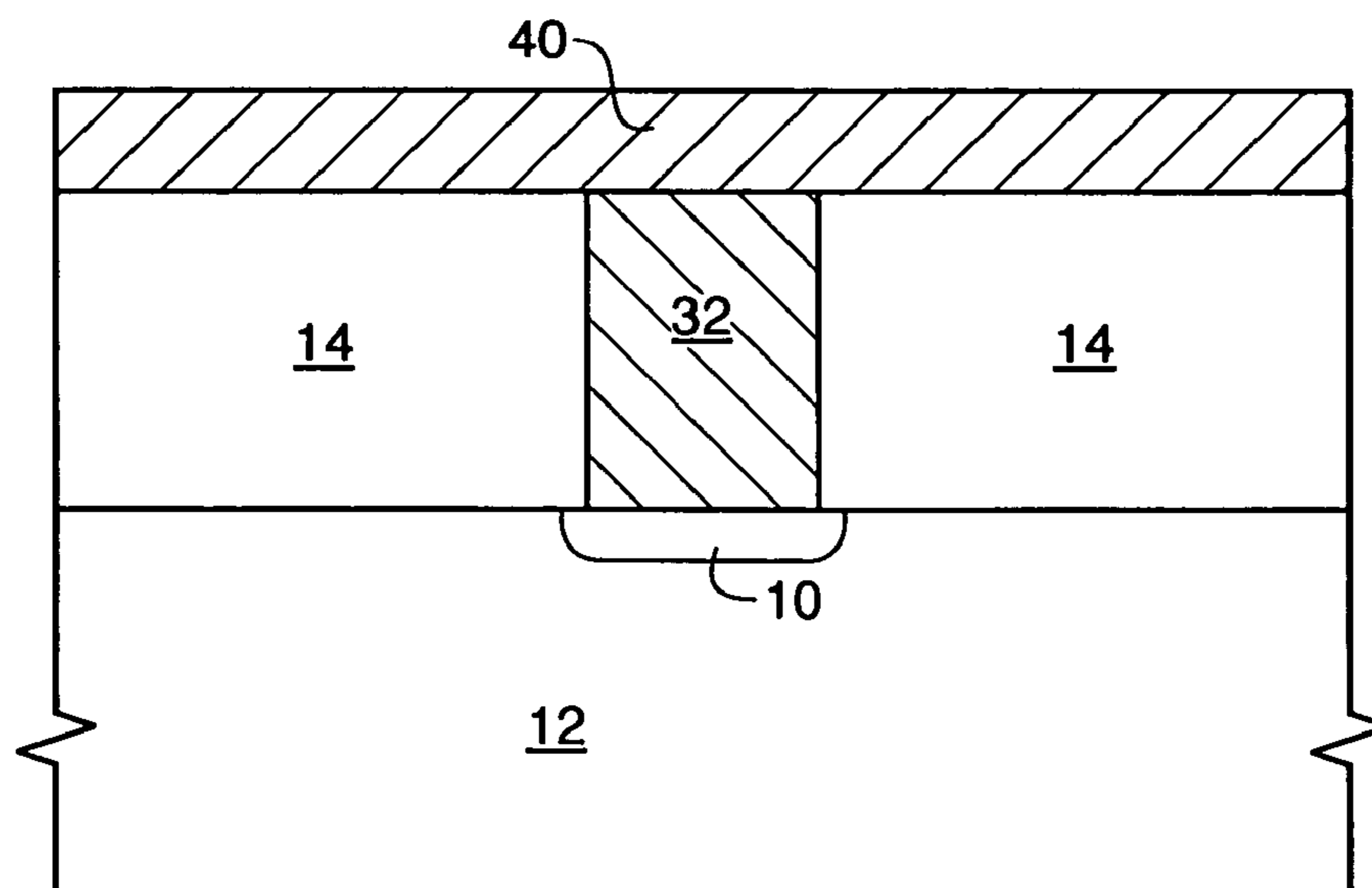
FIG. 4 (RELATED ART)
