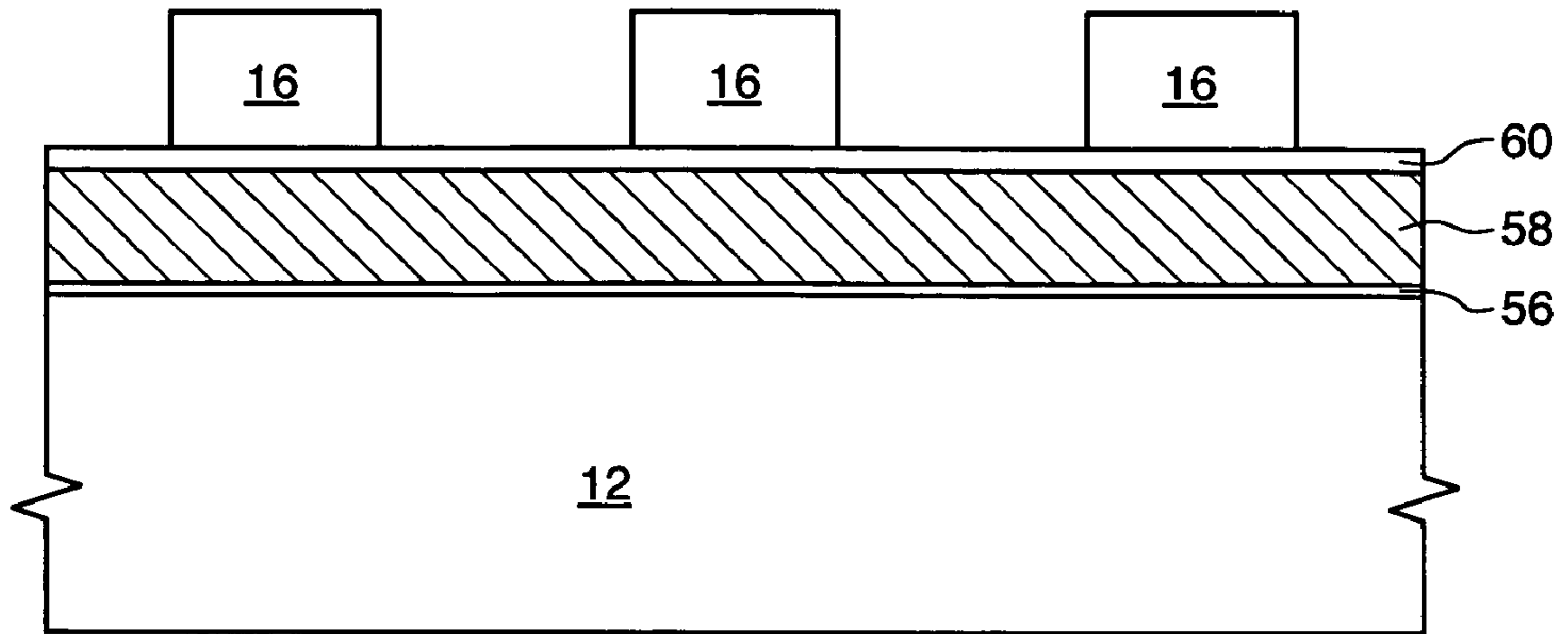
FIG. 6 (RELATED ART)
