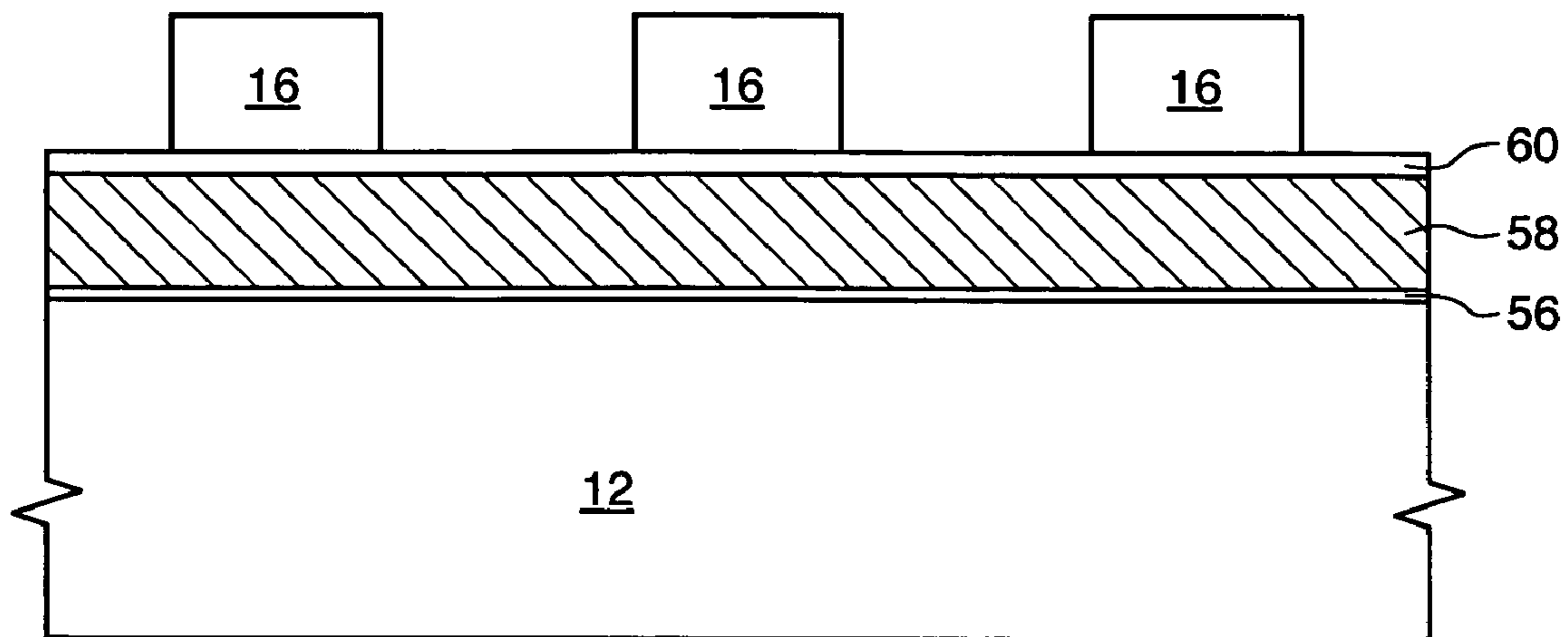
FIG. 6 (RELATED ART)
