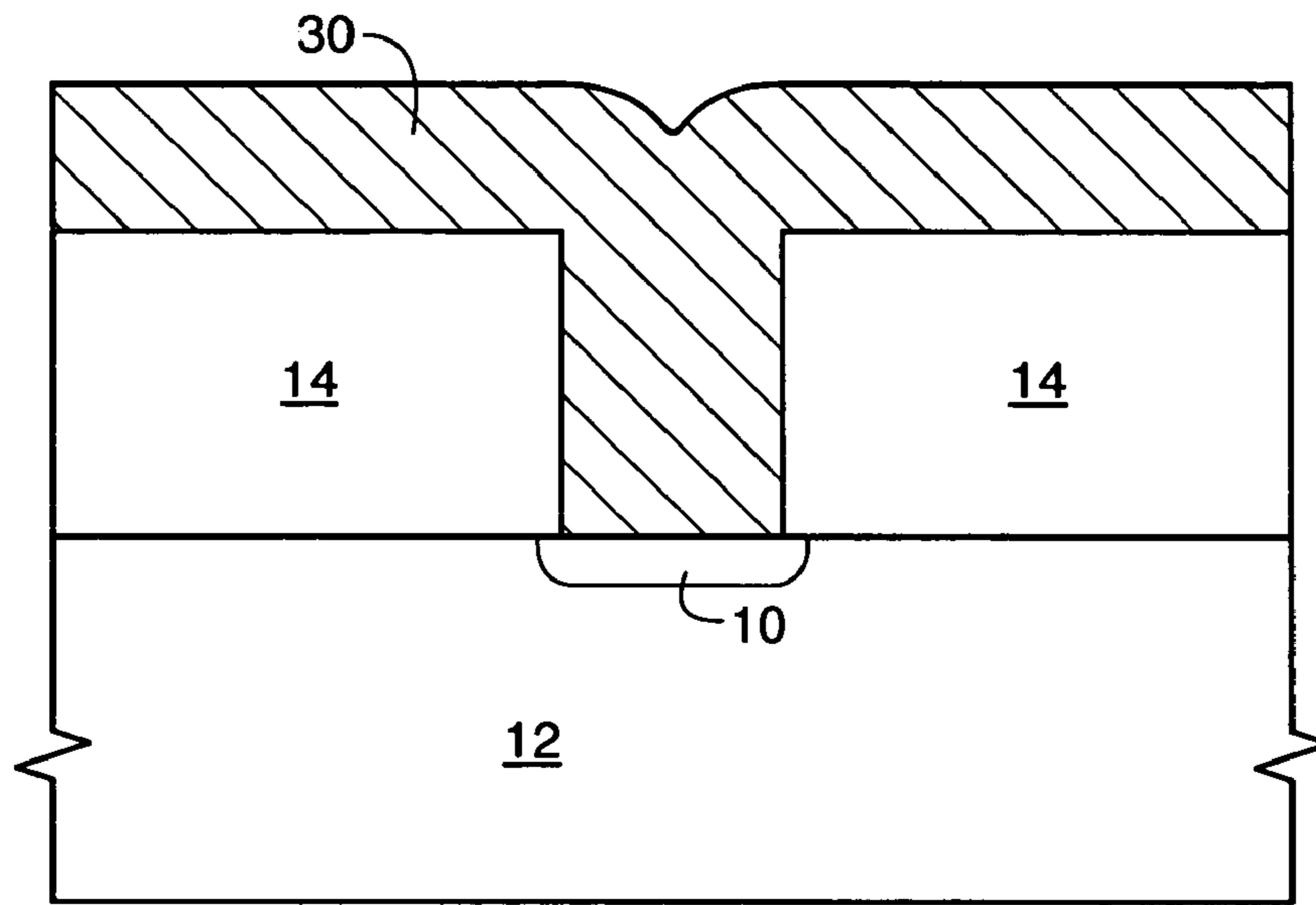
FIG. 3 (RELATED ART)
