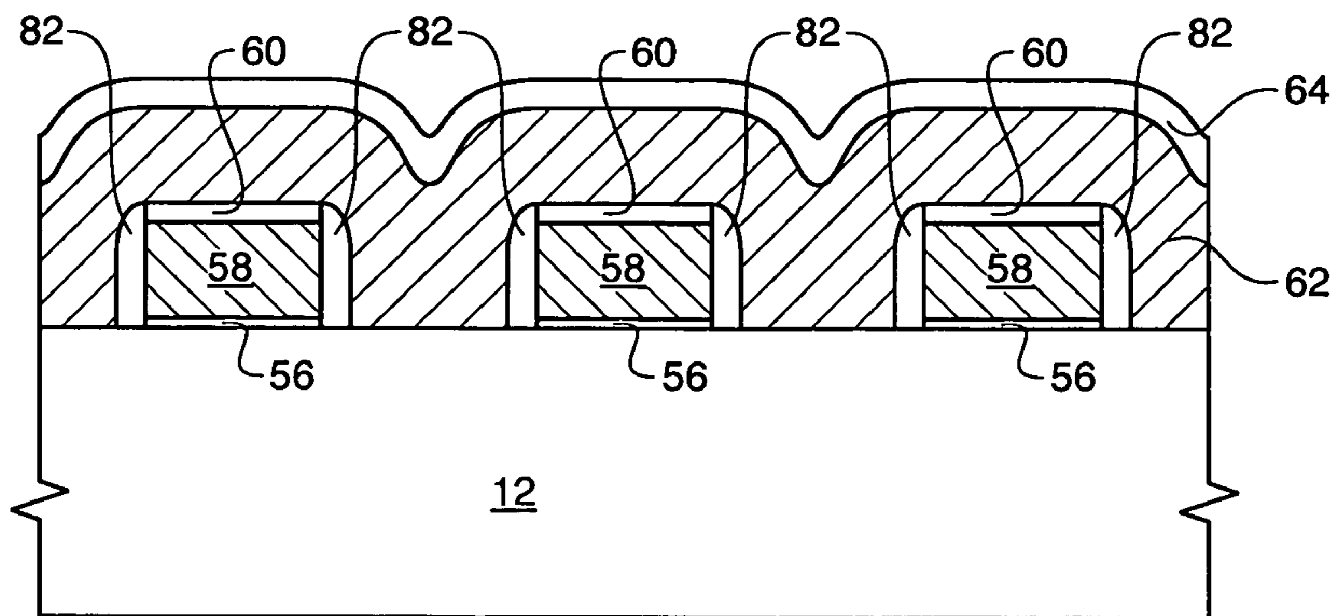
FIG. 7 (RELATED ART)
