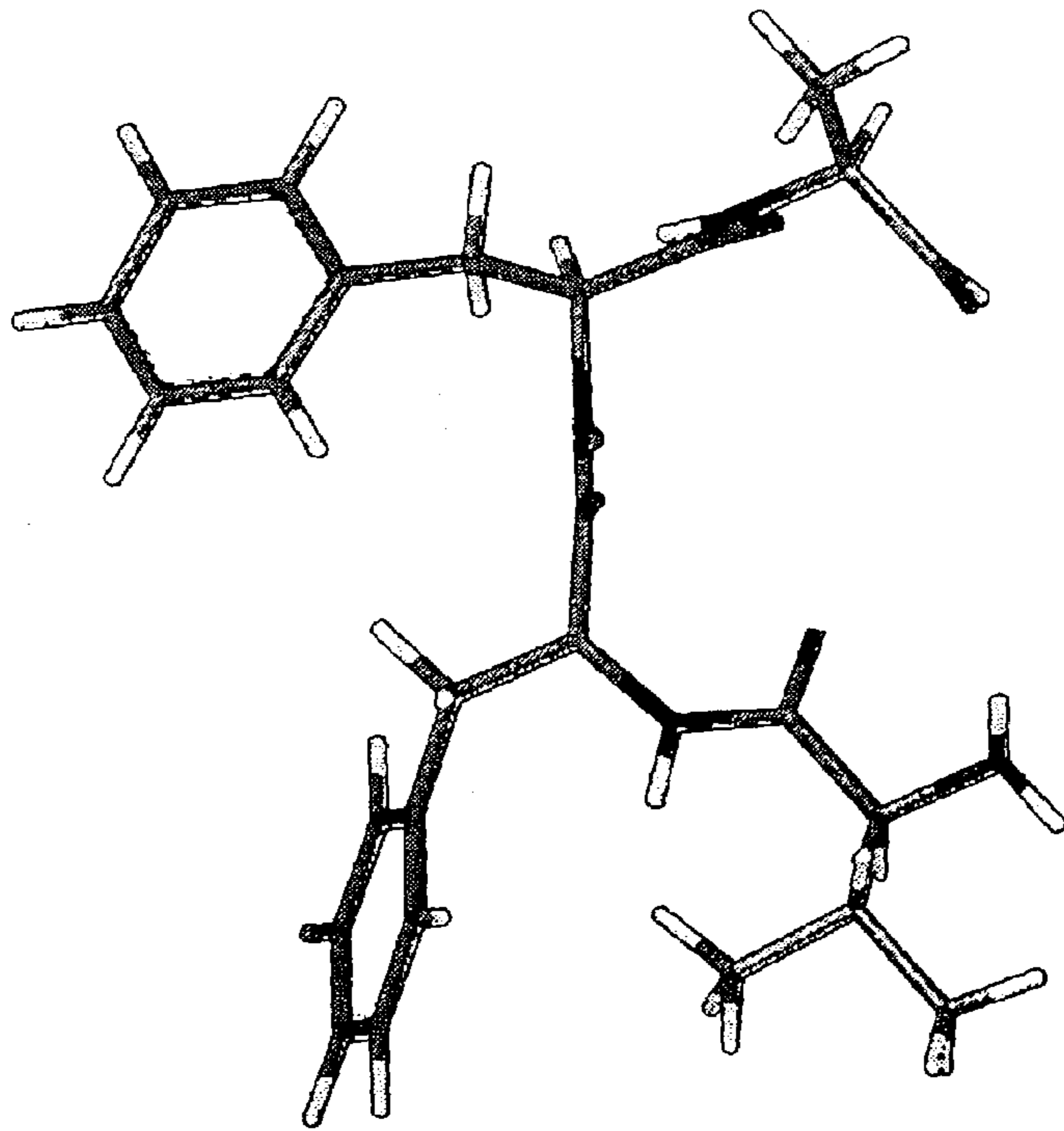
↑ Val-Phe-CO-NH-Phe-Ala
