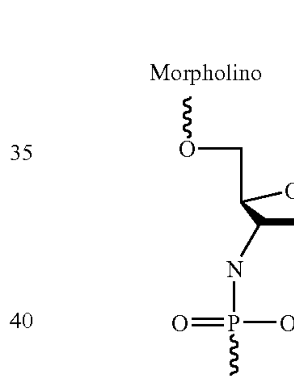
3'-Phosphoramidate
