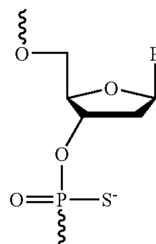
Phosphorothioate
