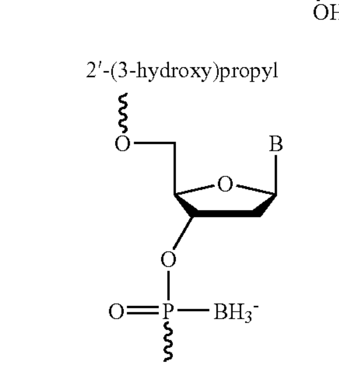
Boranophosphates
