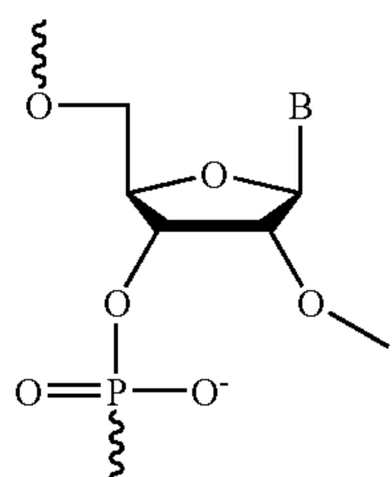
2'-O-Methyl
