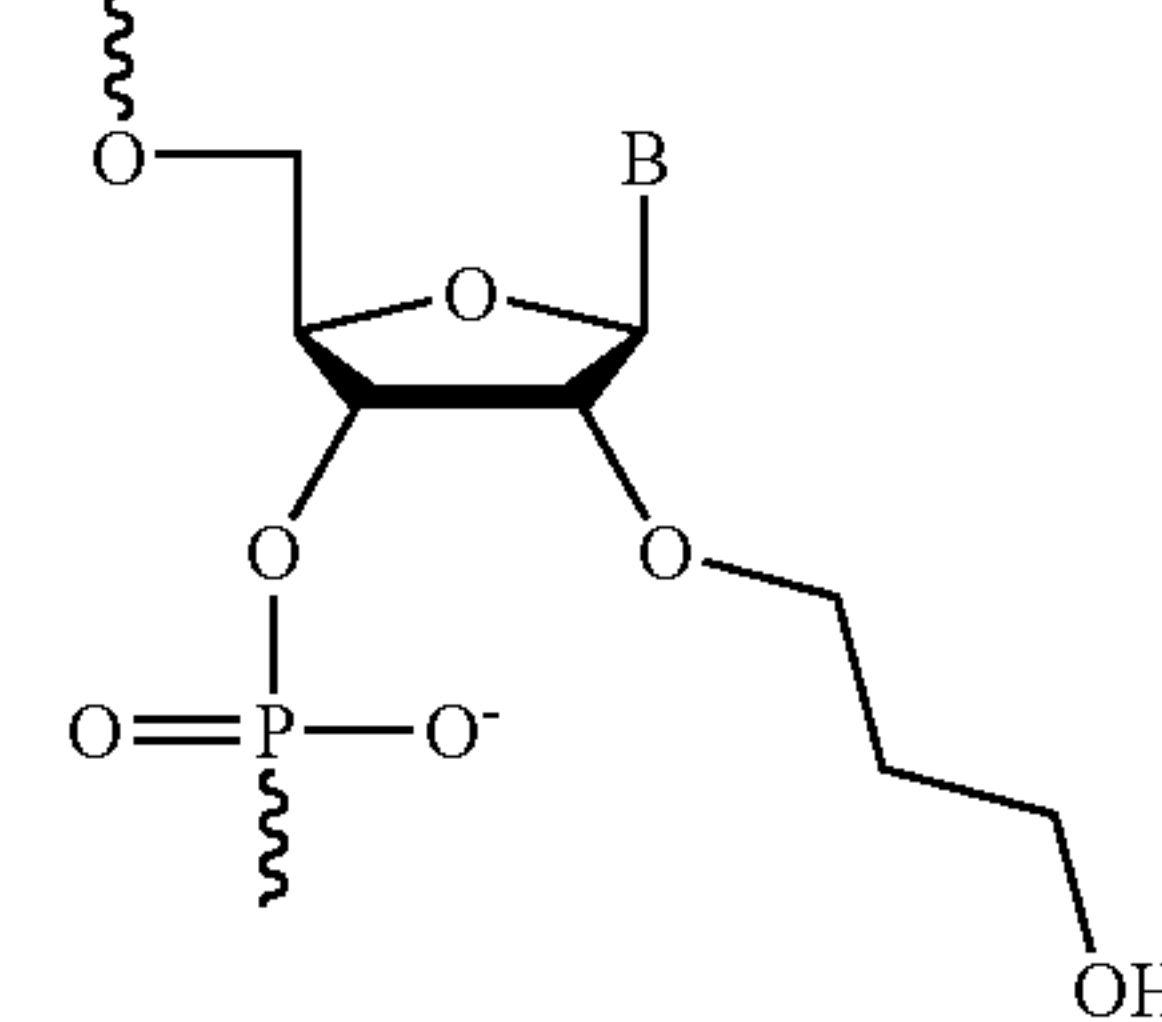
2'-(3-hydroxy)propyl
