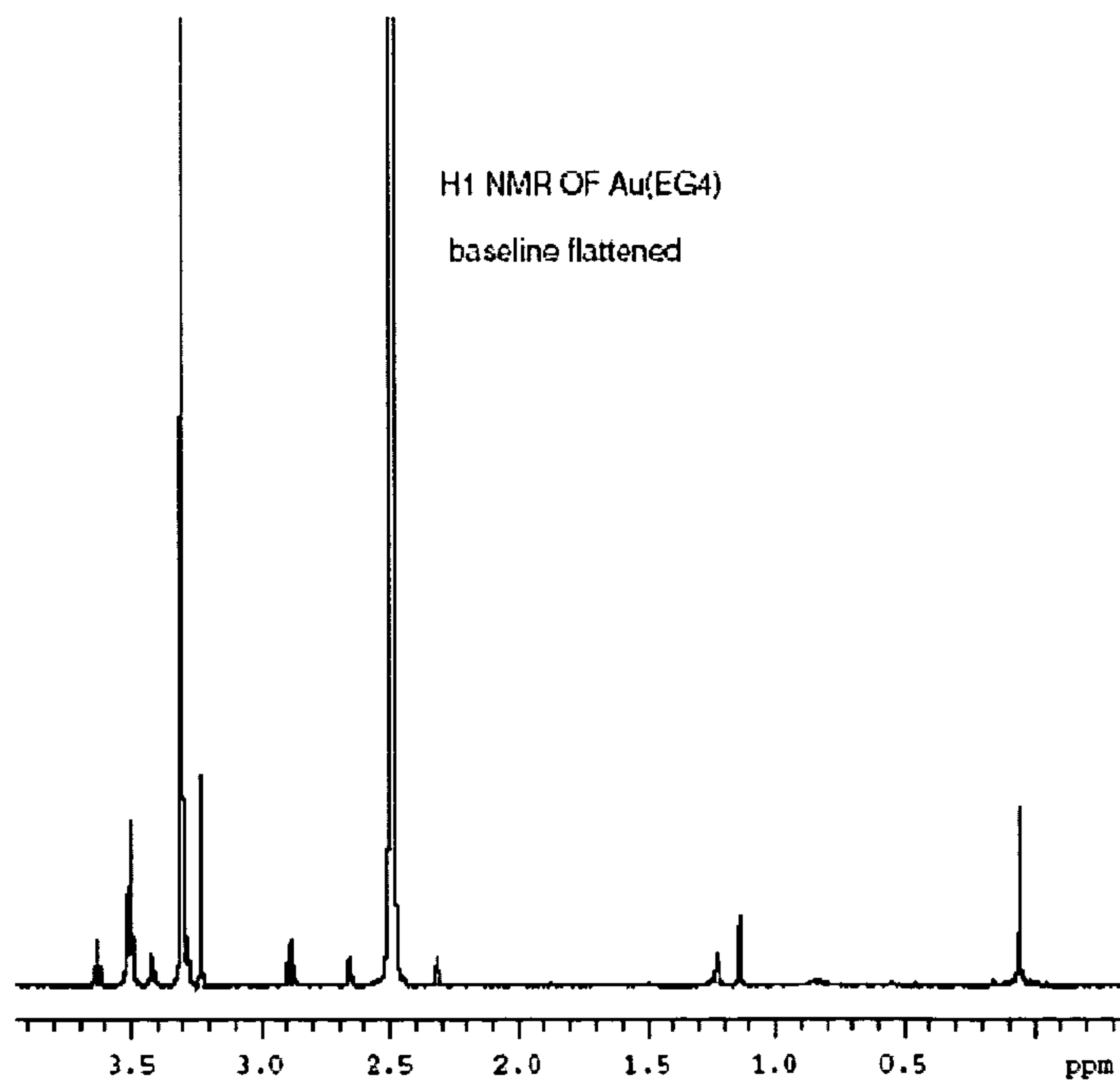
Figure 5b NMR spectra of Au-S-EG4 nanoparticle
