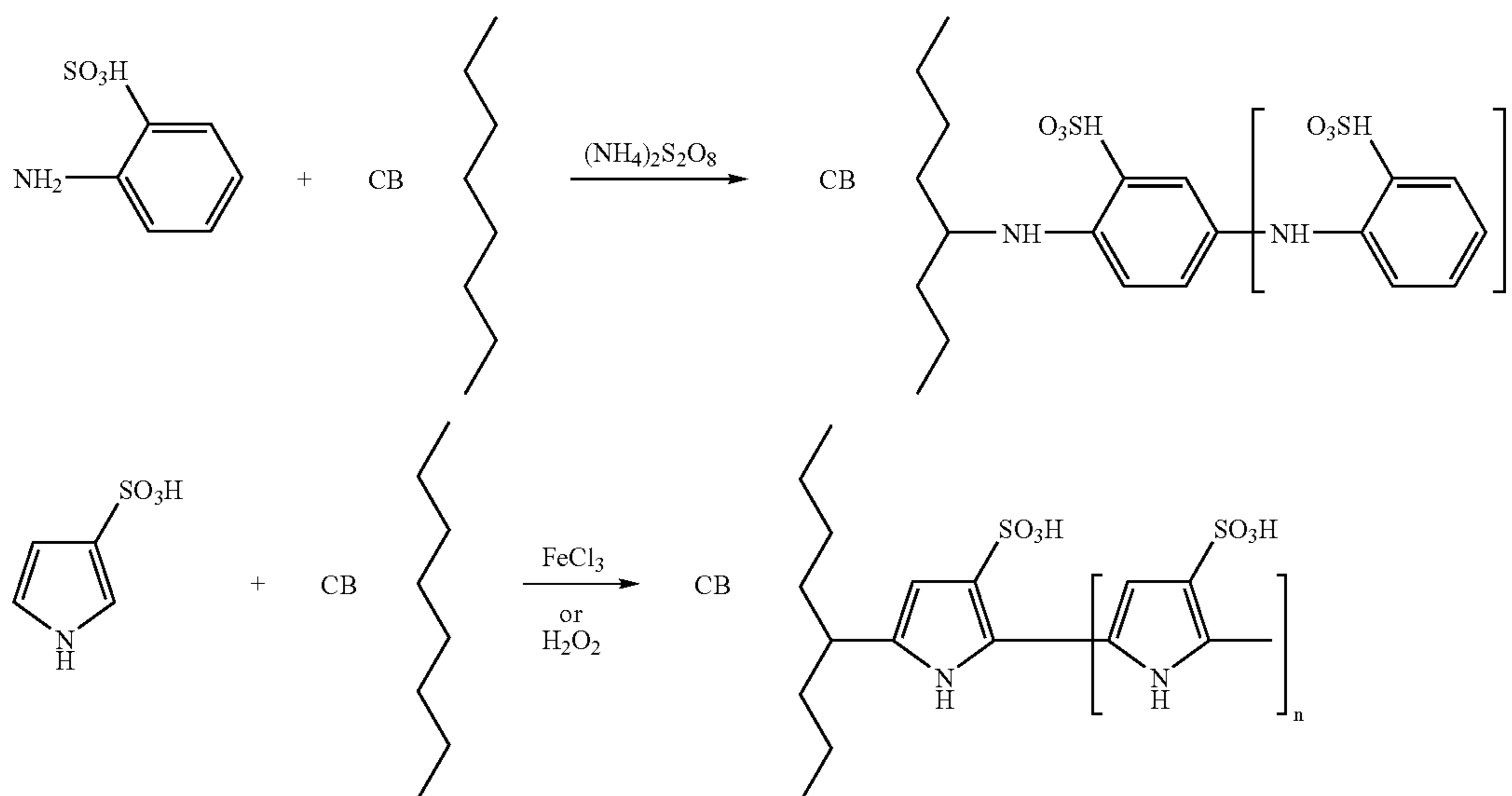
Scheme II
