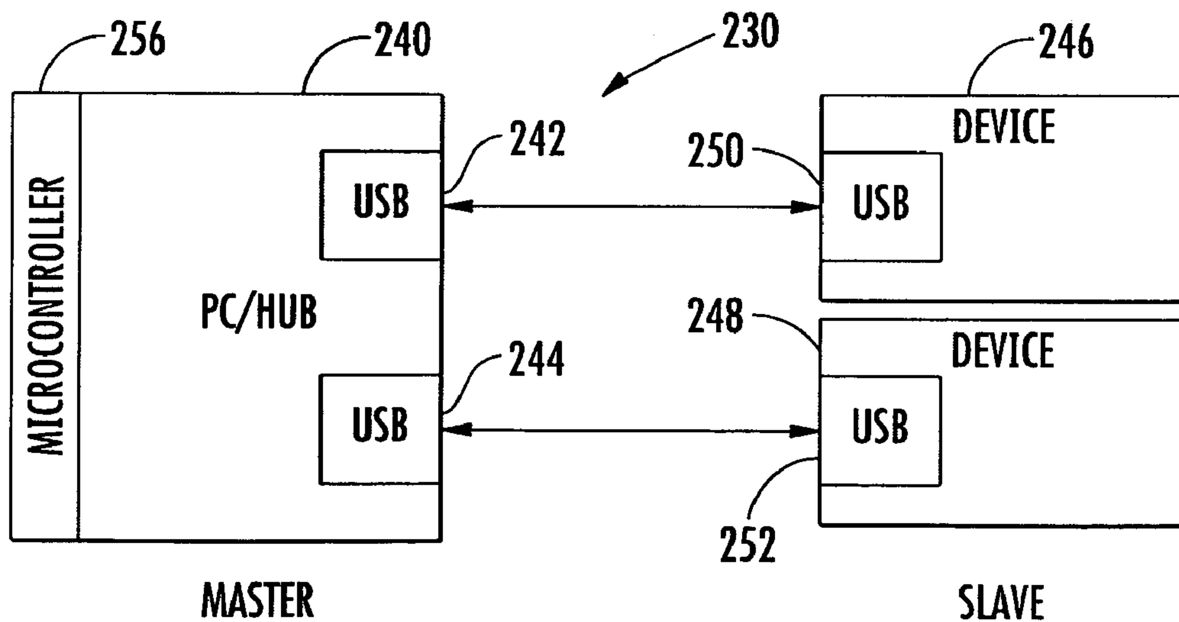
FIG. 5 (PRIOR ART)
