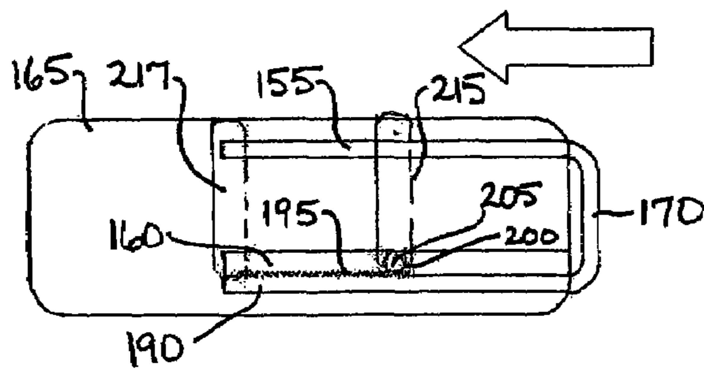
RAIL DOWN
