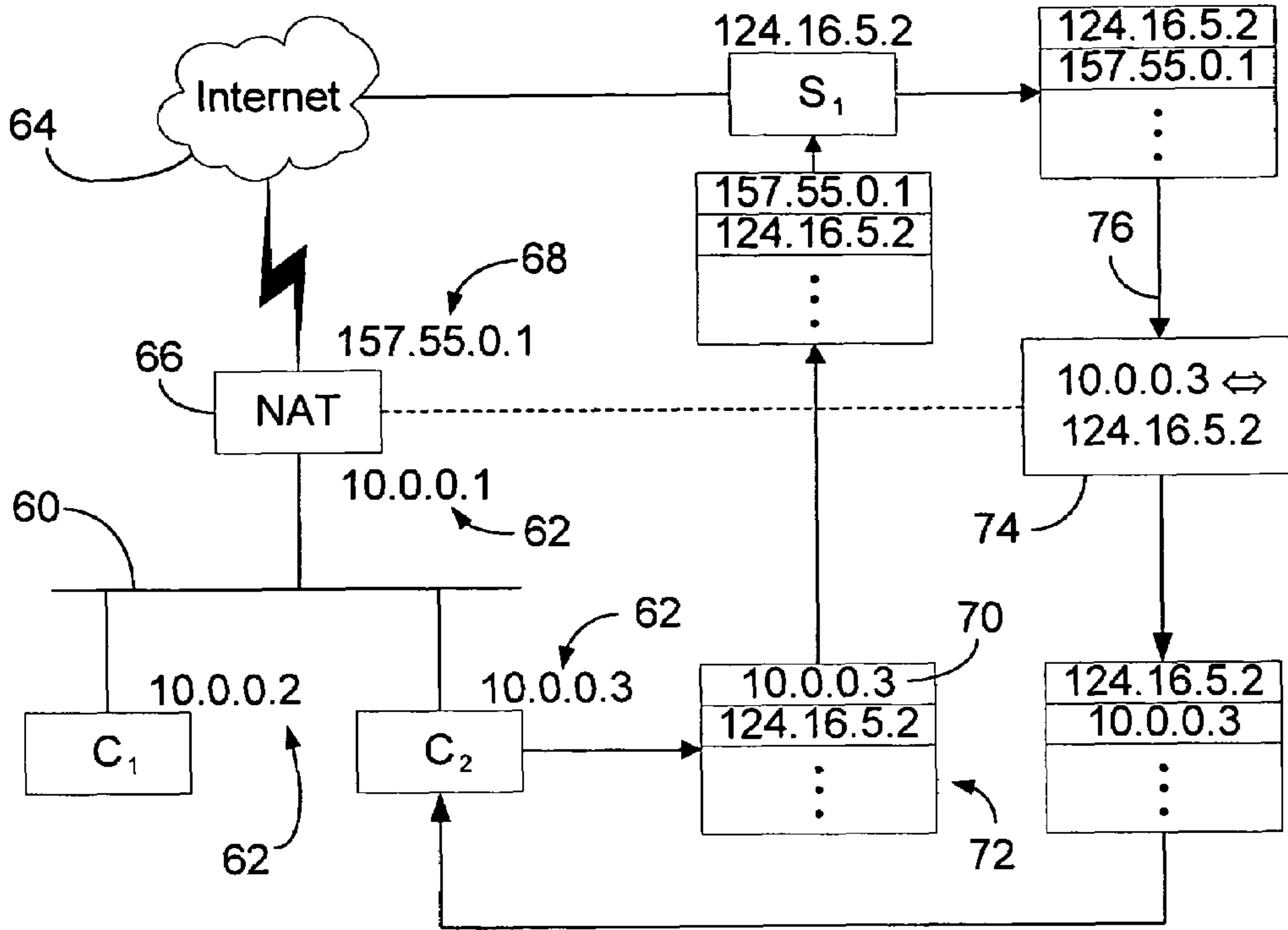
FIG. 2 (PRIOR ART)
