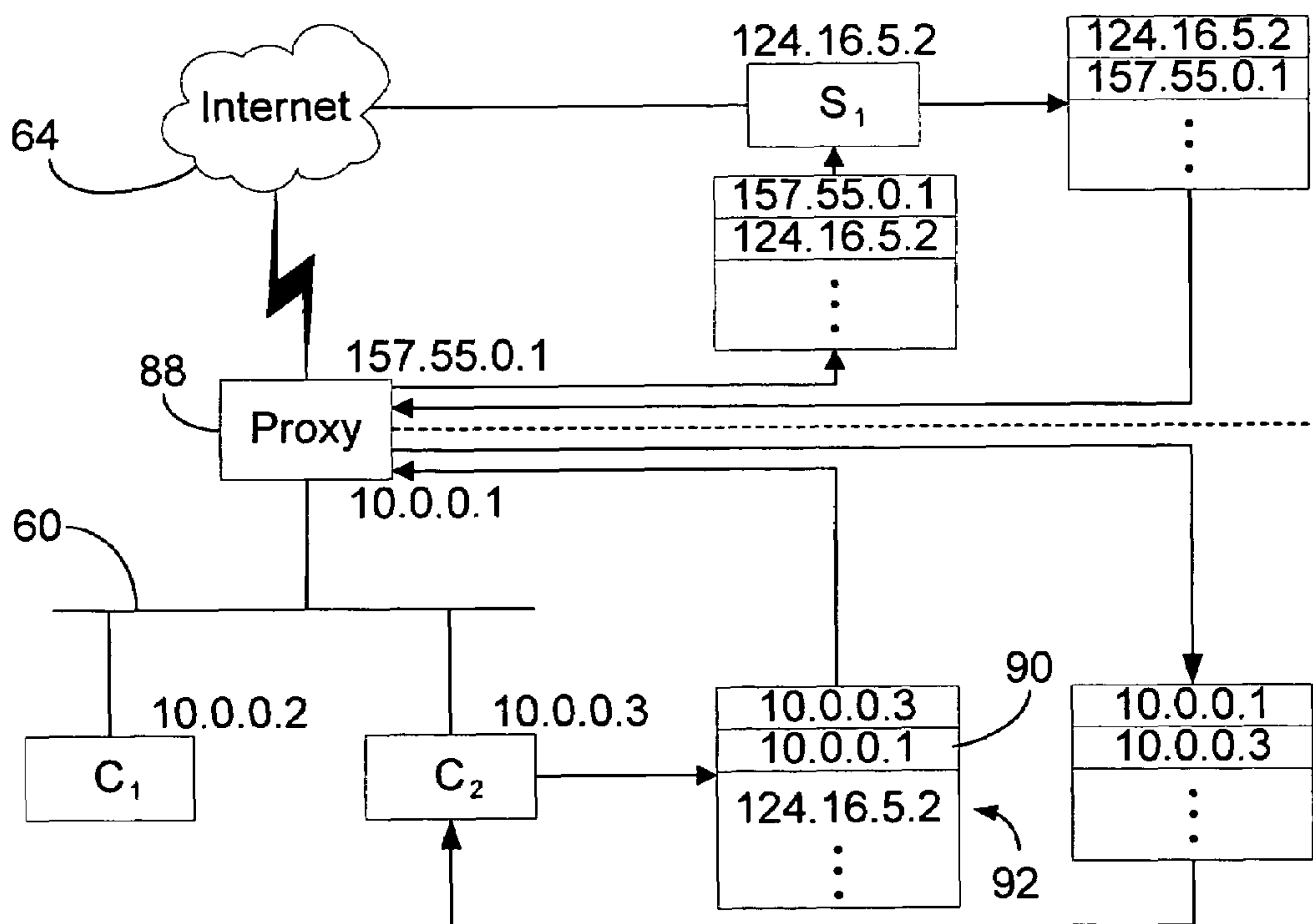
FIG. 6 (PRIOR ART)
