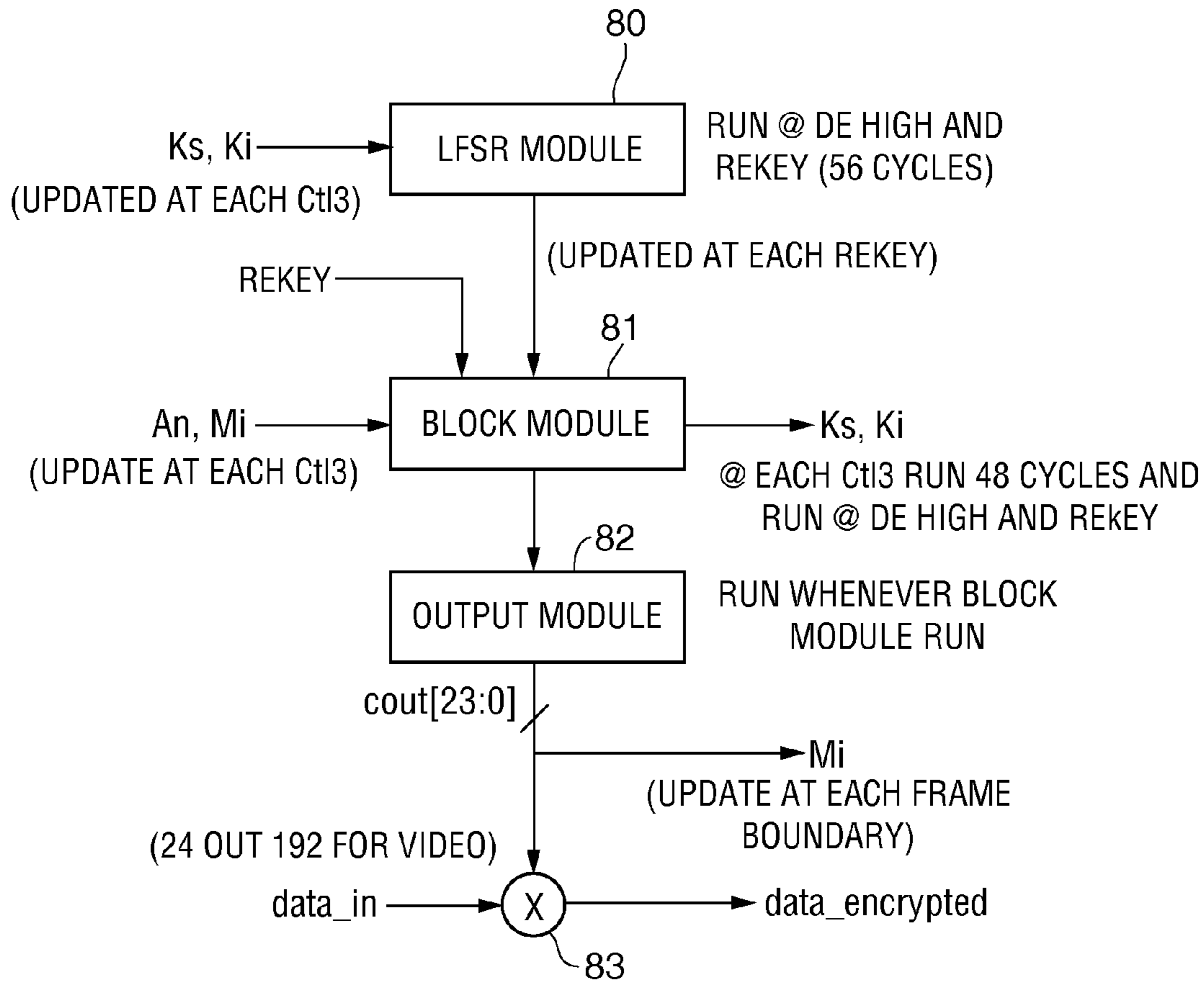
FIG. 3 (PRIOR ART)
