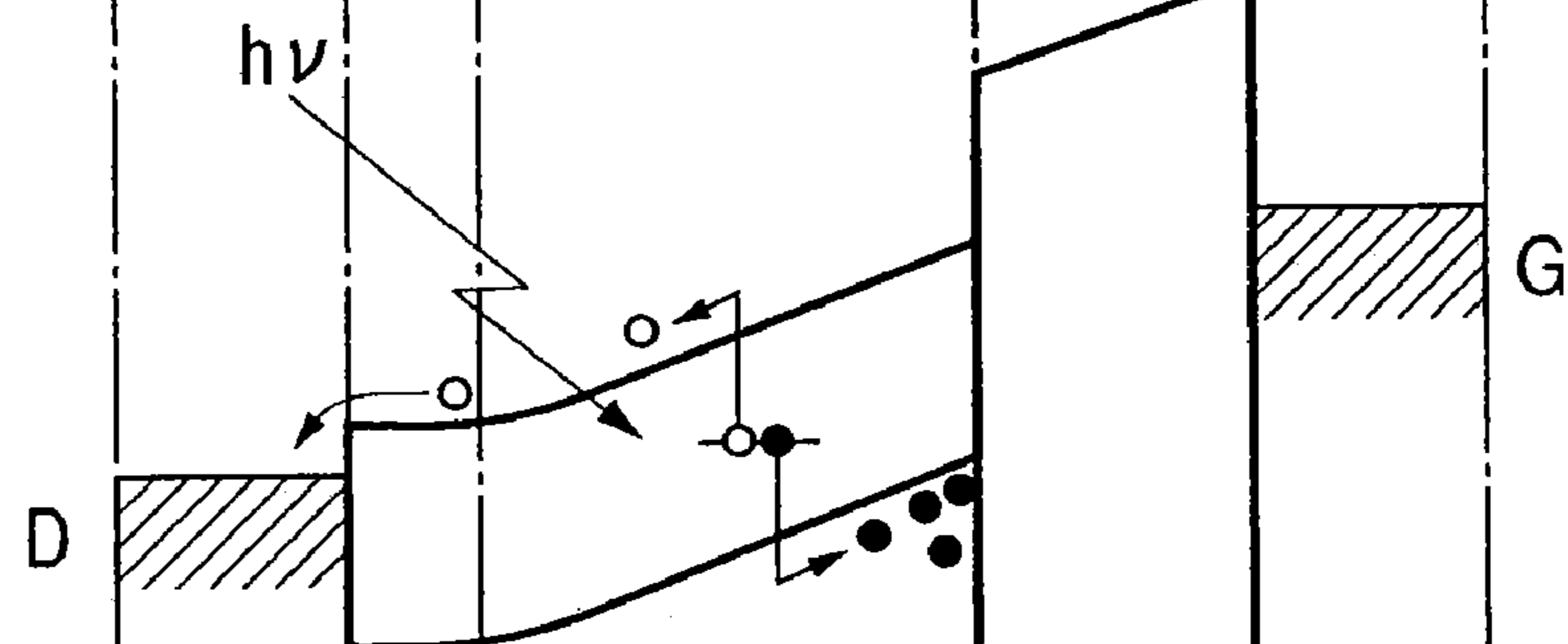
FIG. 6B PHOTOELECTRIC CONVERSION MODE
