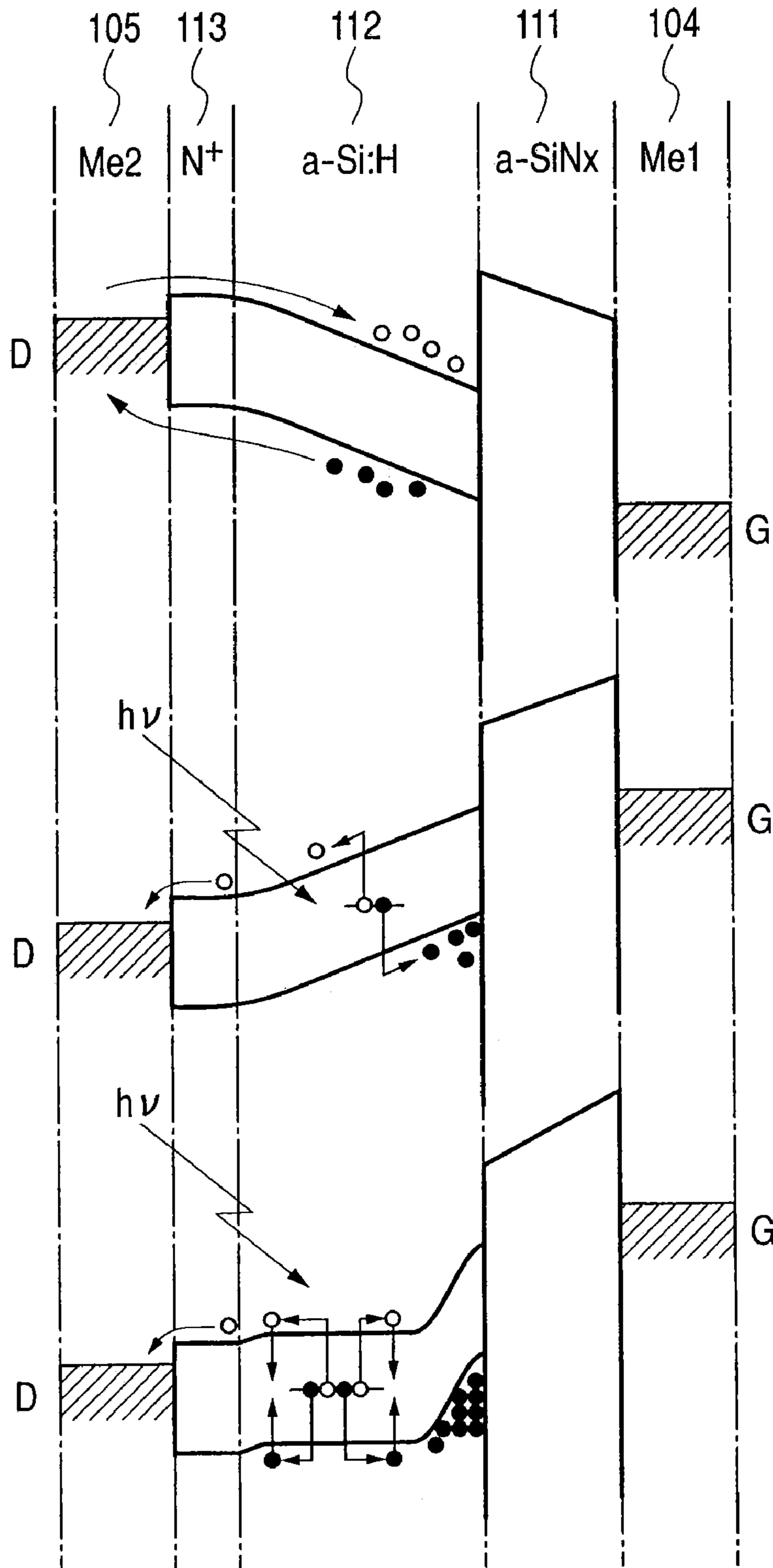
FIG. 6B PHOTOELECTRIC CONVERSION MODE
