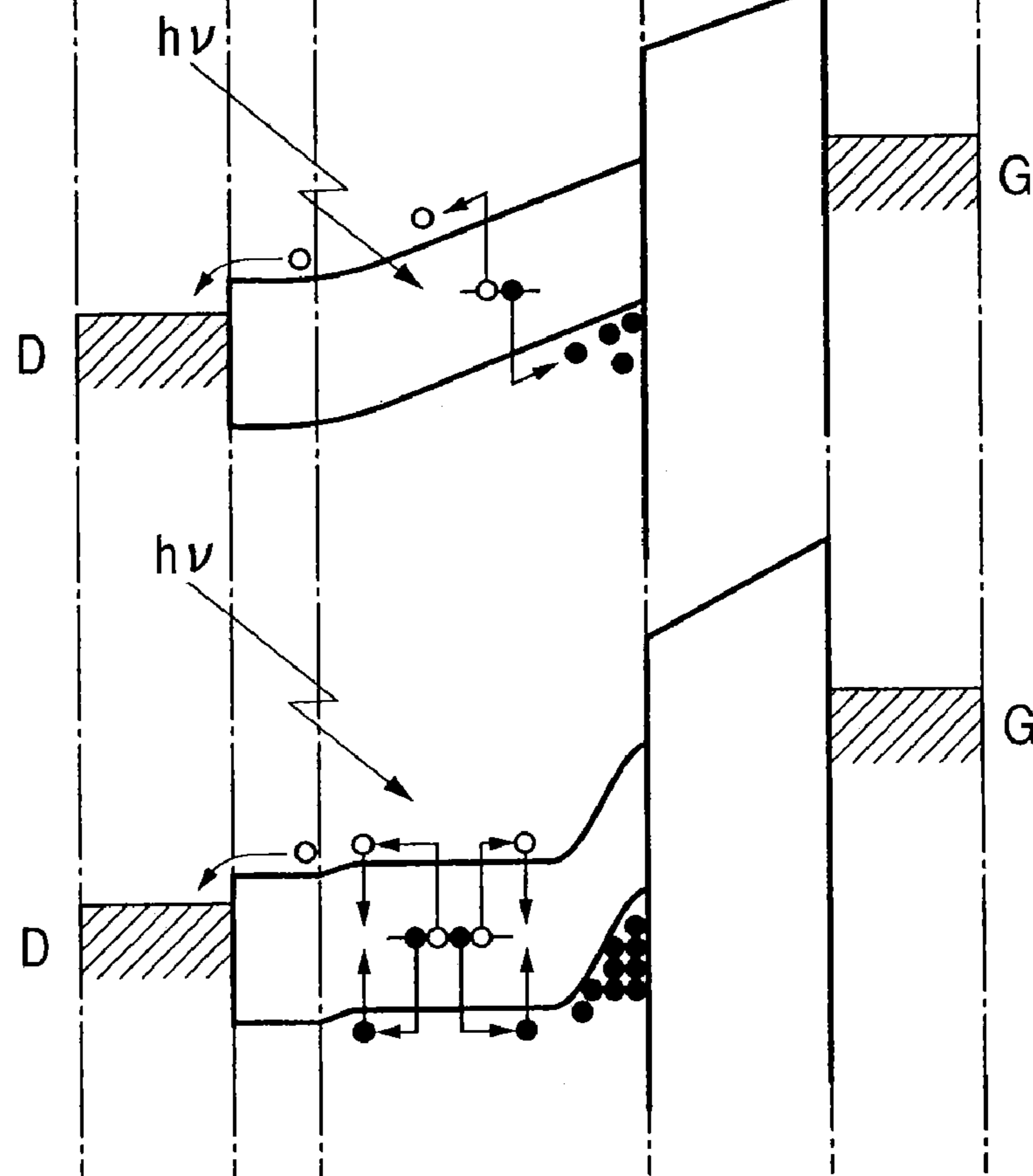
FIG. 6B PHOTOELECTRIC CONVERSION MODE
