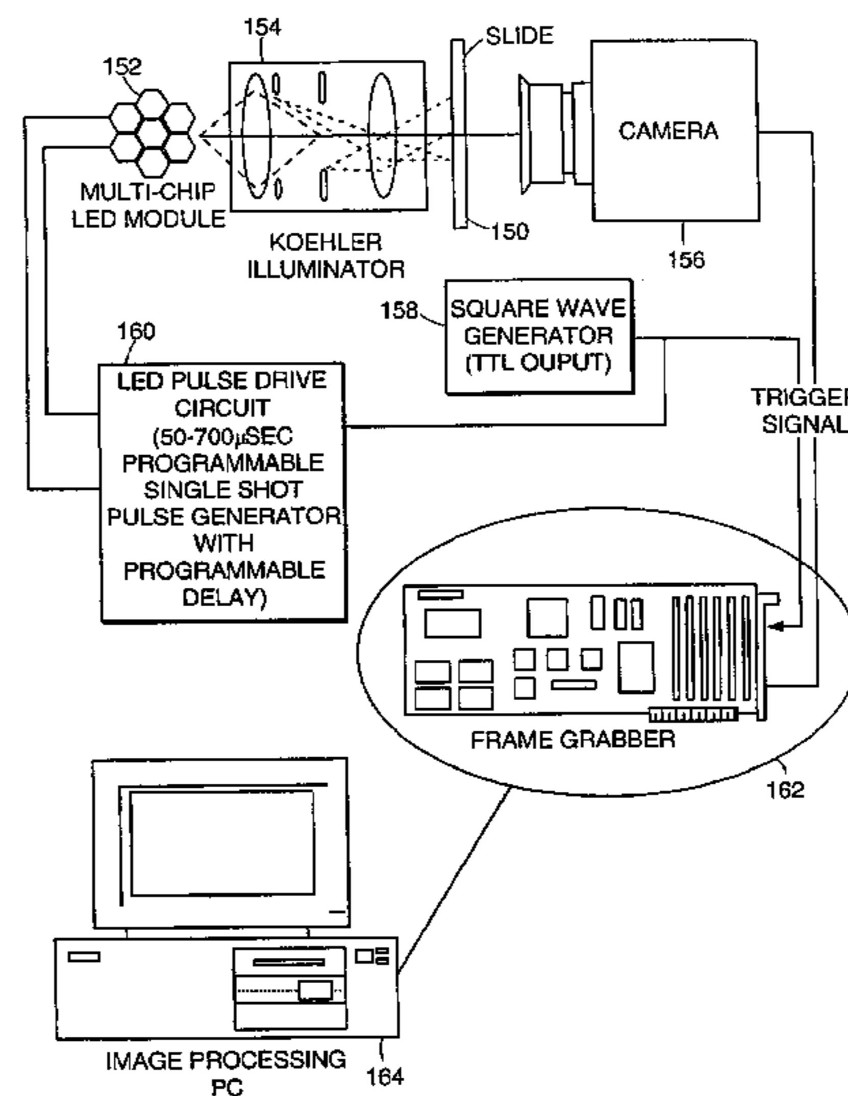
LED KOEHLER ILLUMINATION SYSTEM
