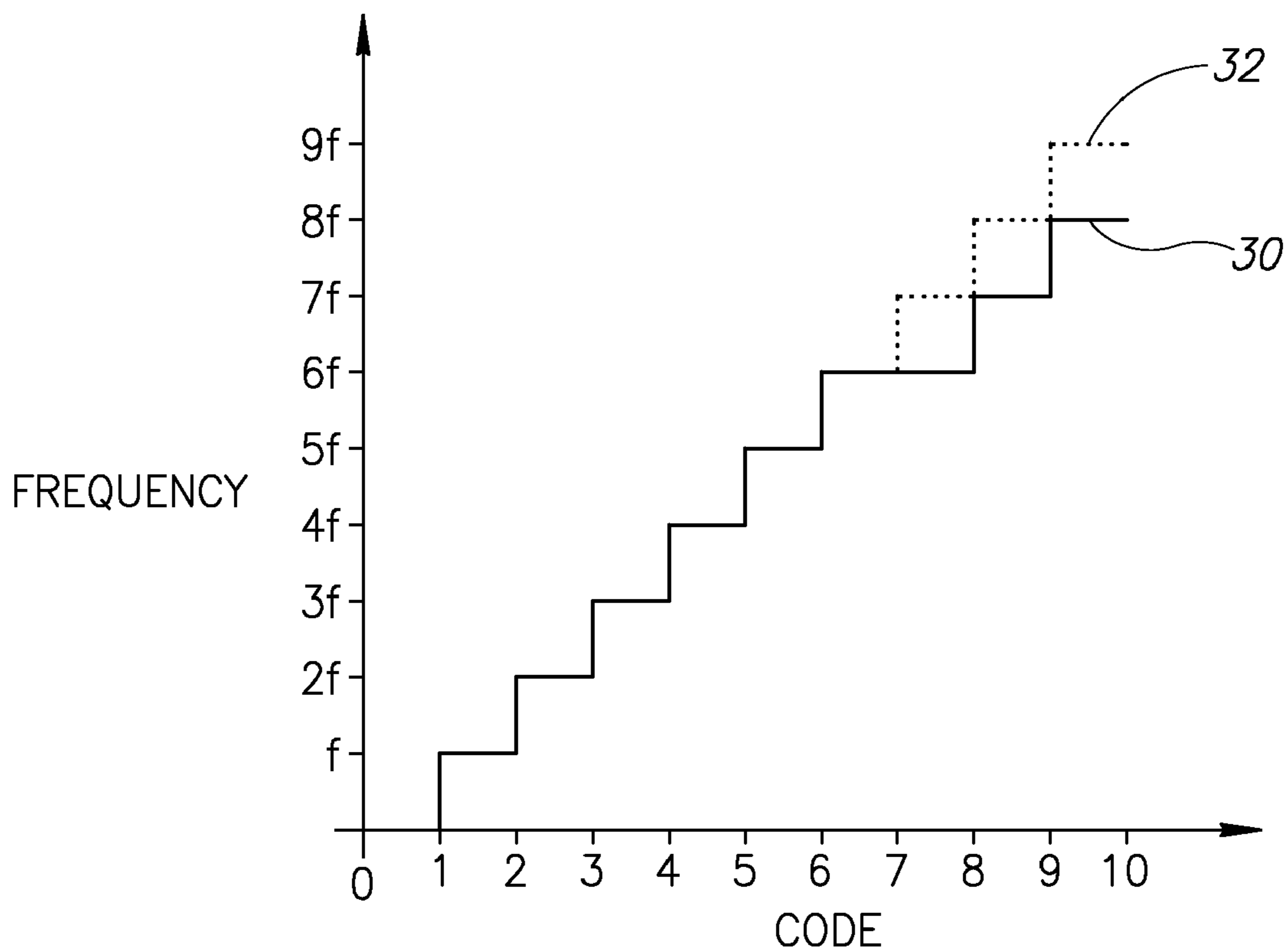
FIG.2 PRIOR ART
