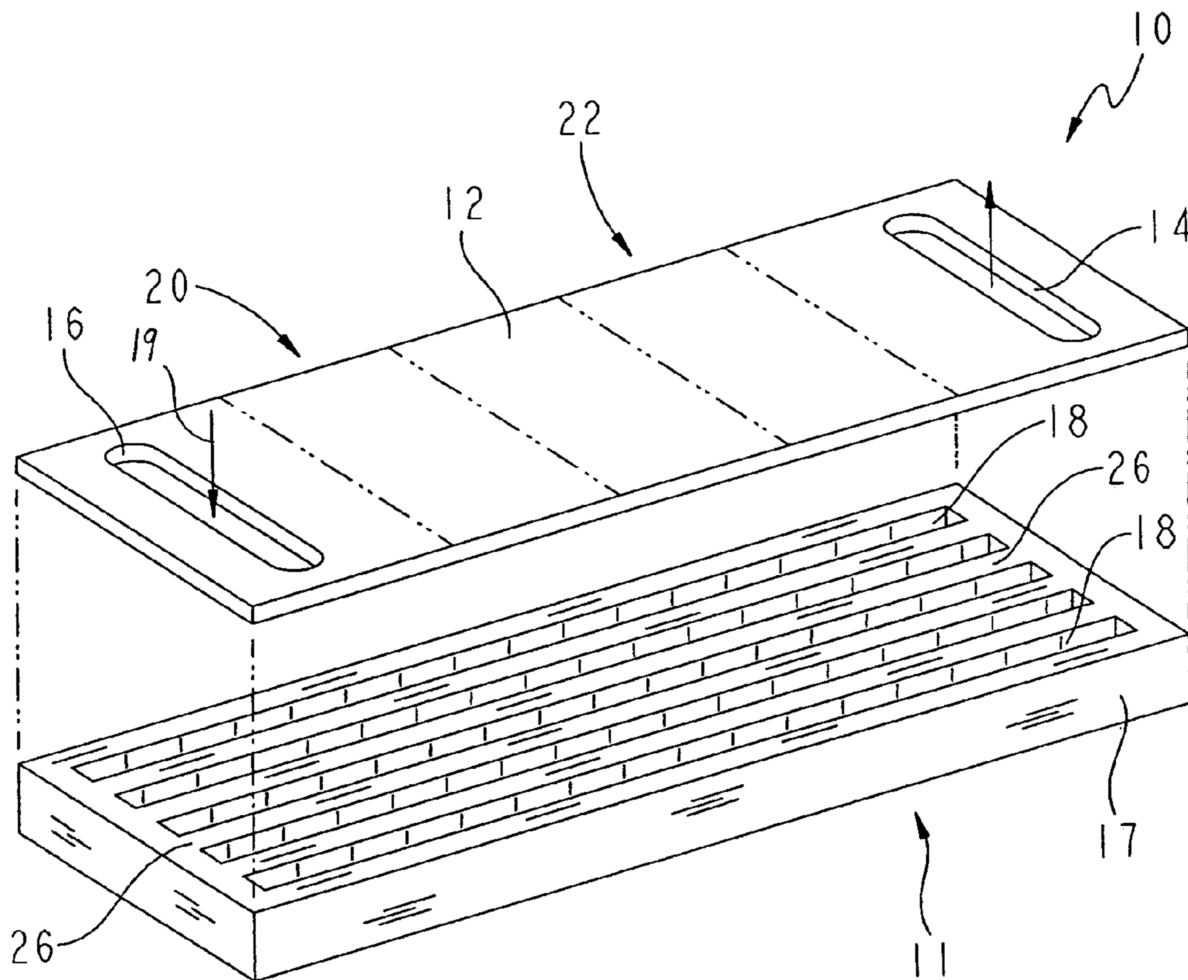
FIG. 1 (Prior Art)
