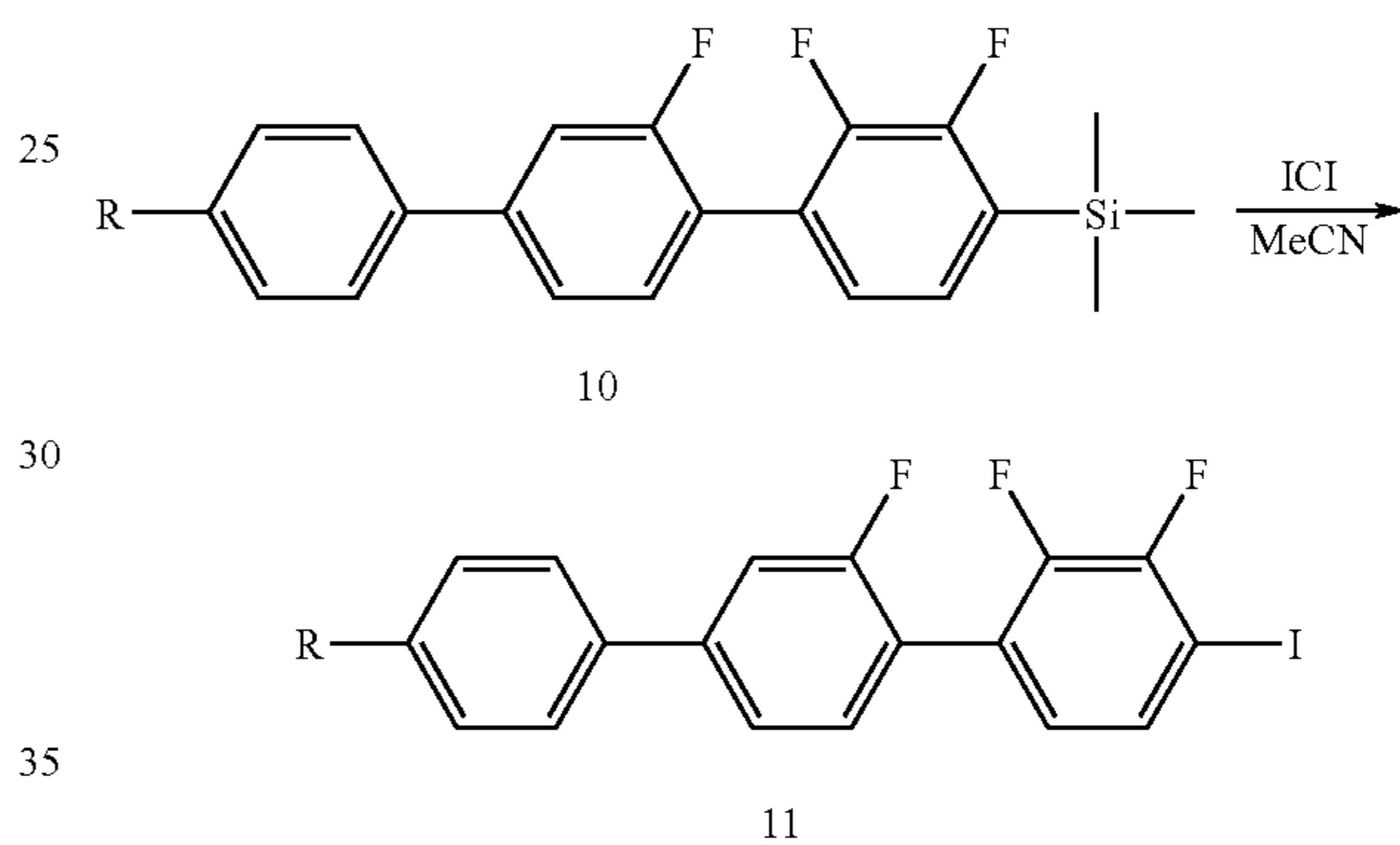
Scheme 3
