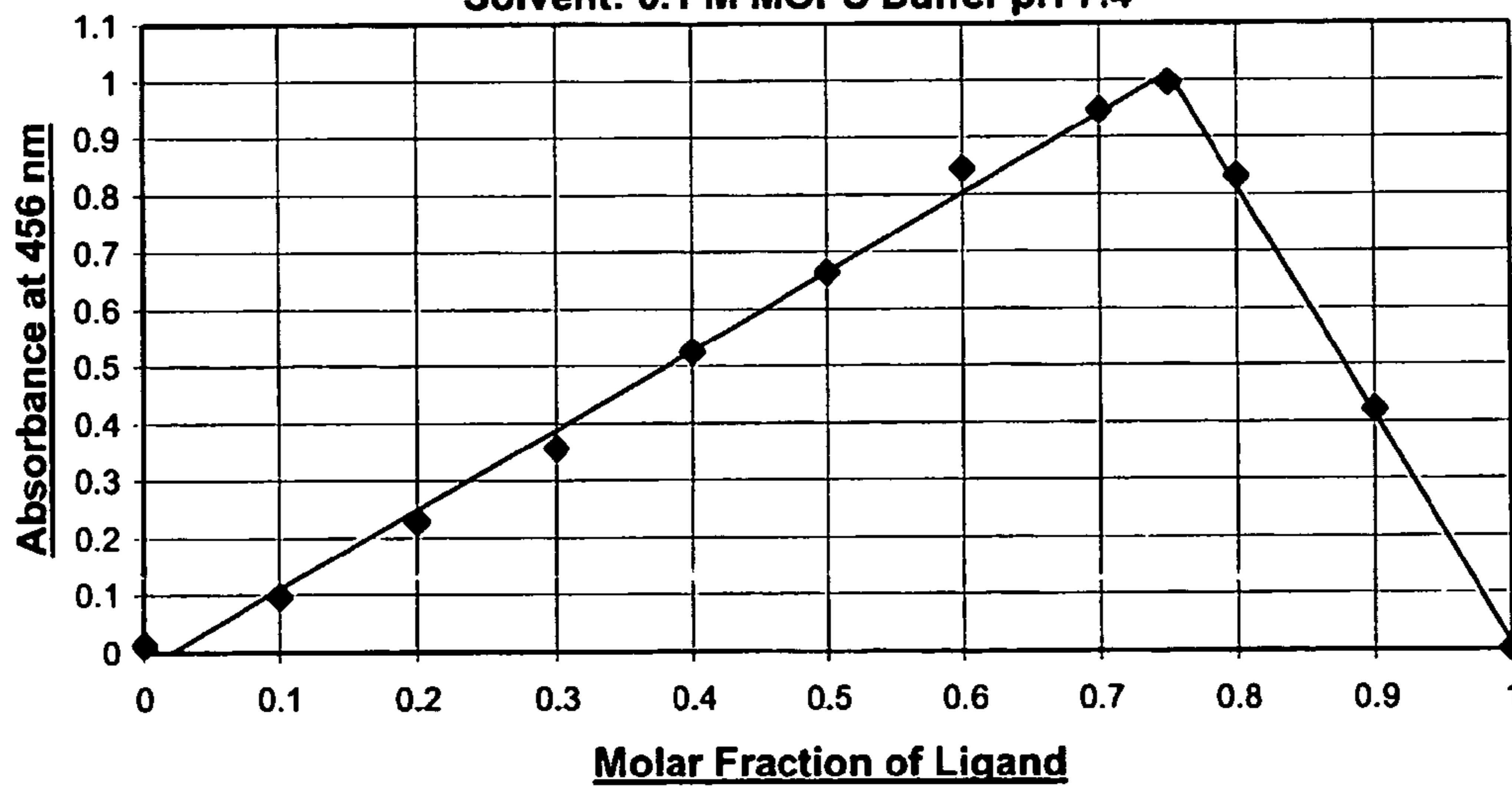
Figure 2: Job's Plot for Apo6617 [Fe^{3+}]_{total} + [Apo6617]_{total} = 8 \times 10^{-4} \text{ M} Solvent: 0.1 M MOPS Buffer pH 7.4
