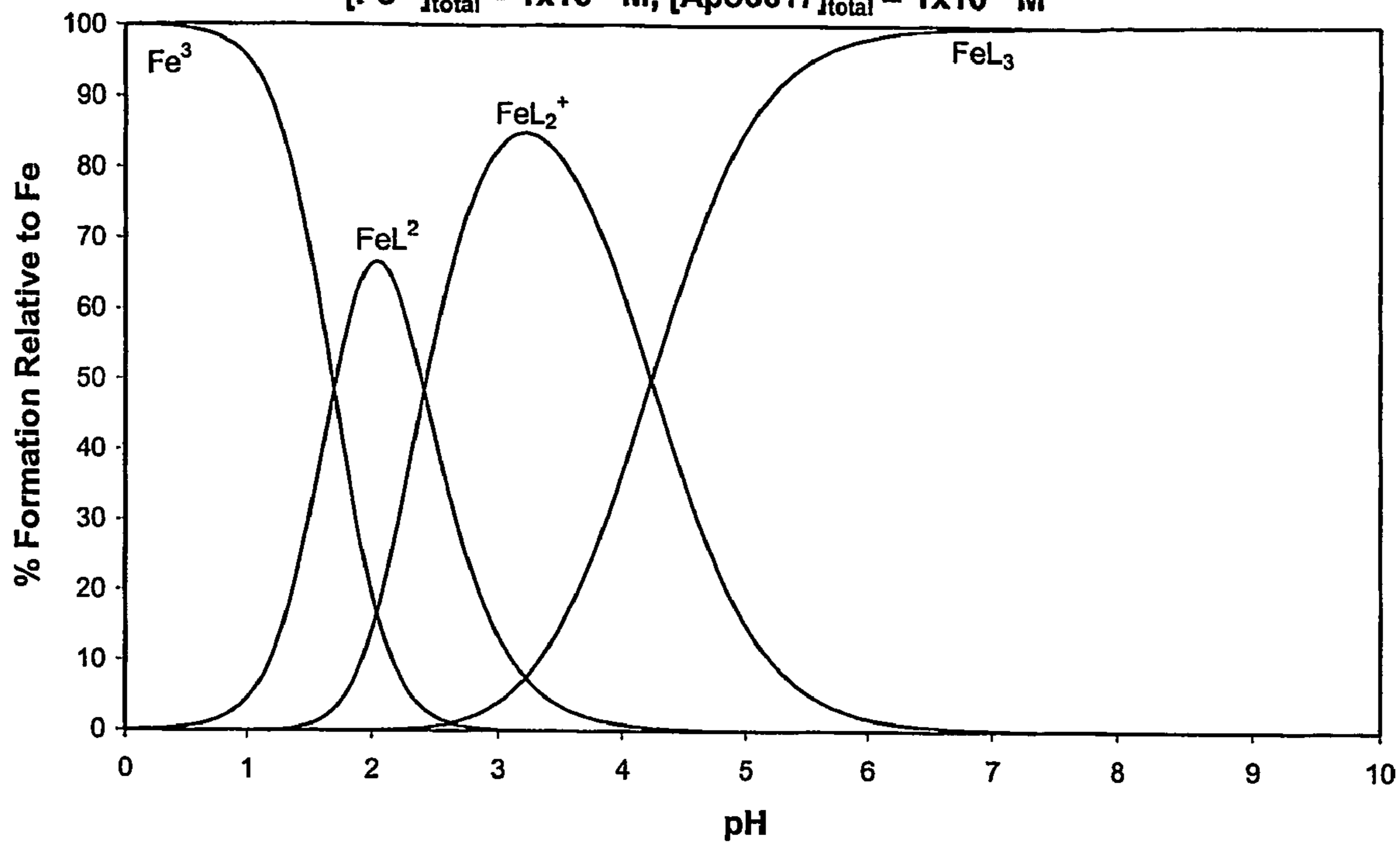
Figure 5: Speciation Plot for Fe 3+ -Apo6617 [Fe 3+ ] total = 1x10 -6 M, [Apo6617] total = 1x10 -5 M
