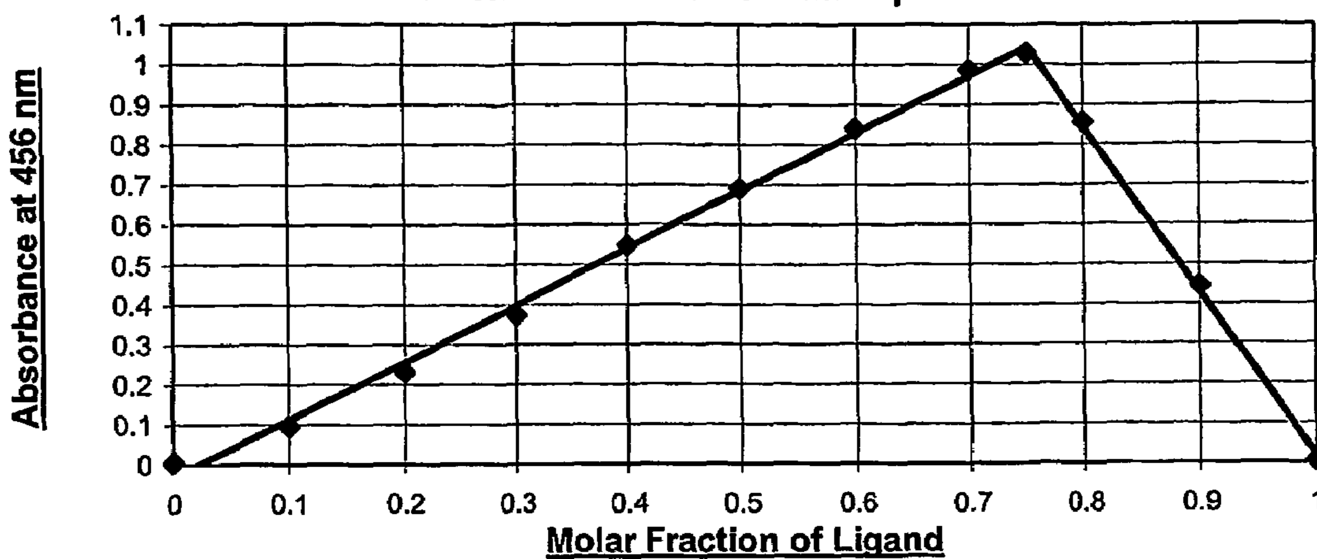
Figure 3: Job's Plot for Apo6619 [\text{Fe}^{3+}]_{\text{total}} + [\text{Apo6619}]_{\text{total}} = 8 \times 10^{-4} Solvent: 0.1 M MOPS Buffer pH 7.4
