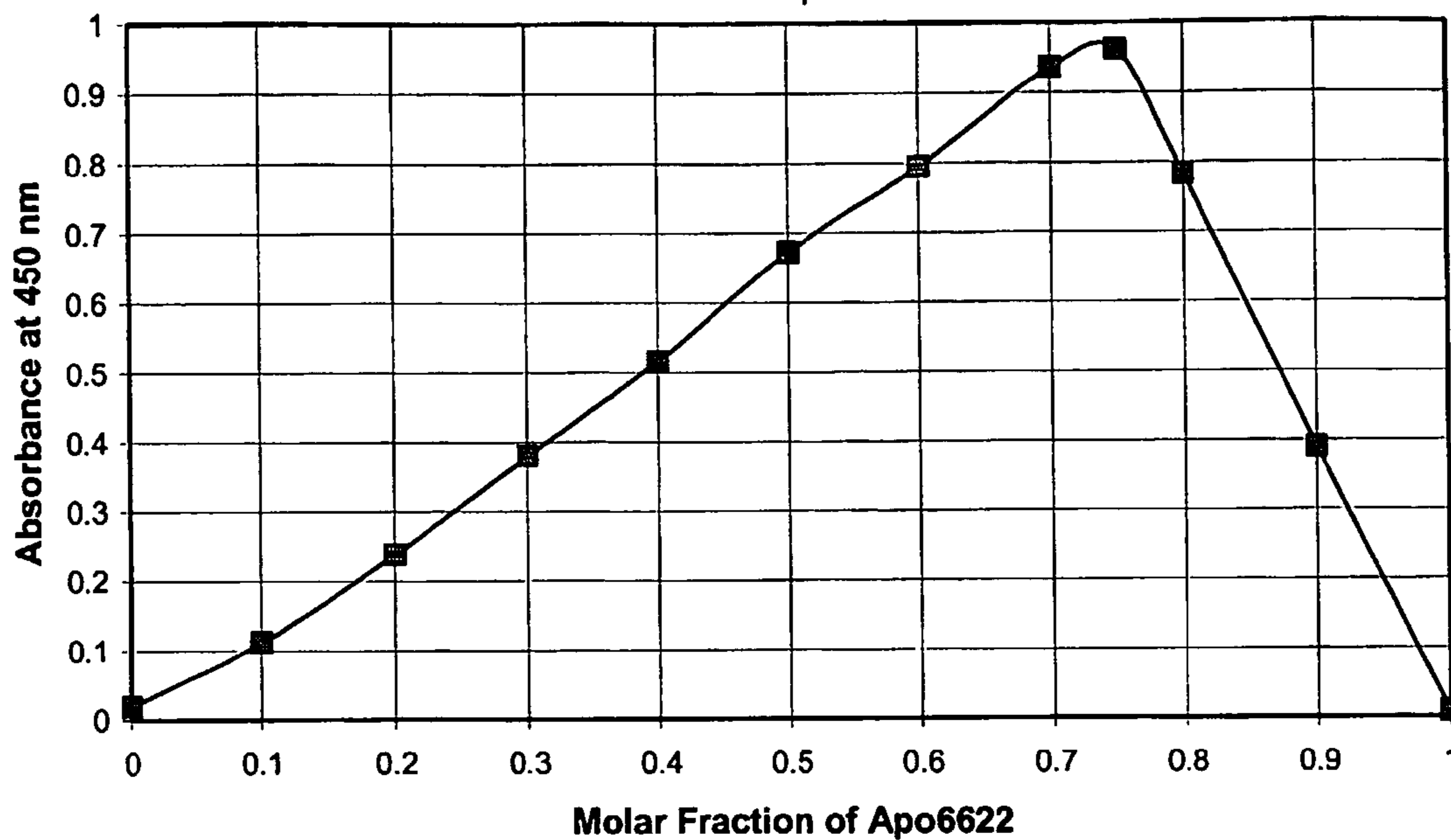
Figure 1: Job's Plot for Apo6622 [Fe^{3+}]_{total} + [Apo6622]_{total} = \text{Constant} = 8 \times 10^{-4} \text{ M} Solvent: 0.1 M MOPS pH=7.4 Buffer
