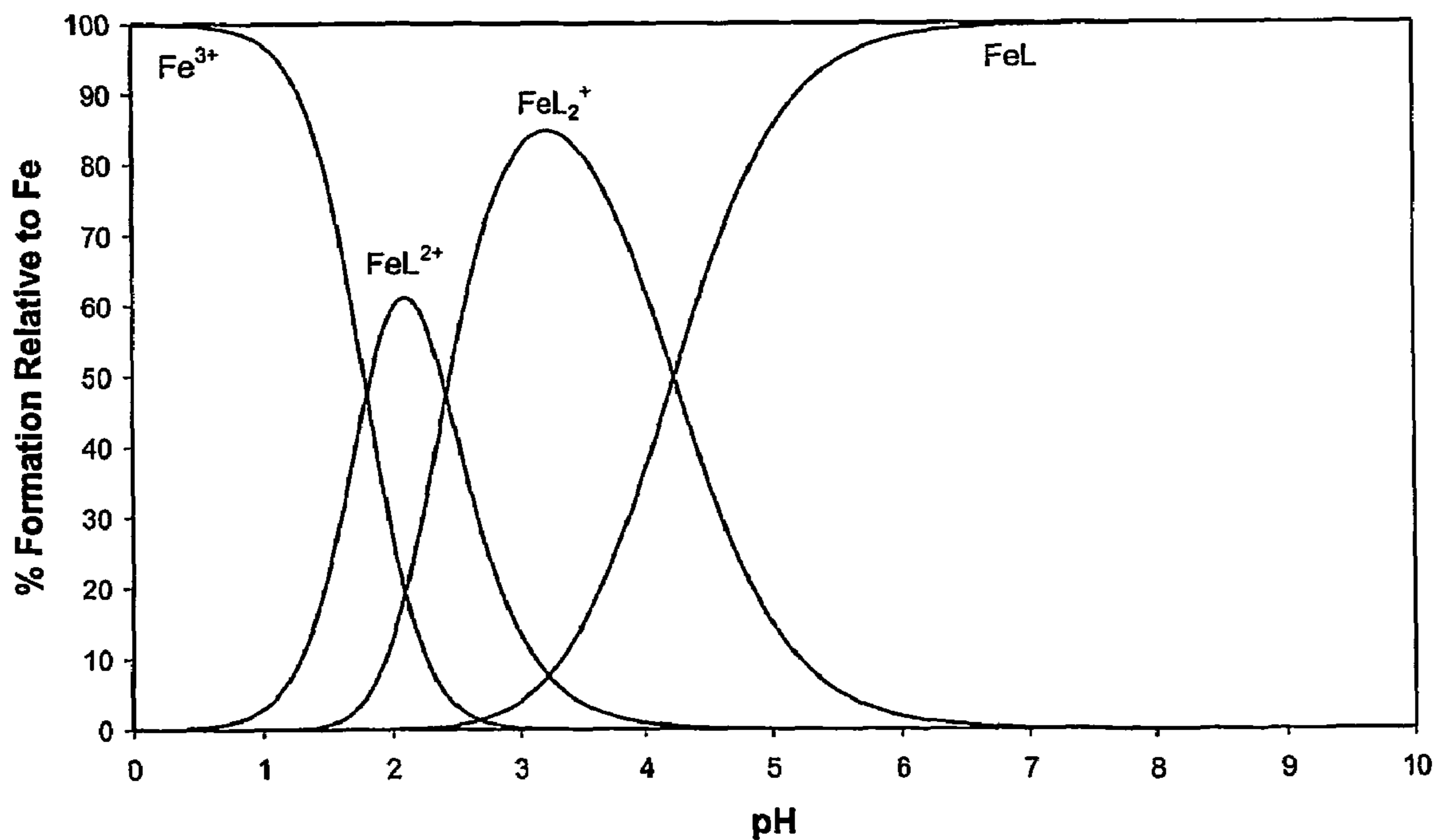
Figure 4: Speciation Plot for Fe 3+ -Apo6619 [\text{Fe}^{3+}]_{\text{total}} = 1 \times 10^{-6} \text{ M} , [\text{Apo6619}]_{\text{total}} = 1 \times 10^{-5} \text{ M}
