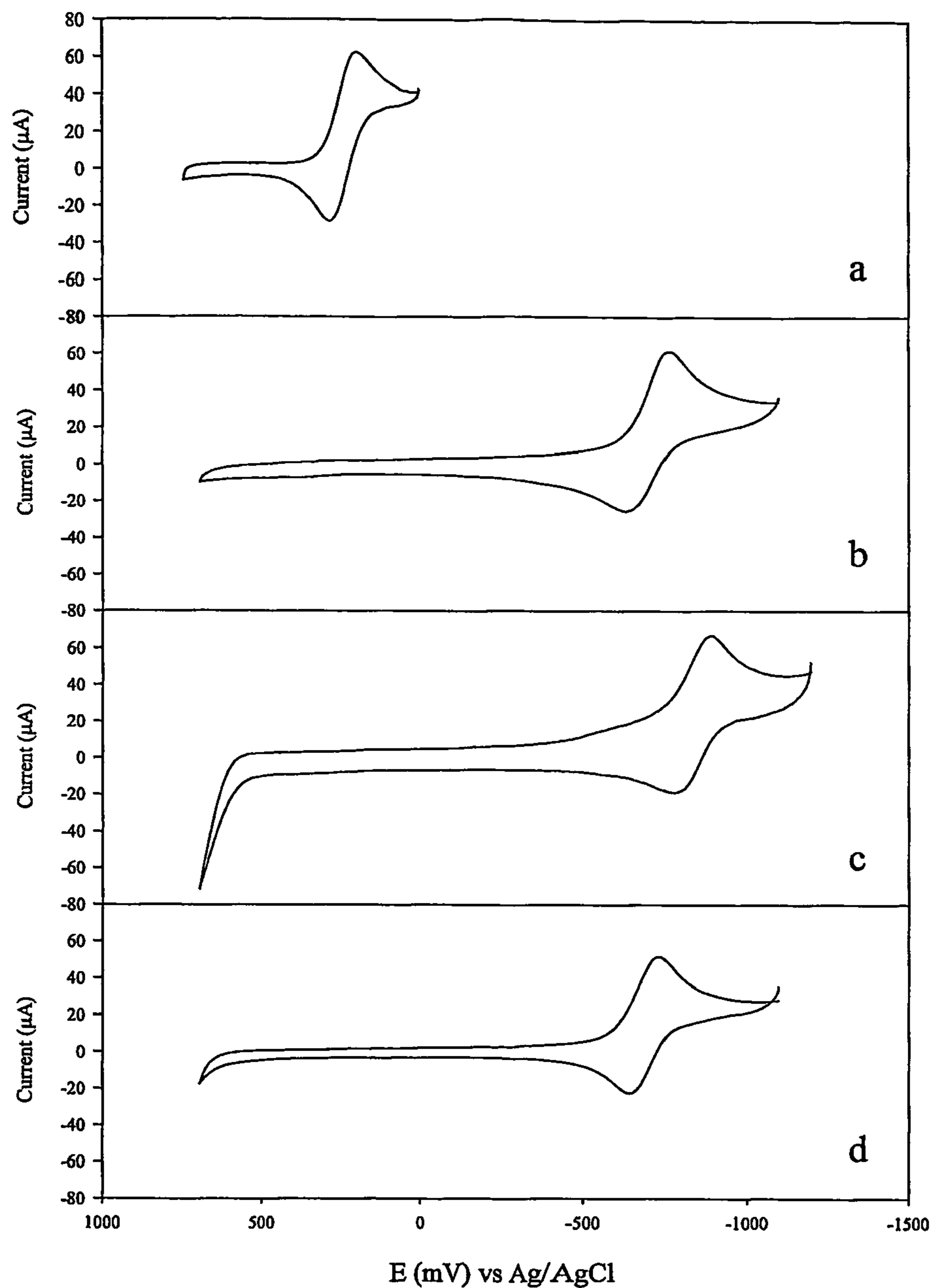
FIG. 9 Cyclic voltammogram of a. \text{K}_3\text{Fe}(\text{CN})_6 ; b. Fe(DFO); c. Fe(deferiprone); d. Fe(Apo6619) 3 at pH 7.4. \text{K}_3\text{Fe}(\text{CN})_6 is used as an standard to validate the results.
