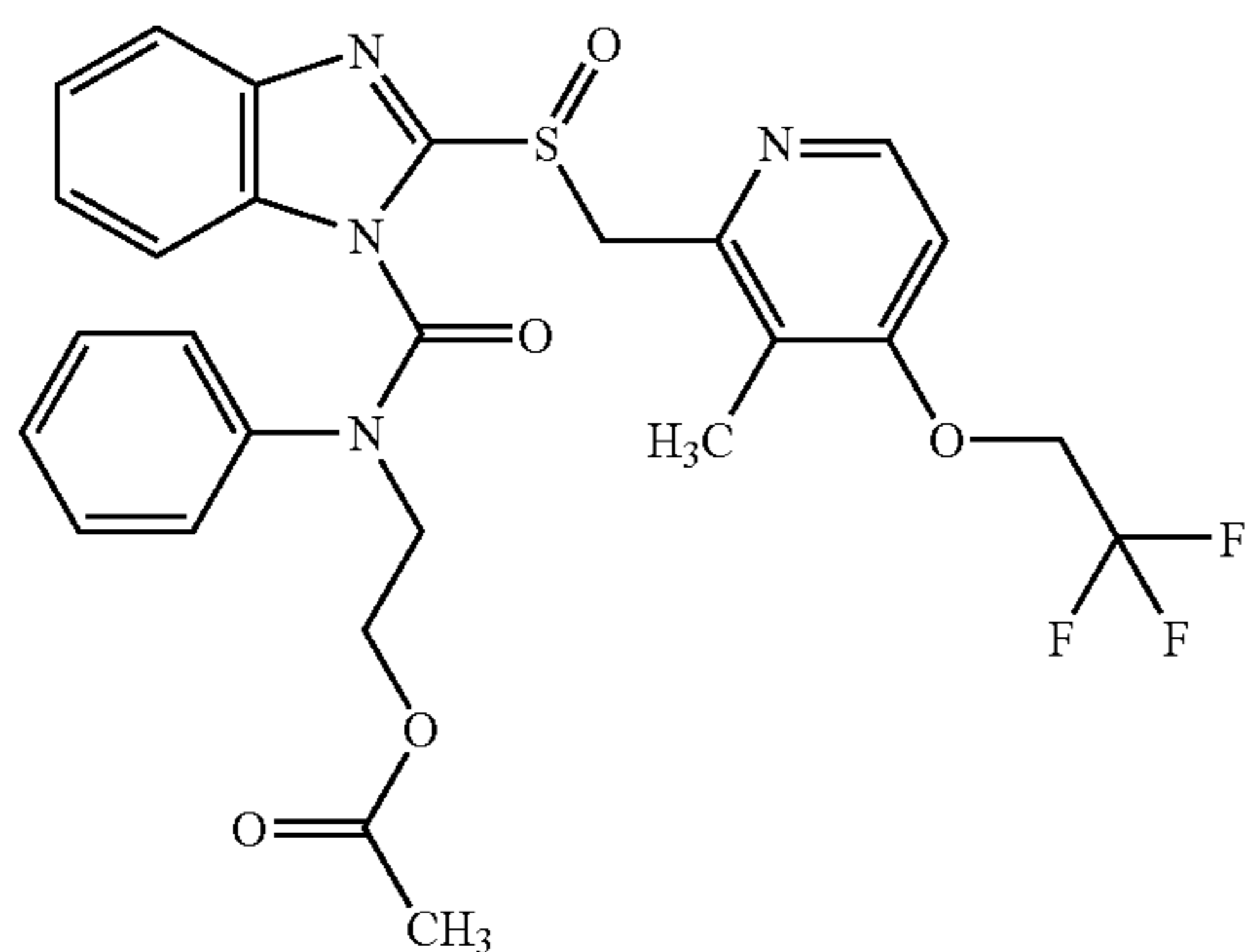
2-[[[2-[[[3-Methyl-4-(2,2,2-trifluoroethoxy)-2-pyridyl]methyl]sulfinyl]-1H-benzimidazol-1-yl]carbonyl](phenyl)amino]ethyl acetate
