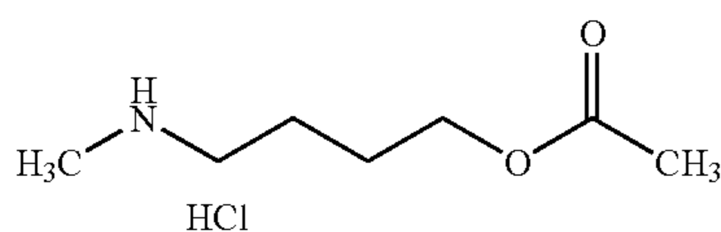
4-(Methylamino)butyl acetate hydrochloride
