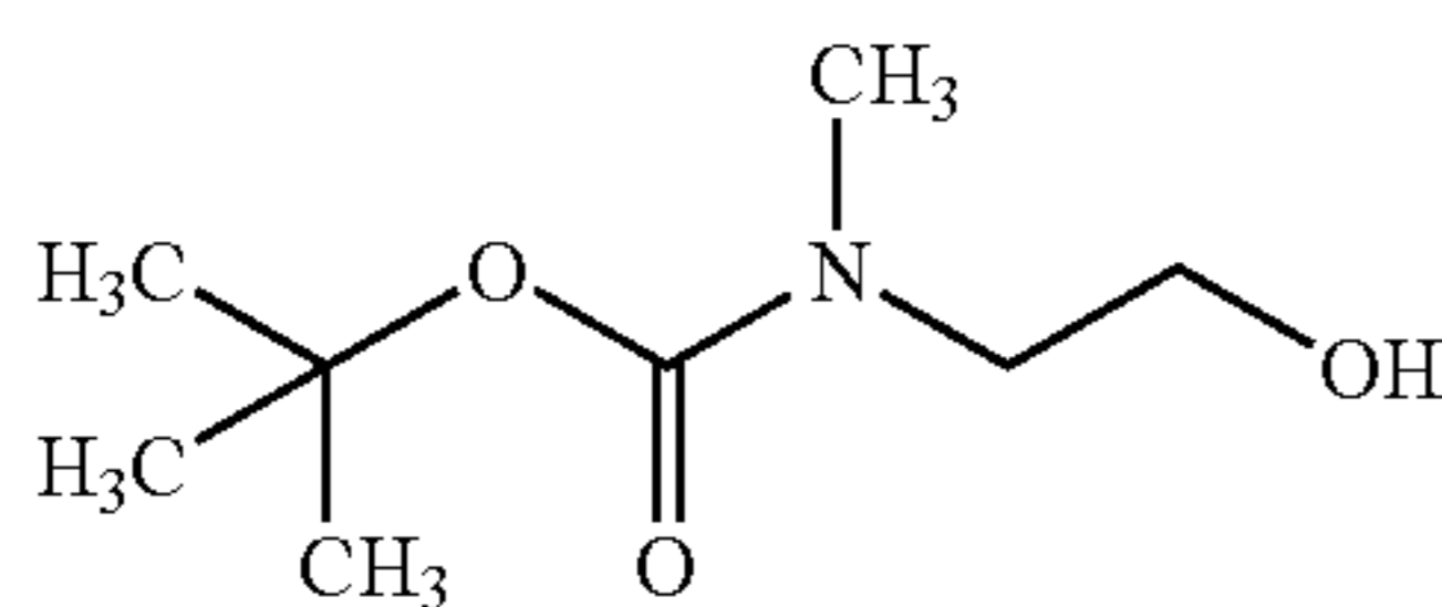
tert-Butyl 2-hydroxyethyl(methyl)carbamate
