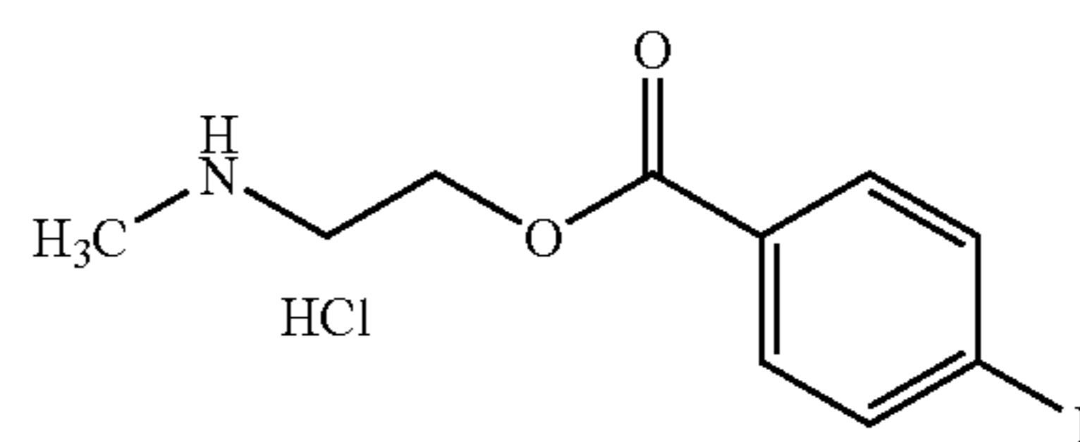
2-(Methylamino)ethyl 4-fluorobenzoate hydrochloride
