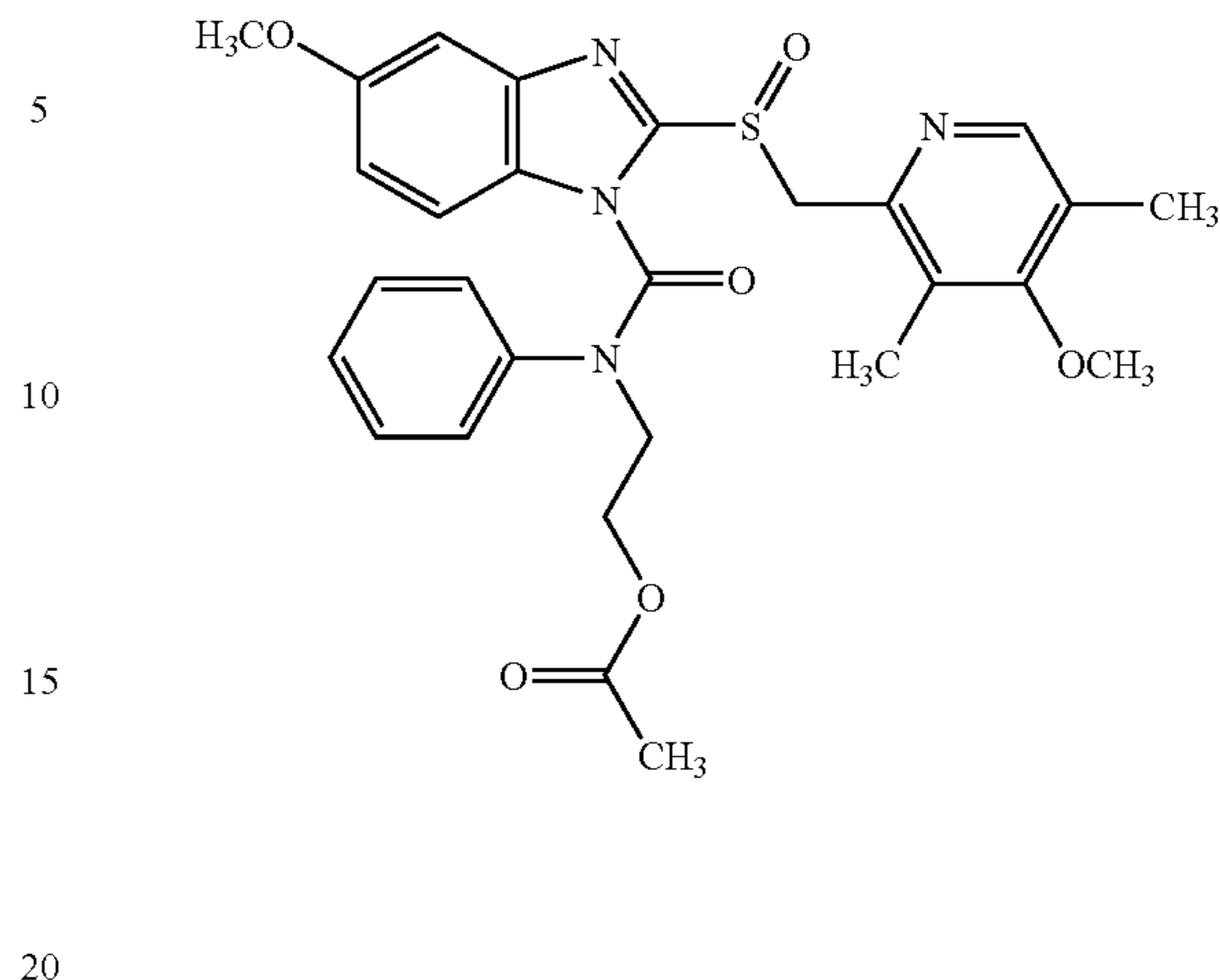
2-[[[5-Methoxy 2-[[[4-methoxy-3,5-dimethyl-2-pyridyl)methyl]sulfinyl]-1H-benzimidazol-1-yl]carbonyl](phenyl)amino]ethyl acetate
