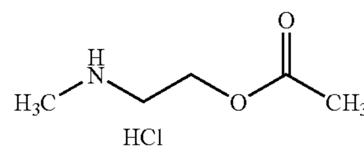
2-(Methylamino)ethyl acetate hydrochloride
