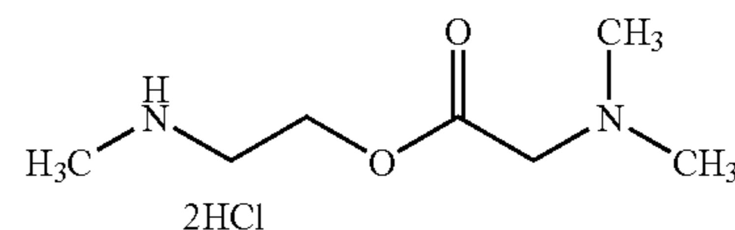
2-(Methylamino)ethyl N,N-dimethylglycinate dihydrochloride
