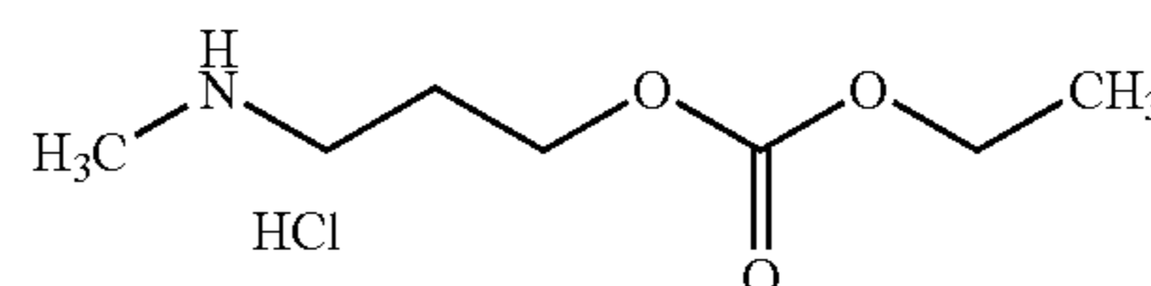
Ethyl 3-(methylamino)propyl carbonate hydrochloride
