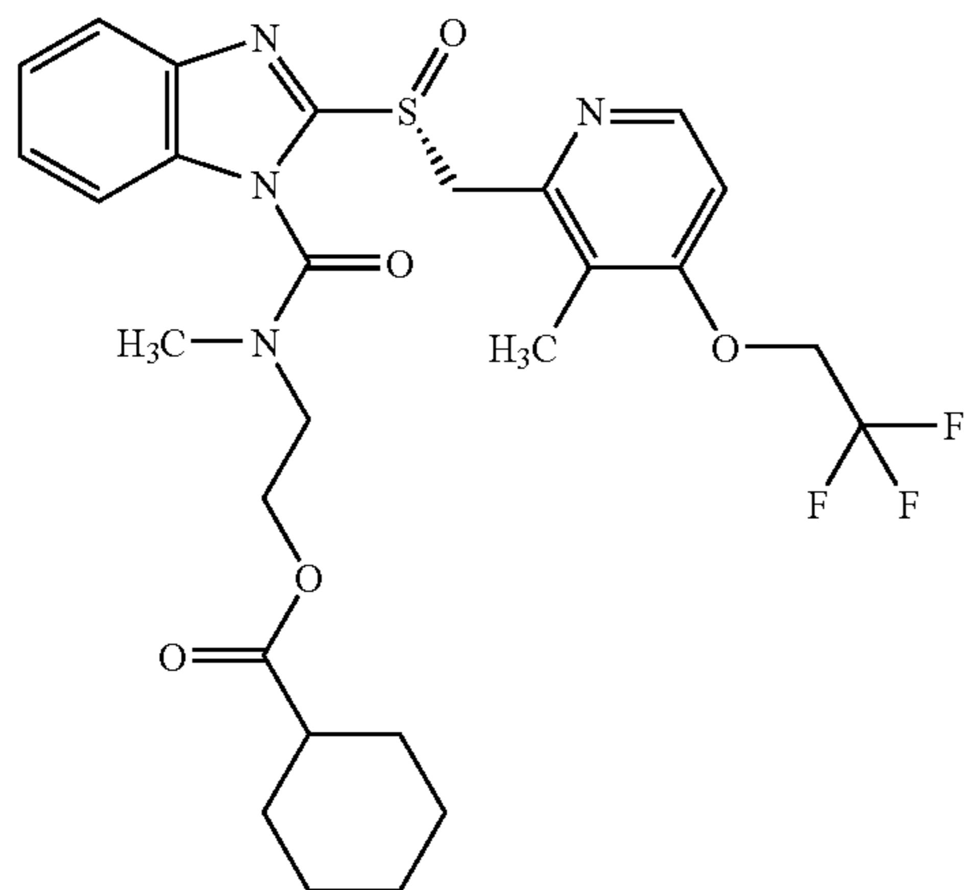
2-[Methyl[[[R]-2-[[[3-methyl-4-(2,2,2-trifluoroethoxy)-2-pyridyl]methyl]sulfinyl]-1H-benzimidazol-1-yl]carbonyl]amino]ethyl cyclohexanecarboxylate
