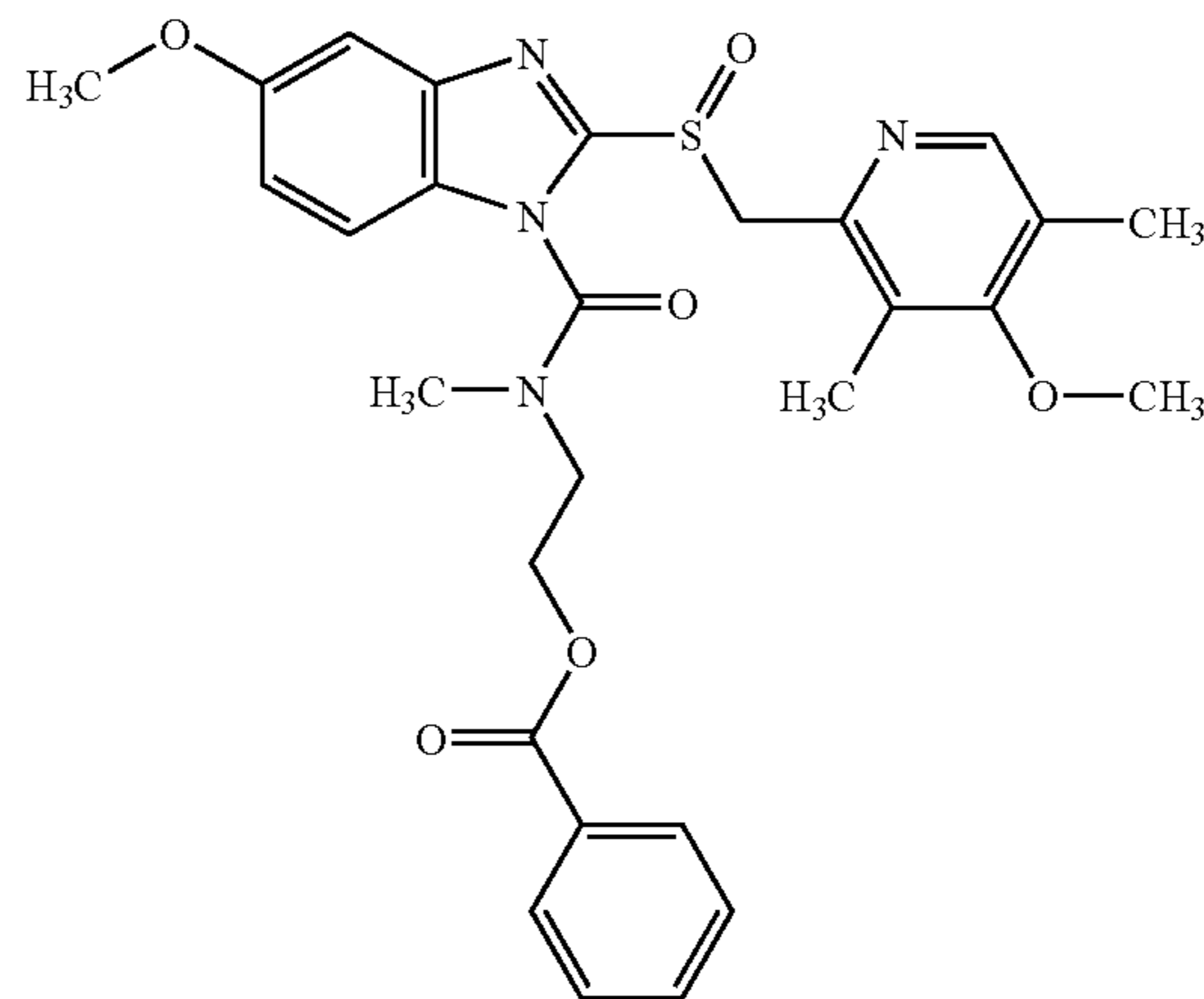
Example 32
