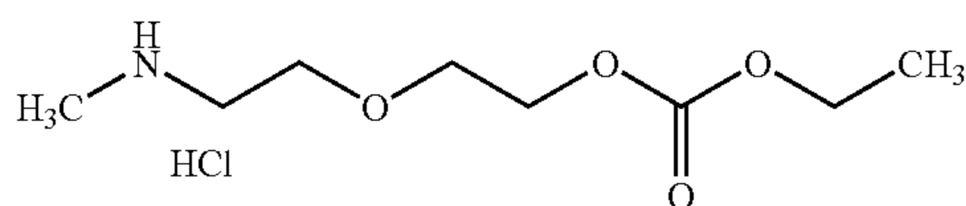
Ethyl 2-[2-(methylamino)ethoxy]ethyl carbonate hydrochloride
