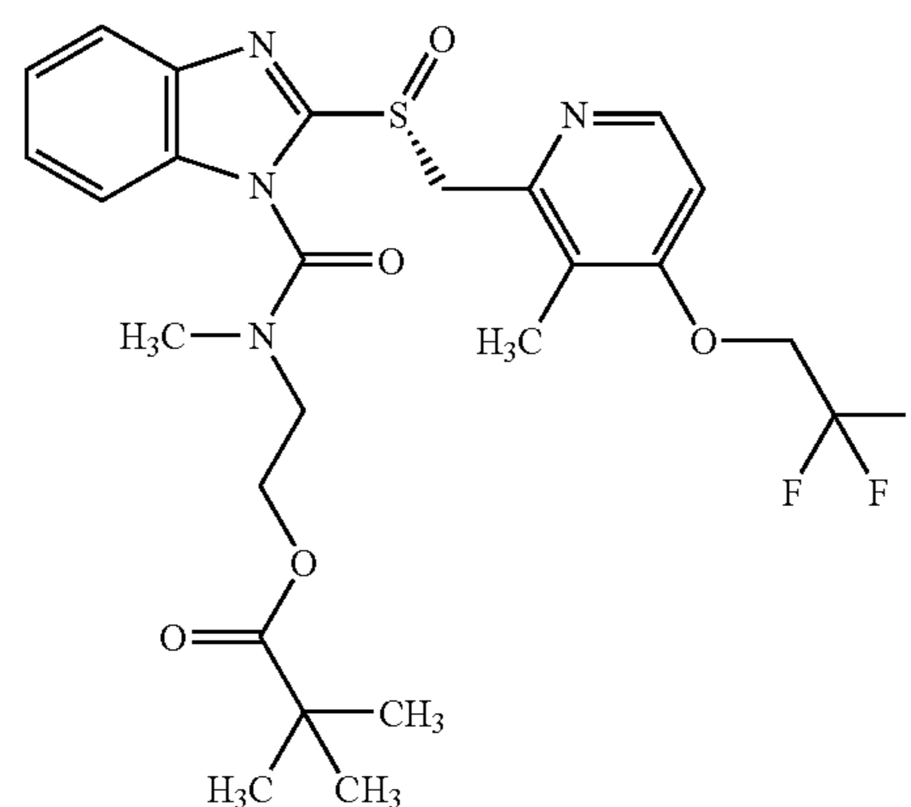
Example 2
