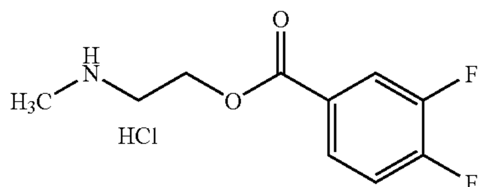
Reference Example 8
