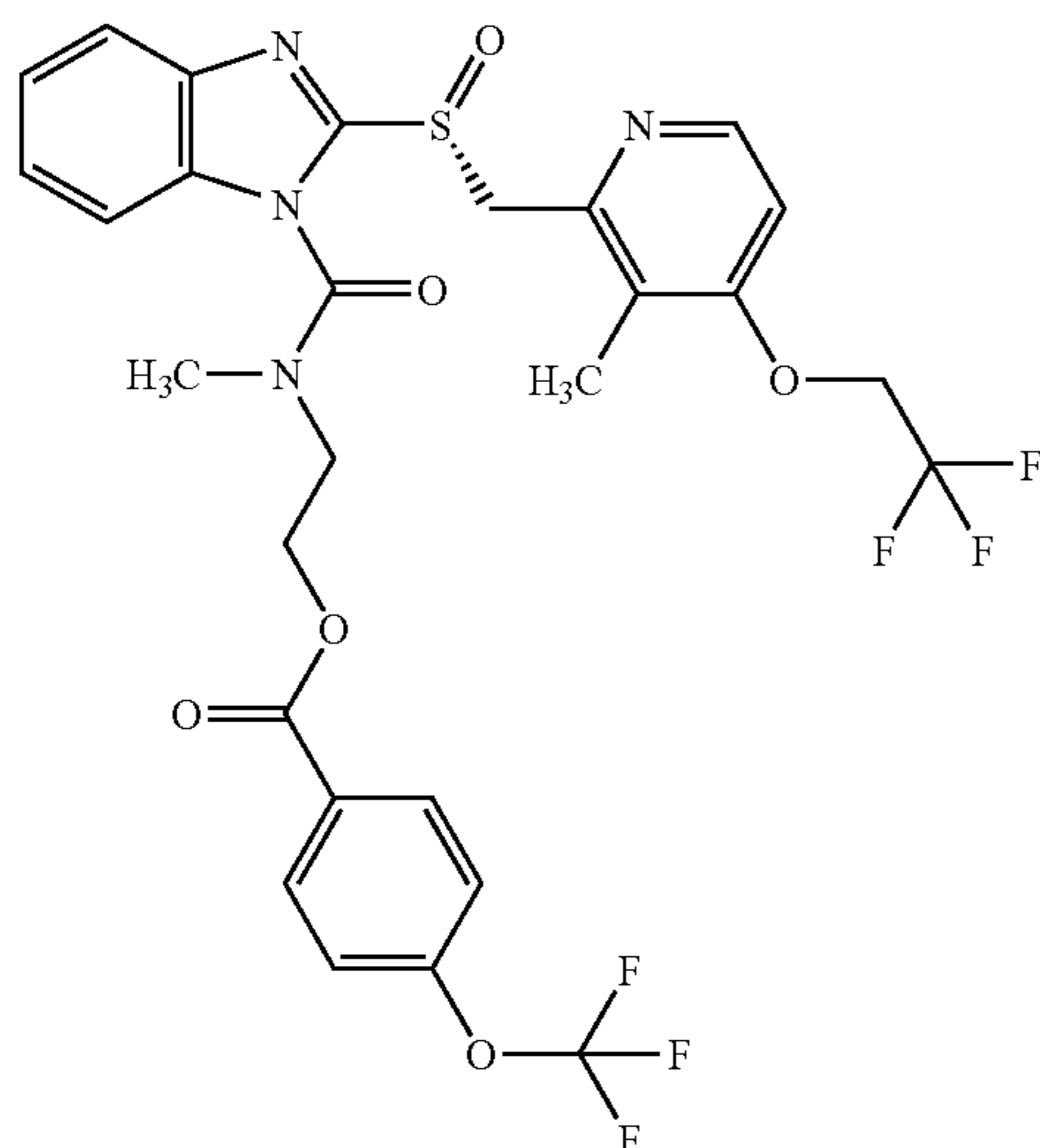
Example 9
