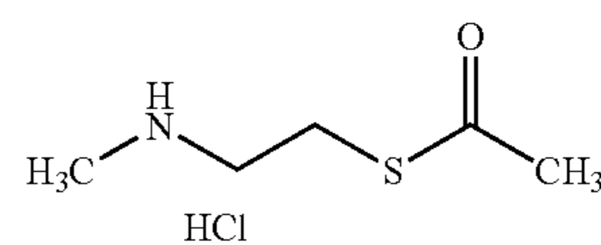
S-[2-(Methylamino)ethyl]thioacetate hydrochloride
