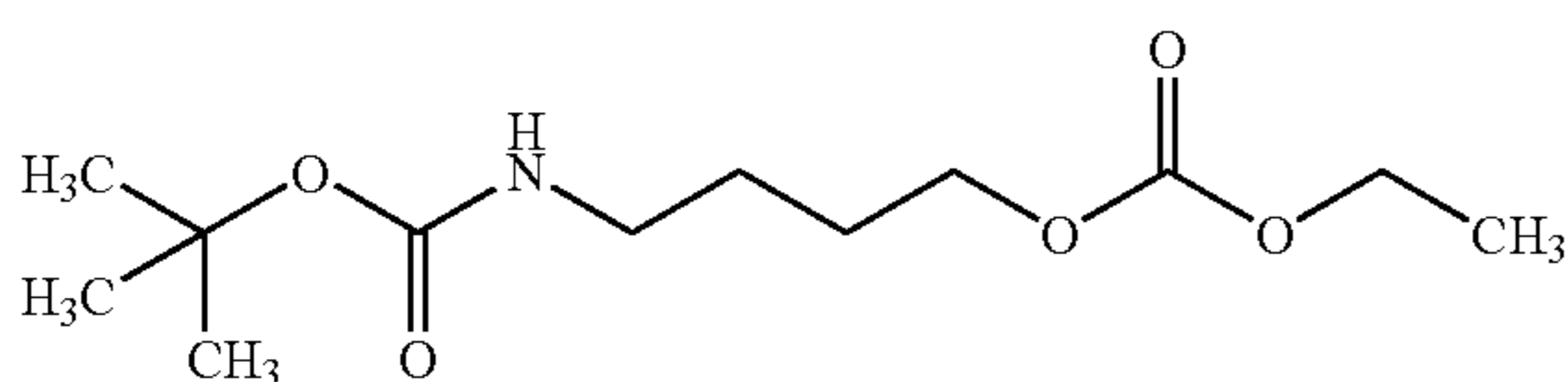
4-[(tert-Butoxycarbonyl)amino]butyl ethyl carbonate
