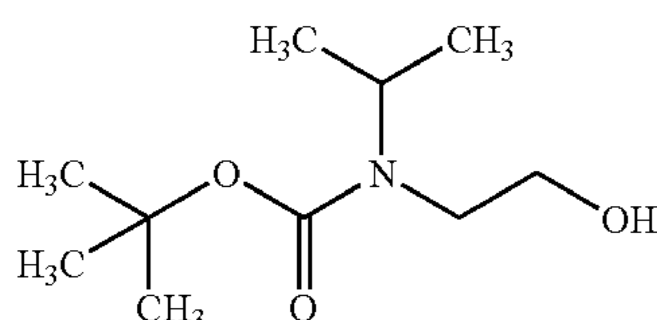
tert-Butyl 2-hydroxyethyl(isopropyl)carbamate
