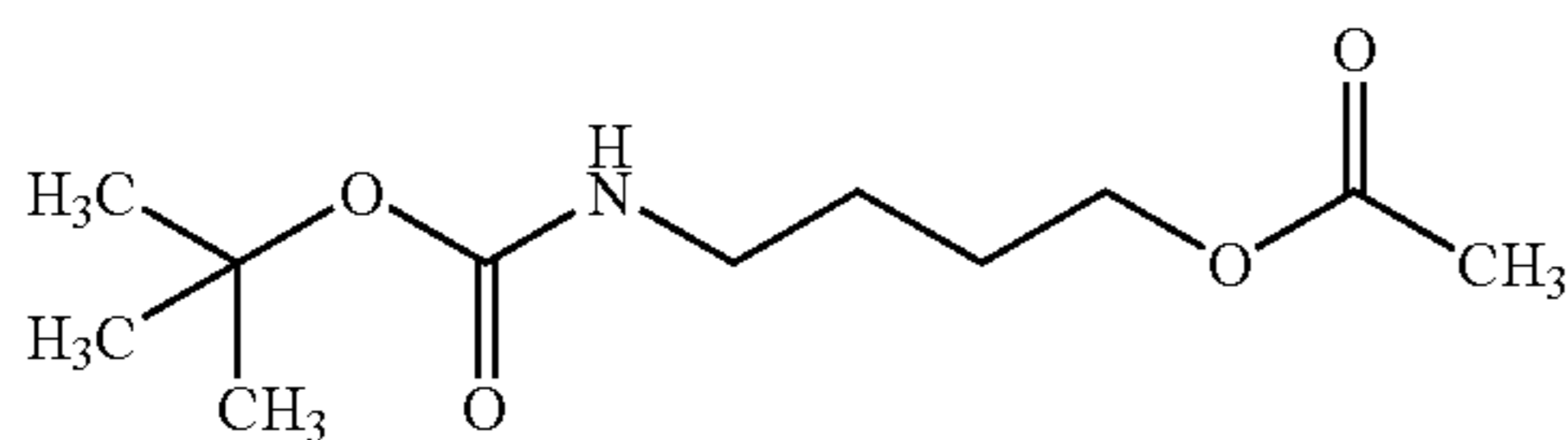
4-[(tert-Butoxycarbonyl)amino]butyl acetate
