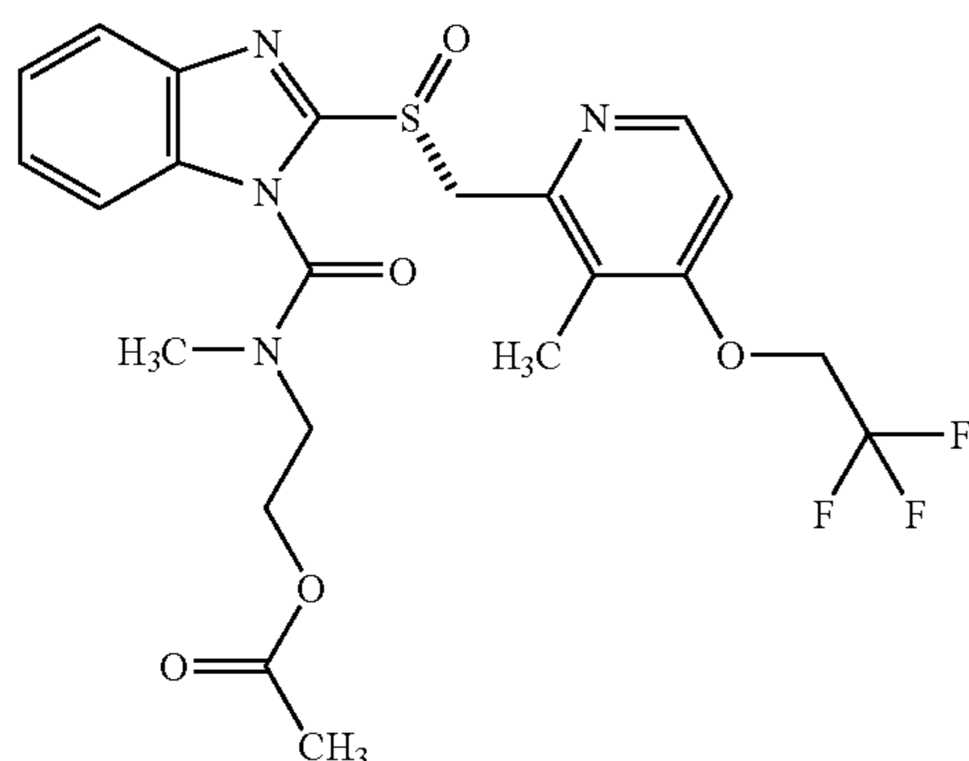
Example 1
