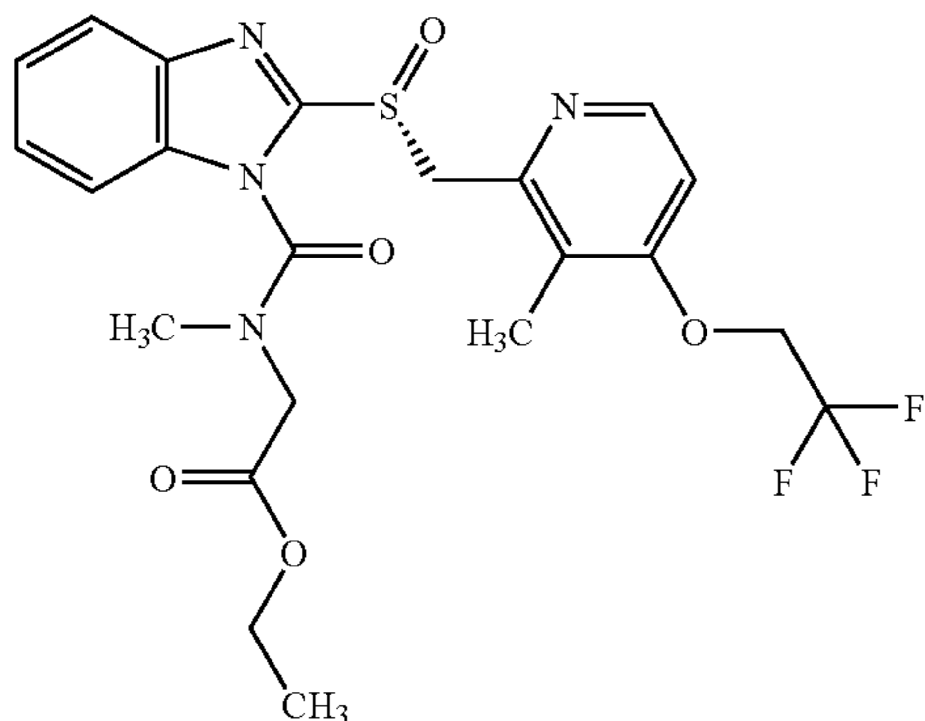
Ethyl[[methyl][(R)-2-[[[3-methyl-4-(2,2,2-trifluoroethoxy)-2-pyridyl]methyl]sulfinyl]-1H-benzimidazol-1-yl]carbonyl]amino]acetate
