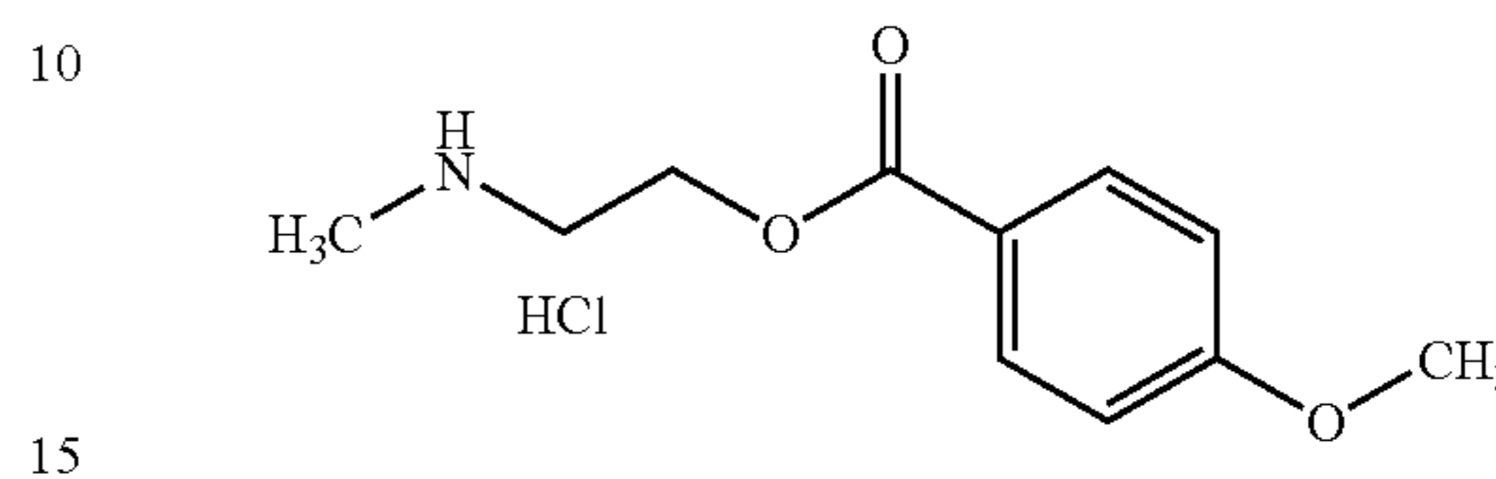
2-(Methylamino)ethyl 4-methoxybenzoate hydrochloride
