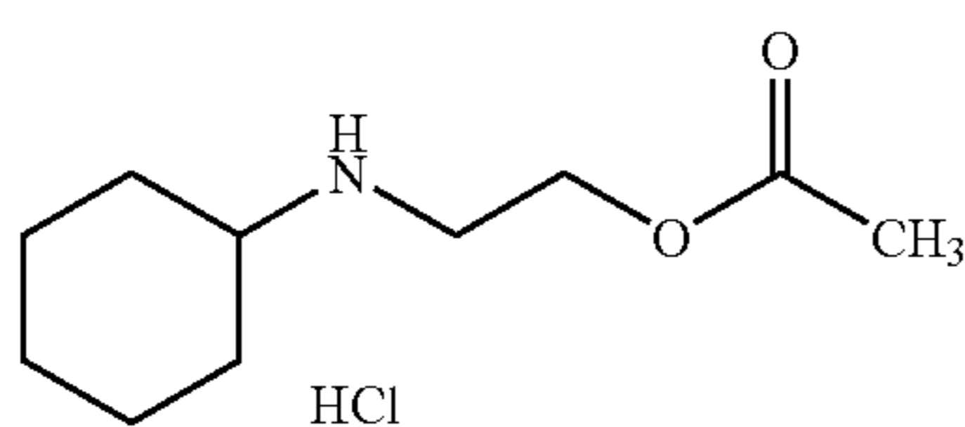
2-(Cyclohexylamino)ethyl acetate hydrochloride
