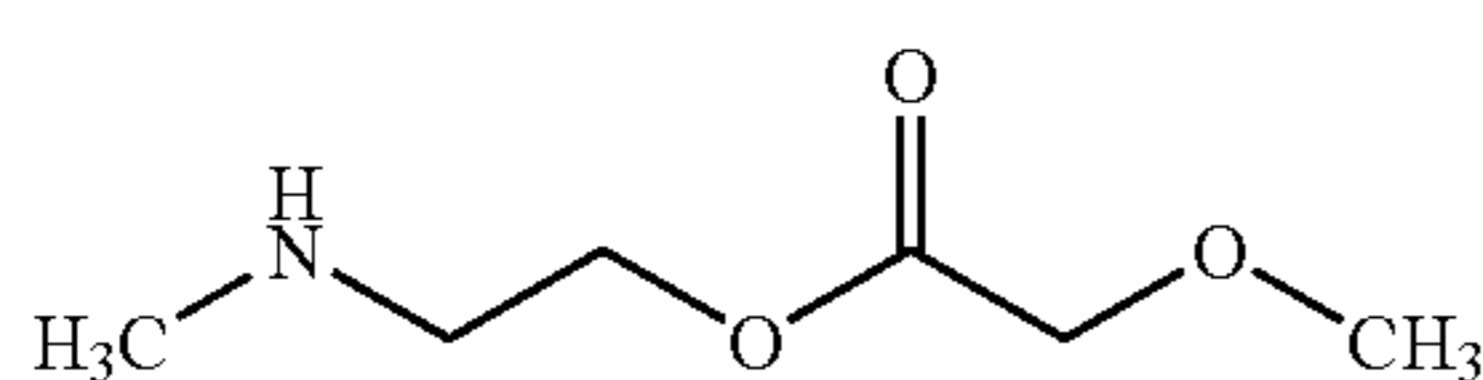
2-(Methylamino)ethyl methoxyacetate
