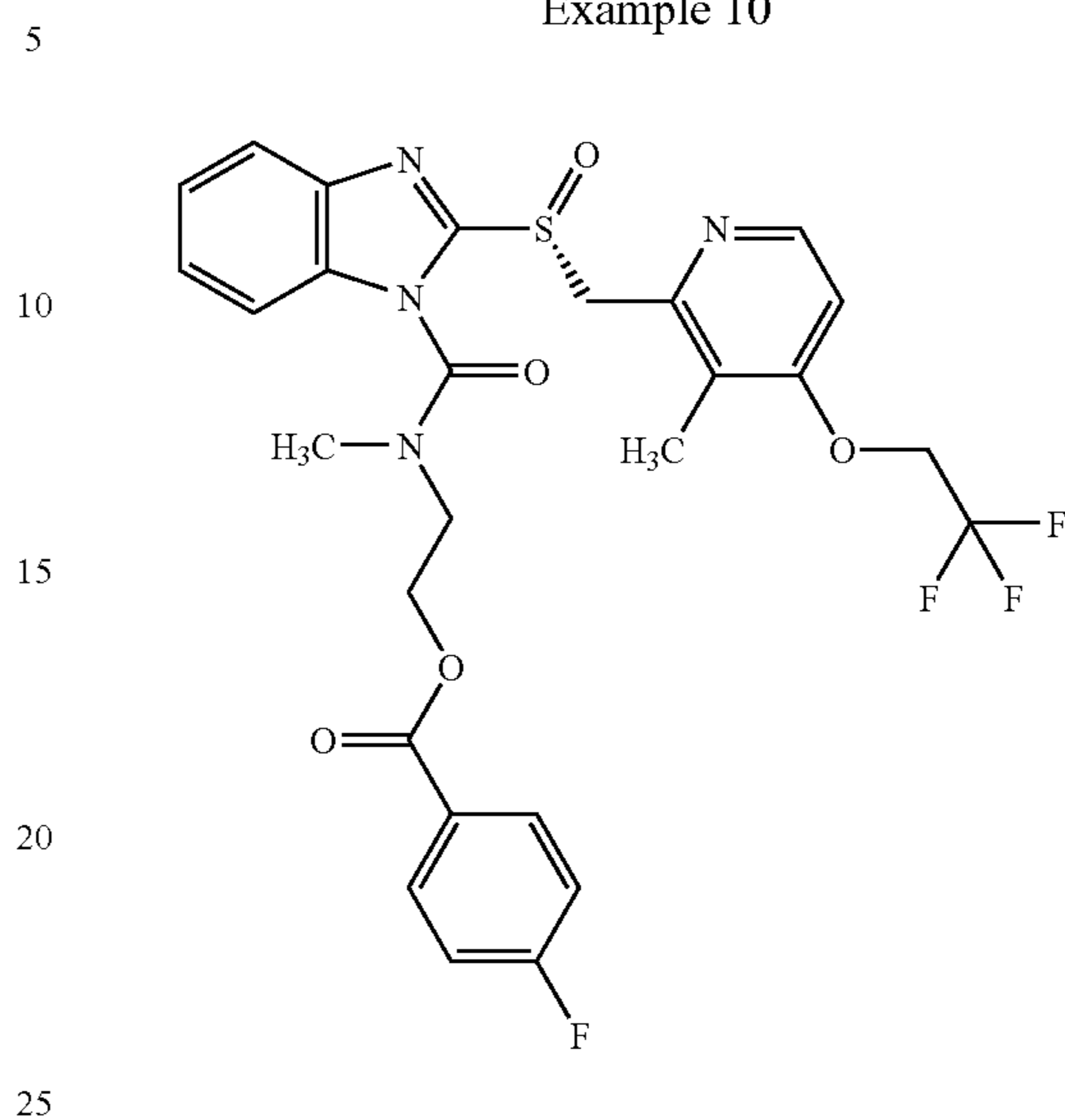
2-[Methyl[[[R]-2-[[[3-methyl-4-(2,2,2-trifluoroethoxy)-2-pyridyl]methyl]sulfinyl]-1H-benzimidazol-1-yl]carbonyl]amino]ethyl 4-fluorobenzoate
