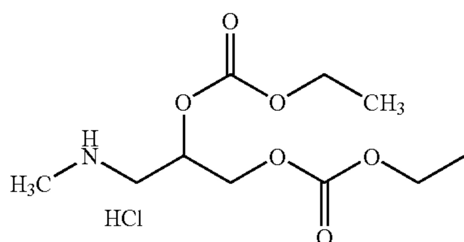
Diethyl 3-(methylamino)propane-1,2-diyl biscarbonate hydrochloride
