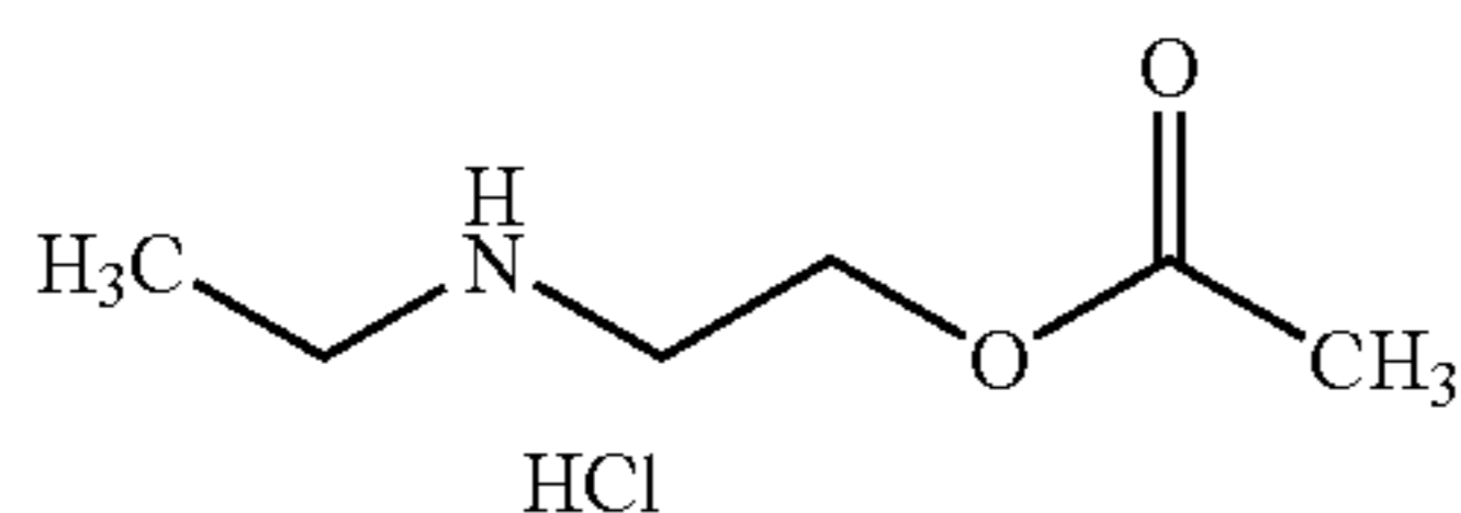
2-(Ethylamino)ethyl acetate hydrochloride
