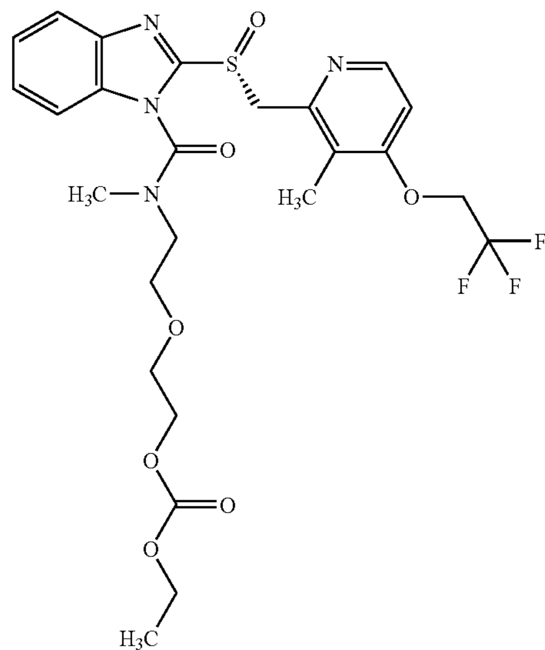
Ethyl 2-[2-[methyl[[R)-2-[[[3-methyl-4-(2,2,2-trifluoroethoxy)-2-pyridyl]methyl]sulfinyl]-1H-benzimidazol-1-yl]carbonyl]amino]ethoxy]ethyl carbonate
