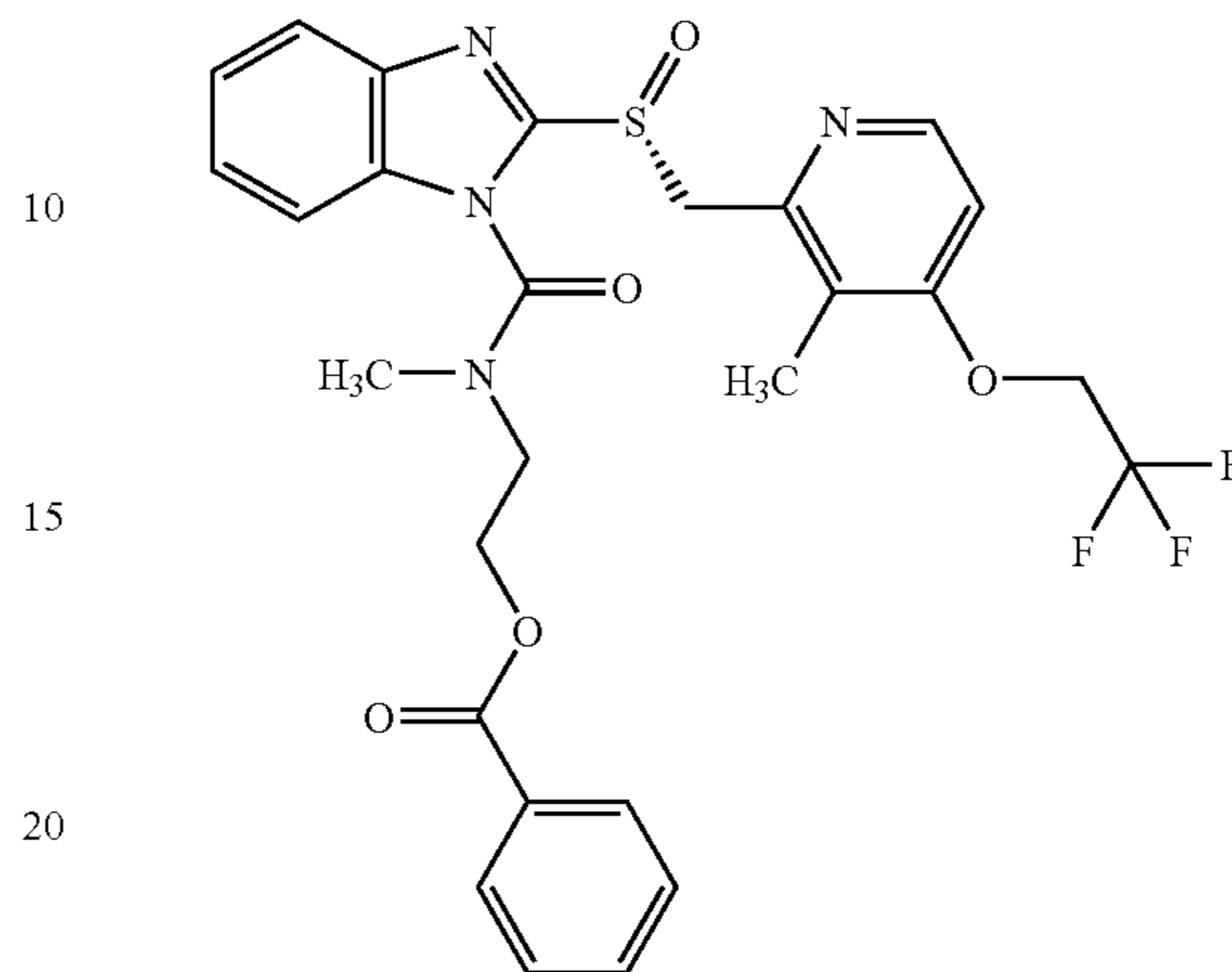
2-[Methyl[[[R]-2-[[[3-methyl-4-(2,2,2-trifluoroethoxy)-2-pyridyl]methyl]sulfinyl]-1H-benzimidazol-1-yl]carbonyl]amino]ethyl benzoate
