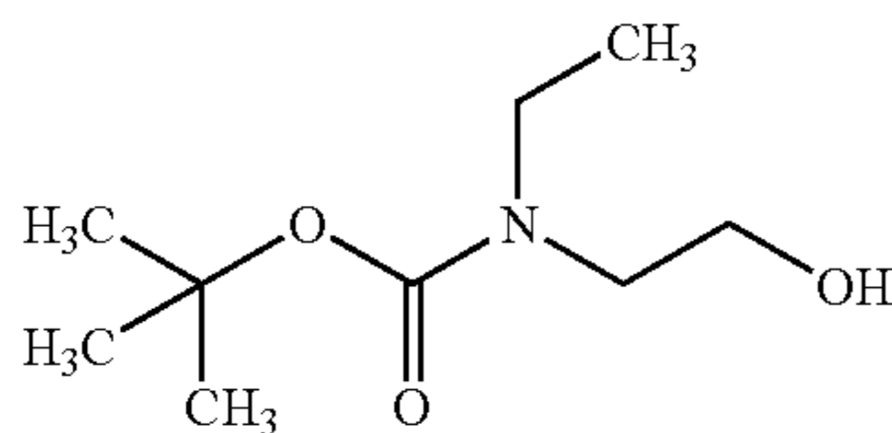
tert-Butyl ethyl(2-hydroxyethyl)carbamate
