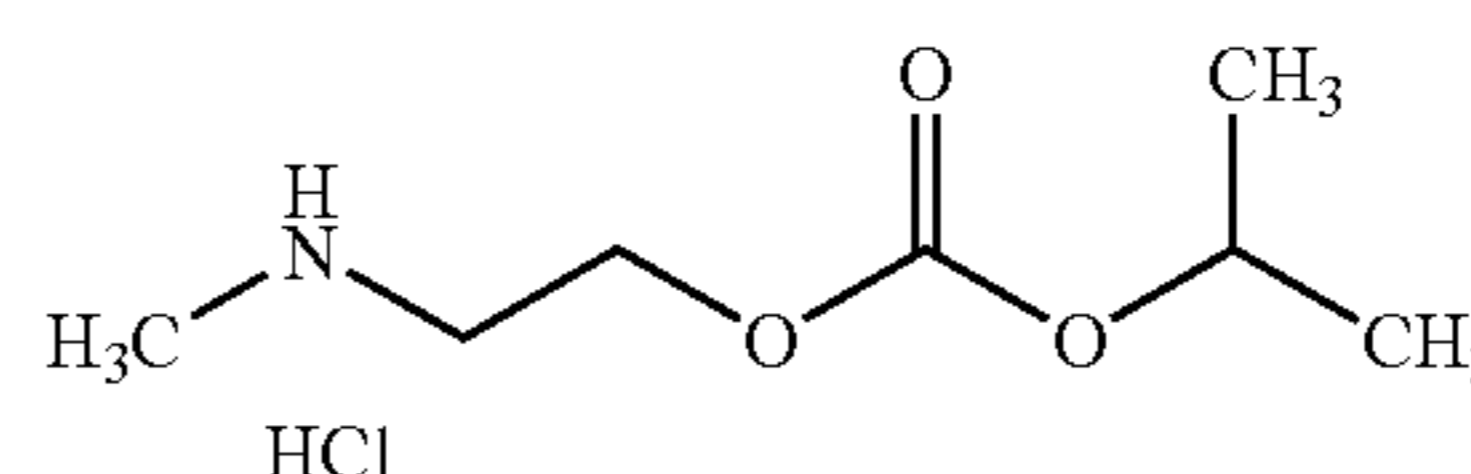
Isopropyl 2-(methylamino)ethyl carbonate hydrochloride
