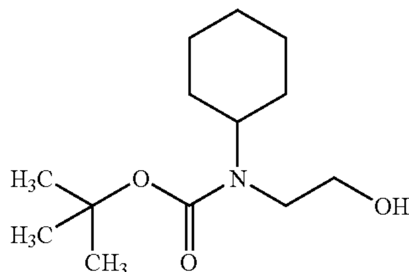
tert-Butyl cyclohexyl(2-hydroxyethyl)carbamate
