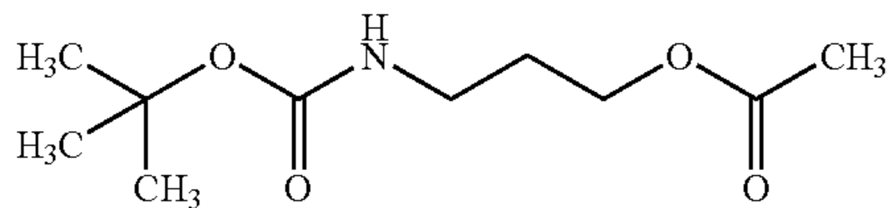
3-[(tert-Butoxycarbonyl)amino]propyl acetate
