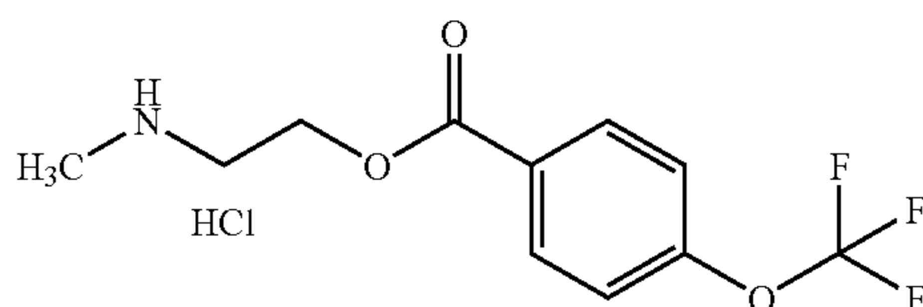
Reference Example 9
