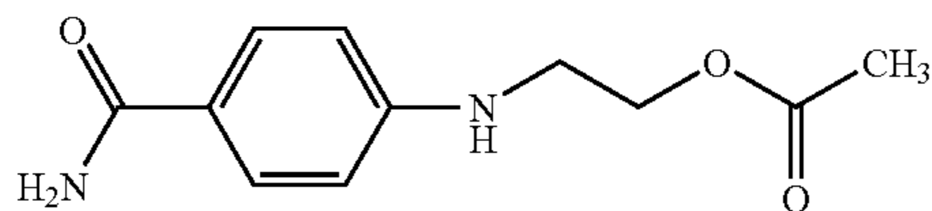
2-[[4-(Aminocarbonyl)phenyl]amino]ethyl acetate
