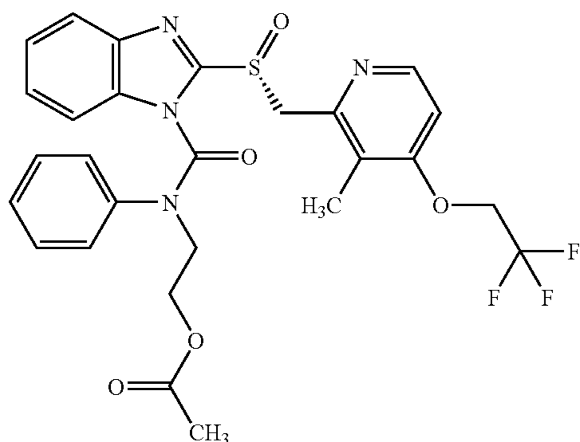
2-[[[(R)-2-[[[3-Methyl-4-(2,2,2-trifluoroethoxy)-2-pyridyl]methyl]sulfinyl]-1H-benzimidazol-1-yl]carbonyl](phenyl)amino]ethyl acetate
