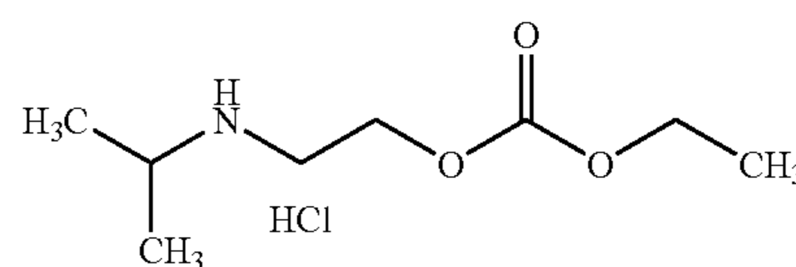
Ethyl 2-(isopropylamino)ethyl carbonate hydrochloride
