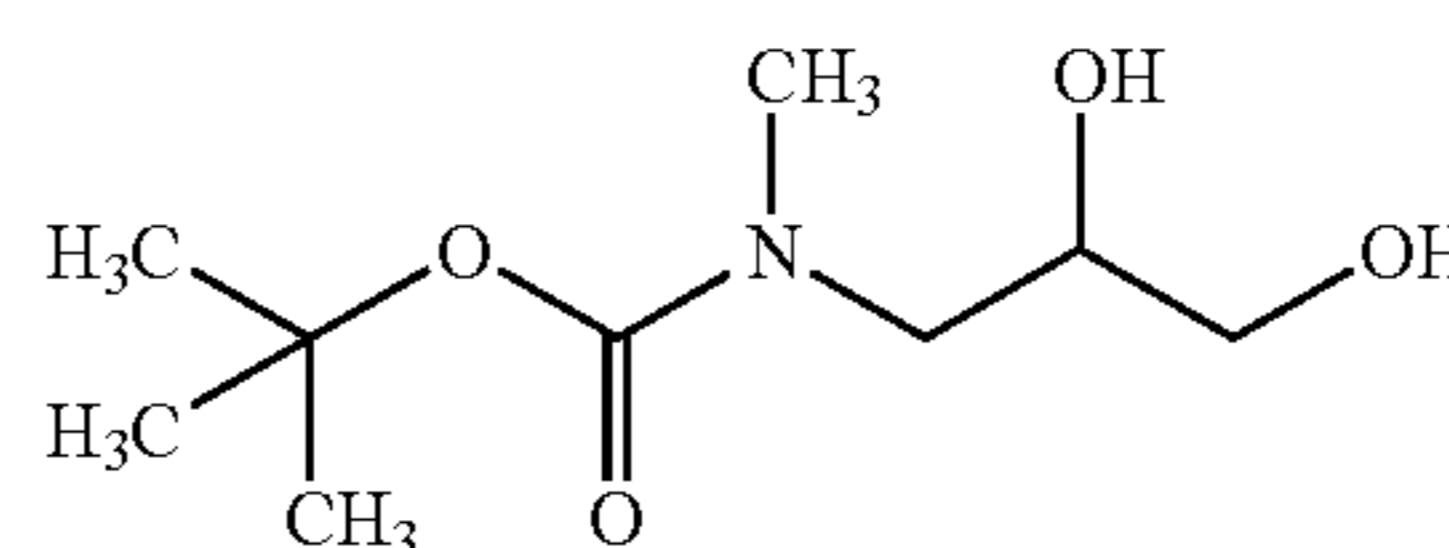
tert-Butyl(2,3-dihydroxypropyl)methylcarbamate
