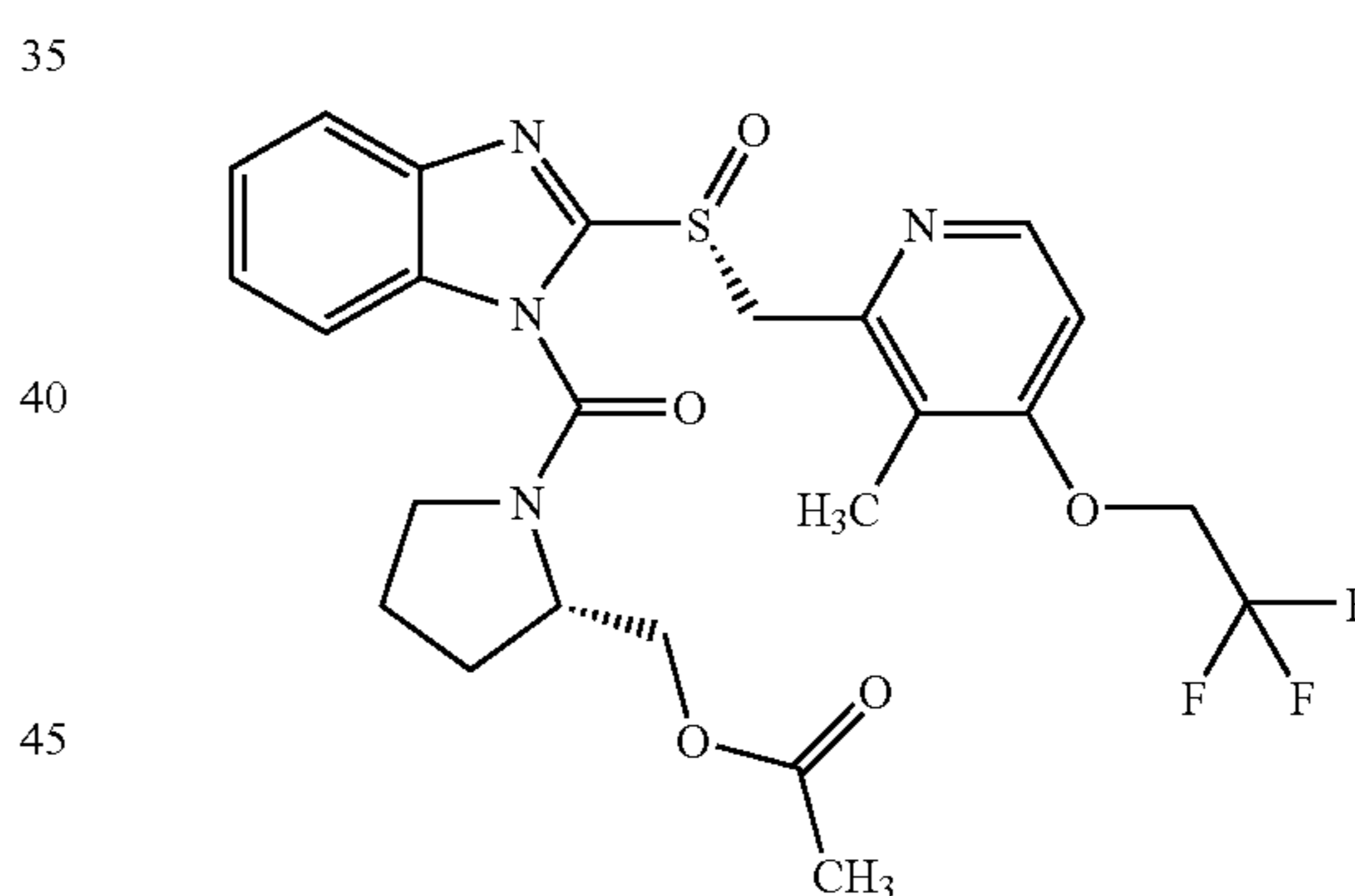
[(2S)-1-[[[R]-2-[[[3-Methyl-4-(2,2,2-trifluoroethoxy)-2-pyridyl]methyl]sulfinyl]-1H-benzimidazol-1-yl]carbonyl]-2-pyrrolidinyl]methyl acetate
