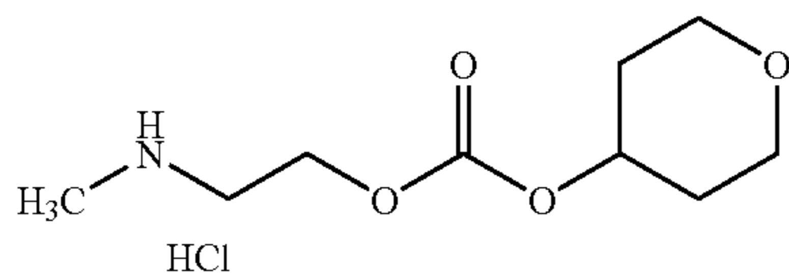
2-(Methylamino)ethyl tetrahydropyran-4-yl carbonate hydrochloride
