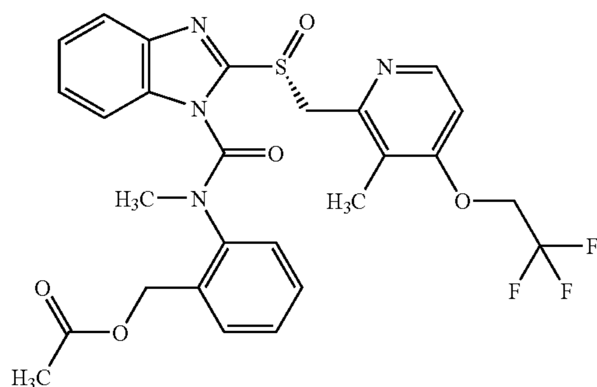
2-[Methyl[[[R]-2-[[[3-methyl-4-(2,2,2-trifluoroethoxy)-2-pyridyl]methyl]sulfinyl]-1H-benzimidazol-1-yl]carbonyl]amino]benzyl acetate
