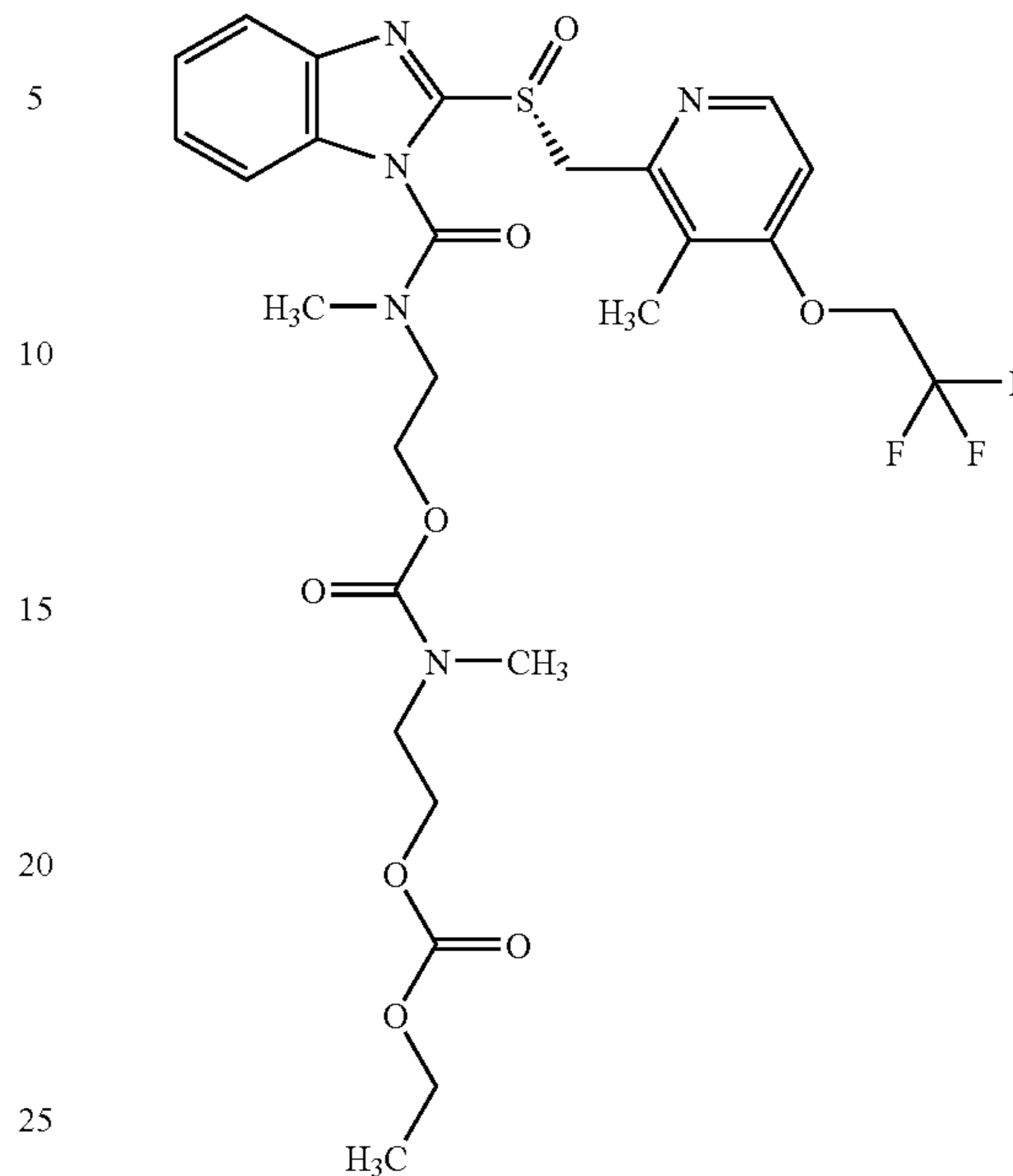
Ethyl 2-[methyl[[2-[methyl[[R)-2-[[[3-methyl-4-(2,2,2-trifluoroethoxy)-2-pyridyl]methyl]sulfinyl]-1H-benzimidazol-1-yl]carbonyl]amino]ethoxy]carbonyl]amino]ethyl carbonate
