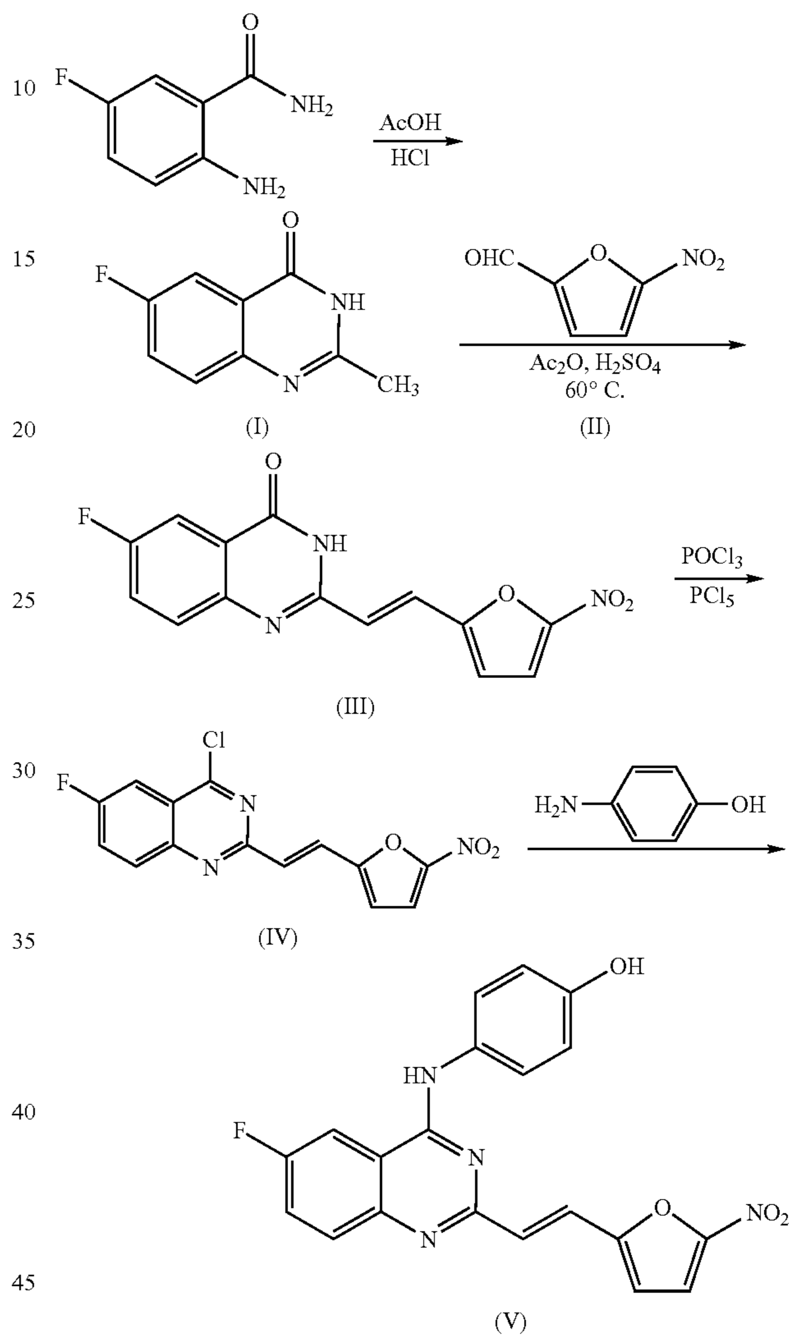
6-Fluoro-2-methyl-4-(3H)quinazolinone (I)
