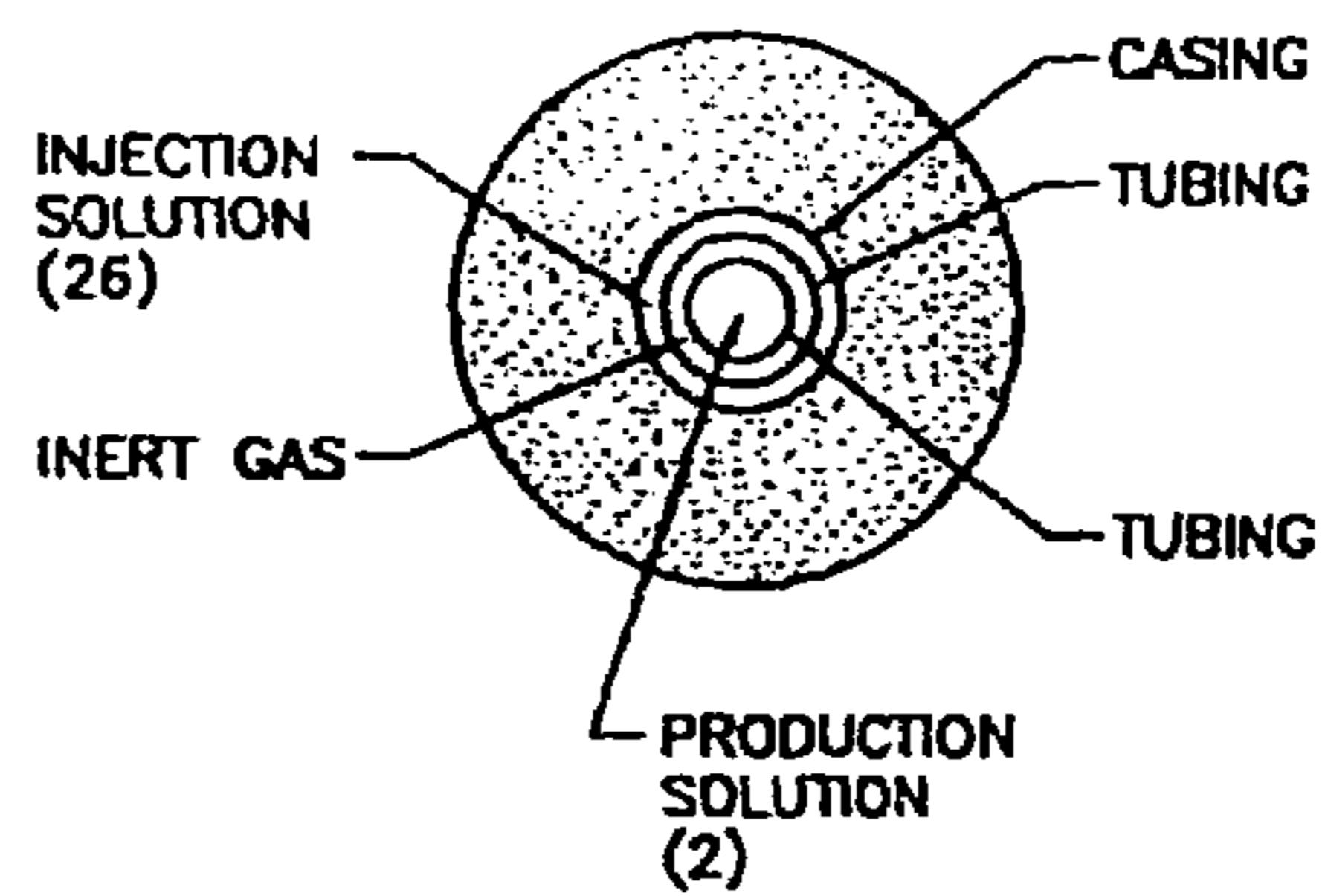
FIGURE 3B CROSS SECTION DETAIL A-A'
