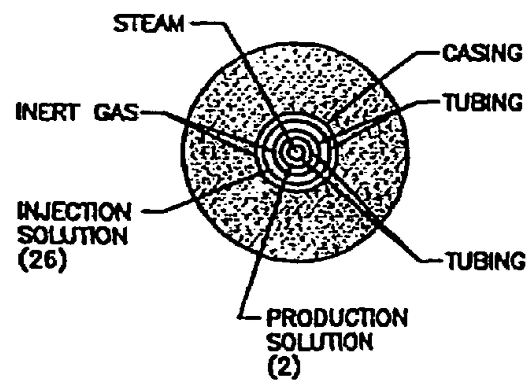
FIGURE 3D CROSS SECTION DETAIL A-A'
