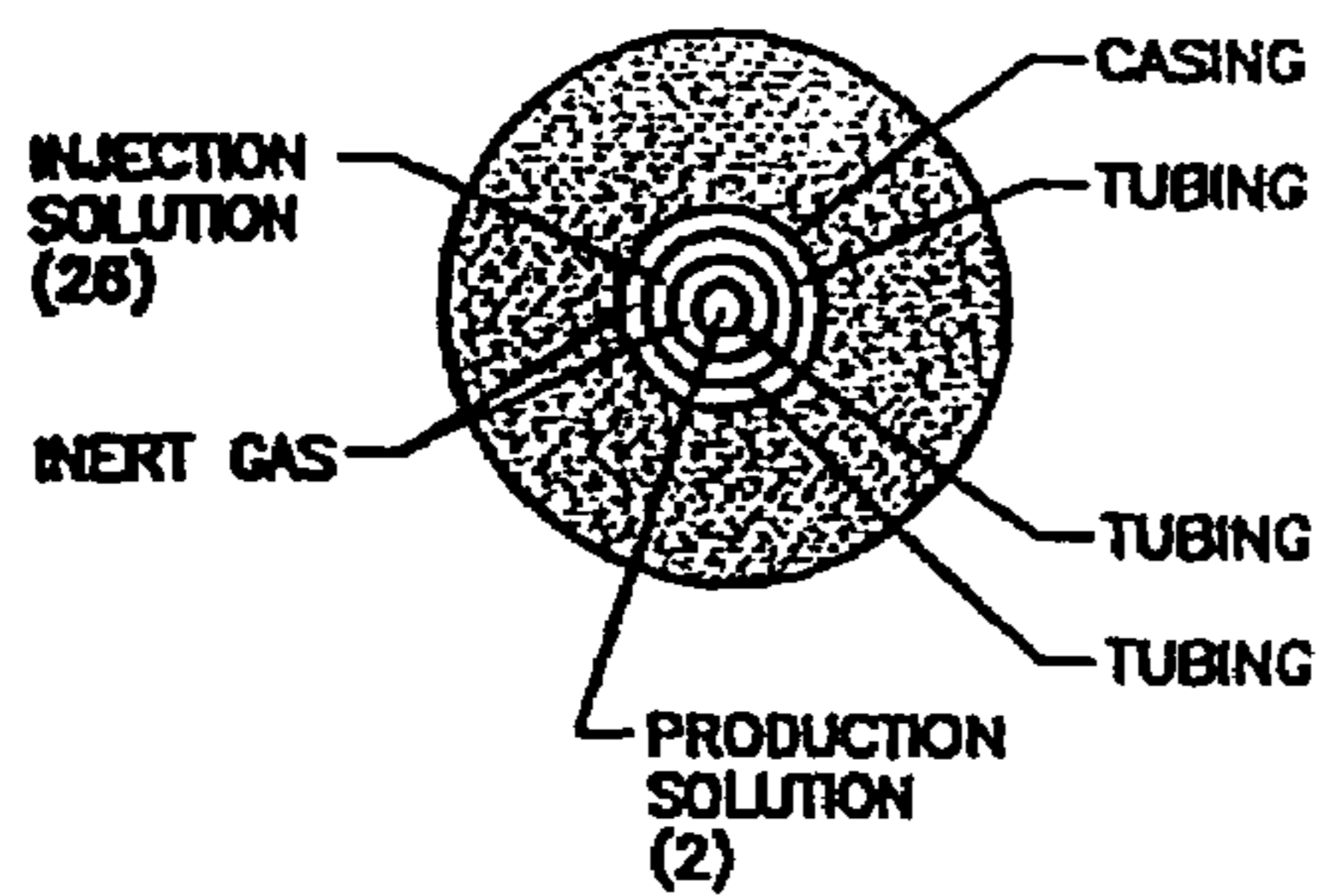
FIGURE 3C CROSS SECTION DETAIL A-A'
