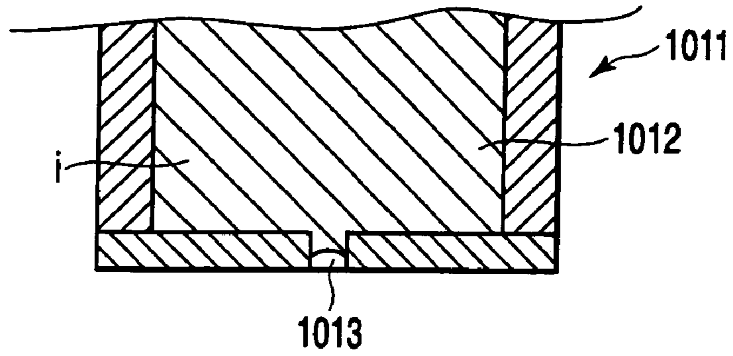
FIG. 24 (PRIOR ART)
