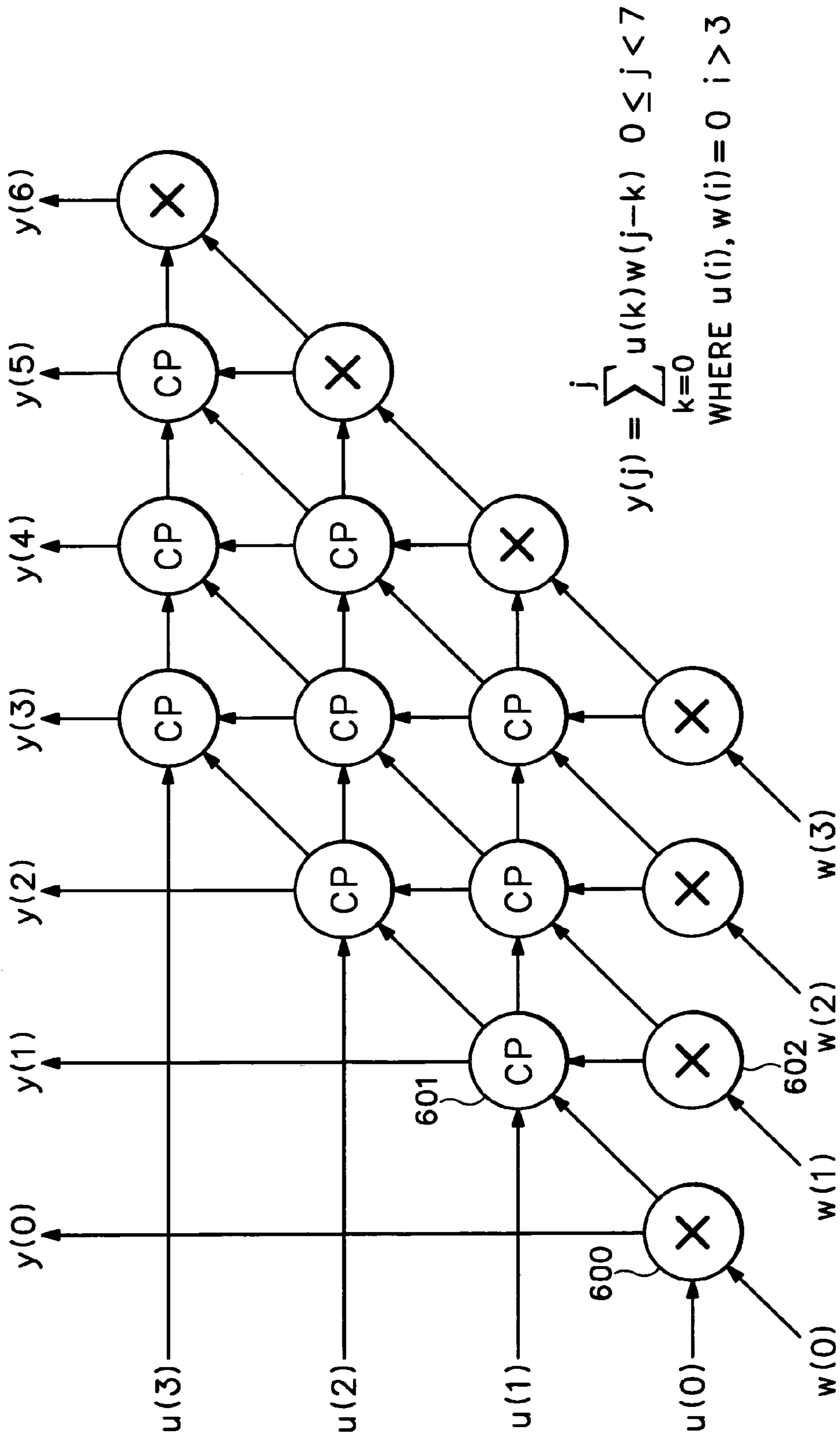
CONVOLUTION OF TWO SEQUENCES
