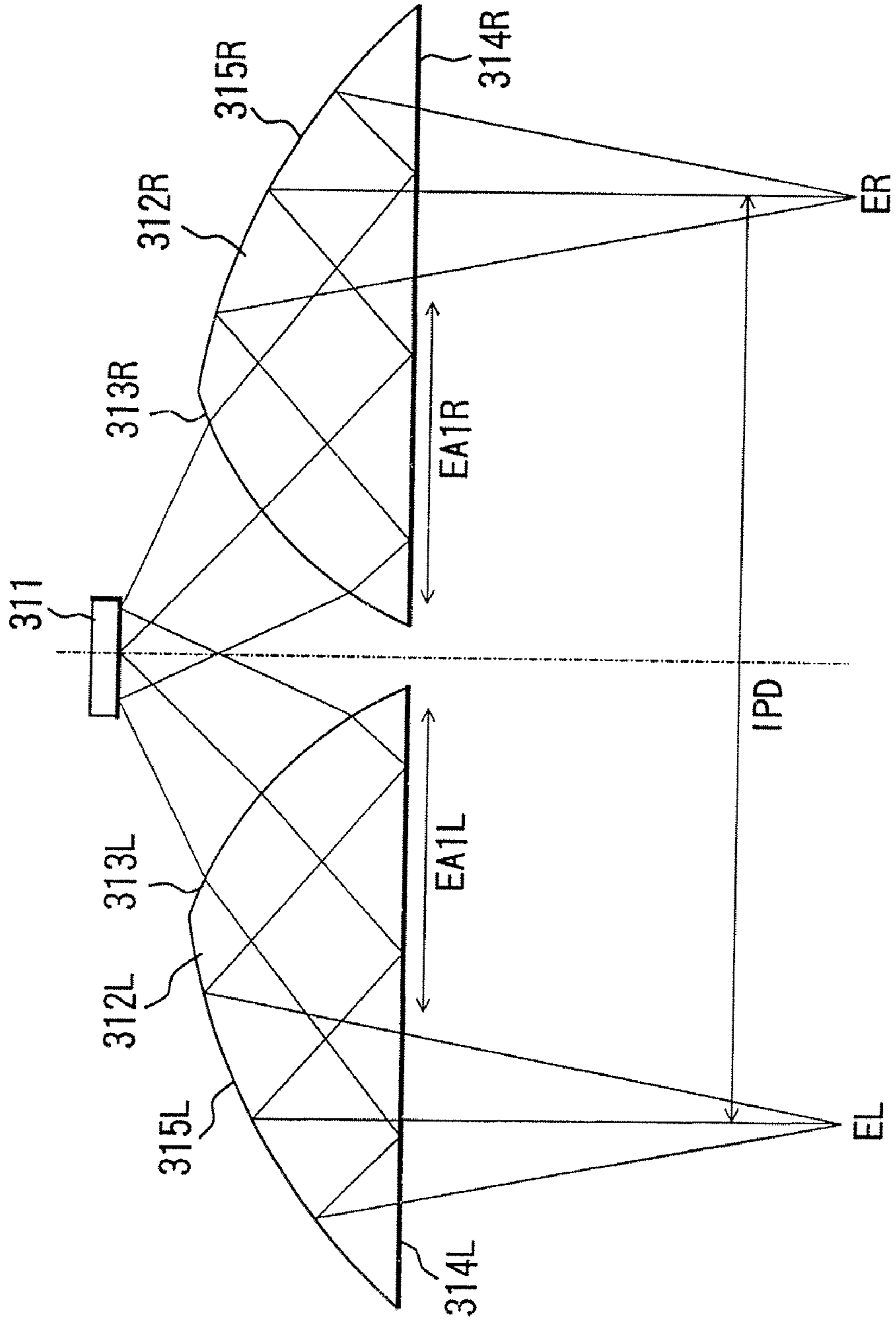
FIG.18 (PRIOR ART)
