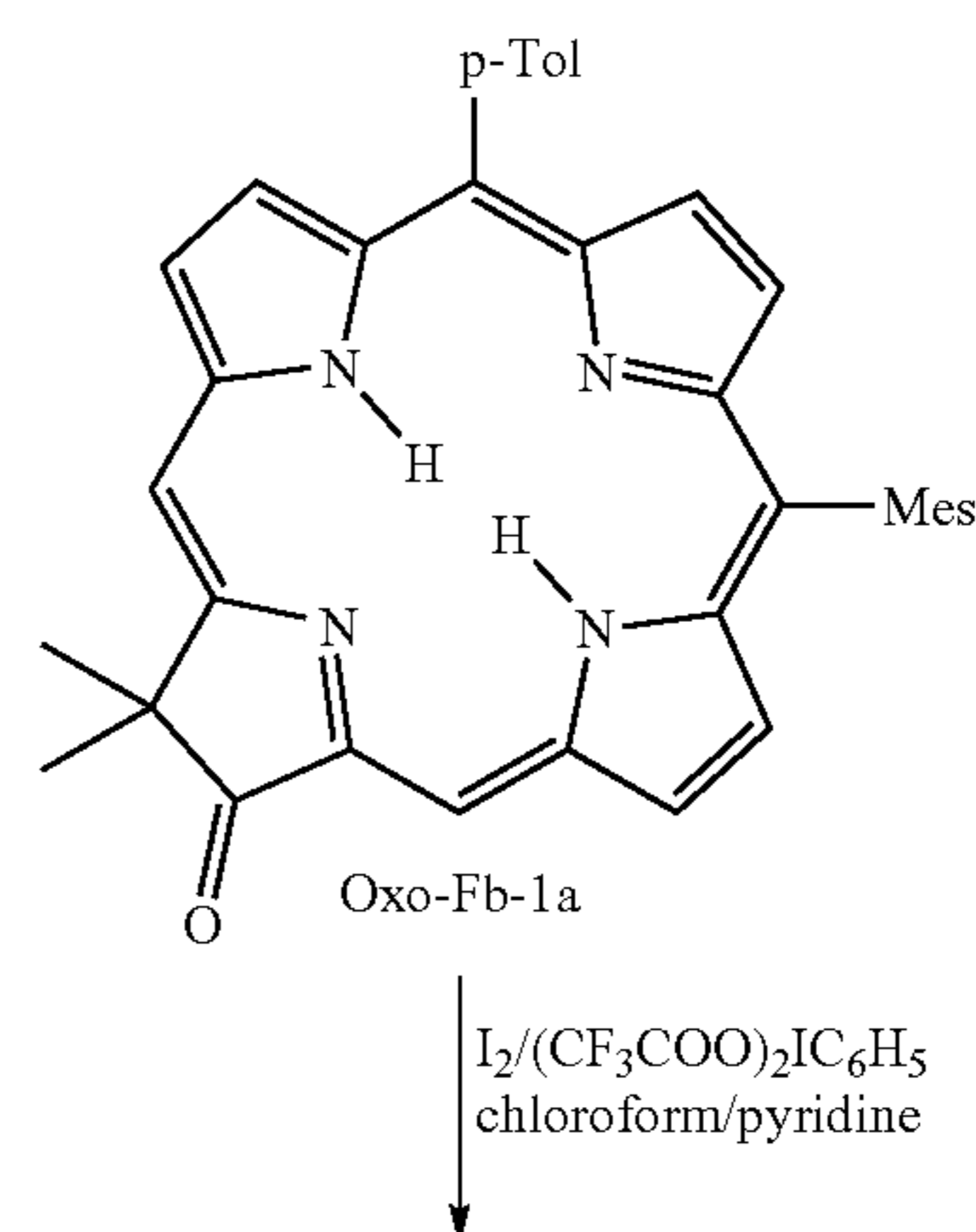
Scheme 9
