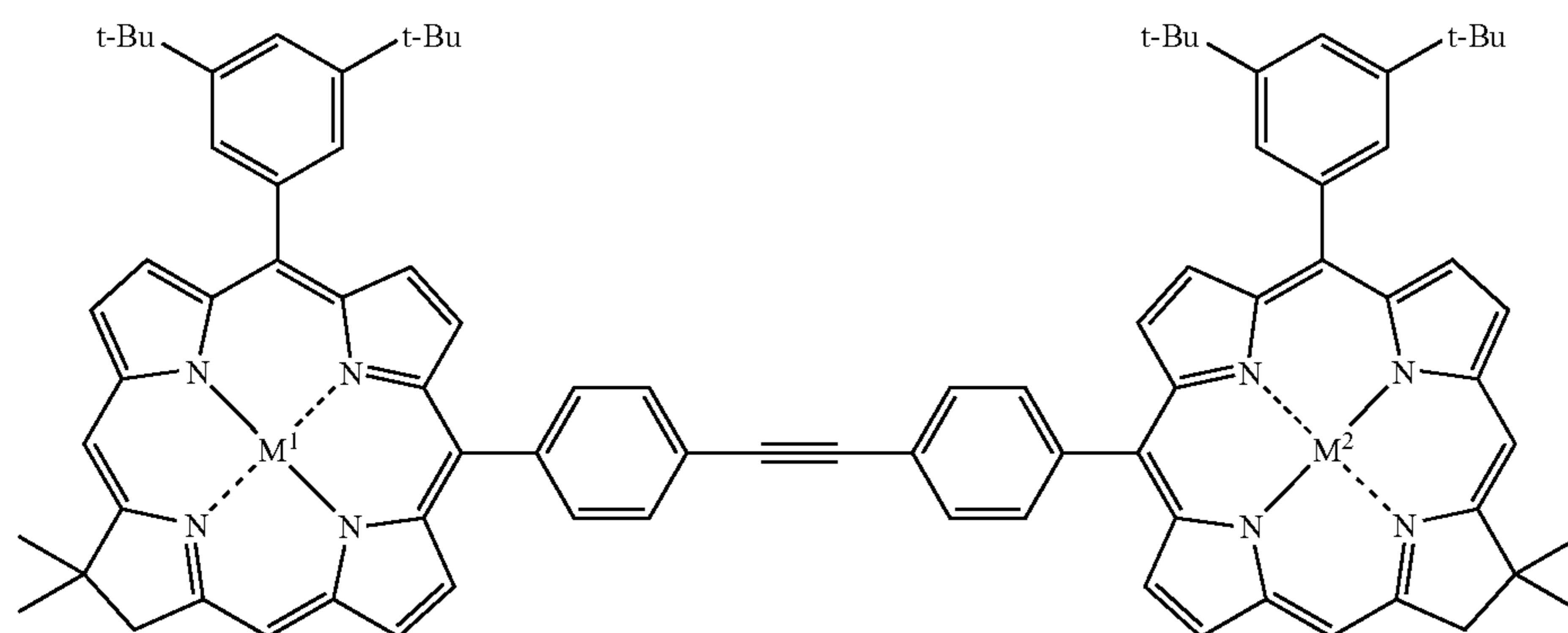
Scheme 11
