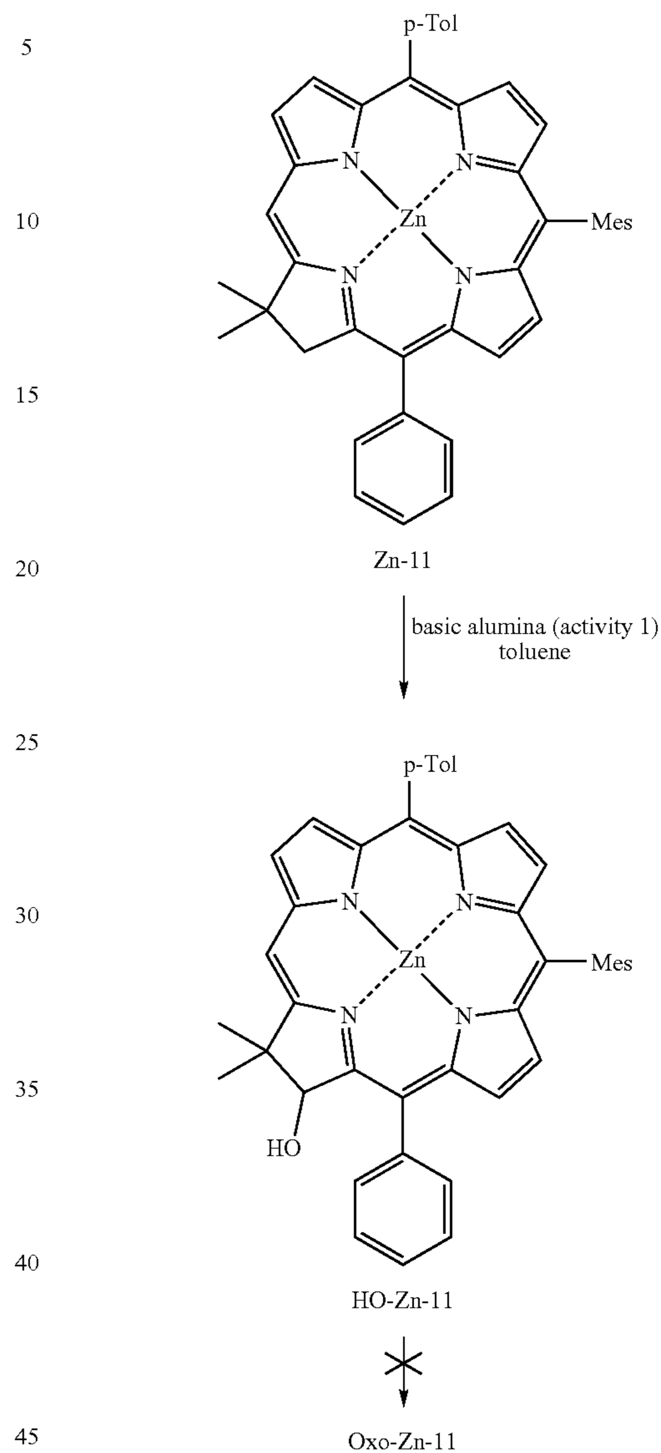
Scheme 7
