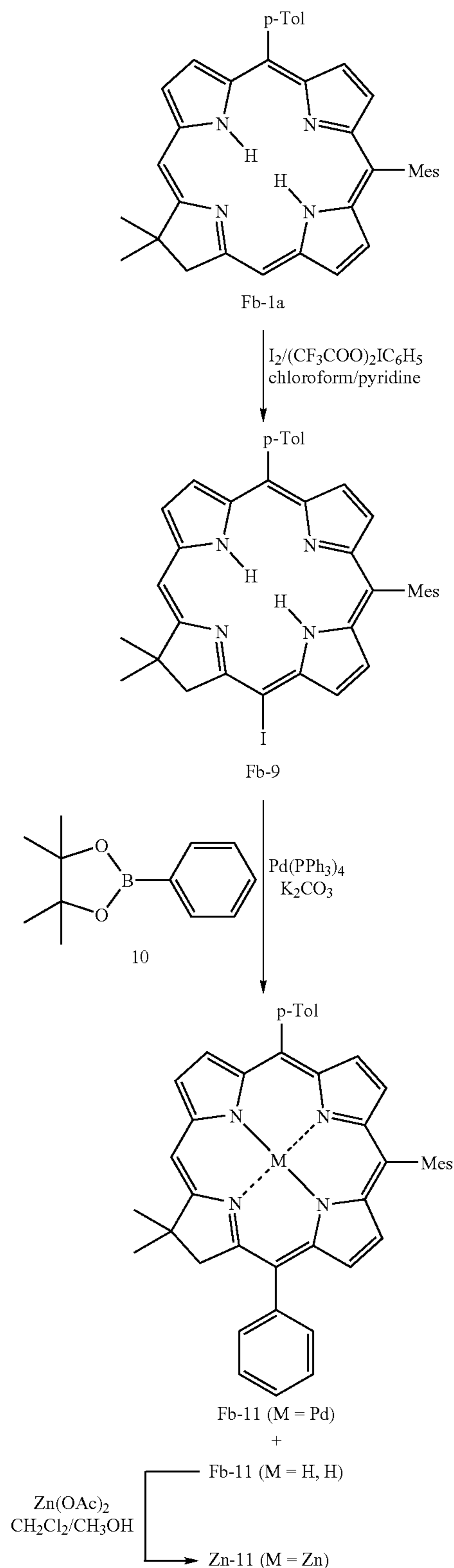
Scheme 6
