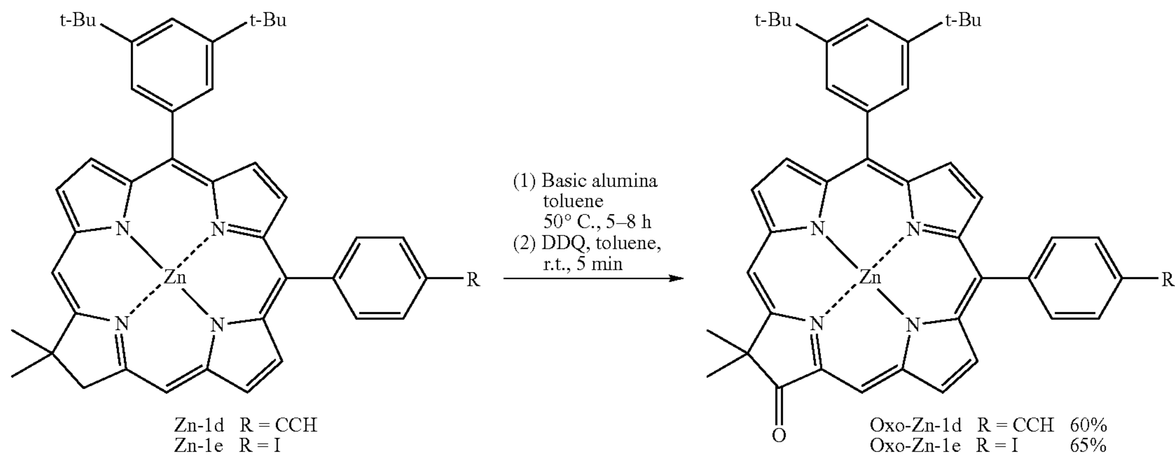
Scheme 3
