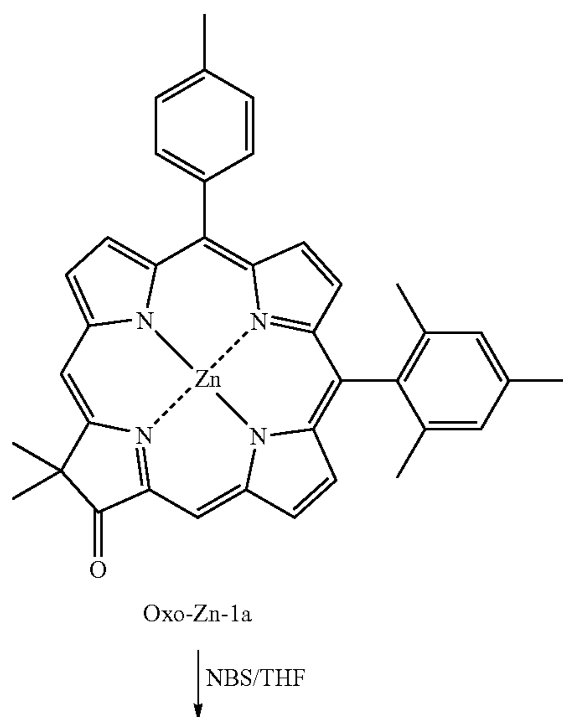
Scheme 10
