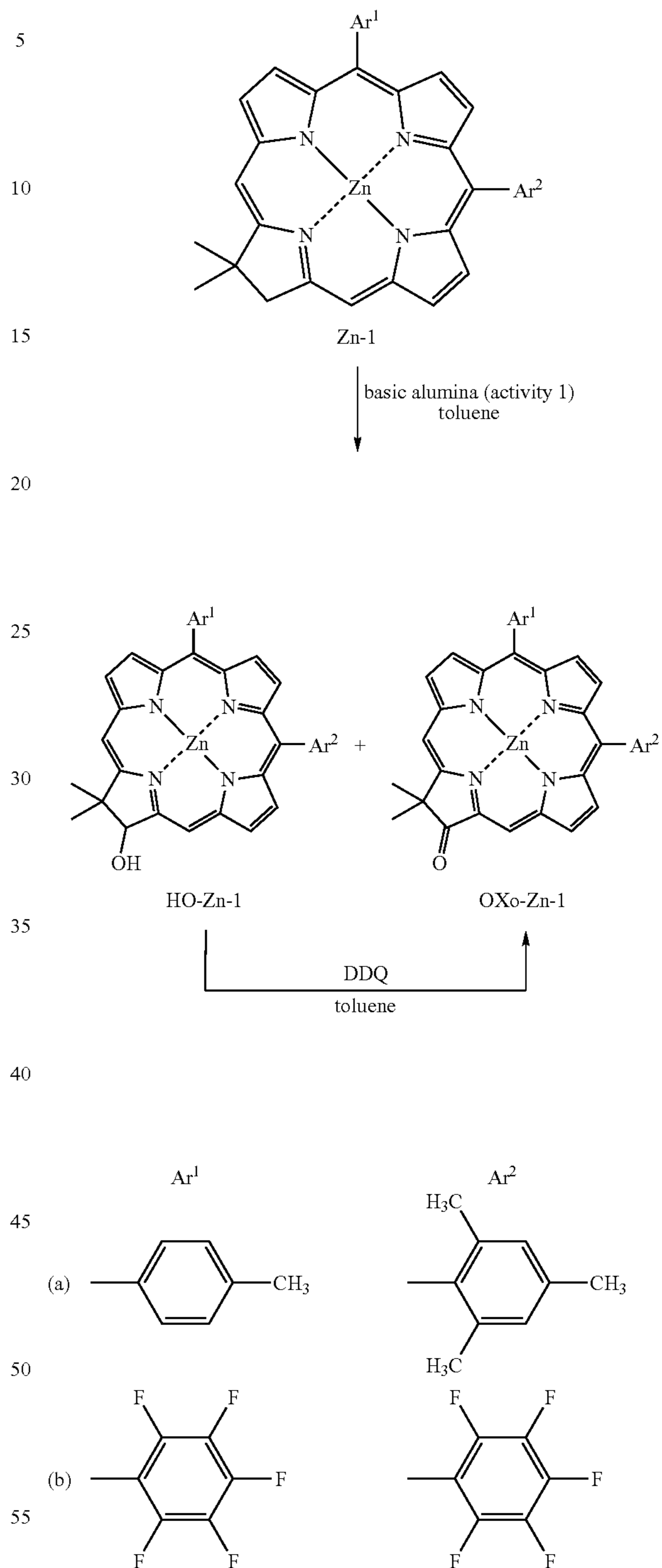
Scheme 1
