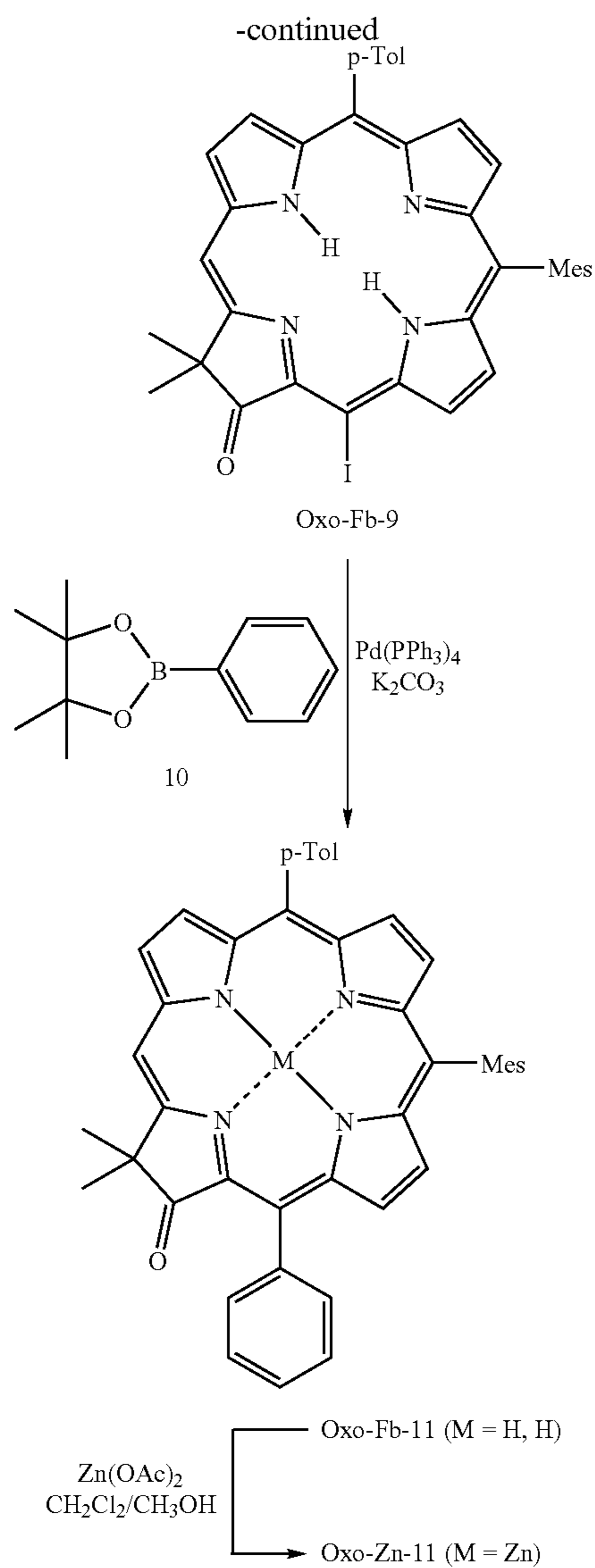
Scheme 10
