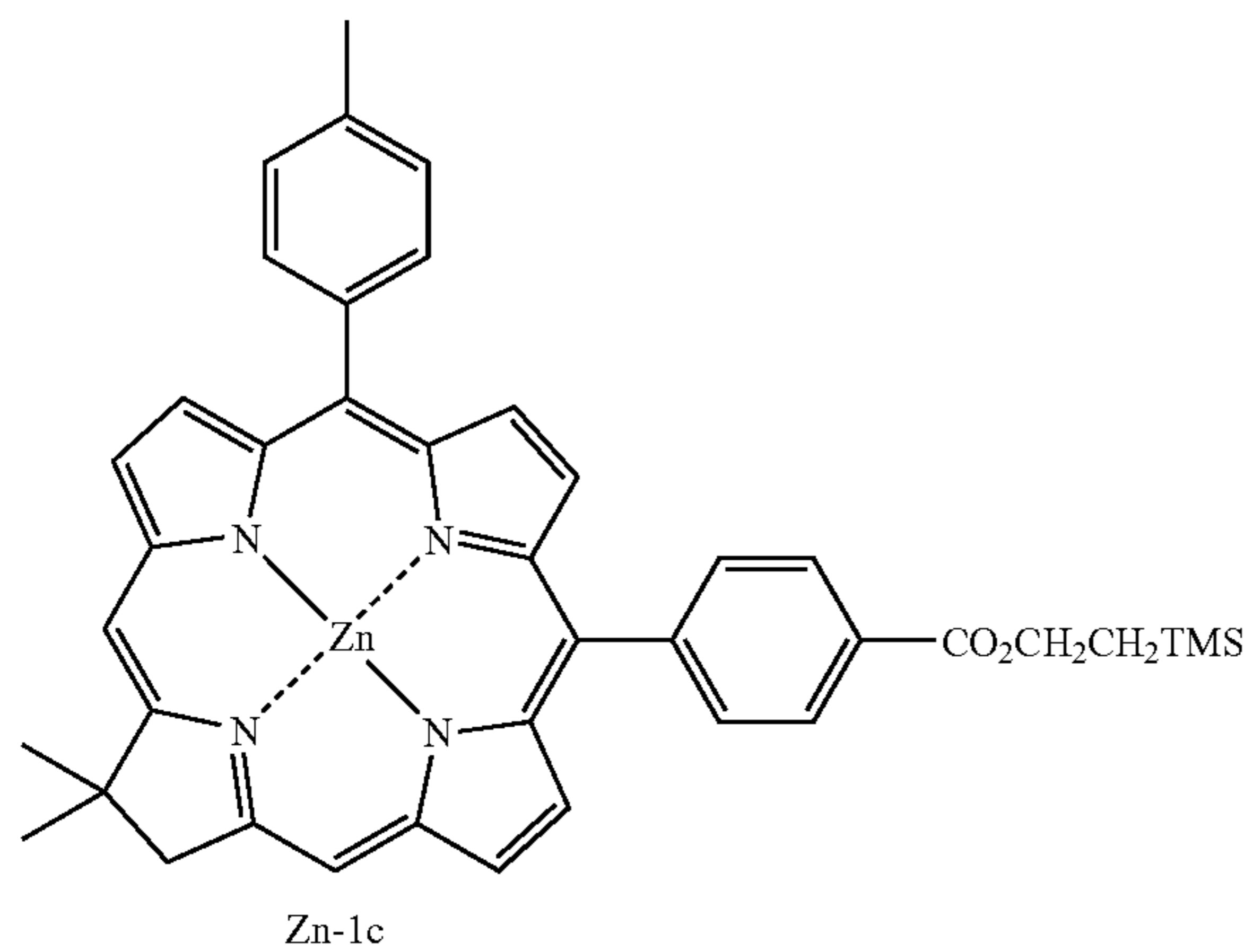
Scheme 2
