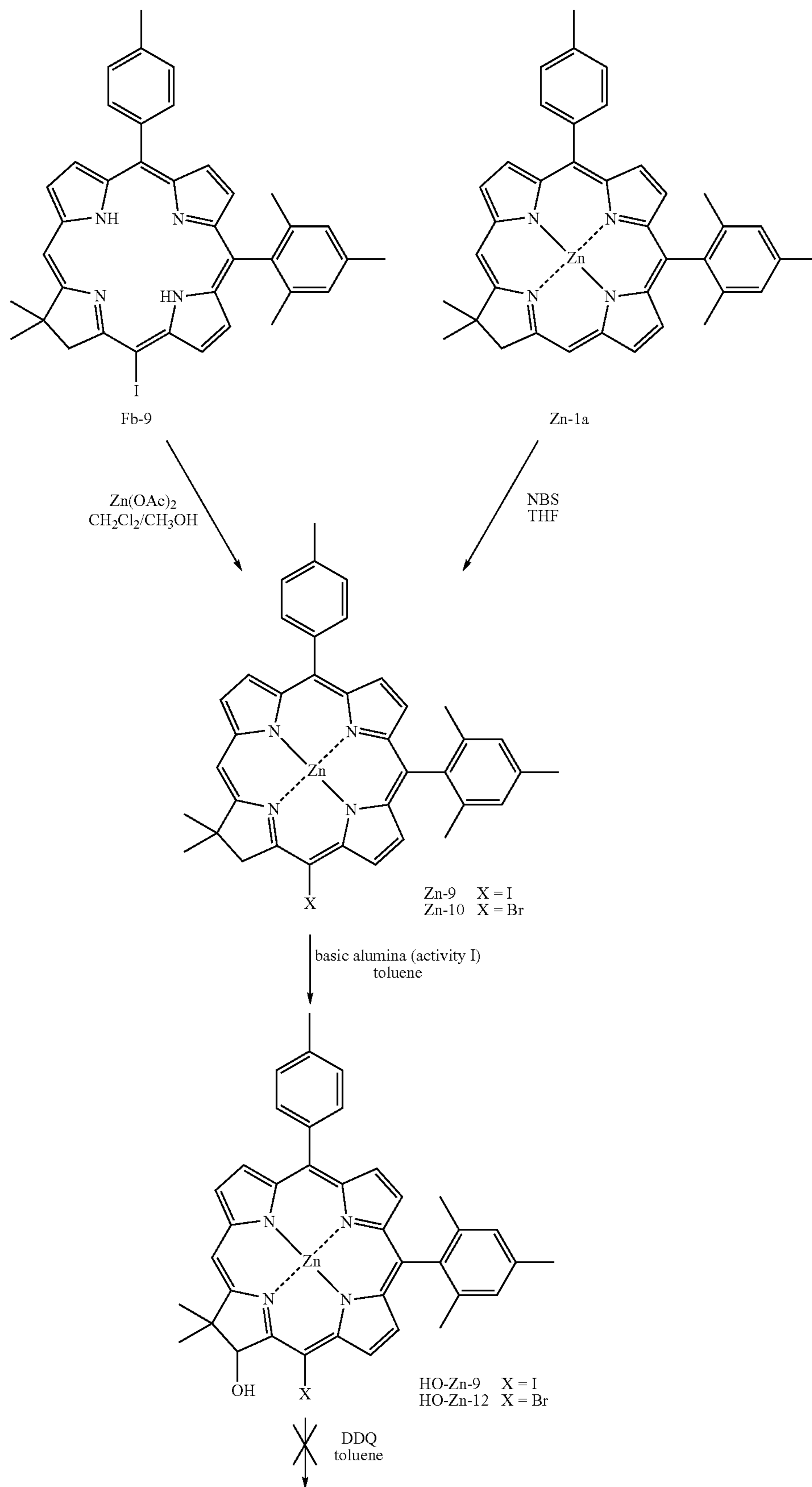
Scheme 8
