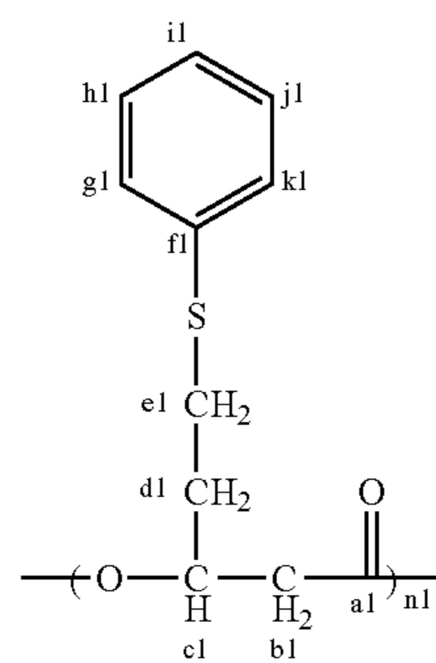
1 H-NMR assignment result
