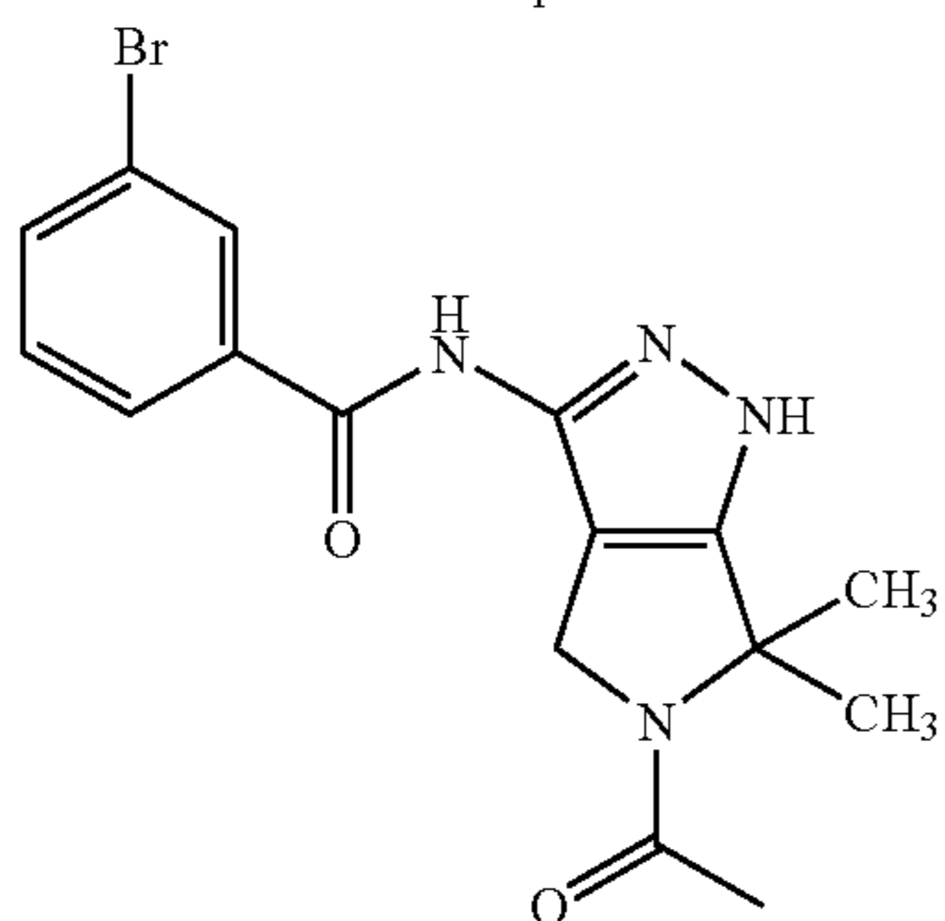
Compound 2
