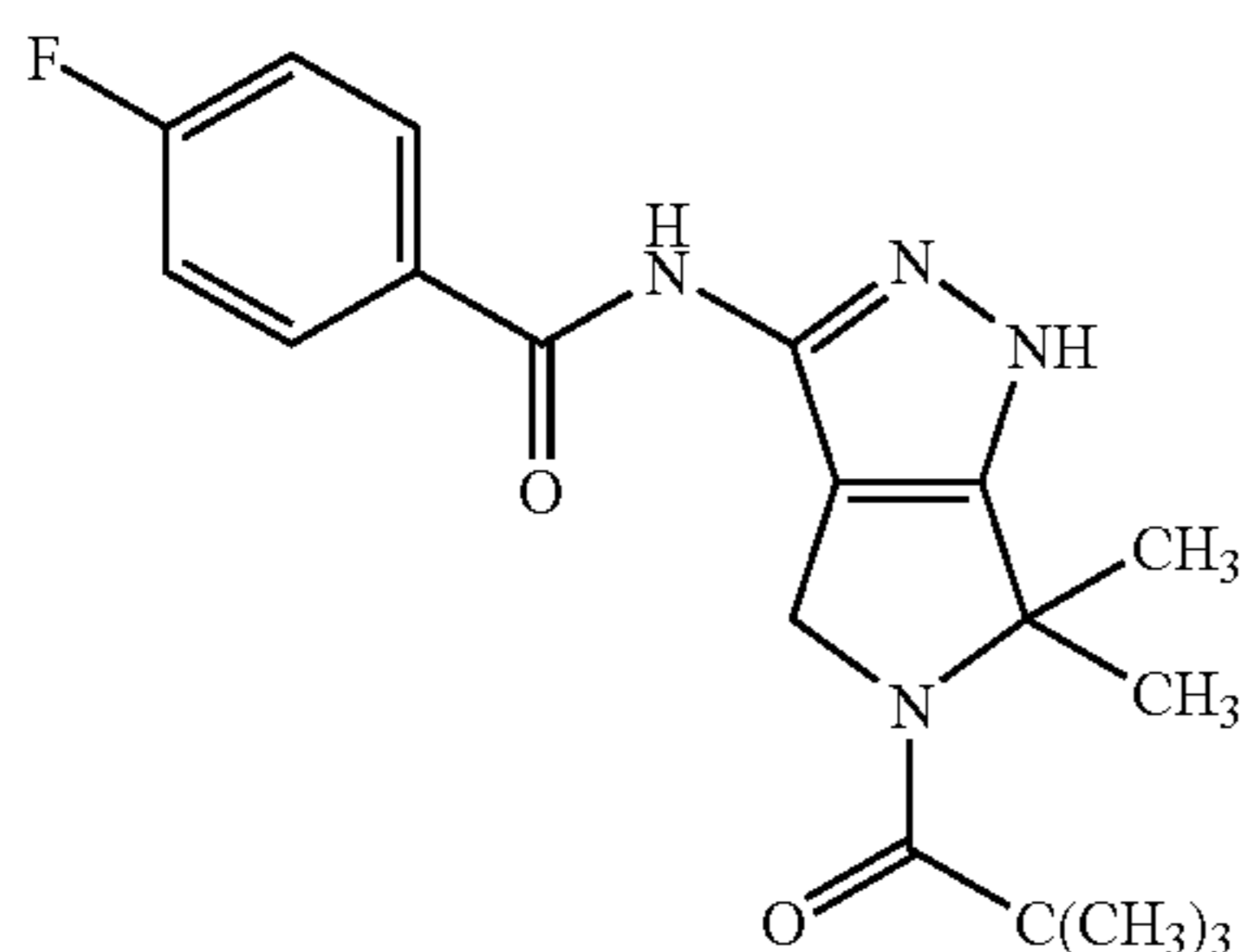
Compound 1
