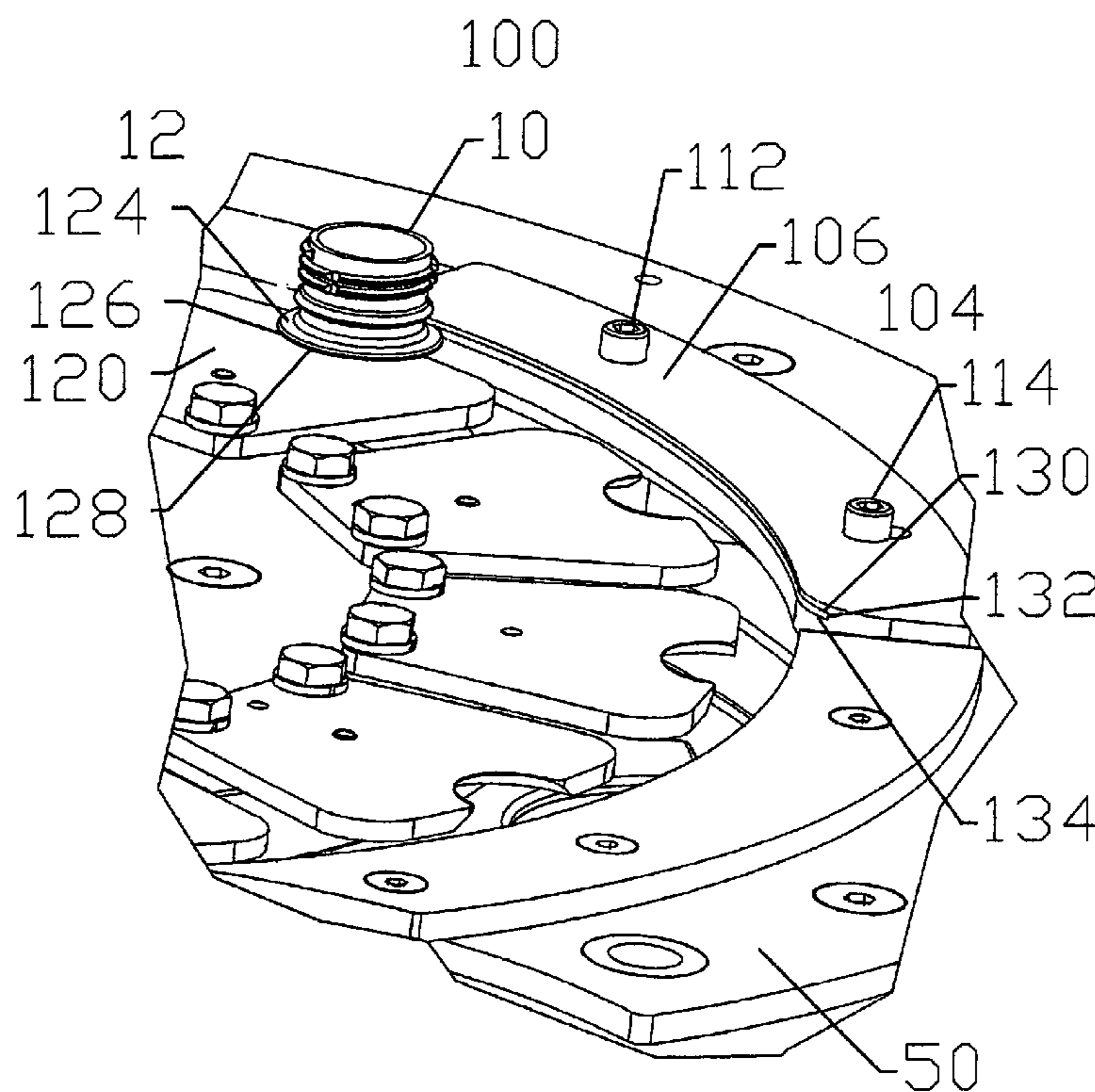
[DETAIL D]
