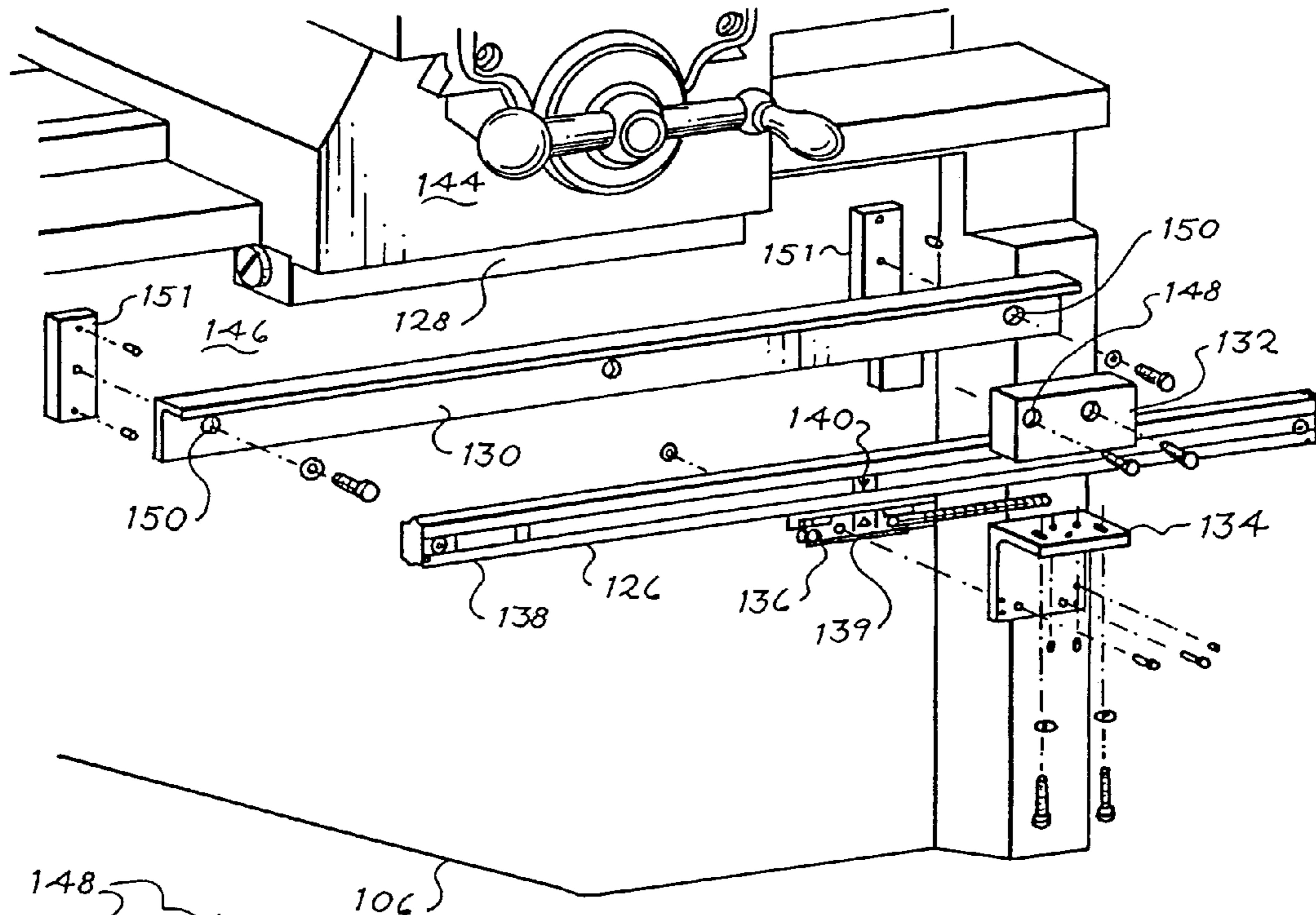
Fig. 6 (PRIOR ART)
