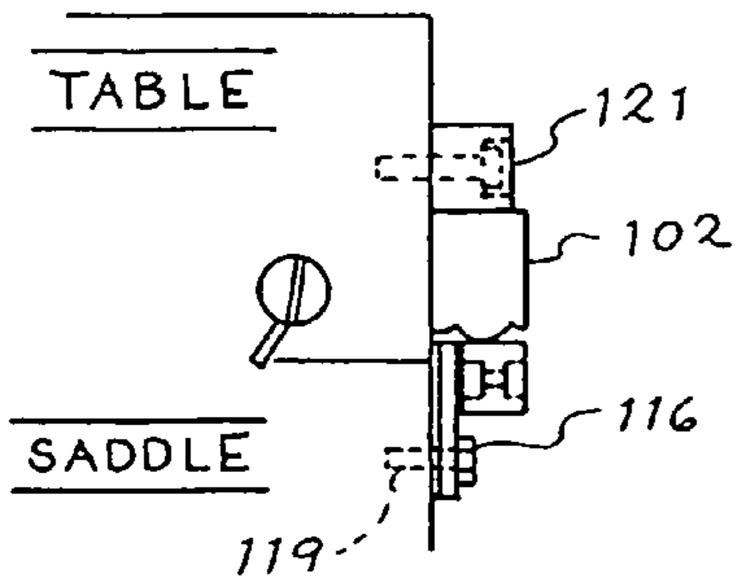
Fig. 5 (PRIOR ART)
