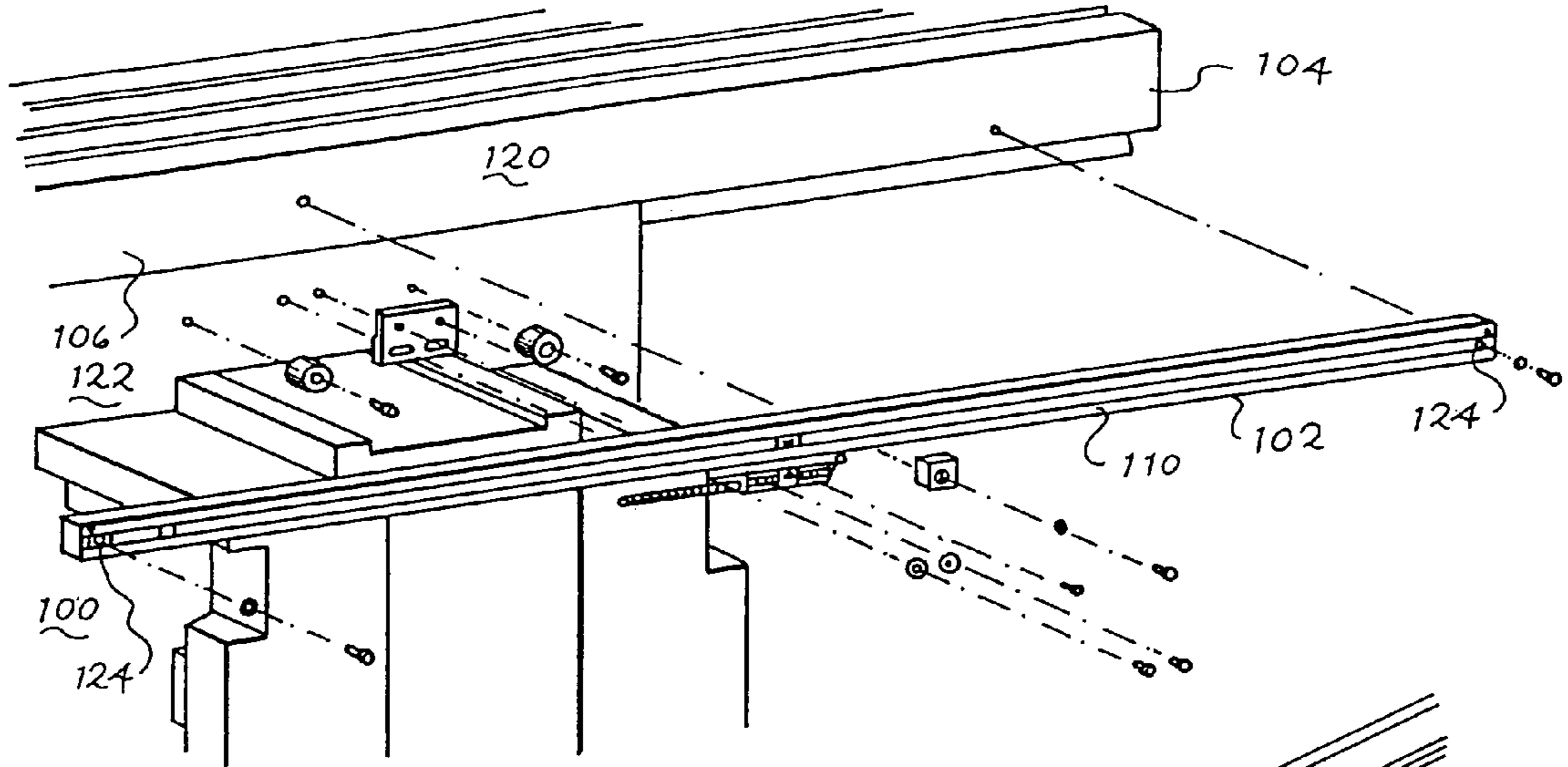
Fig. 1 (PRIOR ART)
