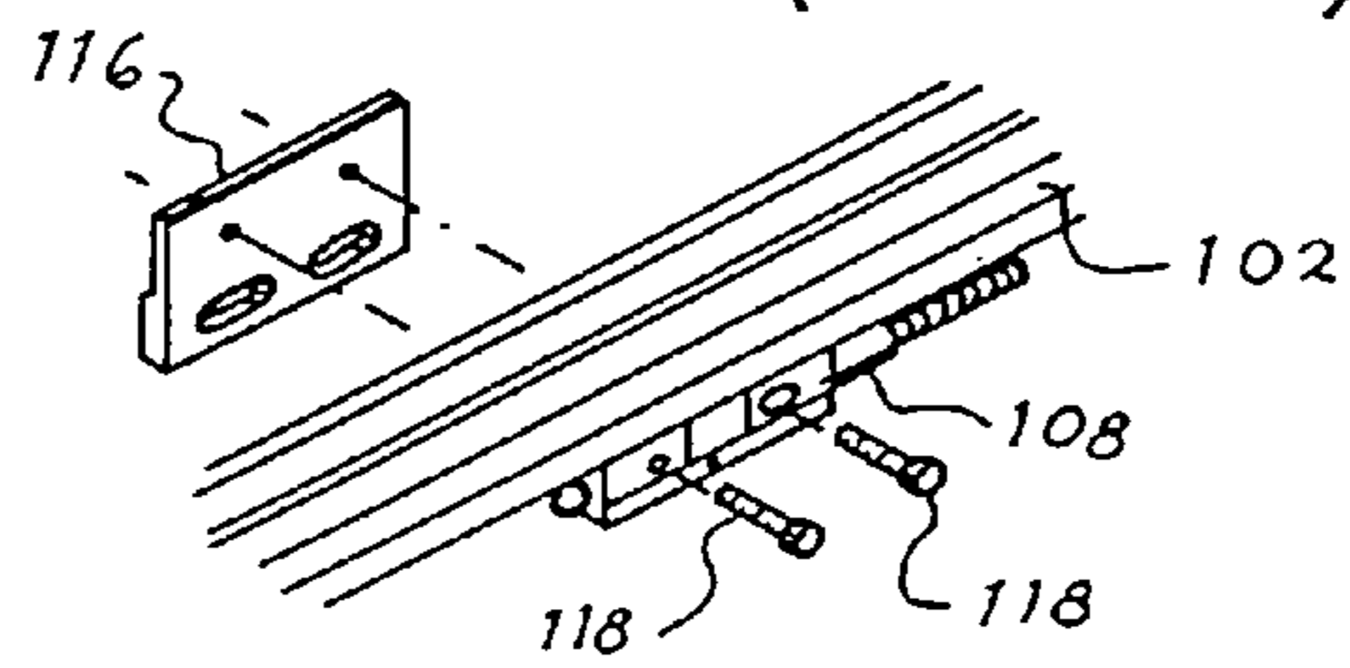
Fig. 4 (PRIOR ART)
