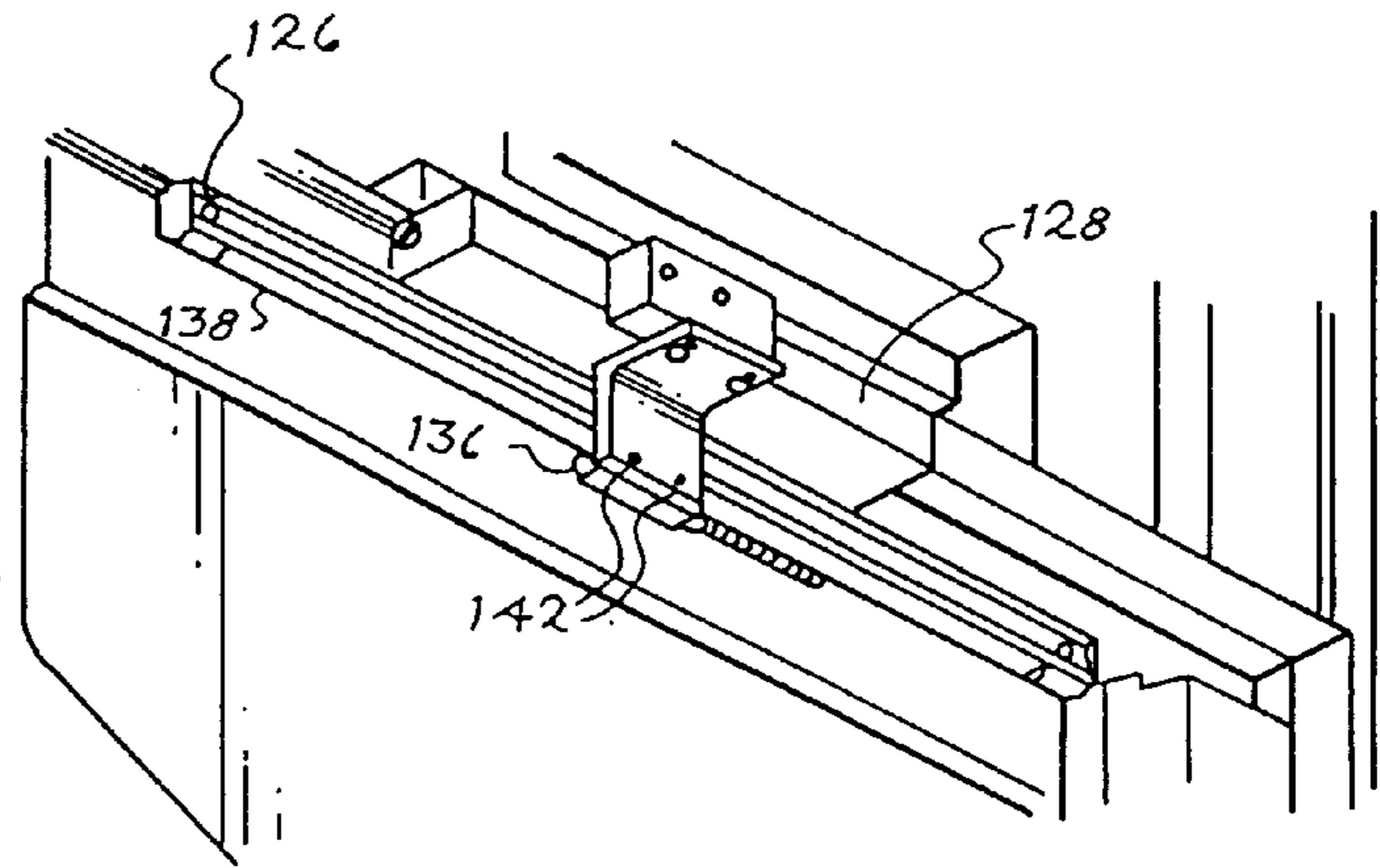
Fig. 8 (PRIOR ART)
