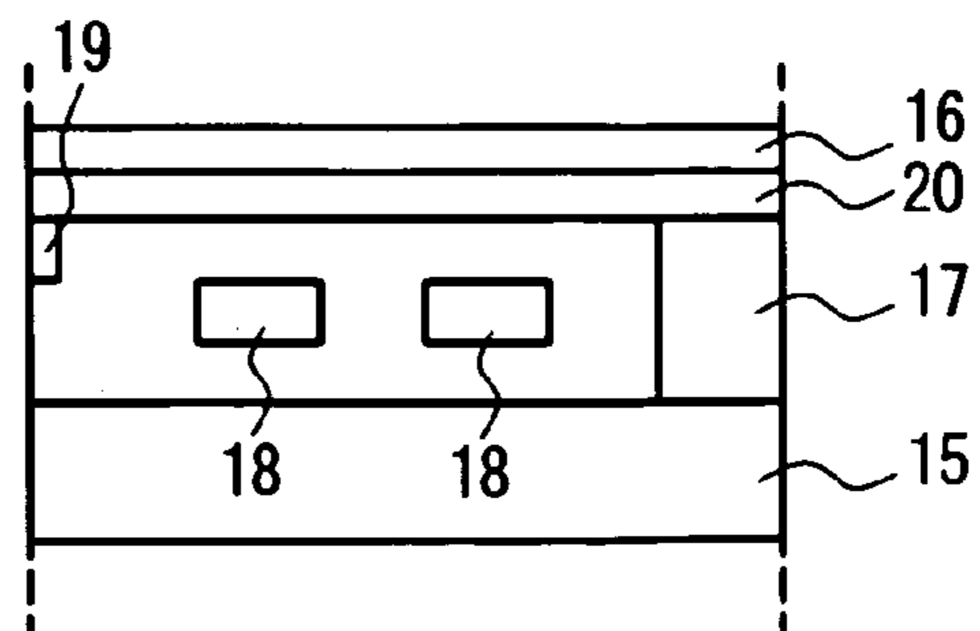
FIG. 9D AIR BEARING SURFACE
