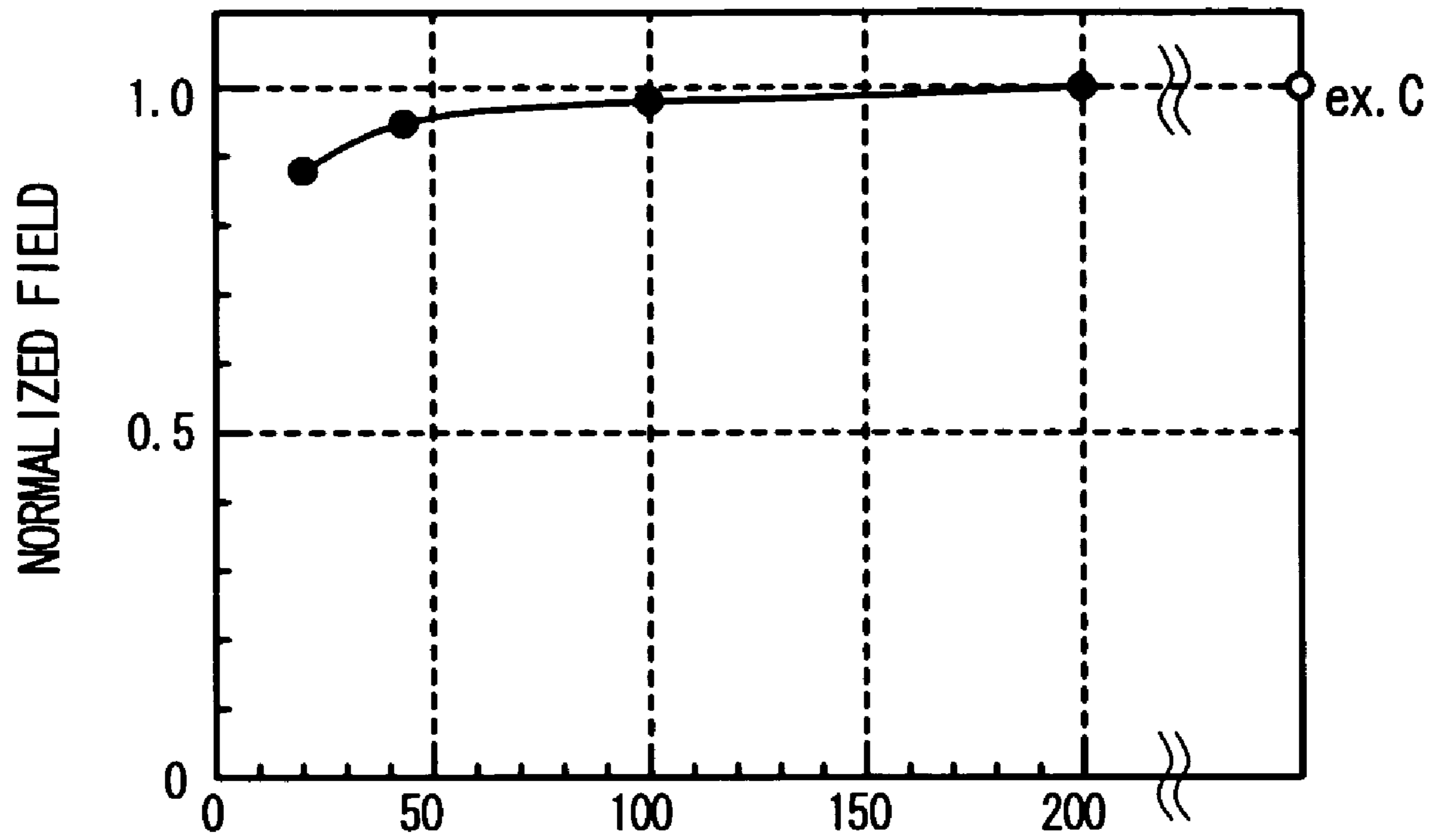
THE DISTANCE BETWEEN WRITE POLE AND THE 3RD MAGNETIC POLE
