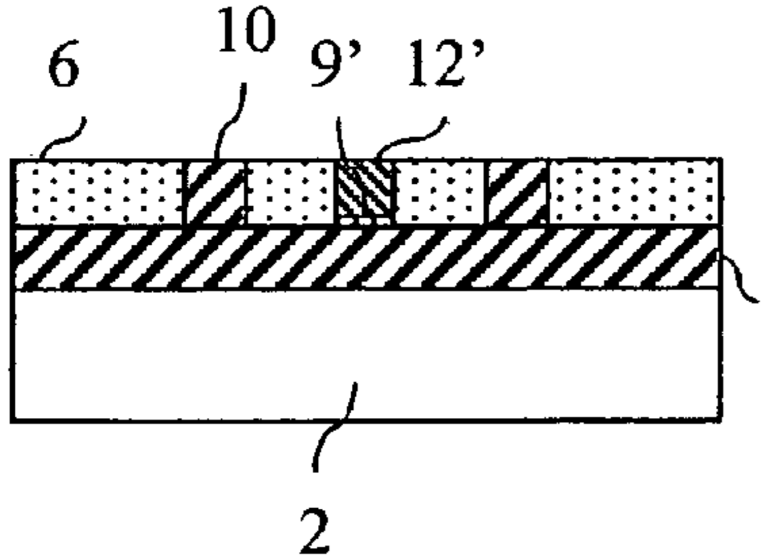
SECTION AA
