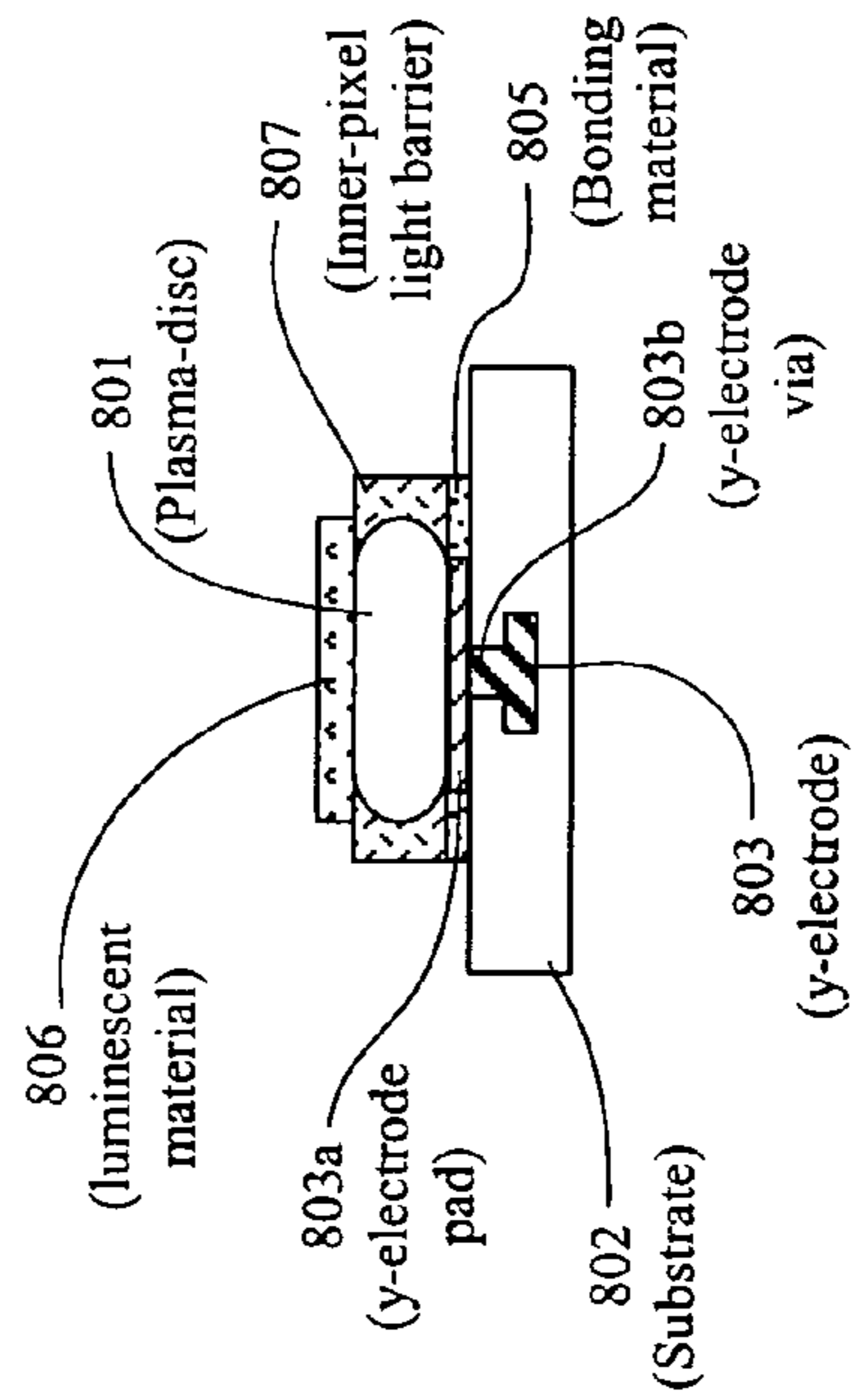
Figure 8A Section A-A View
