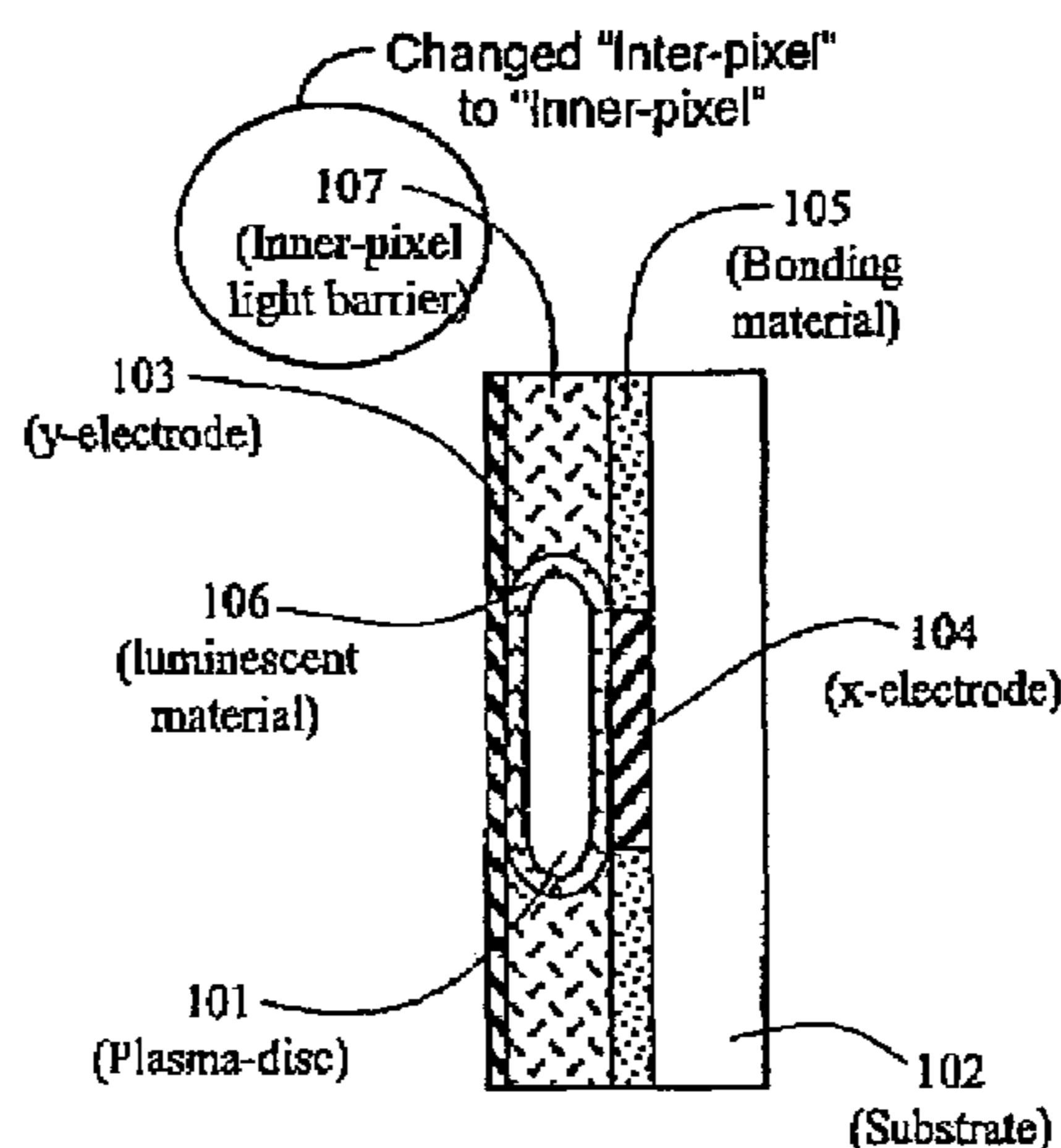
Section B-B View
