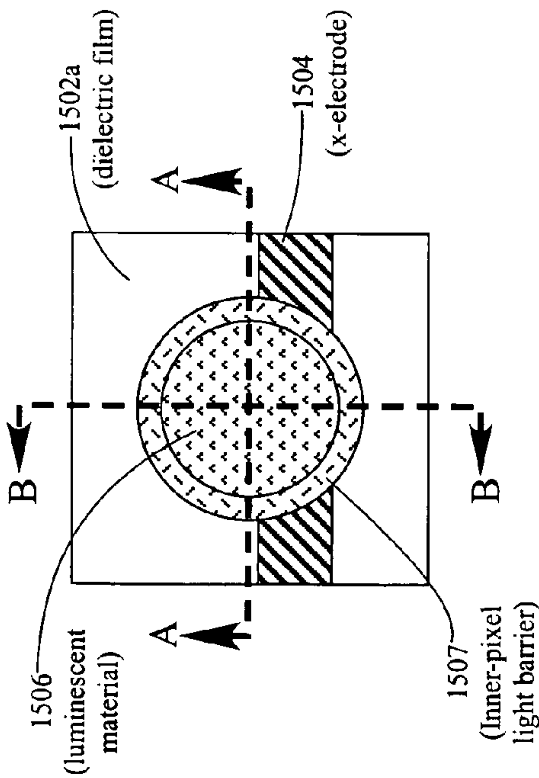
Figure 15 Two Electrodes Top View
