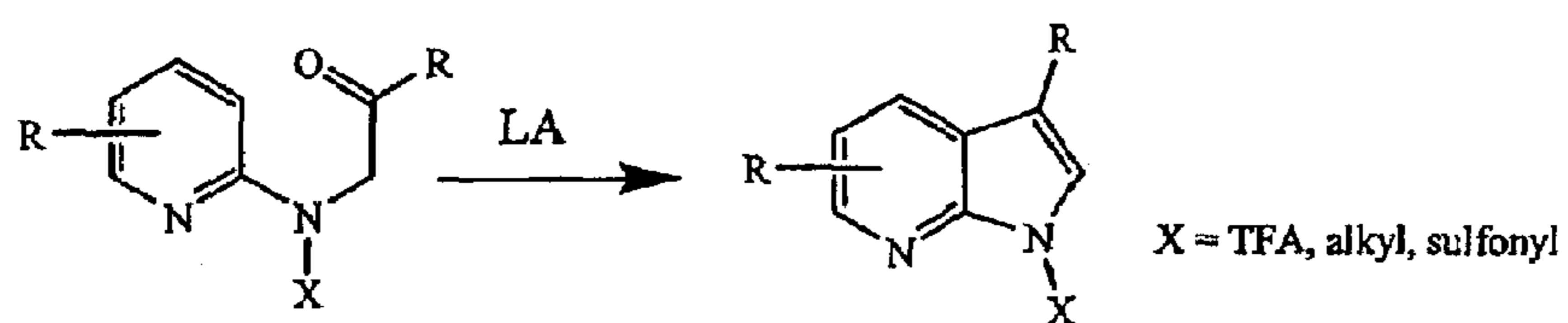
Scheme V: Acid Catalyzed Cyclization
