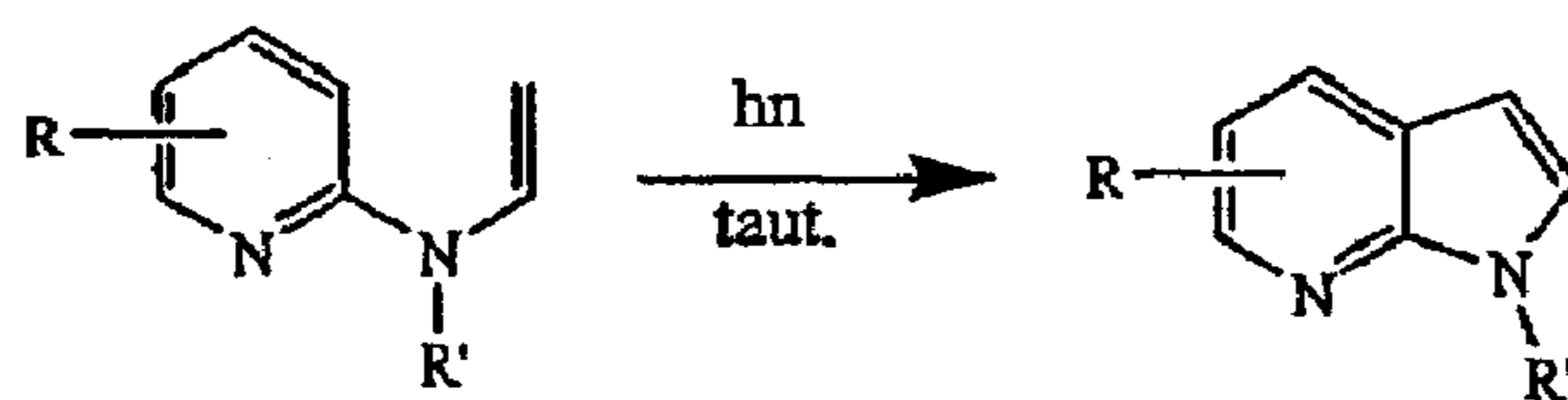
Scheme V: Acid Catalyzed Cyclization
