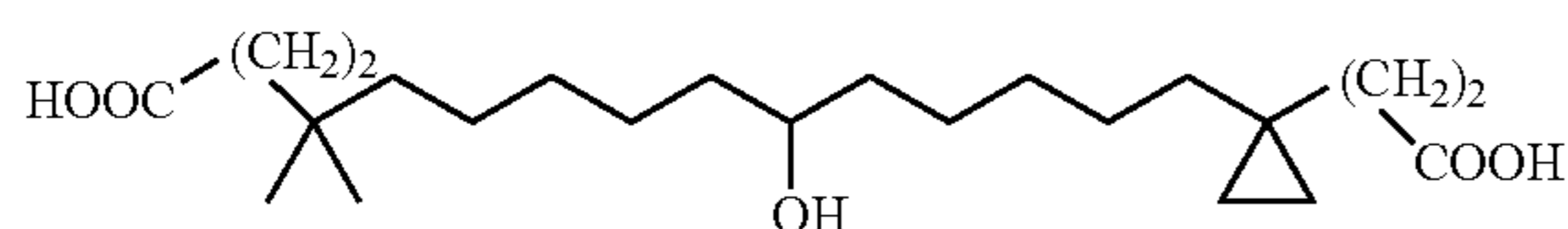
3-[1-(6,15-Dihydroxy-12,12-dimethyl-pentadecyl)-cyclopropyl]-propionic acid
