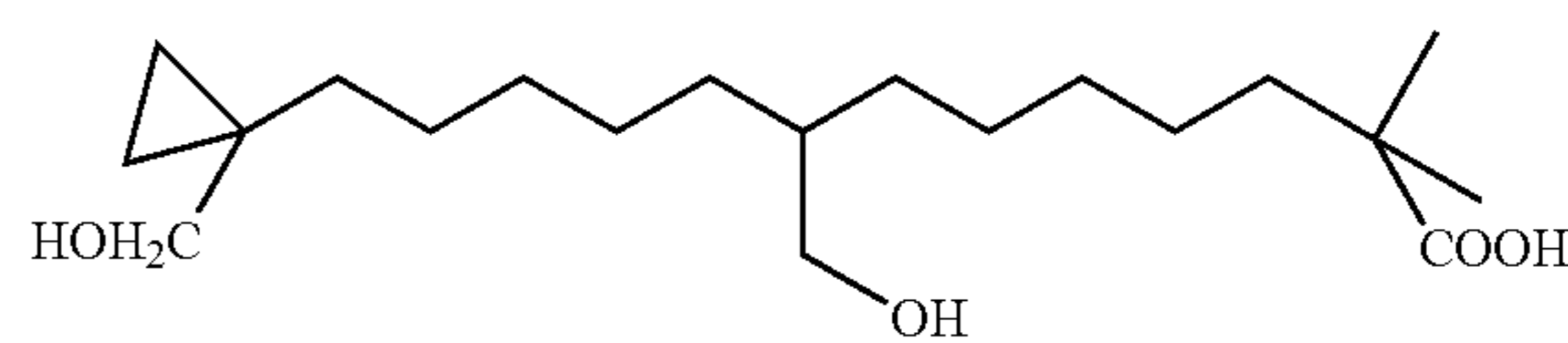
8-Hydroxymethyl-13-(1-hydroxymethyl-cyclopropyl)-2,2-dimethyl-tridecanoic acid
