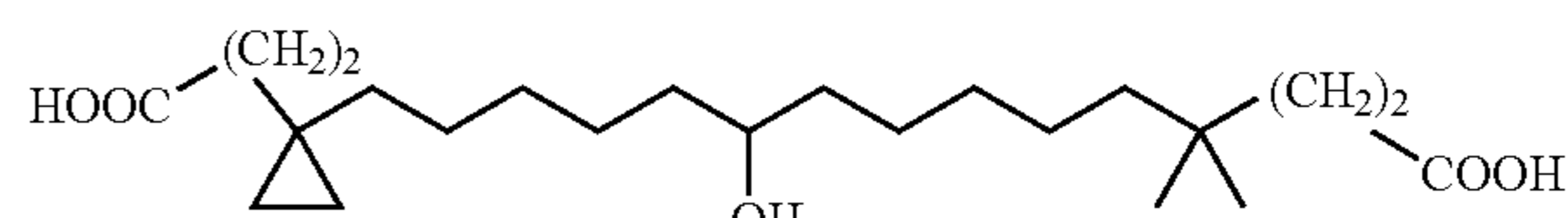
15-[1-(2-Carboxyethyl)-cyclopropyl]-10-hydroxy-4,4-dimethyl-tridecanoic acid
