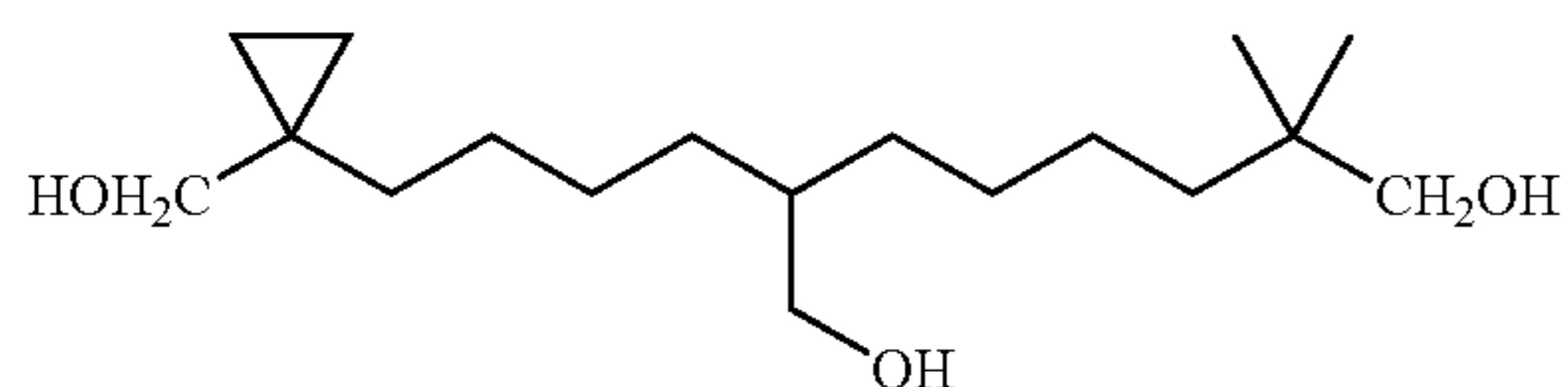
7-[4-(1-Hydroxymethyl-cyclopropyl)-butyl] 2,2-dimethyl-octane-1,8-diol
