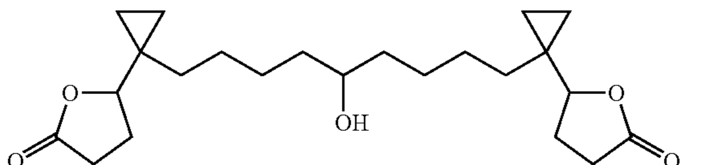
1,9-Bis-[1-(2-oxo-tetrahydrofuran-5-yl)-cyclopropyl]-nonan-5-ol
