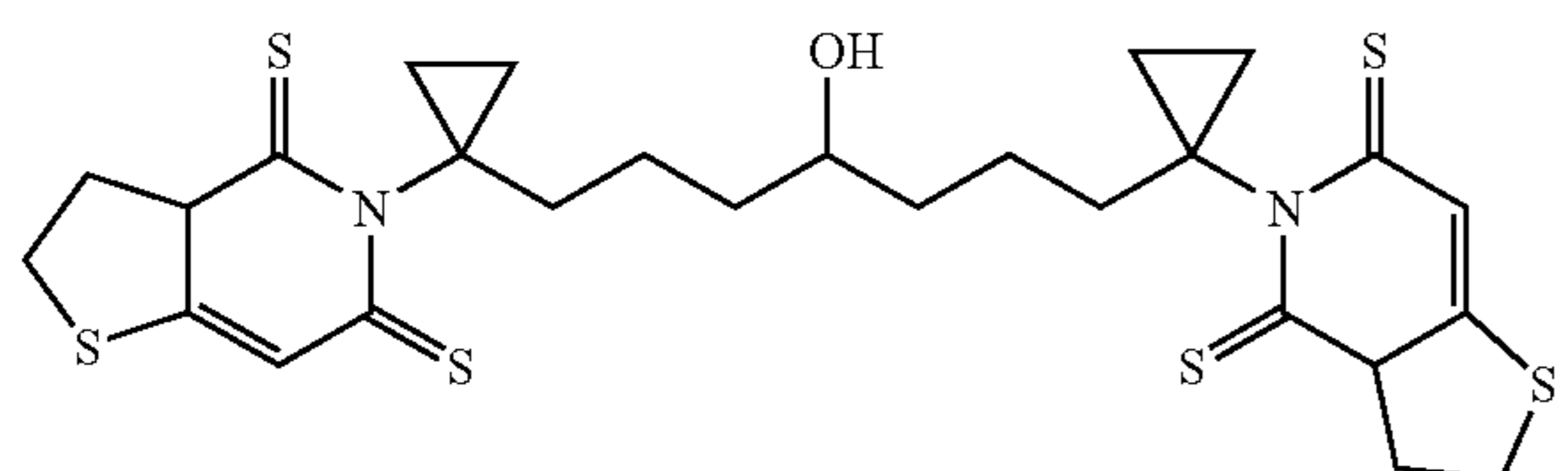
1,7-Bis-(4,6-dithioxo-2,3,3a,6-tetrahydro-4H-thieno[3,2-c]pyridin-5-yl)-1,7-bis-(cyclopropyl)-6-hydroxy-undecane
