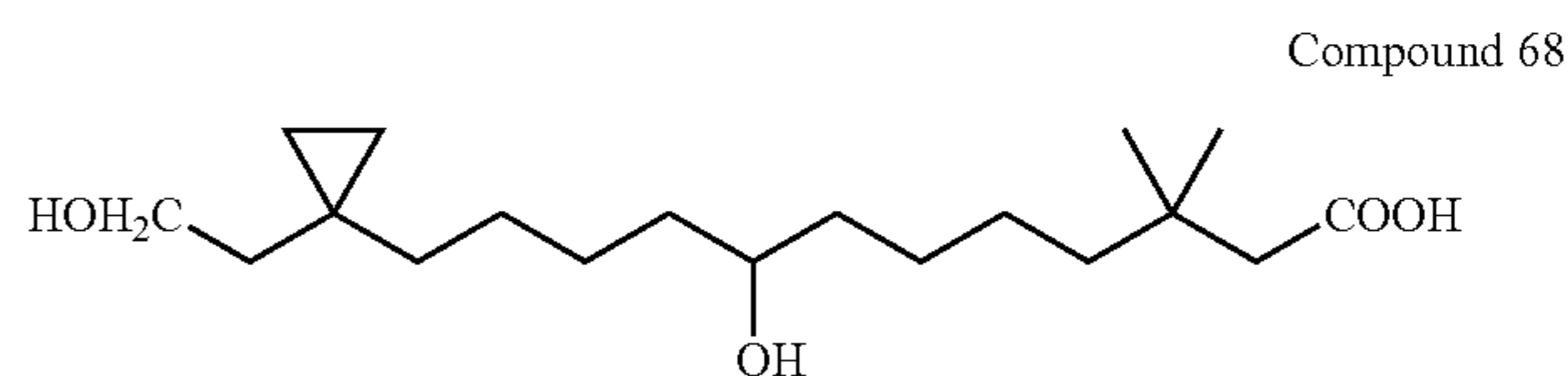
8-Hydroxy-12-[1-(2-hydroxy-ethyl)-cyclopropyl]-3,3-dimethyl-dodecanoic acid
