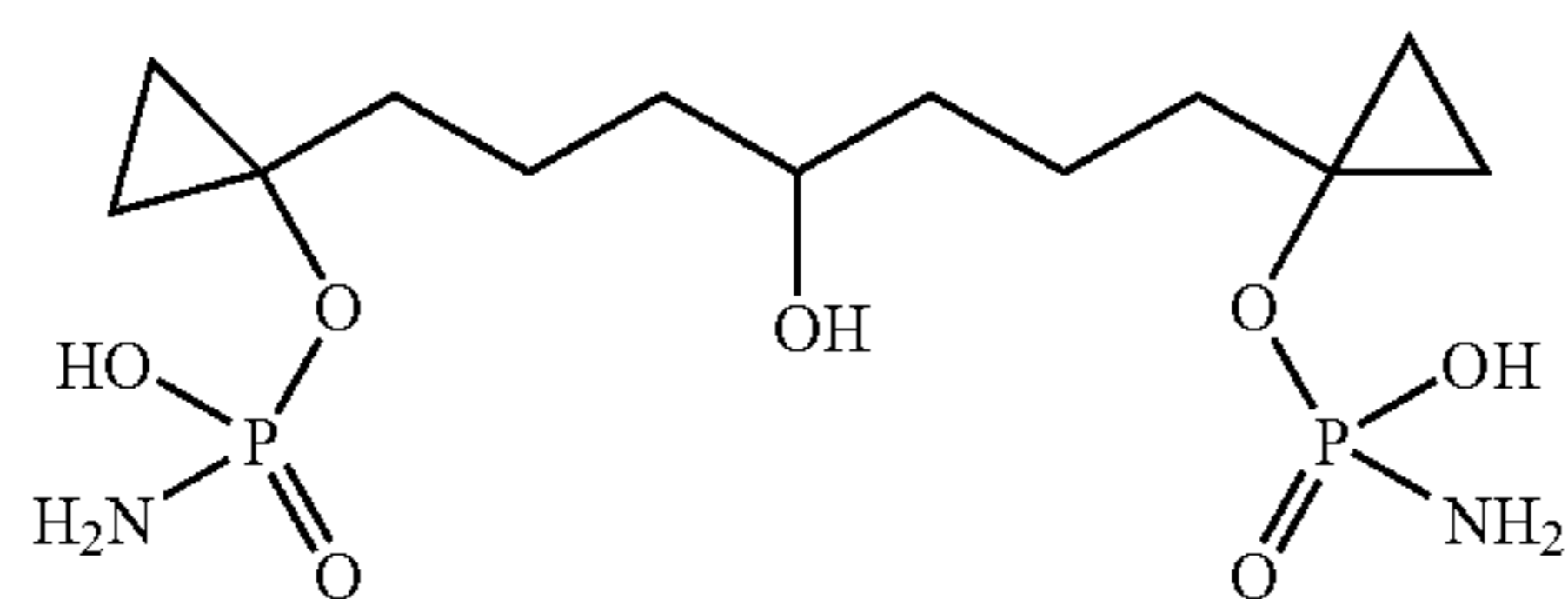
1,7-Bis-(1-phosponamid-cyclopropyl)-4-hydroxy-heptane
