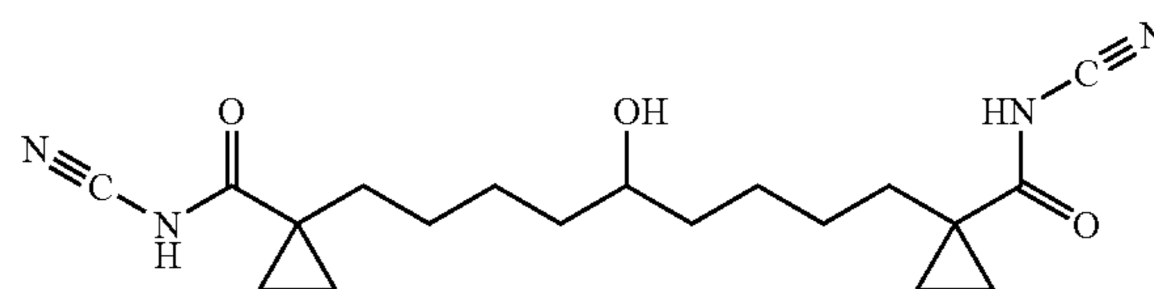
1,7-Bis-(1-dicyanimido-cyclopropyl)-5-hydroxy-nonane
