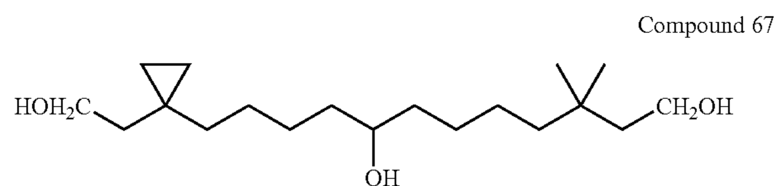
12-[1-(2-Hydroxy-ethyl)-cyclopropyl]-3,3-dimethyl-dodecane-1,8-diol
