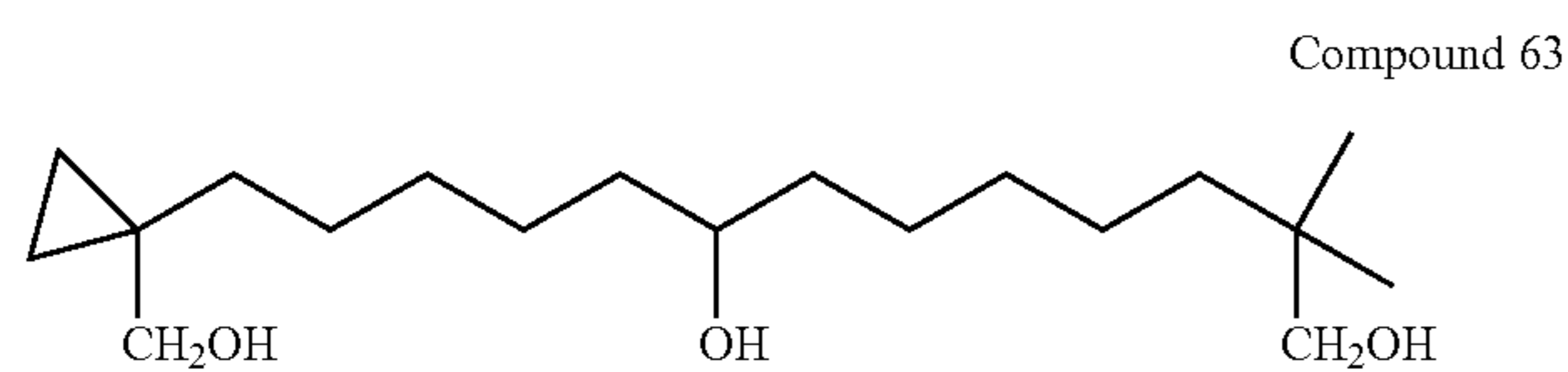
13-(1-Hydroxymethyl-cyclopropyl)-2,2-dimethyl-tridecane-1,8-diol
