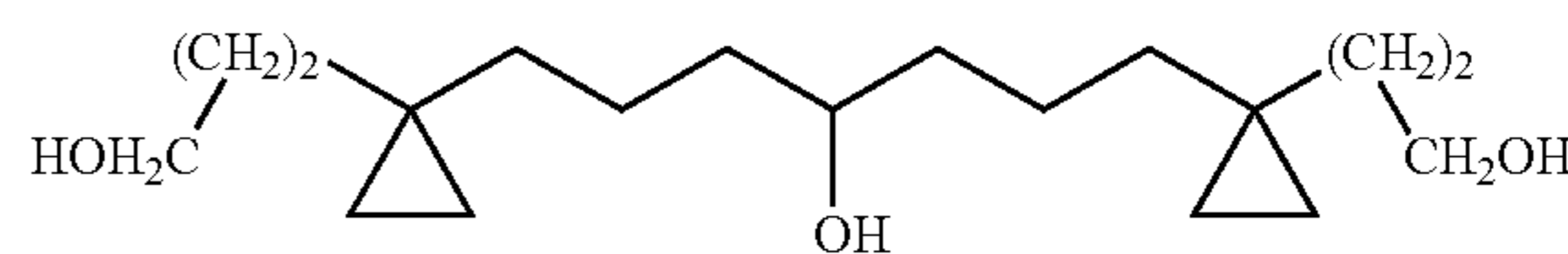
1,7-Bis-[1-(3-hydroxy-propyl)-cyclopropyl]-heptan-4-ol
