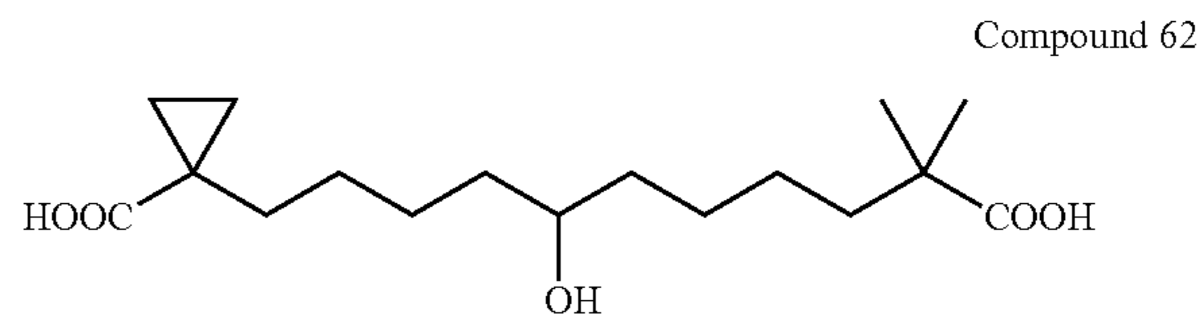
1-(10-Carboxy-5-hydroxy-10-methyl-undecyl)-cyclopropanecarboxylic acid
