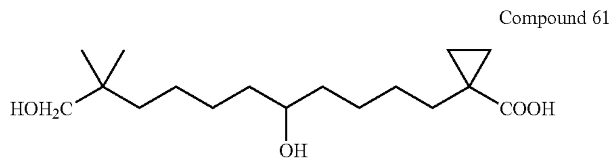
1-(5,11-Dihydroxy-10,10-dimethyl-undecyl)-cyclopropanecarboxylic acid
