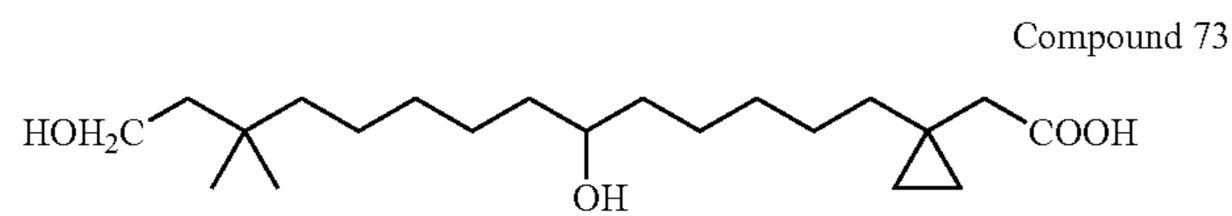
[1-(6,14-Dihydroxy-12,12-dimethyl-tetradecyl)-cyclopropyl]-acetic acid
