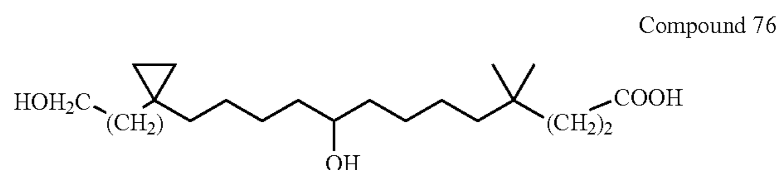
4,4-Dimethyl-9-hydroxy-13-[1-(3-hydroxypropyl)-cyclopropyl]-tridecanoic acid
