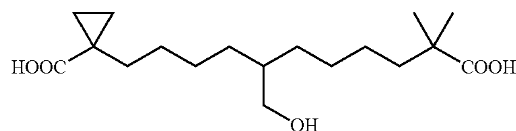
1-(1,0-Carboxy-5-hydroxymethyl-10-methyl-undecyl)-cyclopropanecarboxylic acid
