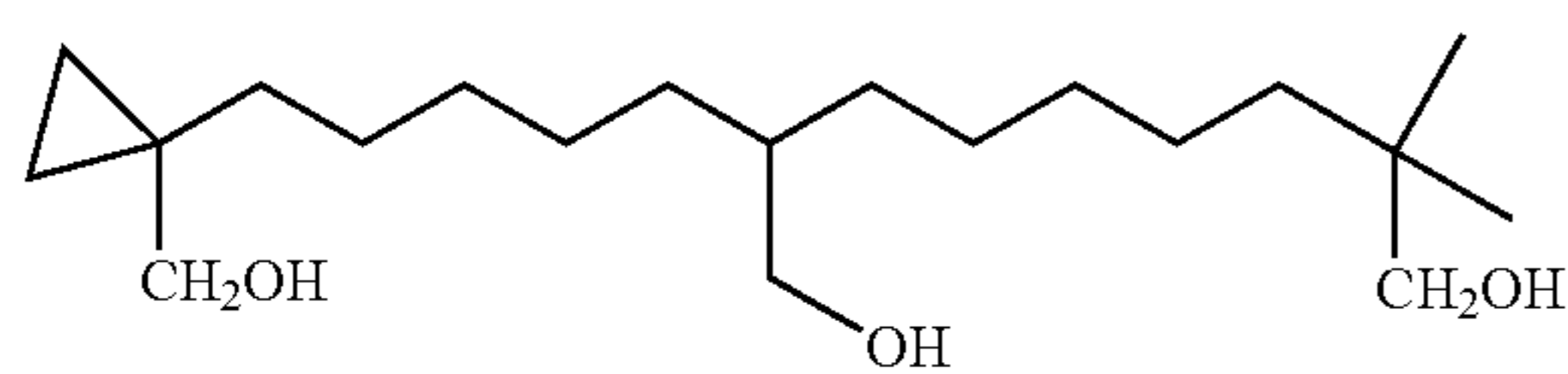
8-[5-(1-Hydroxymethyl-cyclopropyl)-pentyl]-2,2-dimethyl-nonane,1,9-diol
