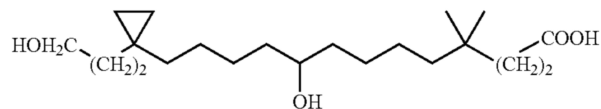
13-[1-(2-Carboxyethyl)-cyclopropyl]-9-hydroxy-4,4-dimethyl-tridecanoic acid
