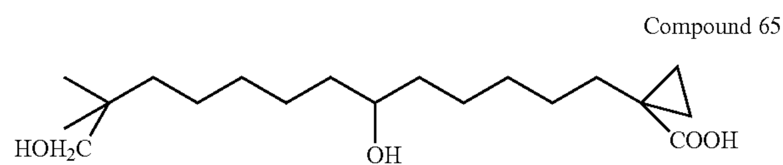
1-(6,13-Dihydroxy-12,12-dimethyl-tridecyl)-cyclopropanecarboxylic acid
