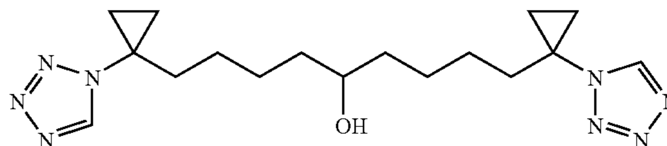
1,9-Bis-(1-tetrazol-1-yl-cyclopropyl)-nonan-5-ol
