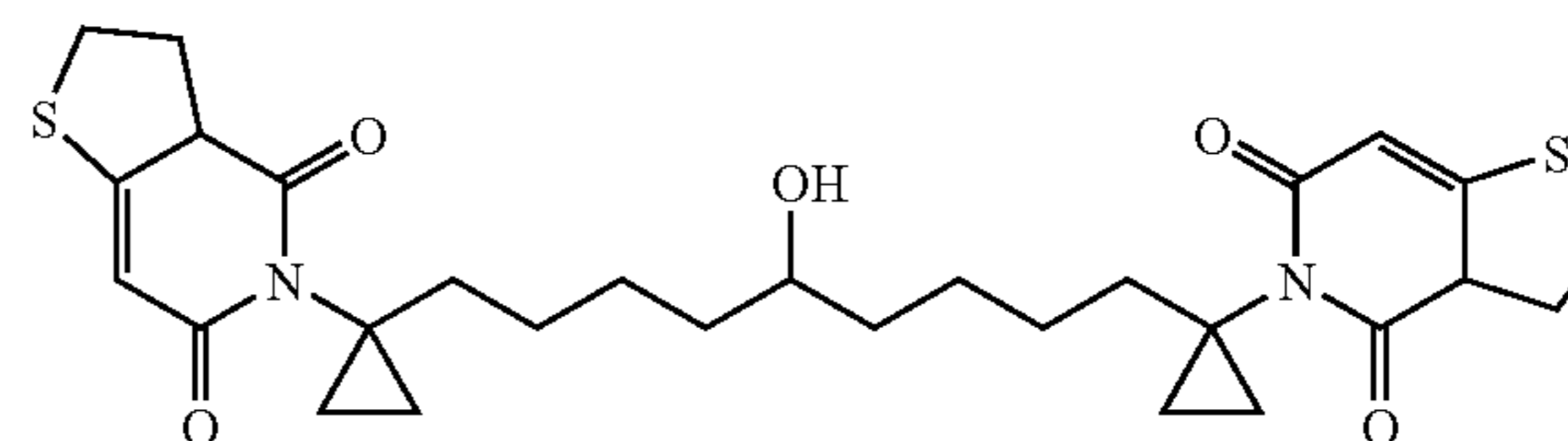
2,9-Bis-(4,6-dioxo-2,3,3a,6-tetrahydro-4H-thieno[3,2-c]pyridin-5-yl)-2,9-bis-(cyclopropyl)-5-hydroxy-nonane
