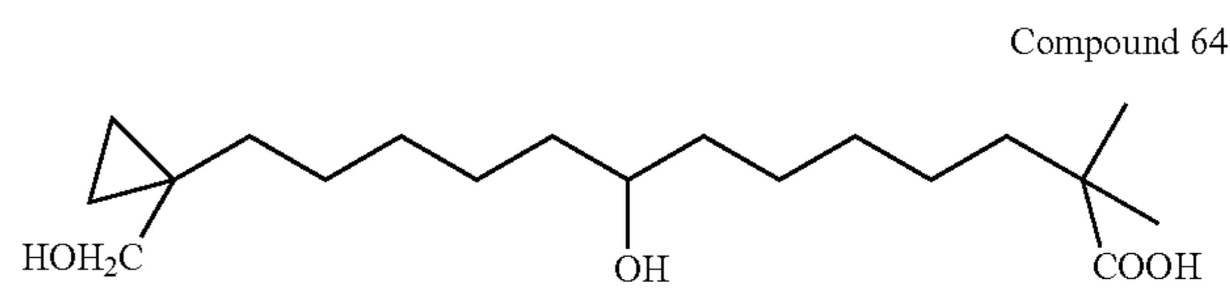
8-Hydroxy-13-(1-hydroxymethyl-cyclopropyl)-2,2-dimethyl-tridecanoic acid
