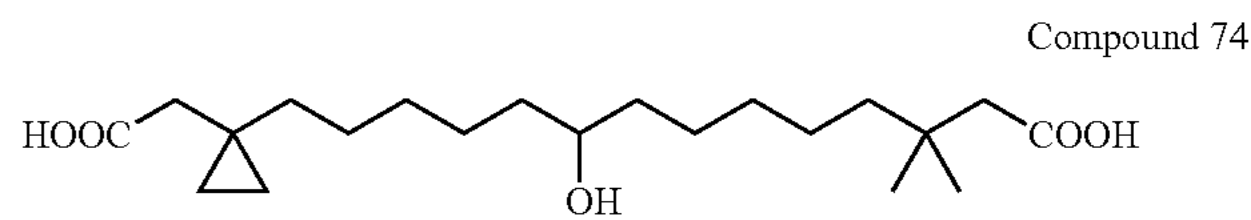
14-(1-Carboxymethyl-cyclopropyl)-9-hydroxy-3,3-dimethyl-tetradecanoic acid
