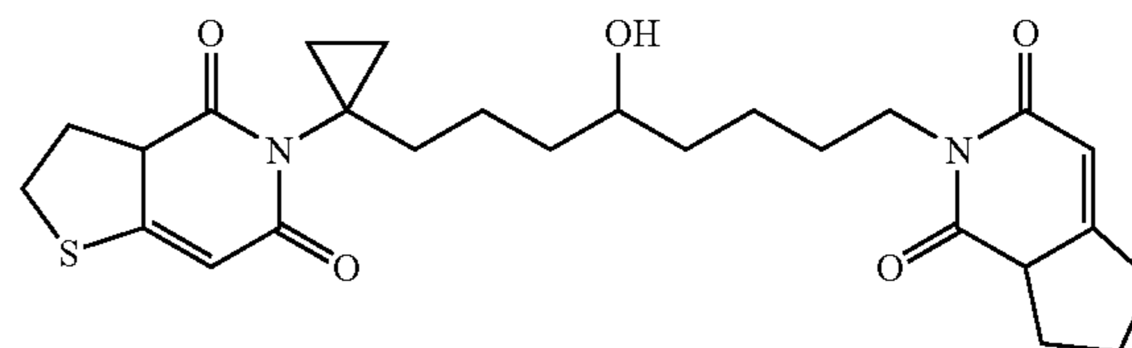
1,7-Bis-(4,6-dioxo-2,3,3a,6-tetrahydro-4H-thieno[3,2-c]-pyridin-5-yl)-1-(cyclopropyl)-6-hydroxy-heptane
