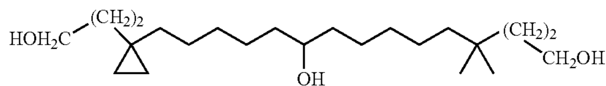
15-[1-(3-Hydroxy-propyl)-cyclopropyl]-4,4-dimethyl-pentadecane-1,10-diol
