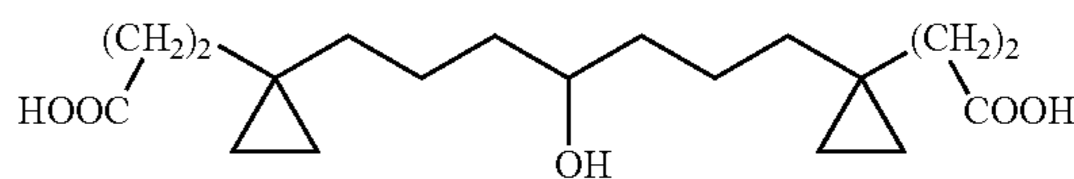
3-(1-(7-[1-(2-Carboxy-ethyl)-cyclopropyl]-4-hydroxy-heptyl)-cyclopropyl)-propionic acid
