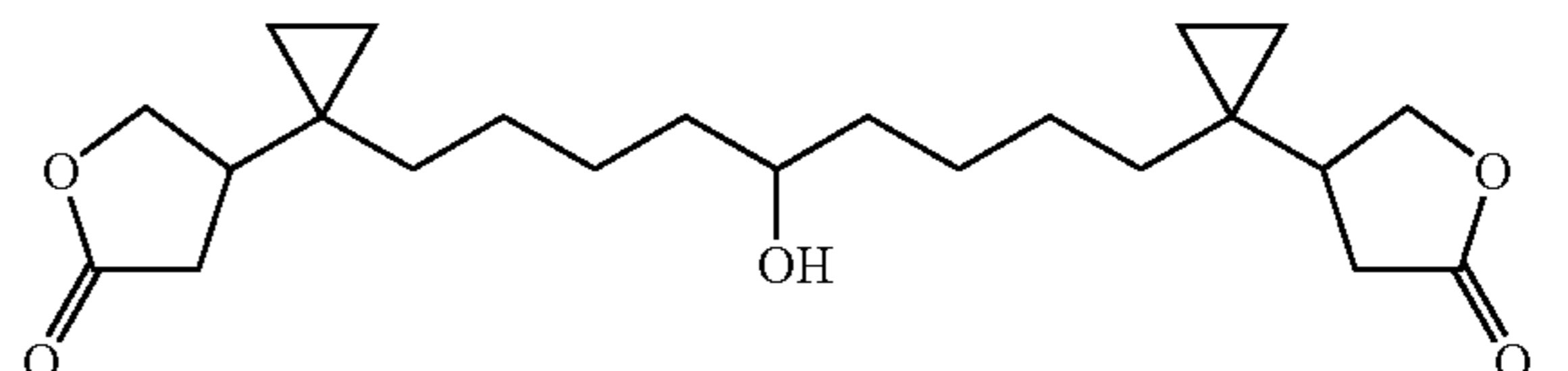
1,9-Bis-[1-(2-oxo-tetrahydrofuran-4-yl)-cyclopropyl]-nonan-5-ol
