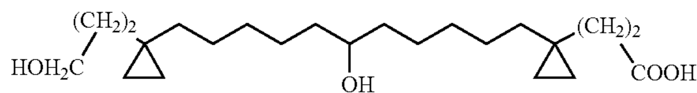
3-(1-(11-[1-(2-Carboxy-ethyl)-cyclopropyl]-6-hydroxy-undecyl)-cyclopropyl)-propionic acid
