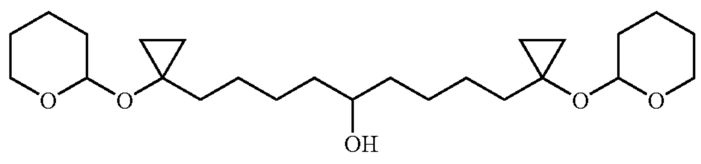
1,9-Bis-[1-(tetrahydro-pyran-2-yloxy)-cyclopropyl]-nonan-5-ol
