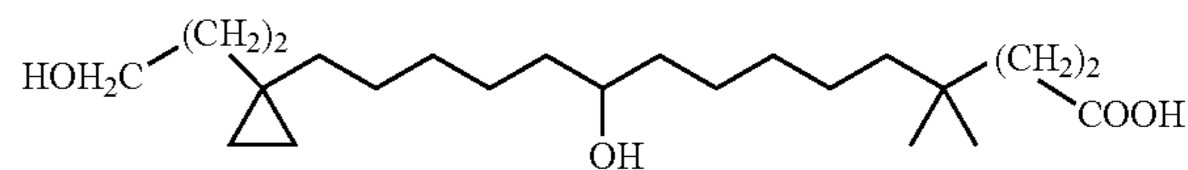
4,4-Dimethyl-10-hydroxy-15-[1-(3-hydroxy-propyl)-cyclopropyl]-pentadecanoic acid
