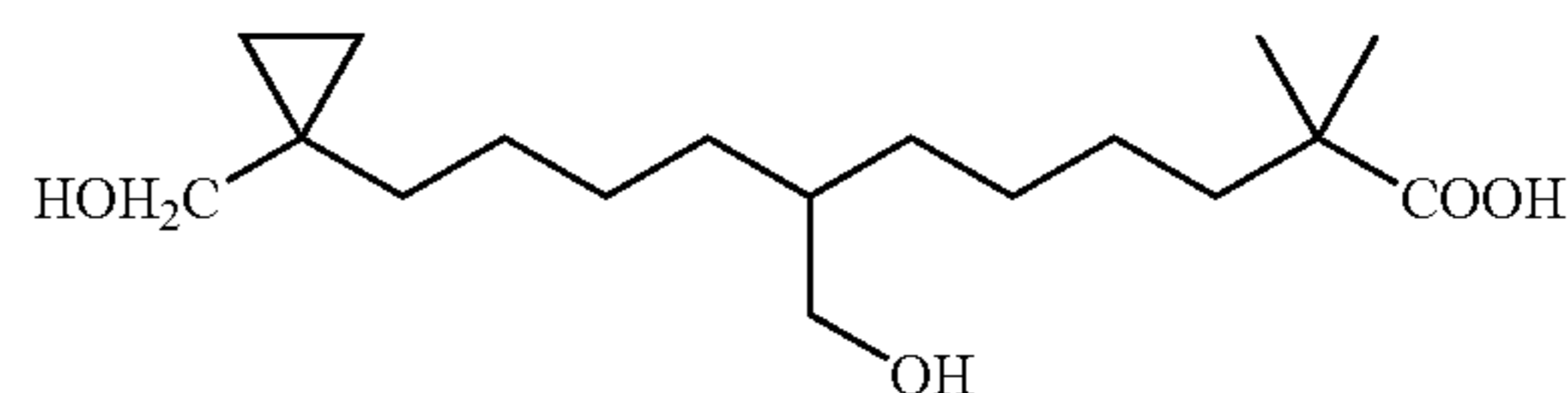
7-Hydroxymethyl-11-(1-hydroxymethyl-cyclopropyl)-2,2-dimethyl-undecanoic acid
