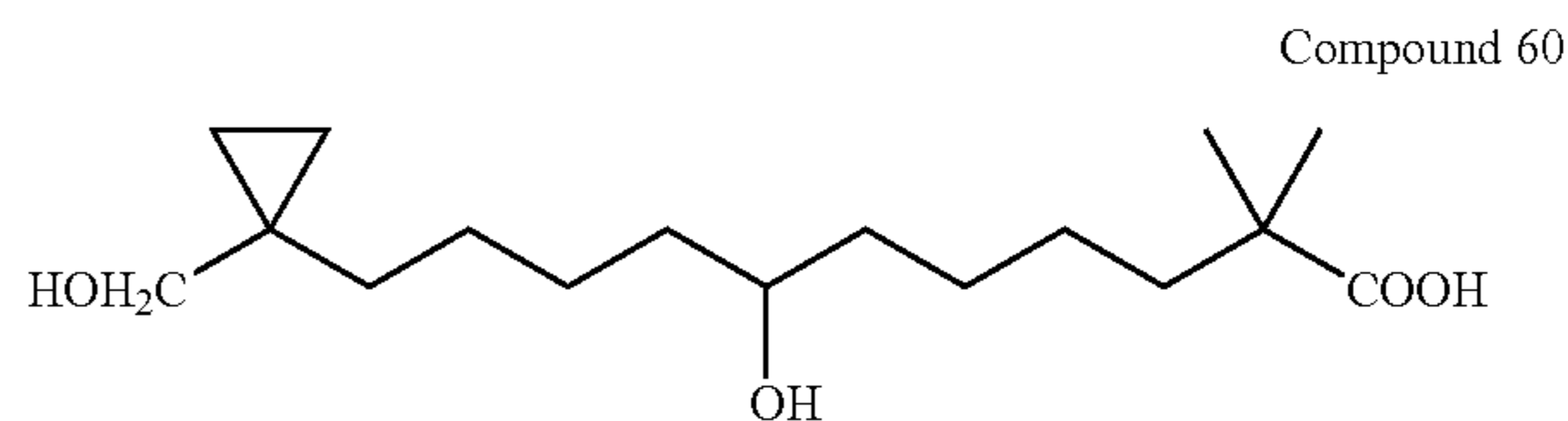
7-Hydroxy-11-(1-hydroxymethyl-cyclopropyl)-2,2-dimethyl-undecanoic acid
