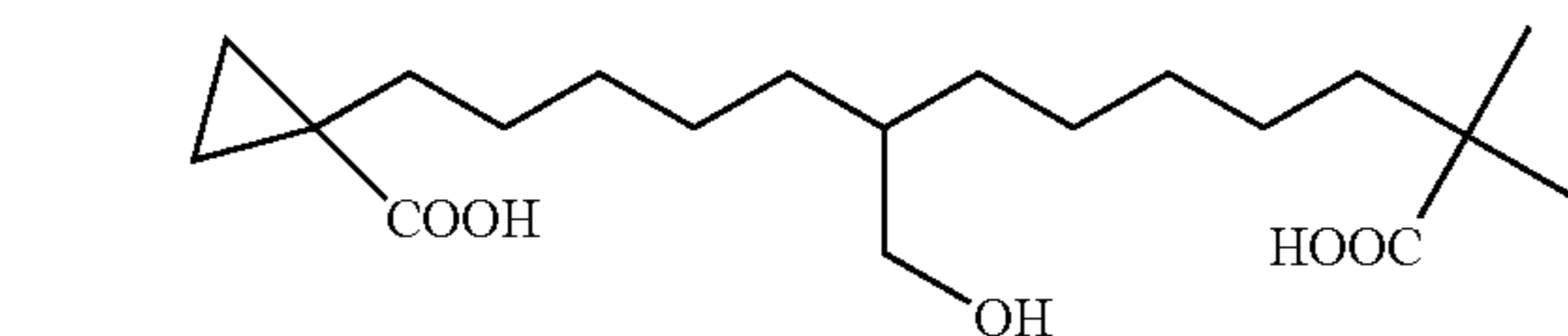
1-(12-Carboxy-6-hydroxymethyl-12-methyl-tridecyl)-cyclopropanecarboxylic acid
