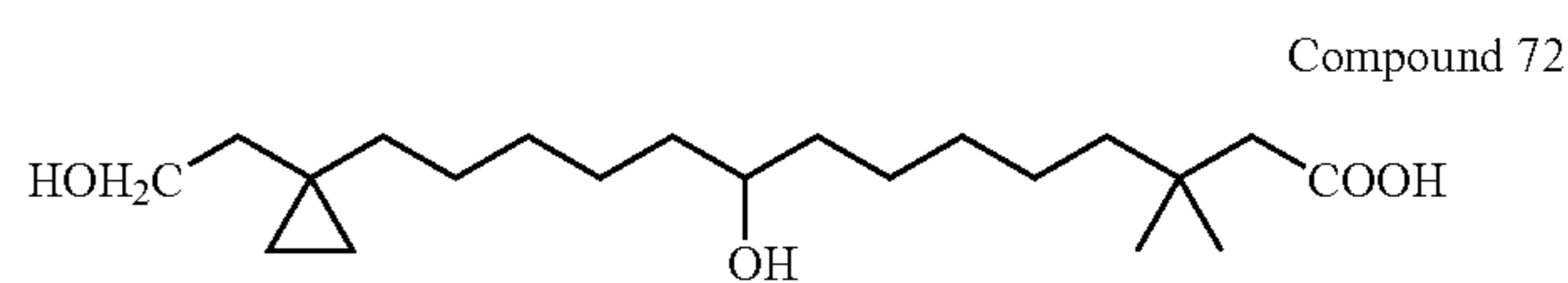
9-Hydroxy-14-[1-(2-hydroxy-ethyl)-cyclopropyl]-3,3-dimethyl-tetradecanoic acid
