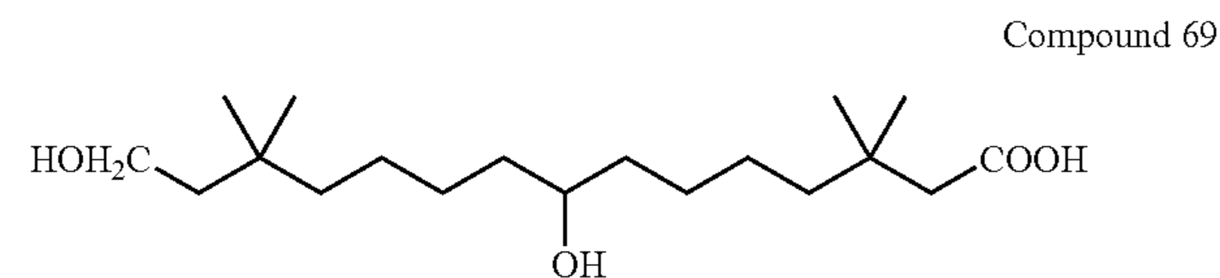
[1-(5,12-Dihydroxy-10,10-dimethyl-dodecyl)-cyclopropyl]-acetic acid
