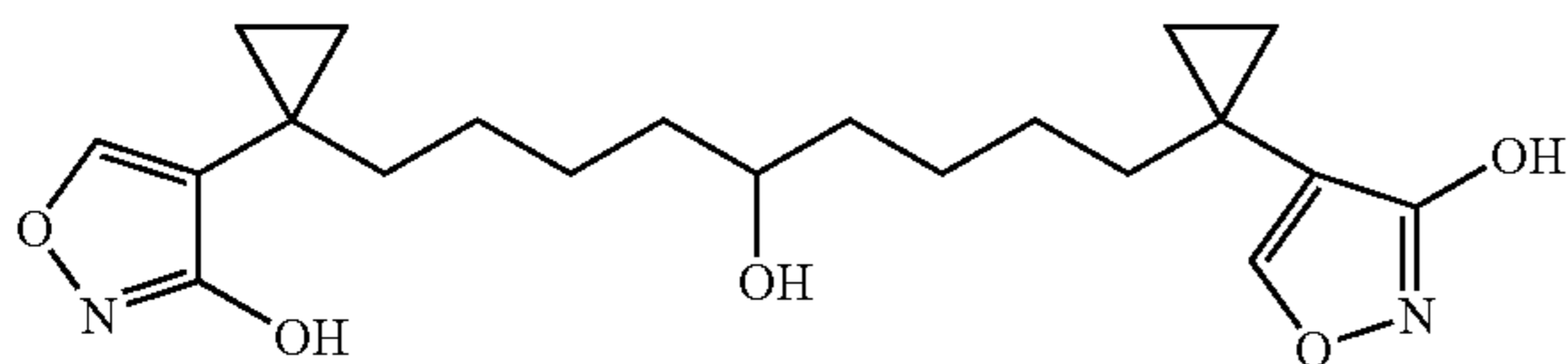
1,9-Bis-[1-(3-hydroxy-isoxazol-4-yl)-cyclopropyl]-nonan-5-ol
