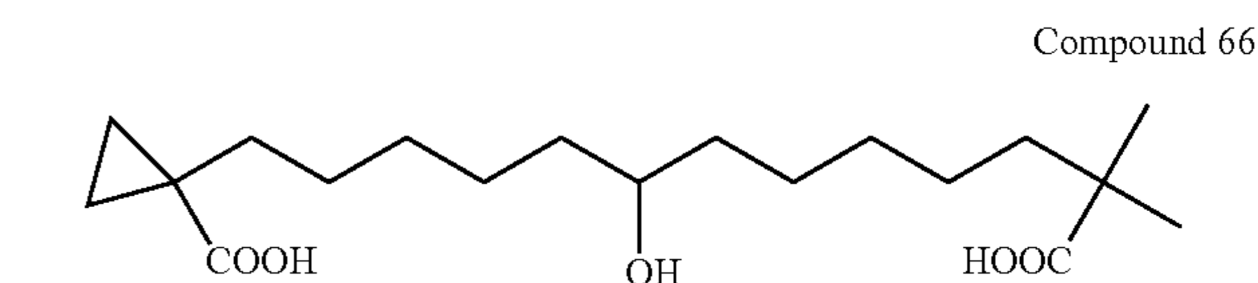
1-(12-Carboxy-6-hydroxy-12-methyl-tridecyl)-cyclopropanecarboxylic acid
