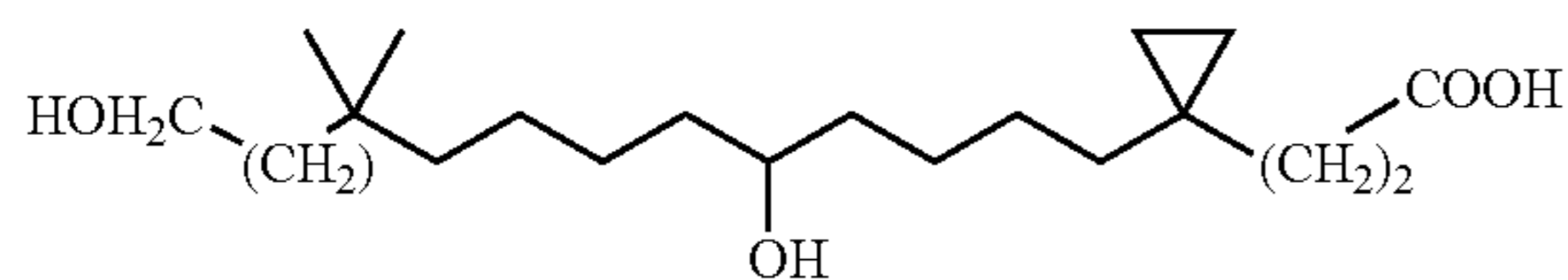
3-[1-(5,13-Dihydroxy-10,10-dimethyl-tridecyl)-cyclopropyl]-propionic acid
