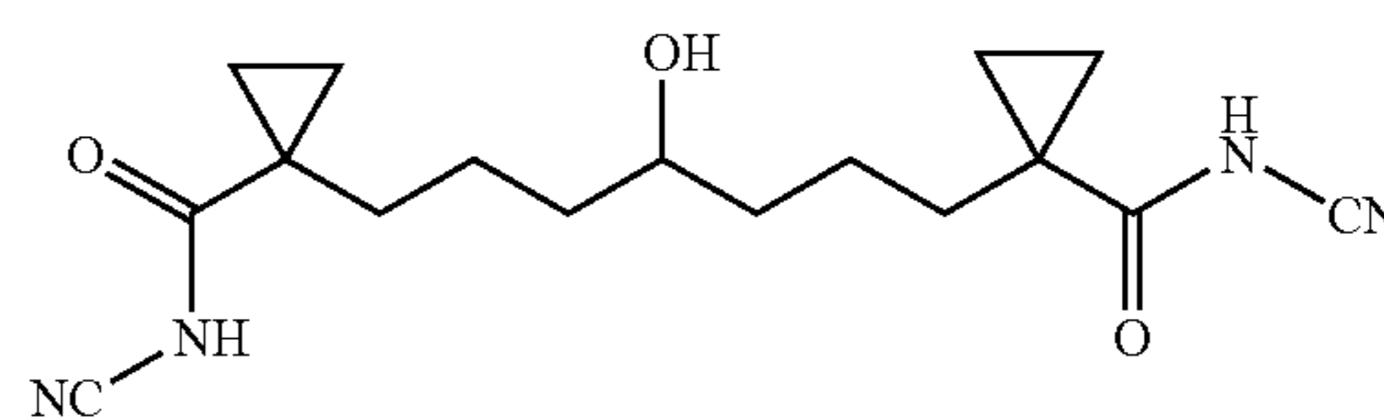
1,7-Bis-(1-dicyanimido-cyclopropyl)-4-hydroxy-heptane
