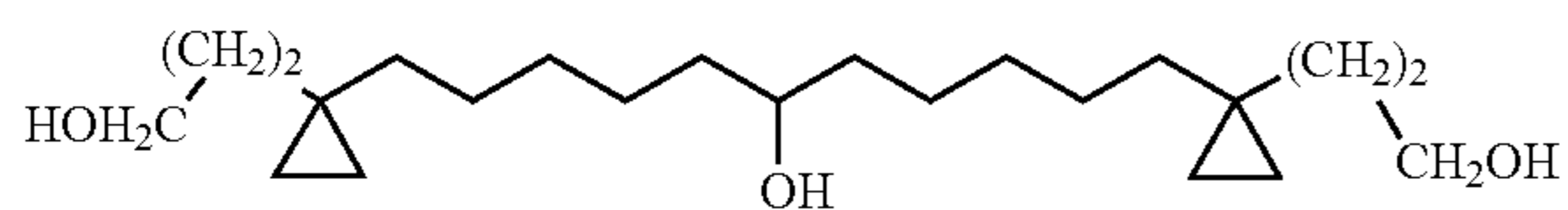
1,11-Bis-[1-(3-hydroxy-propyl)-cyclopropyl]-undecan-6-ol
