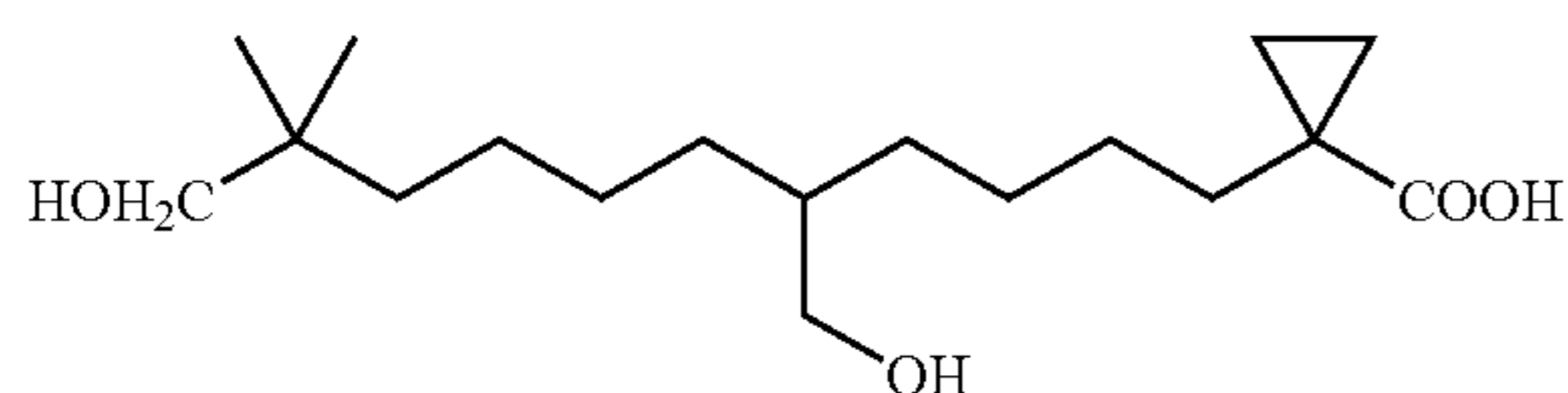
1-(11-Hydroxy-5-hydroxymethyl-10,10-dimethyl-undecyl)-cyclopropanecarboxylic acid
