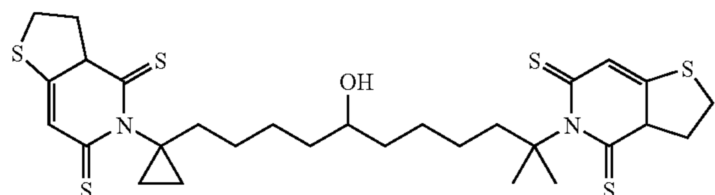
2,12-Bis-(4,6-dithioxo-2,3,3a,6-tetrahydro-4H-thieno[3,2-c]pyridin-5-yl)-2-methyl-12-(cyclopropyl)-7-hydroxy-dodecane
