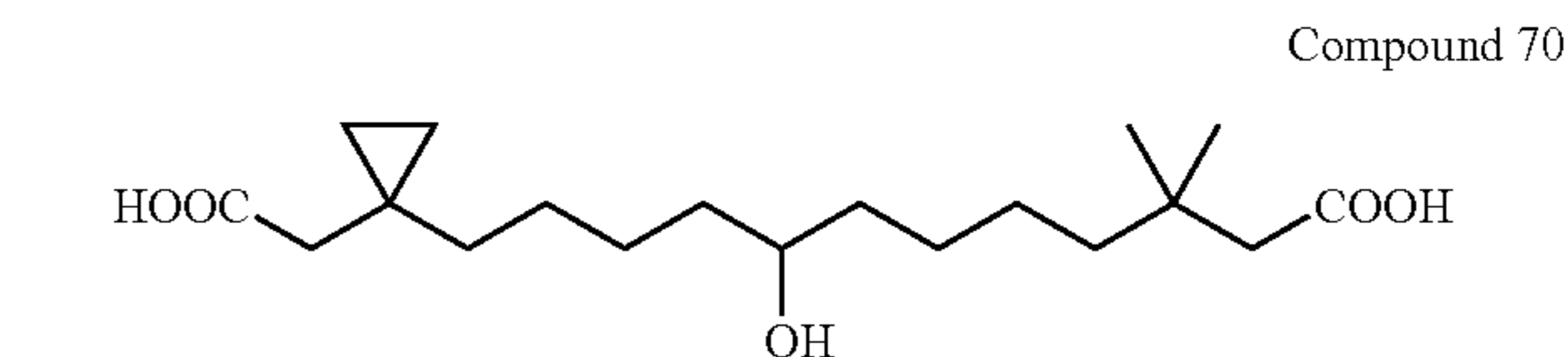
12-(1-Carboxymethyl-cyclopropyl)-8-hydroxy-3,3-dimethyl-dodecanoic acid
