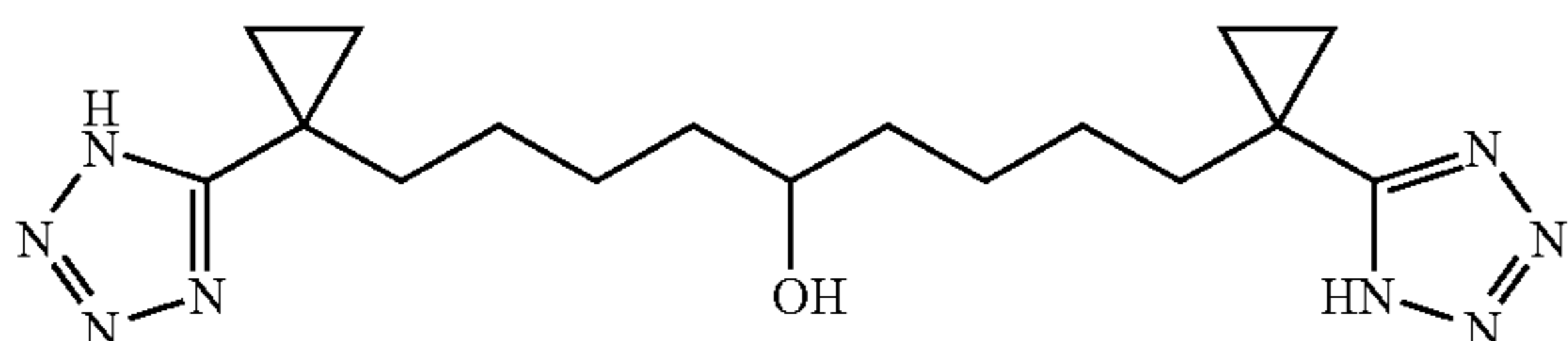
1,9-Bis-(1-(1H-tetrazol-5-yl)-cyclopropyl)-nonan-5-ol
