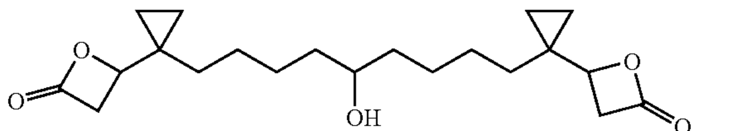
1,9-Bis-[1-(2-oxo-oxoethan-3-yl)-cyclopropyl]-nonan-5-ol
