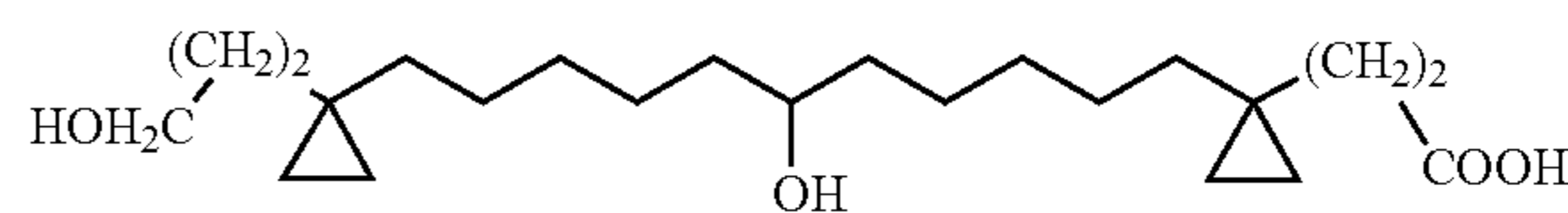
3-(1-(6-Hydroxy-11-[1-(3-hydroxy-propyl)-cyclopropyl]-undecyl)-cyclopropyl)-propionic acid
