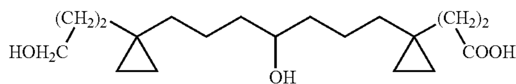
3-(1-(4-Hydroxy-7-[1-(3-hydroxy-propyl)-cyclopropyl]-heptyl)-cyclopropyl)-propionic acid
