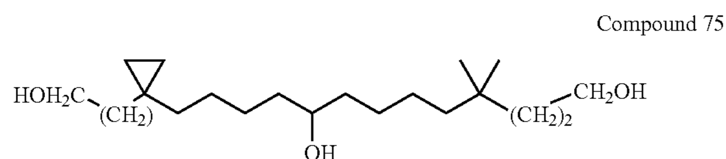
13-[1-(3-Hydroxy-propyl)-cyclopropyl]-4,4-dimethyl-tridecane-1,9-diol
