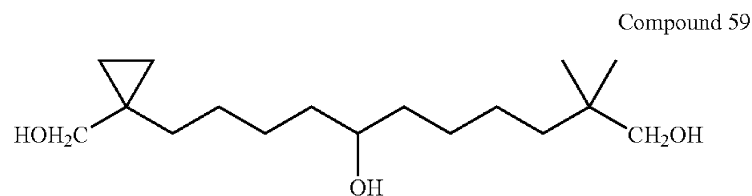
11-(1-Hydroxymethyl-cyclopropyl)-2,2-dimethyl-undecane-1,7-diol
