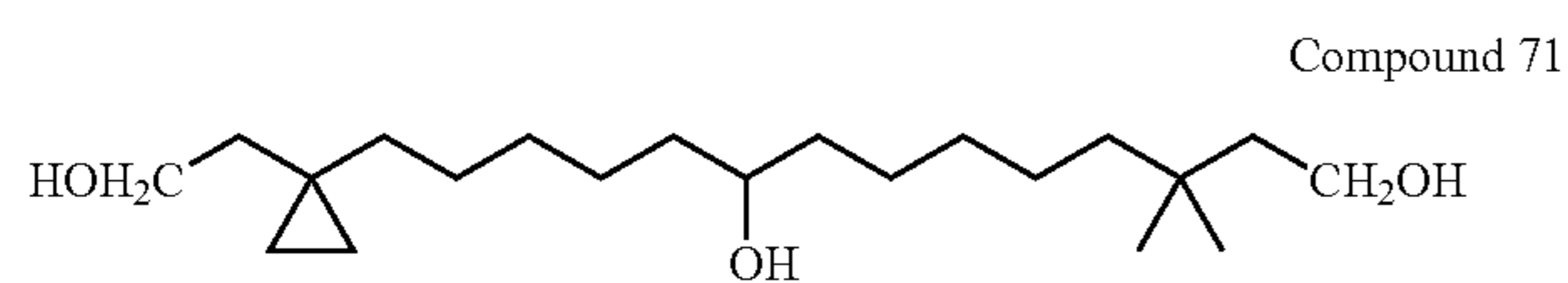
14-[1-(2-Hydroxy-ethyl)-cyclopropyl]-3,3-dimethyl-tetradecane-1,9-diol
