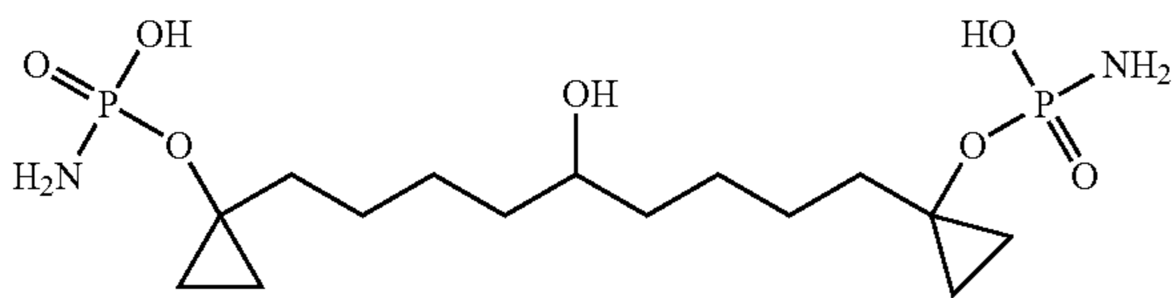
1,7-Bis-(1-phosphonamido-cyclopropyl)-5-hydroxy-nonane
