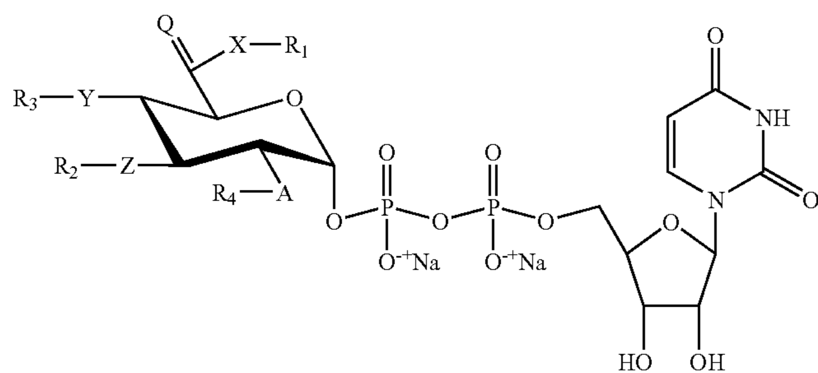
UDP-Glucosamine-derivatives (when A = NH, R 4 may be acetyl)
