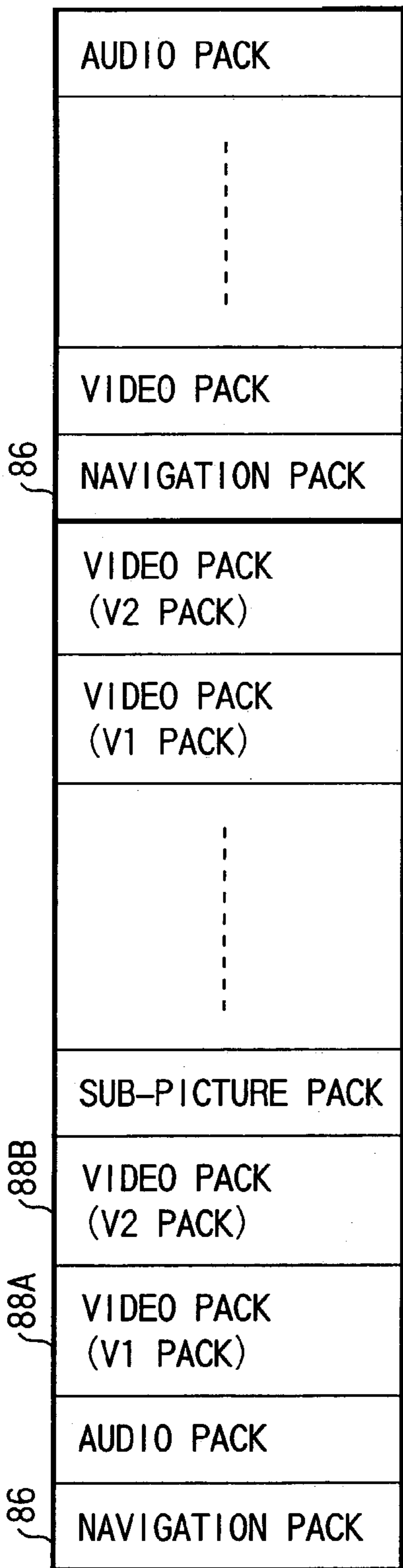
V1 PACK 88A = MAIN PICTURE PACK (MPEG2 VIDEO): STREAM ID = 0xe0 V2 PACK 88B = SEARCH PICTURE PACK (STREAM ID = 0xe1 FOR MPEG2 VIDEO), ETC.
