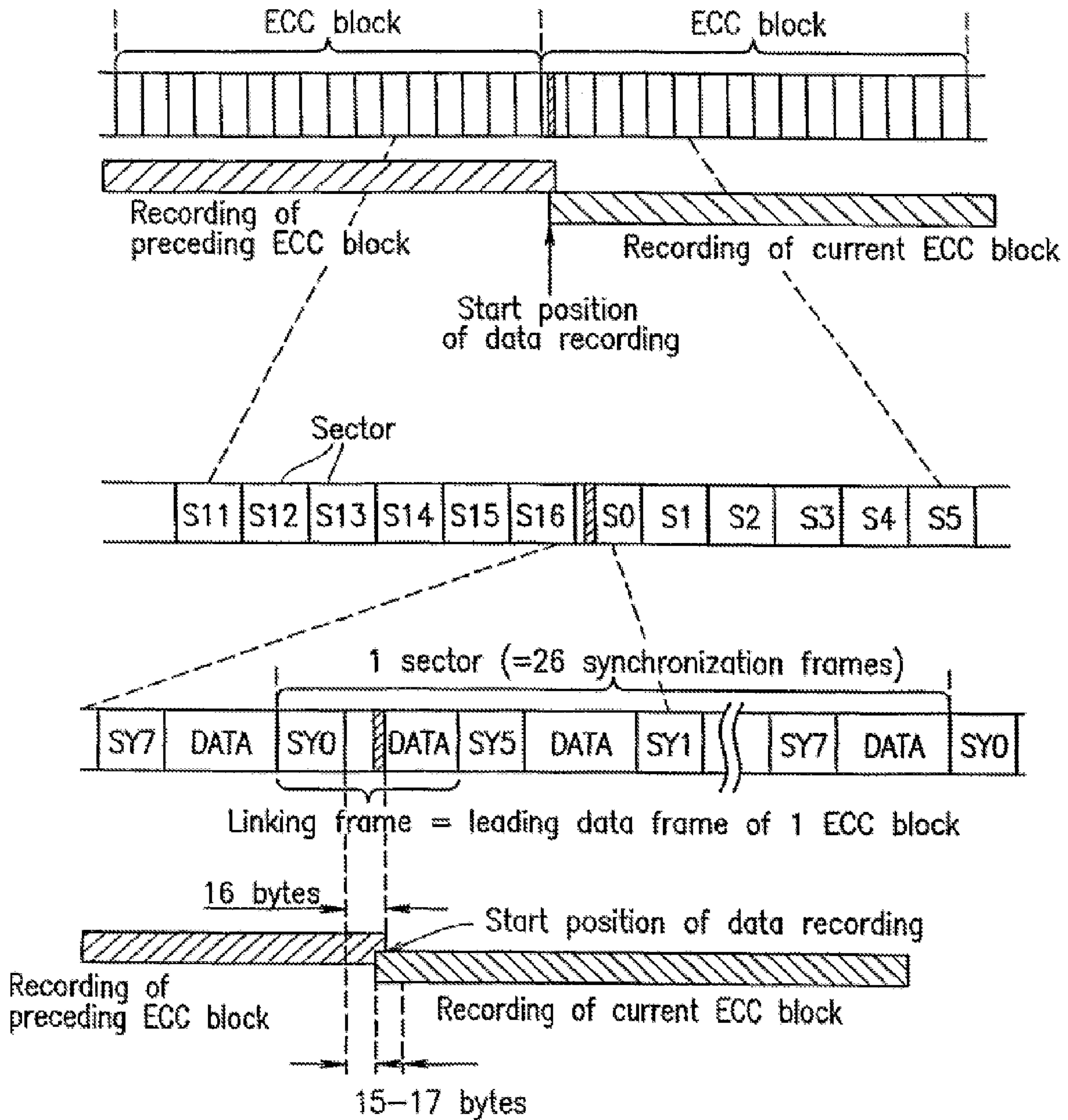
FIG. 44 CONVENTIONAL ART
