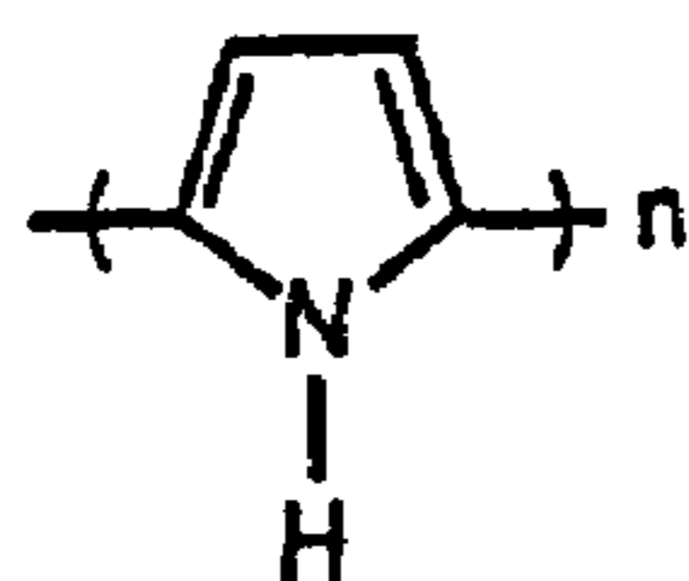
POLYPYRROLE
