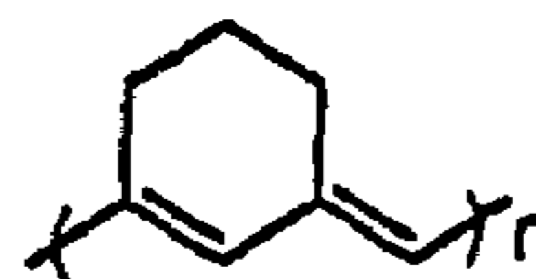
POLY(1,6-HEPTADIYNE)
