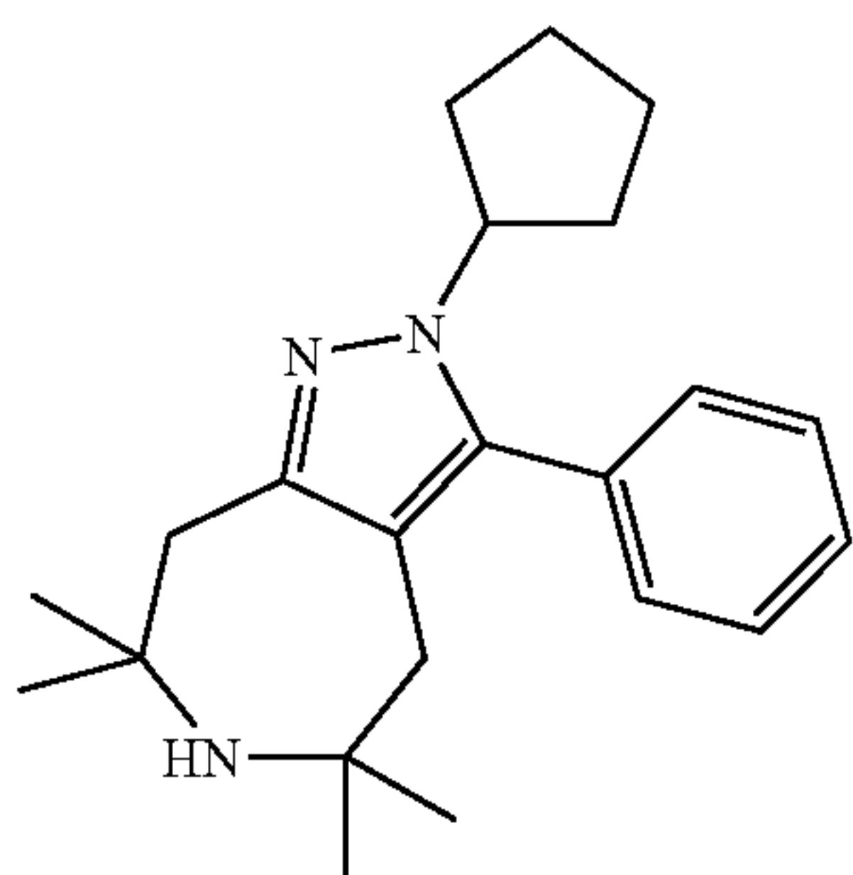
2-Cyclopentyl-5,5,7,7-tetramethyl-3-phenyl-2,4,5,6,7,8-hexahydro-1,2,6-triaza-azulene
