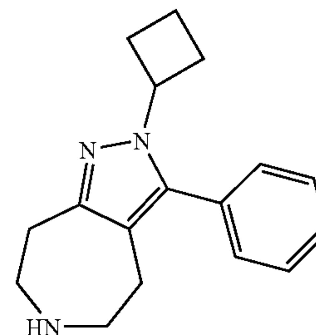
2-Cyclobutyl-3-phenyl-2,4,5,6,7,8-hexahydro-1,2,6-triaza-azulene
