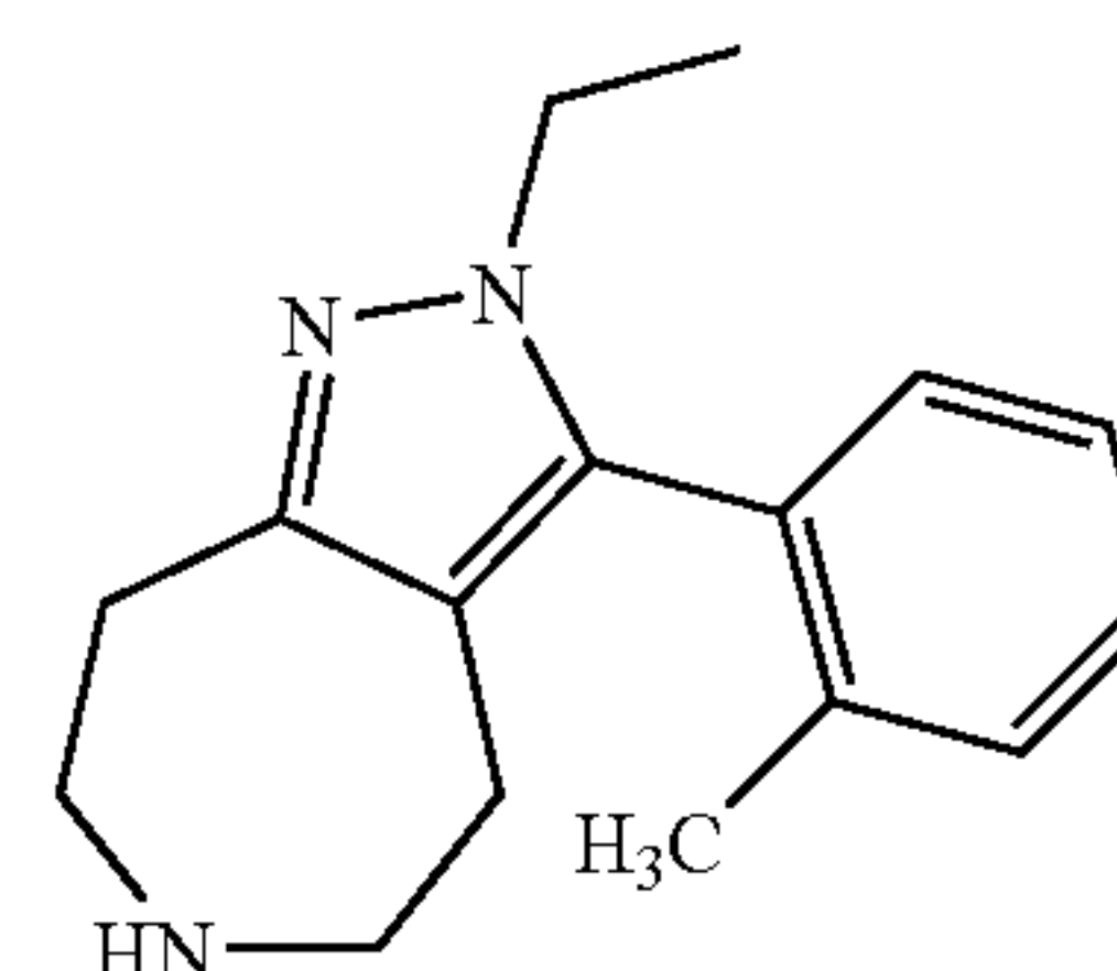
2-Ethyl-3-o-tolyl-2,4,5,6,7,8-hexahydro-1,2,6-triaza-azulene
