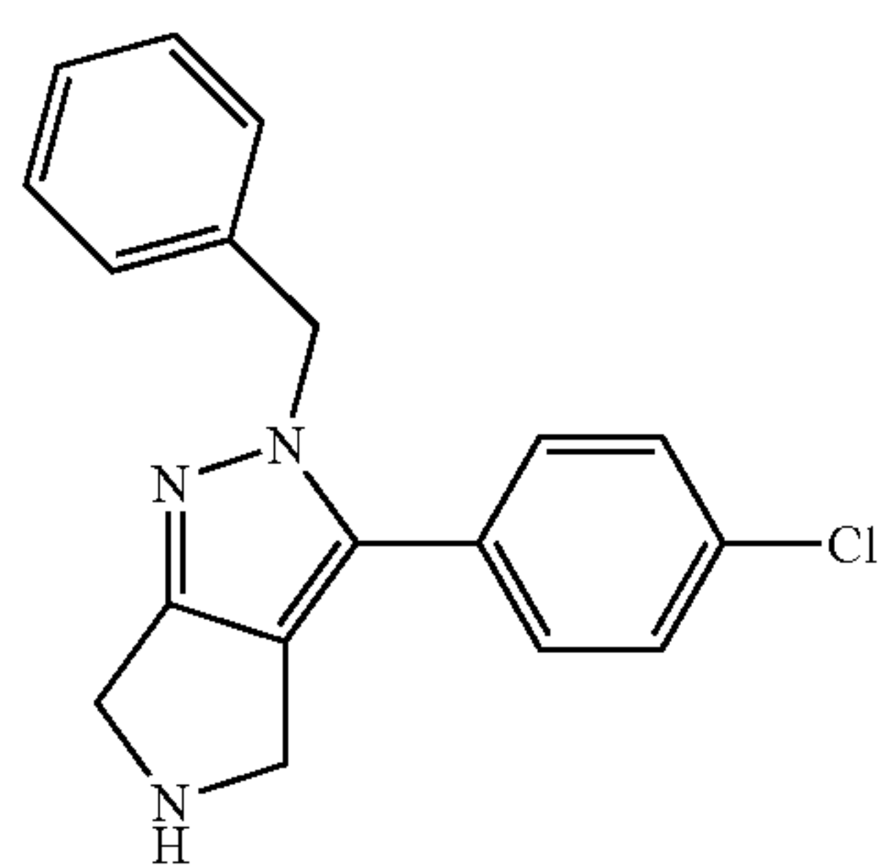
2-Benzyl-3-(4-chloro-phenyl)-2,4,5,6-tetrahydro-pyrrolo[3,4-c]pyrazole
