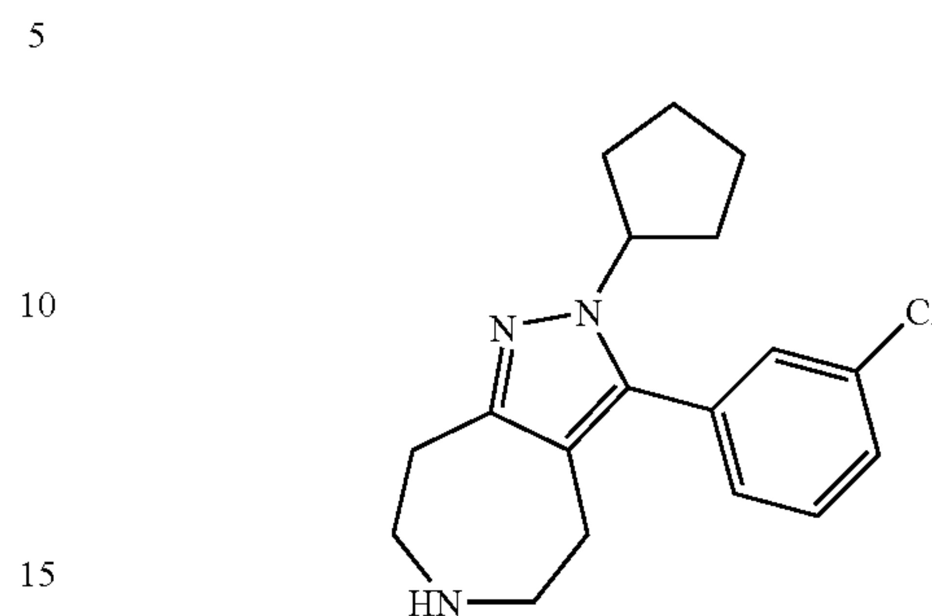
3-(3-Chloro-phenyl)-2-cyclopentyl-2,4,5,6,7,8-hexahydro-1,2,6-triaza-azulene
