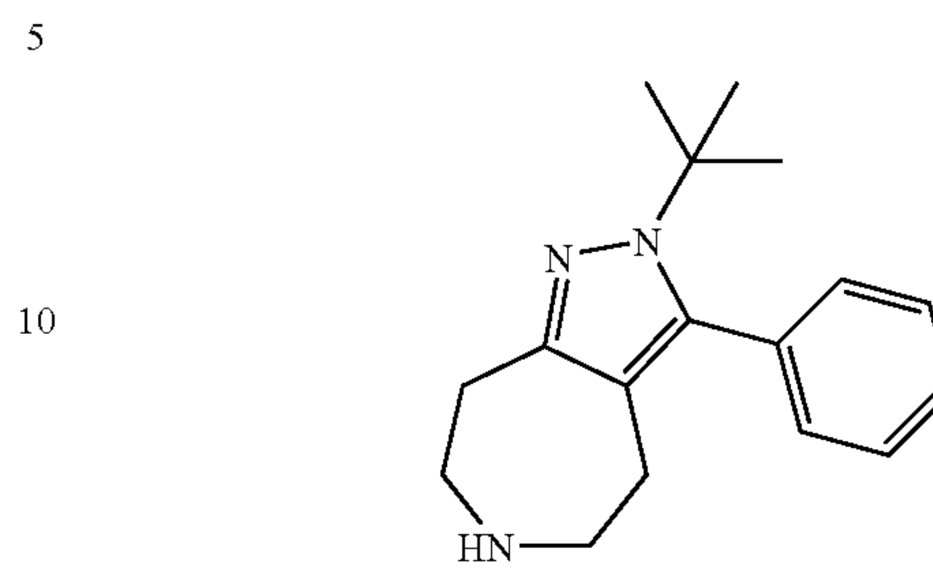
2-tert-Butyl-3-phenyl-2,4,5,6,7,8-hexahydro-1,2,6-triaza-azulene
