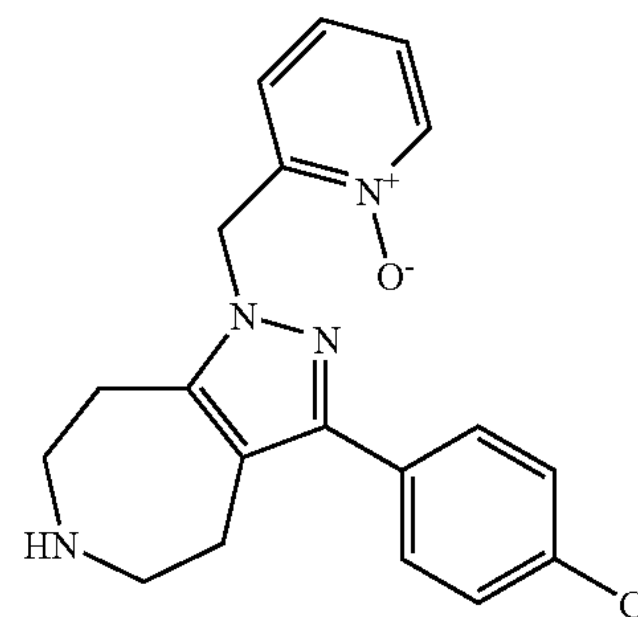
3-(4-Chloro-phenyl)-1-(1-oxy-pyridin-2-ylmethyl)-1,4,5,6,7,8-hexahydro-1,2,6-triaza-azulene
