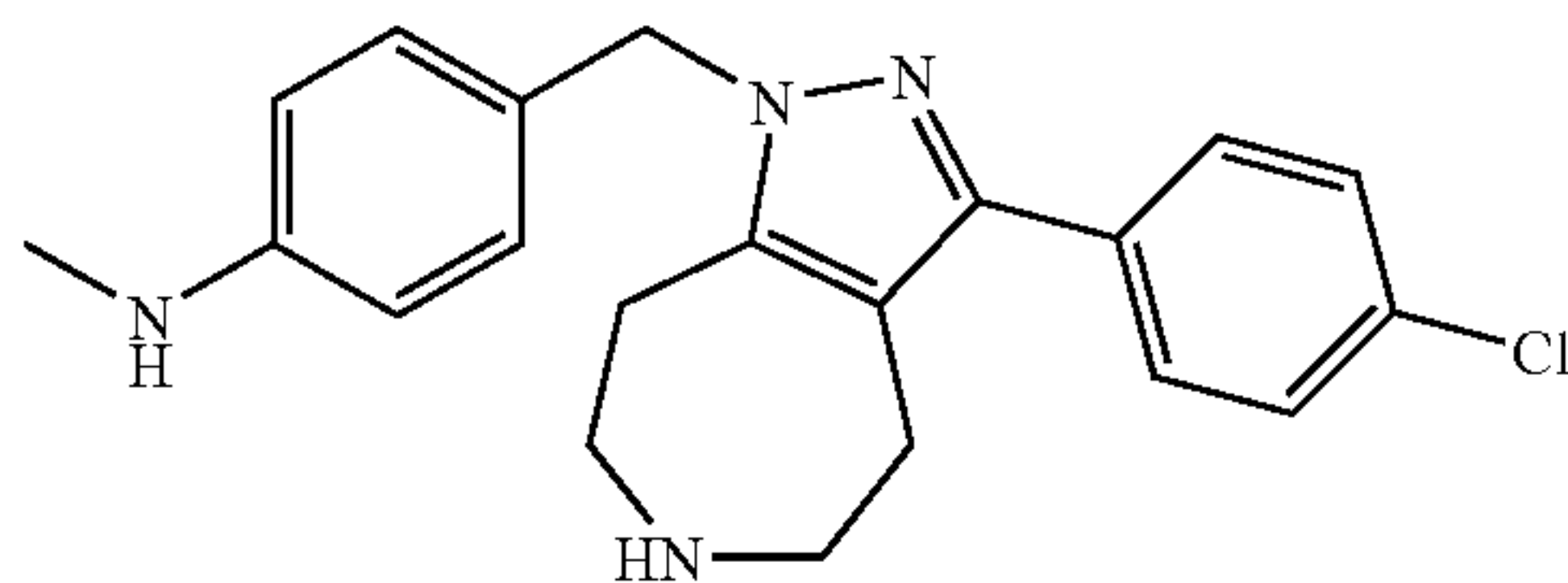
{4-[3-(4-Chloro-phenyl)-5,6,7,8-tetrahydro-4H-1,2,6-triaza-azulen-1-ylmethyl]-phenyl}-methyl-amine
