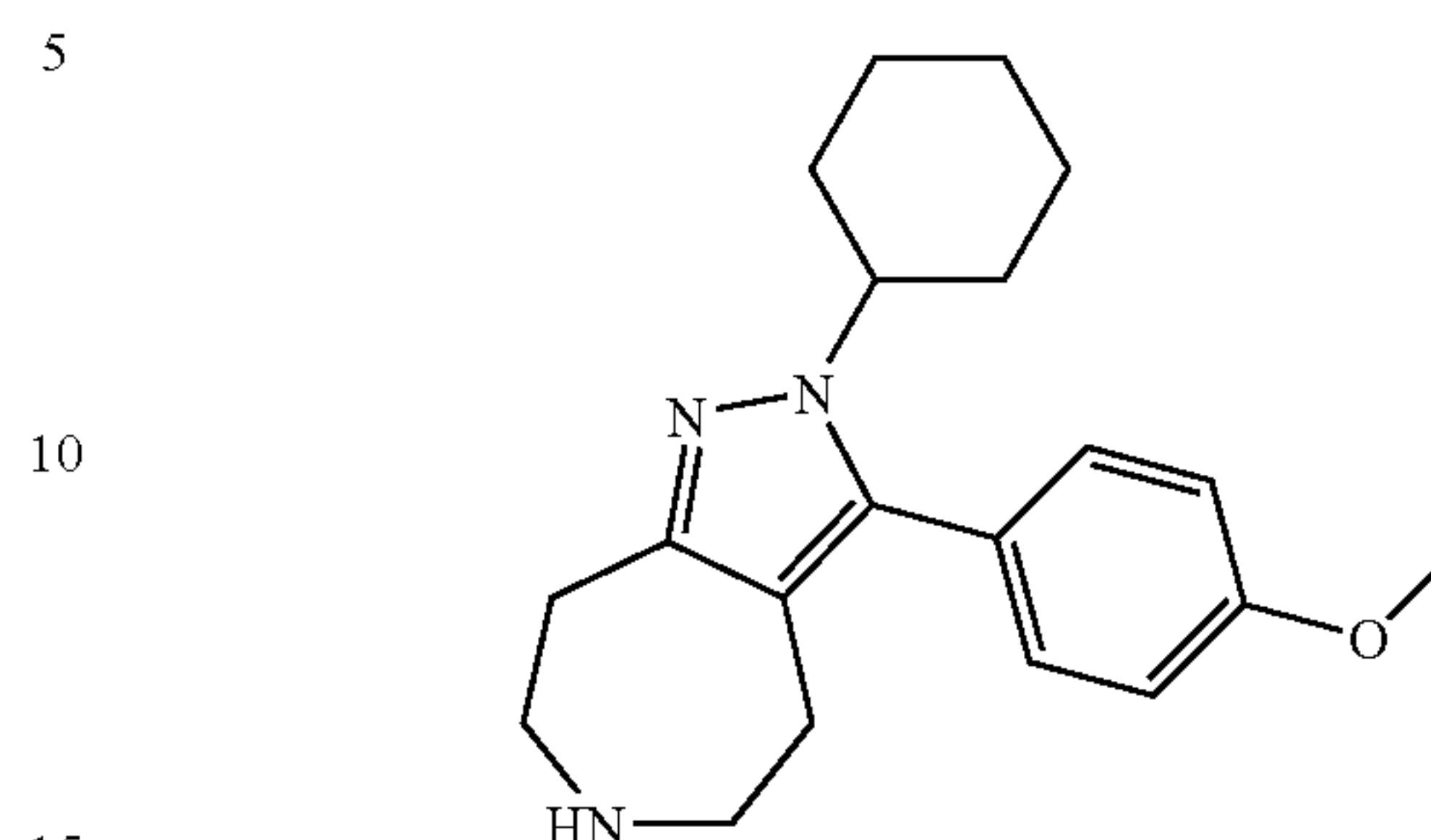
2-Cyclohexyl-3-(4-methoxy-phenyl)-2,4,5,6,7,8-hexahydro-1,2,6-triaza-azulene
