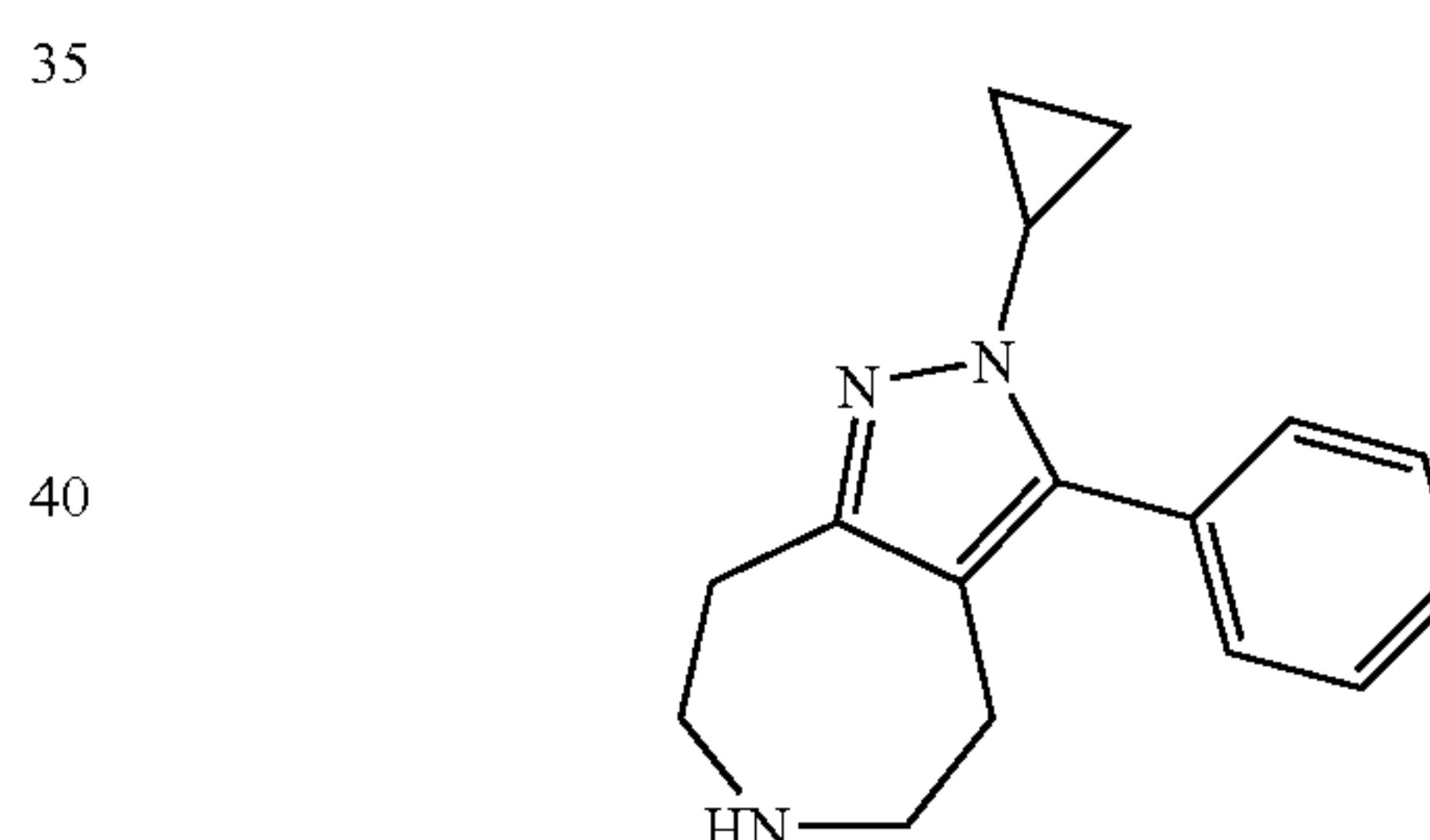
2-Cyclopropyl-3-phenyl-2,4,5,6,7,8-hexahydro-1,2,6-triaza-azulene
