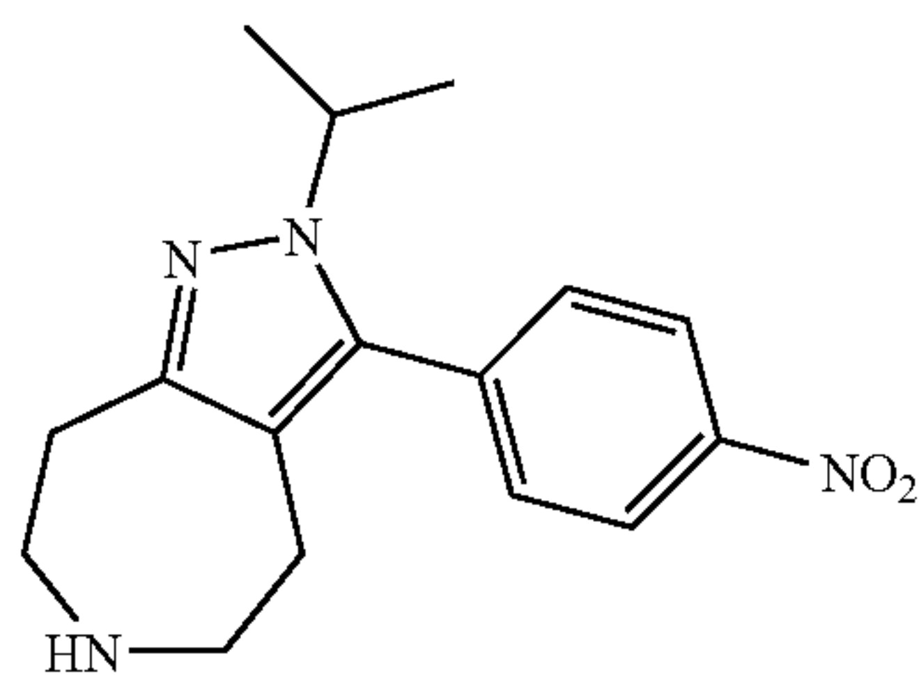
2-Isopropyl-3-(4-nitro-phenyl)-2,4,5,6,7,8-hexahydro-1,2,6-triaza-azulene
