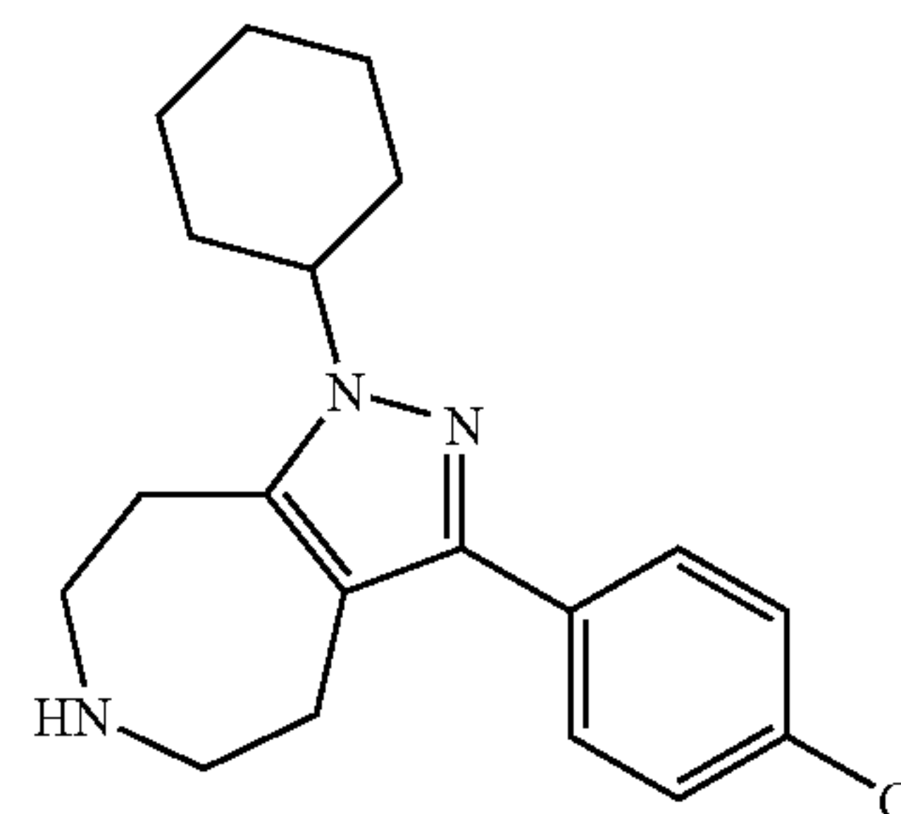
3-(4-Chloro-phenyl)-1-cyclohexyl-1,4,5,6,7,8-hexahydro-1,2,6-triaza-azulene
