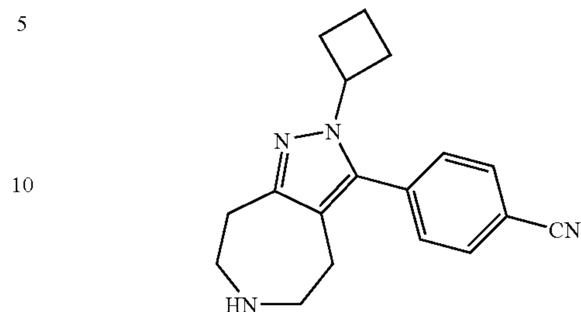
4-(2-Cyclobutyl-2,4,5,6,7,8-hexahydro-1,2,6-triaza-azulen-3-yl)-benzonitrile
