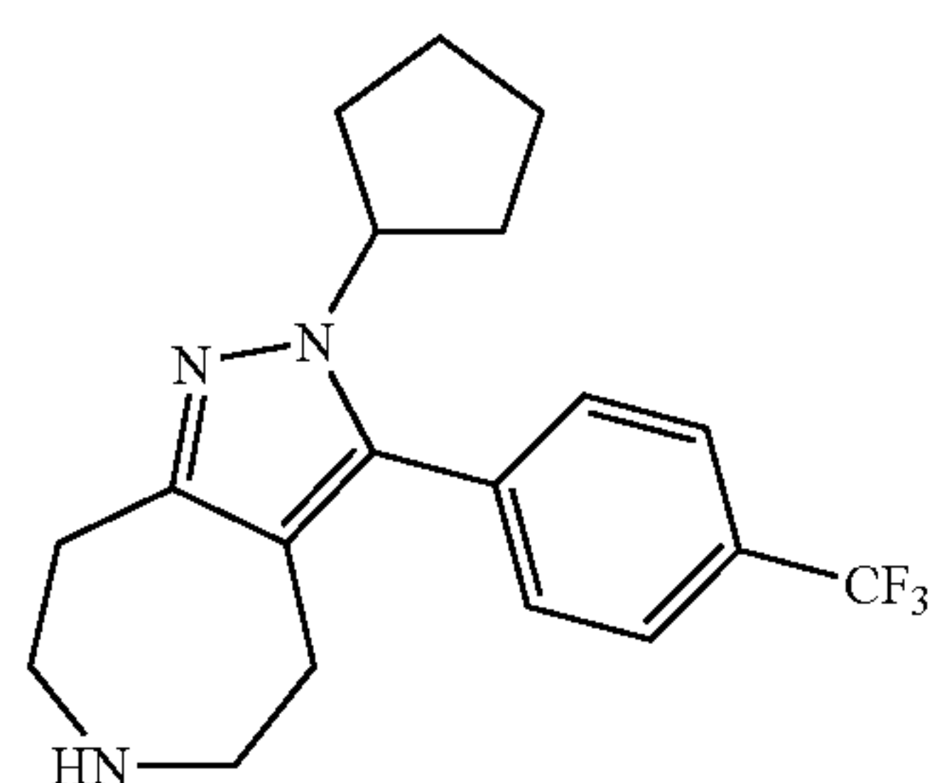
2-Cyclopentyl-3-(4-trifluoromethyl-phenyl)-2,4,5,6,7,8-hexahydro-1,2,6-triaza-azulene
