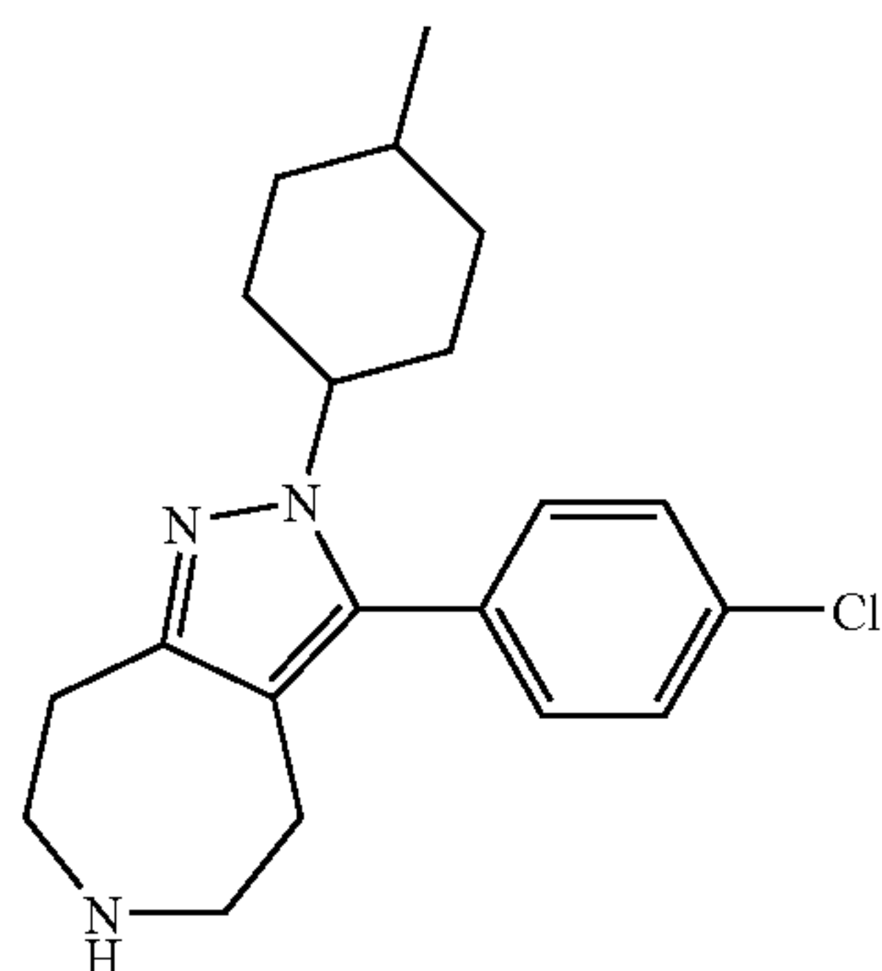
3-(4-Chloro-phenyl)-2-(4-methyl-cyclohexyl)-2,4,5,6,7,8-hexahydro-1,2,6-triaza-azulene
