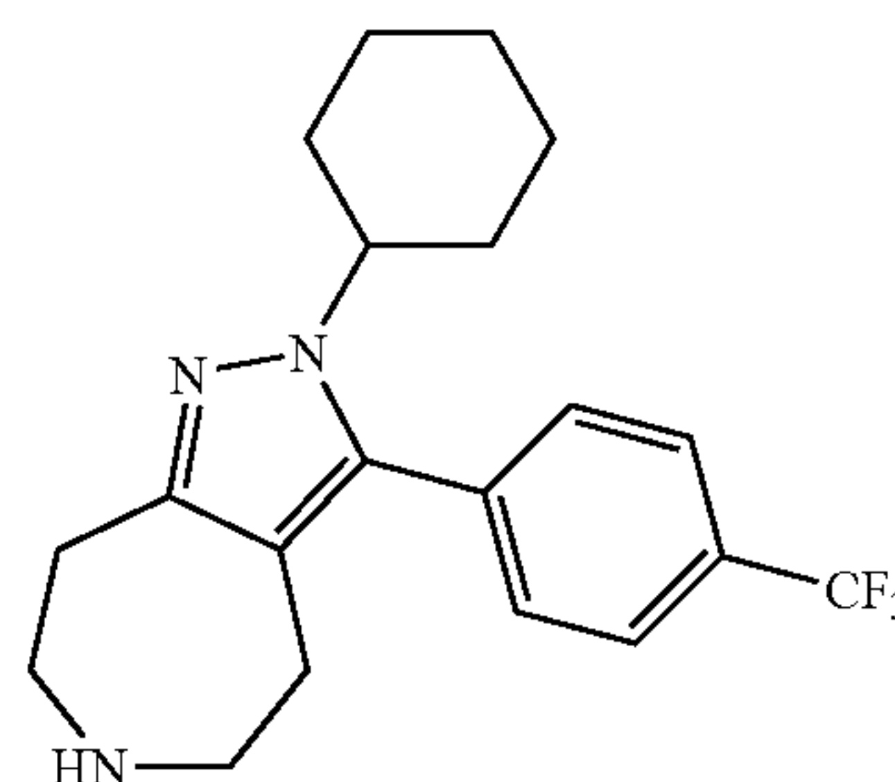
2-Cyclohexyl-3-(4-trifluoromethyl-phenyl)-2,4,5,6,7,8-hexahydro-1,2,6-triaza-azulene
