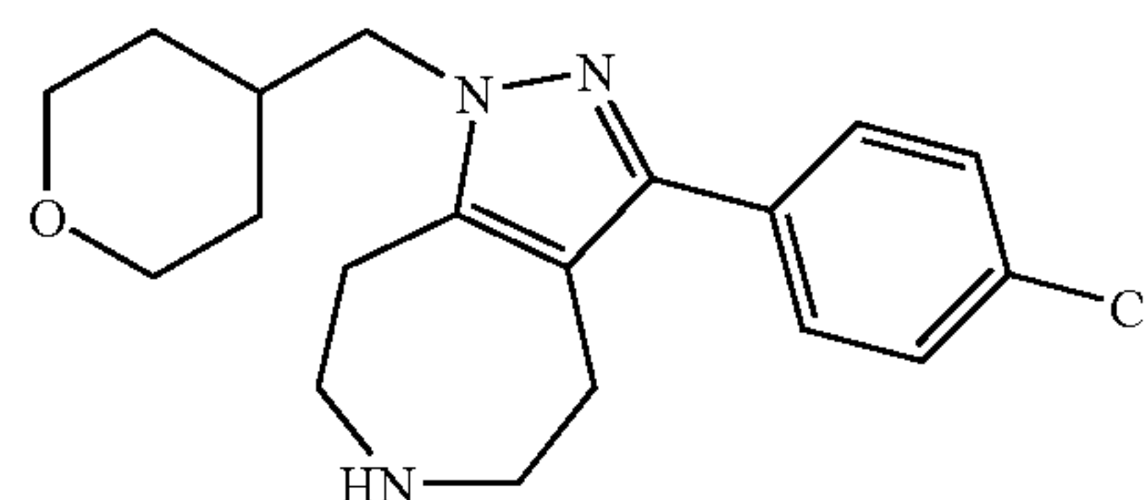
3-(4-Chloro-phenyl)-1-(tetrahydro-pyran-4-ylmethyl)-1,4,5,6,7,8-hexahydro-1,2,6-triaza-azulene
