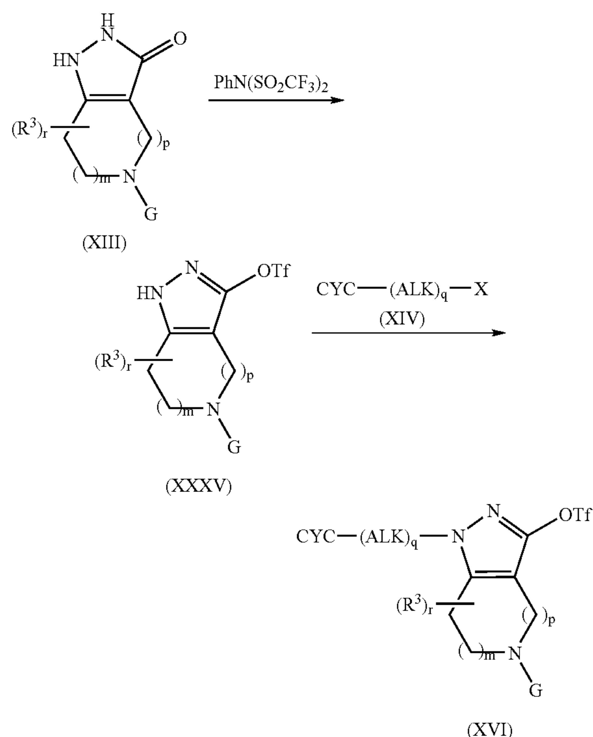
Scheme 6
