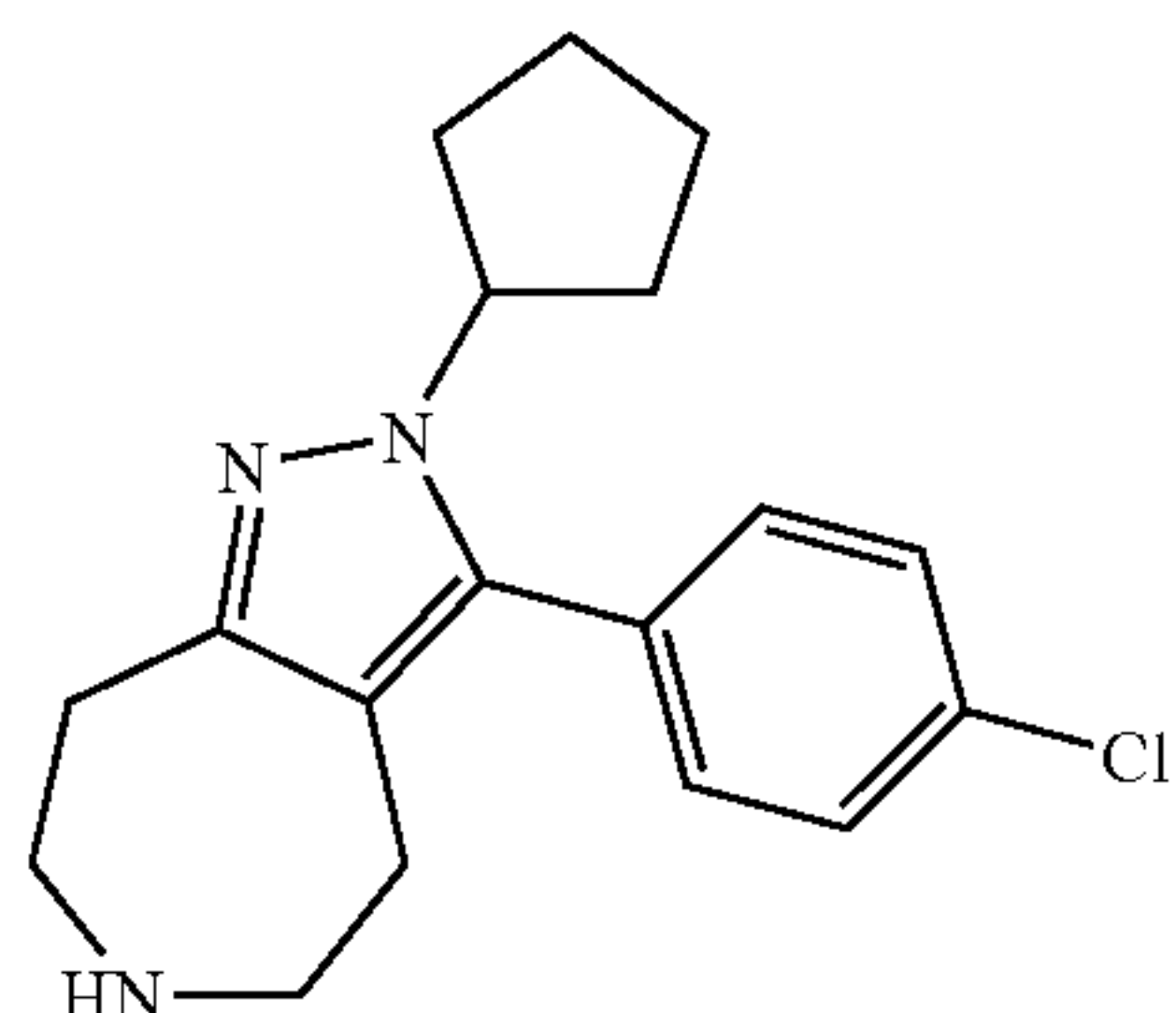
3-(4-Chloro-phenyl)-2-cyclopentyl-2,4,5,6,7,8-hexahydro-1,2,6-triaza-azulene
