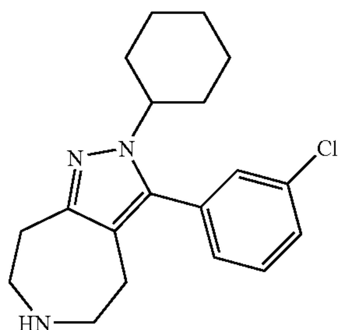
3-(3-Chloro-phenyl)-2-cyclohexyl-2,4,5,6,7,8-hexahydro-1,2,6-triaza-azulene
