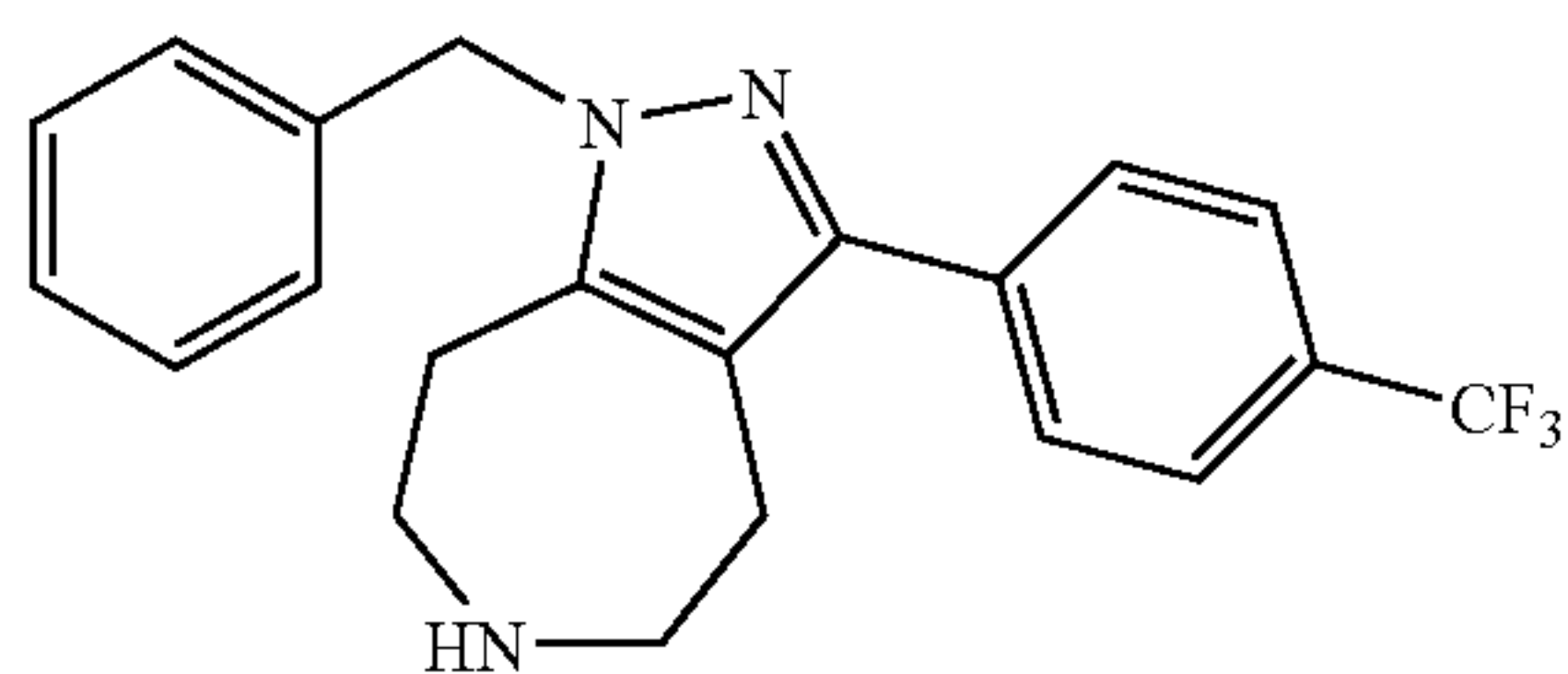
1-Benzyl-3-(4-trifluoromethyl-phenyl)-1,4,5,6,7,8-hexahydro-1,2,6-triaza-azulene
