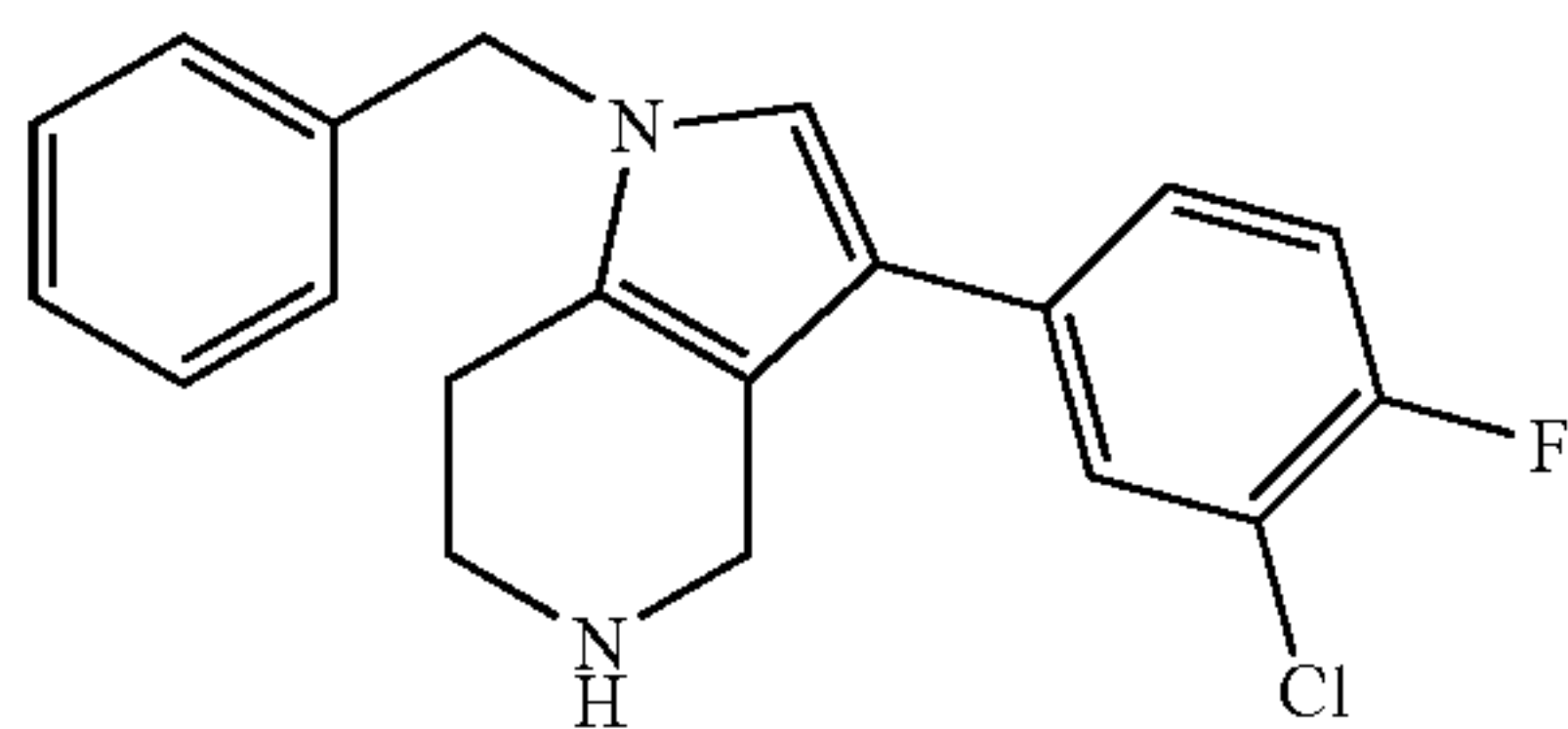
1-Benzyl-3-(3-chloro-4-fluoro-phenyl)-4,5,6,7-tetrahydro-1H-pyrrolo[3,2-c]pyridine
