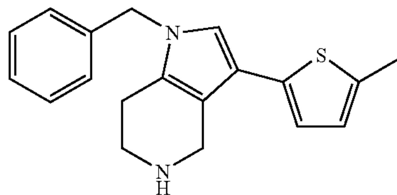
1-Benzyl-3-(5-methyl-thiophen-2-yl)-4,5,6,7-tetrahydro-1H-pyrrolo[3,2-c]pyridine
