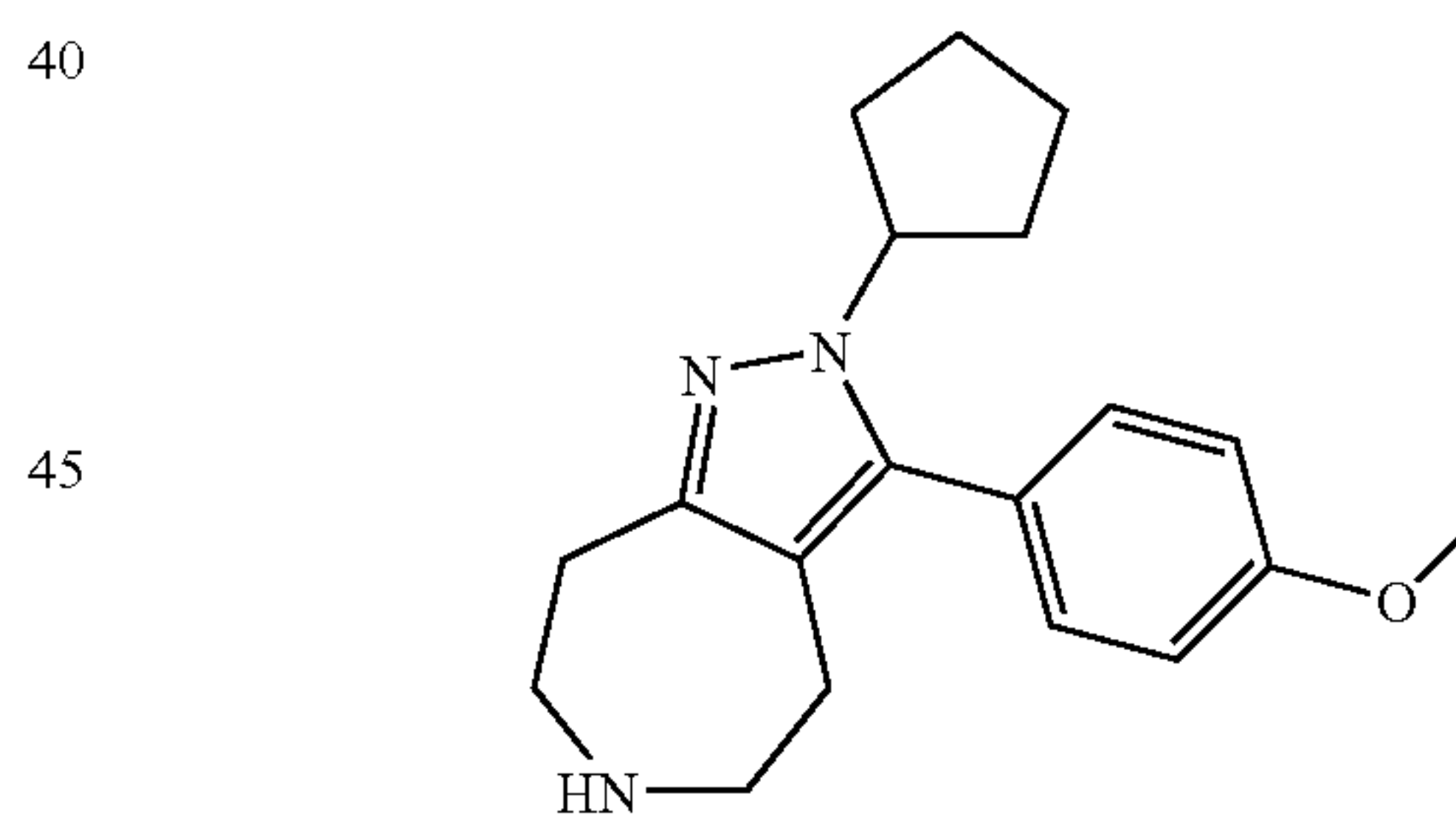
2-Cyclopentyl-3-(4-methoxy-phenyl)-2,4,5,6,7,8-hexahydro-1,2,6-triaza-azulene
