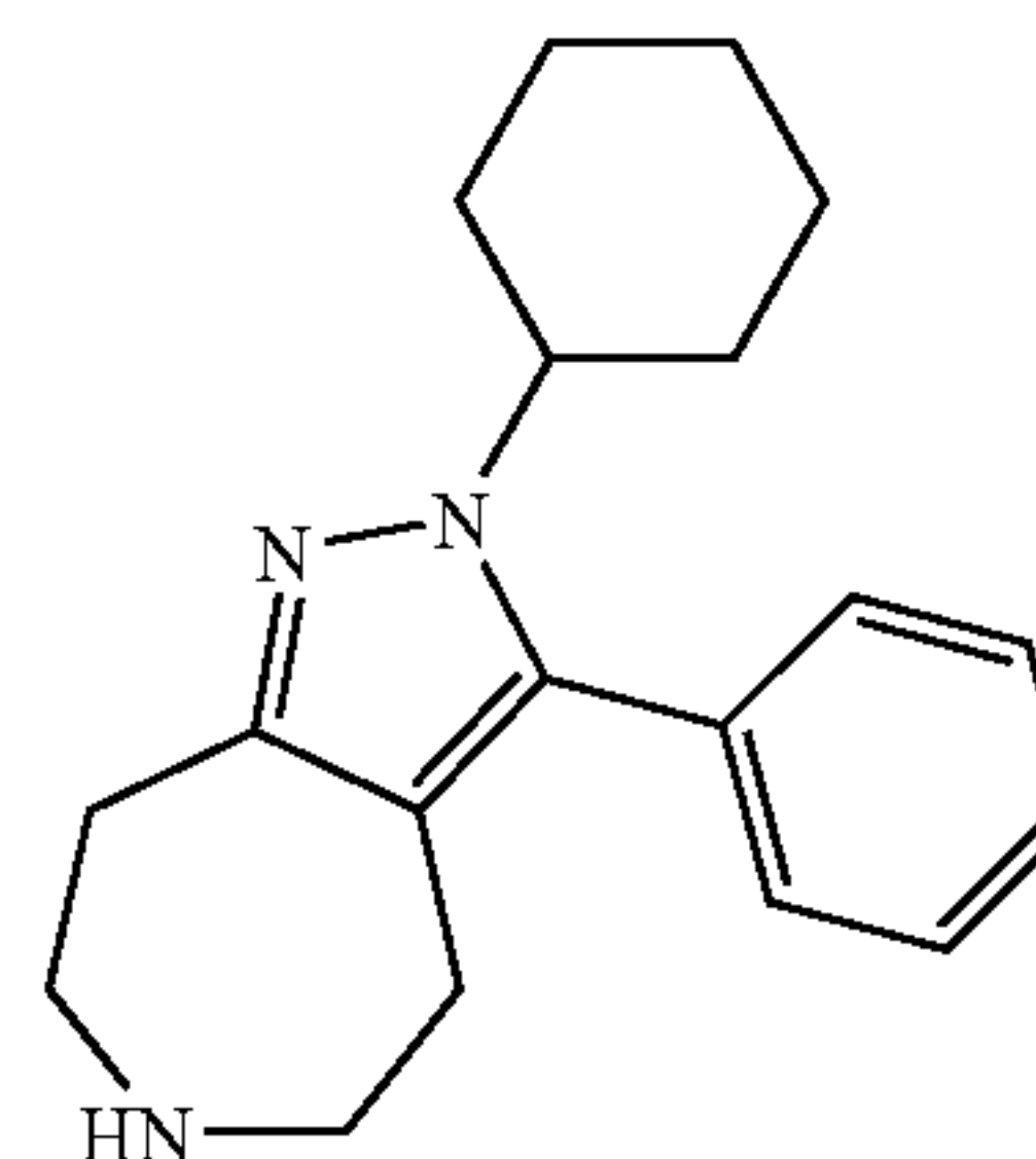
2-Cyclohexyl-3-phenyl-2,4,5,6,7,8-hexahydro-1,2,6-triaza-azulene
