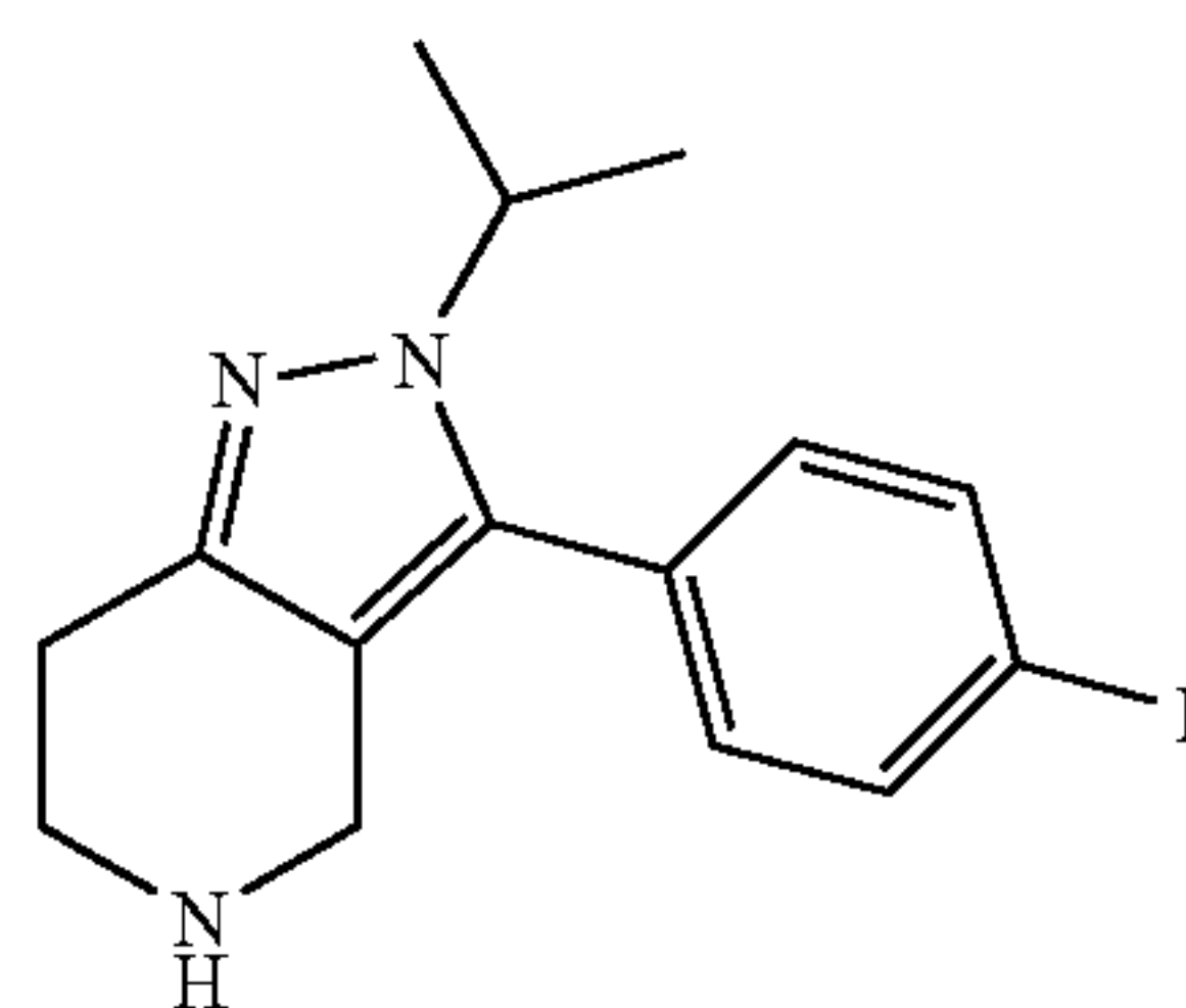
3-(4-Fluoro-phenyl)-2-isopropyl-4,5,6,7-tetrahydro-2H-pyrazolo[4,3-c]pyridine
