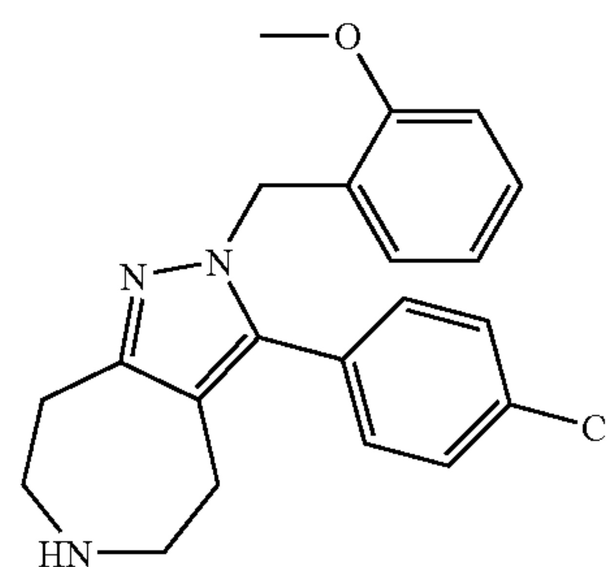
3-(4-Chloro-phenyl)-2-(2-methoxy-benzyl)-2,4,5,6,7,8-hexahydro-1,2,6-triaza-azulene
