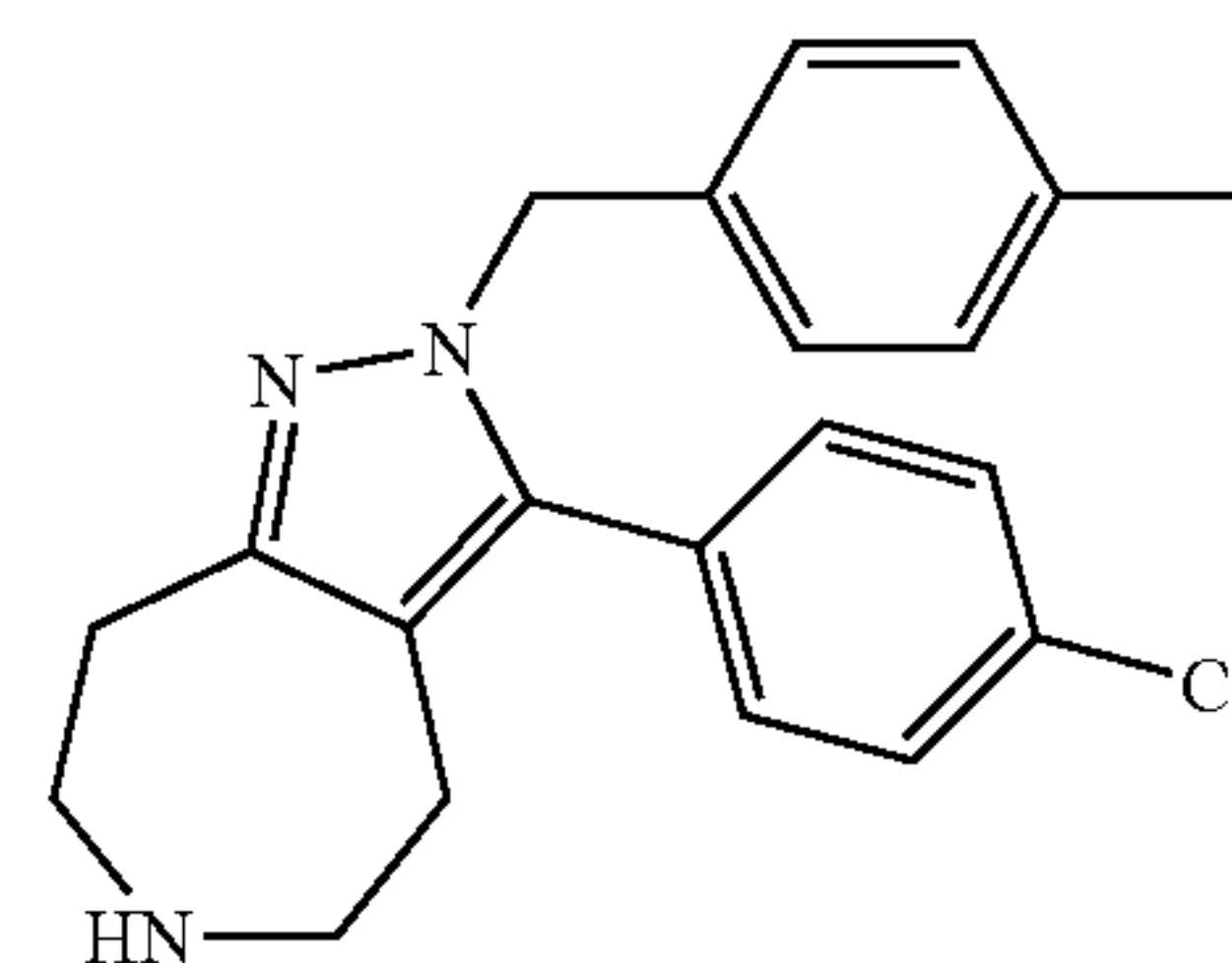
3-(4-Chloro-phenyl)-2-(4-methyl-benzyl)-2,4,5,6,7,8-hexahydro-1,2,6-triaza-azulene
