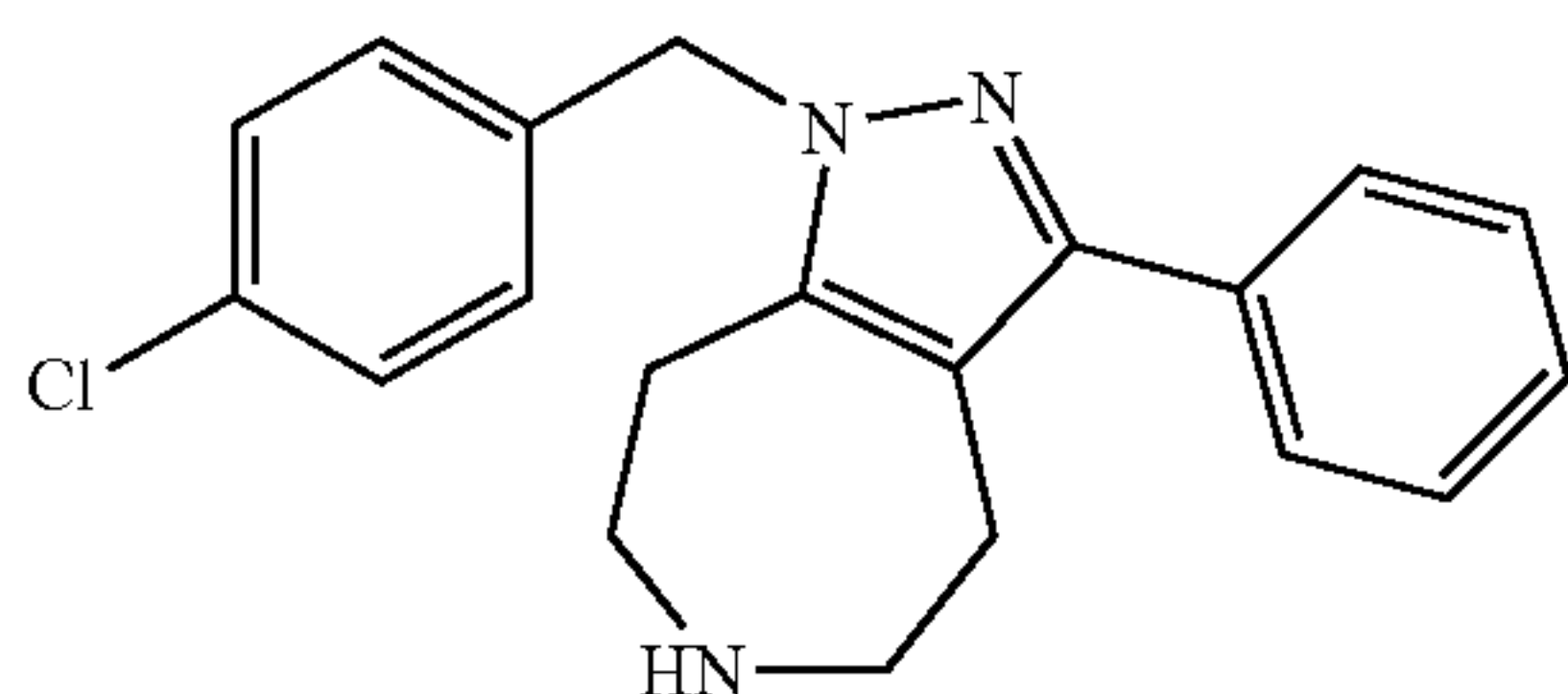
1-(4-Chloro-benzyl)-3-phenyl-1,4,5,6,7,8-hexahydro-1,2,6-triaza-azulene
