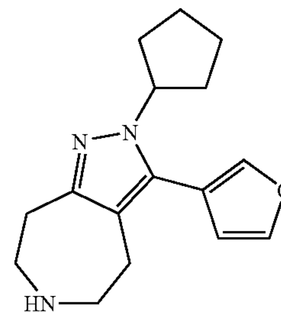
2-Cyclopentyl-3-furan-3-yl-2,4,5,6,7,8-hexahydro-1,2,6-triaza-azulene
