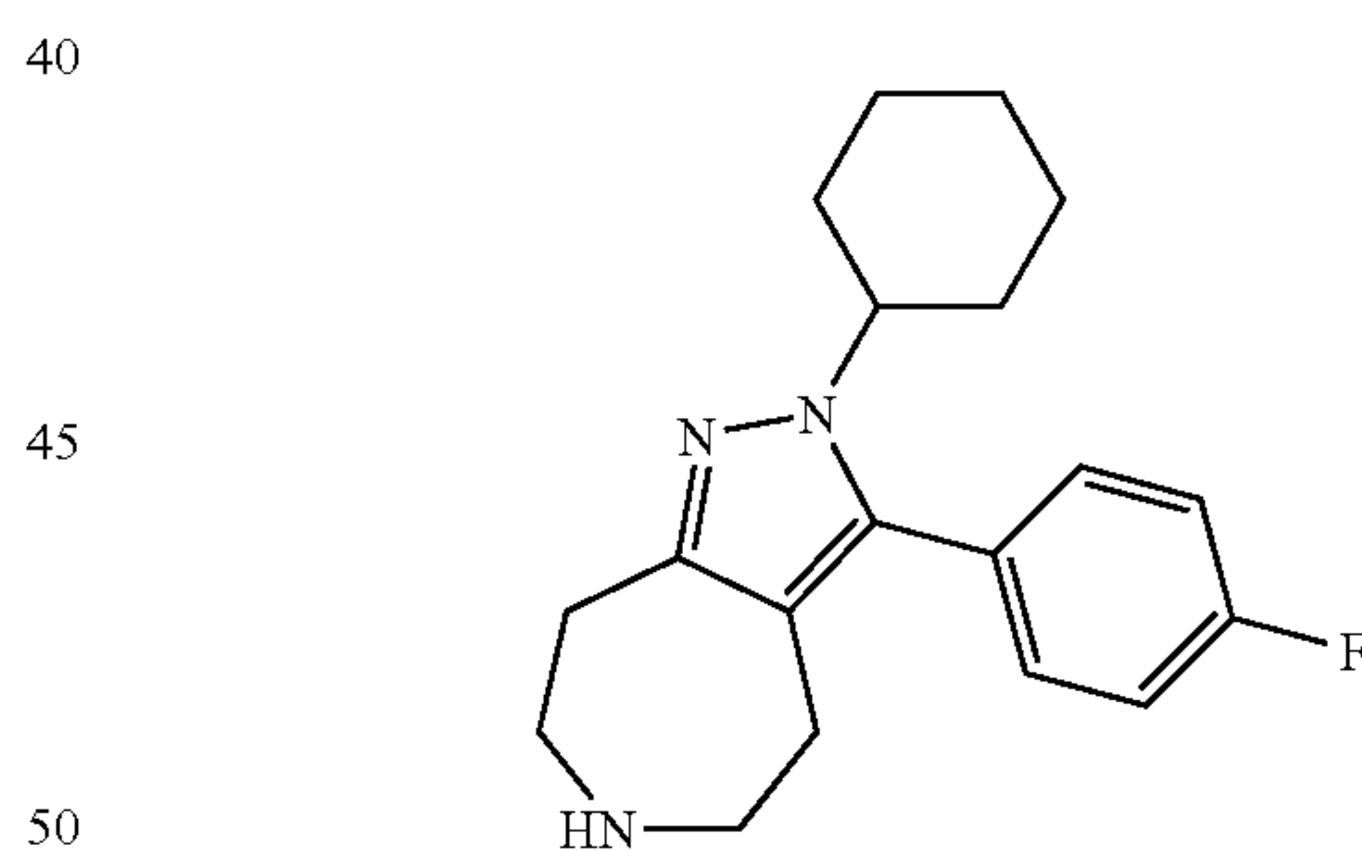
2-Cyclohexyl-3-(4-fluoro-phenyl)-2,4,5,6,7,8-hexahydro-1,2,6-triaza-azulene
