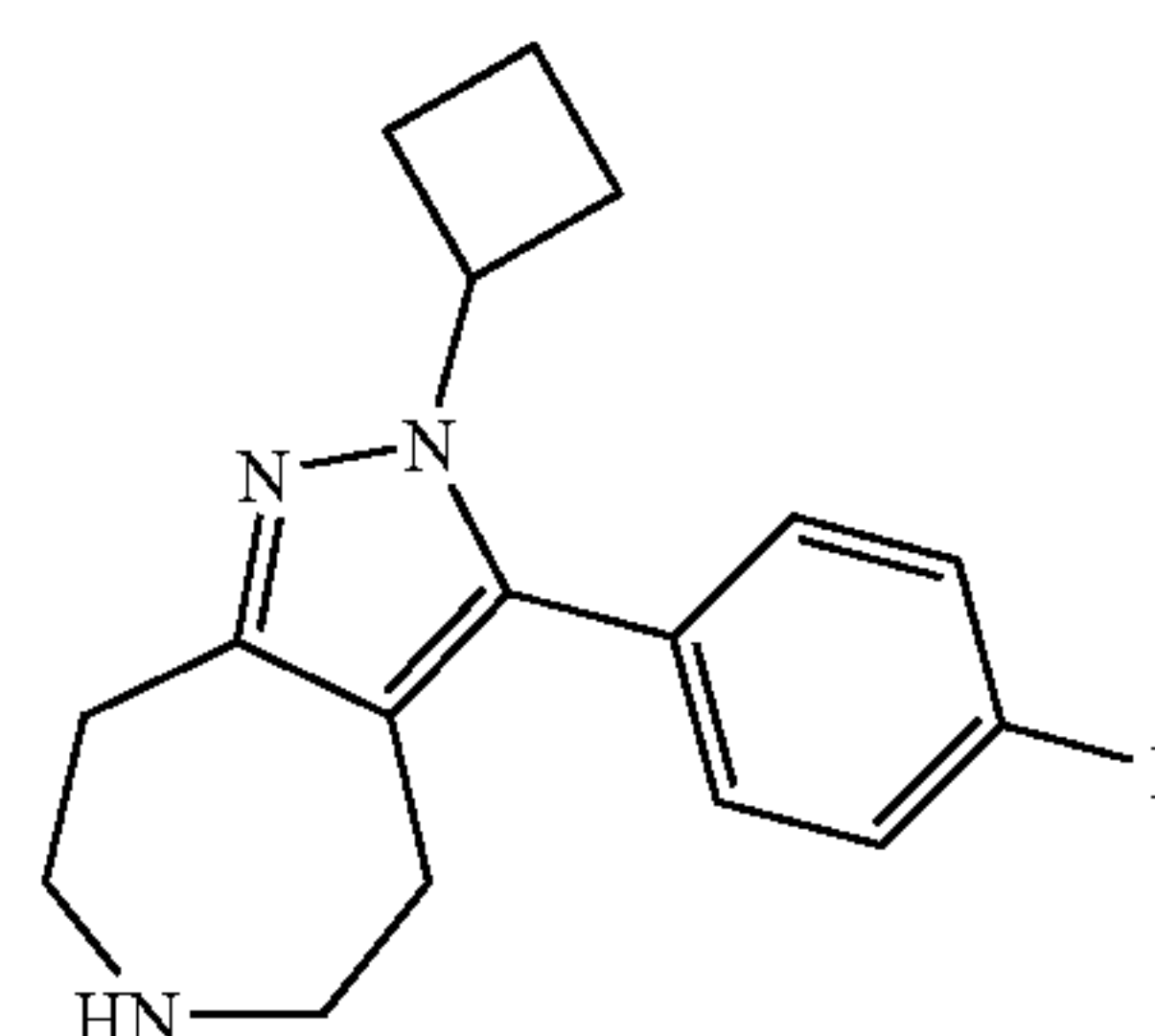
2-Cyclobutyl-3-(4-fluorophenyl)-2,4,5,6,7,8-hexahydro-1,2,6-triaza-azulene
