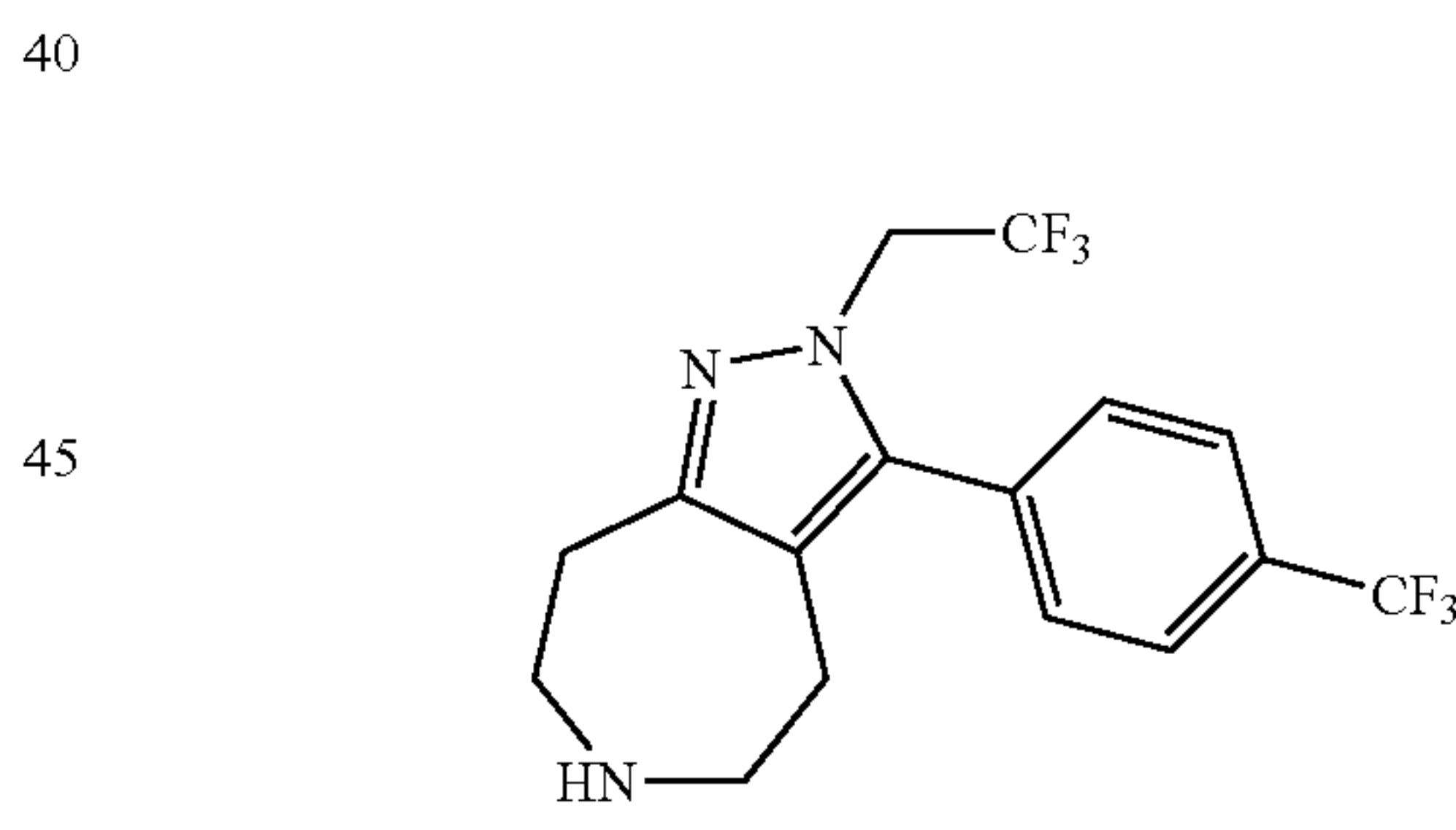
2-(2,2,2-Trifluoro-ethyl)-3-(4-trifluoromethyl-phenyl)-2,4,5,6,7,8-hexahydro-1,2,6-triaza-azulene
