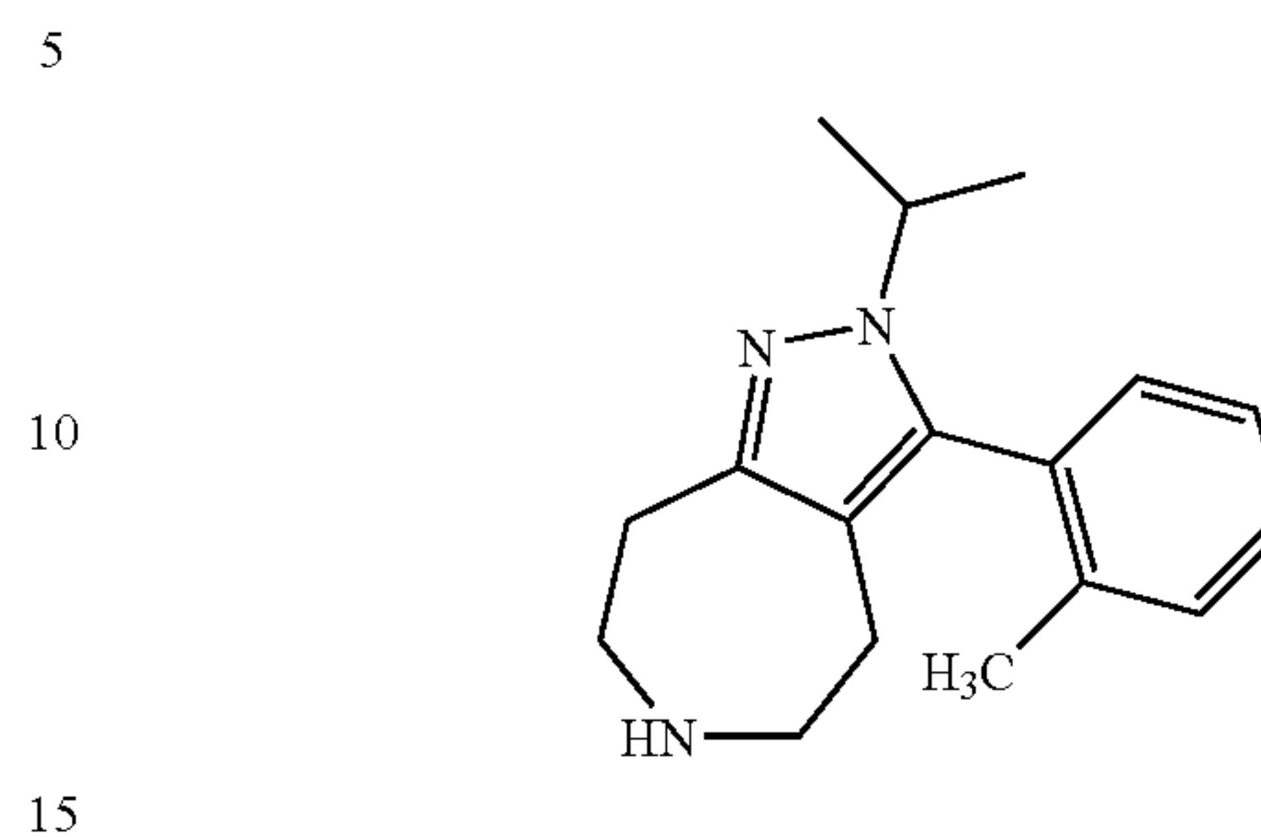
2-Isopropyl-3-o-tolyl-2,4,5,6,7,8-hexahydro-1,2,6-triaza-azulene
