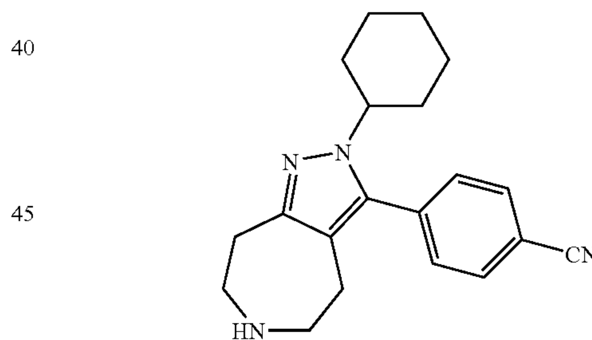
4-(2-Cyclohexyl-2,4,5,6,7,8-hexahydro-1,2,6-triaza-azulen-3-yl)-benzonitrile
