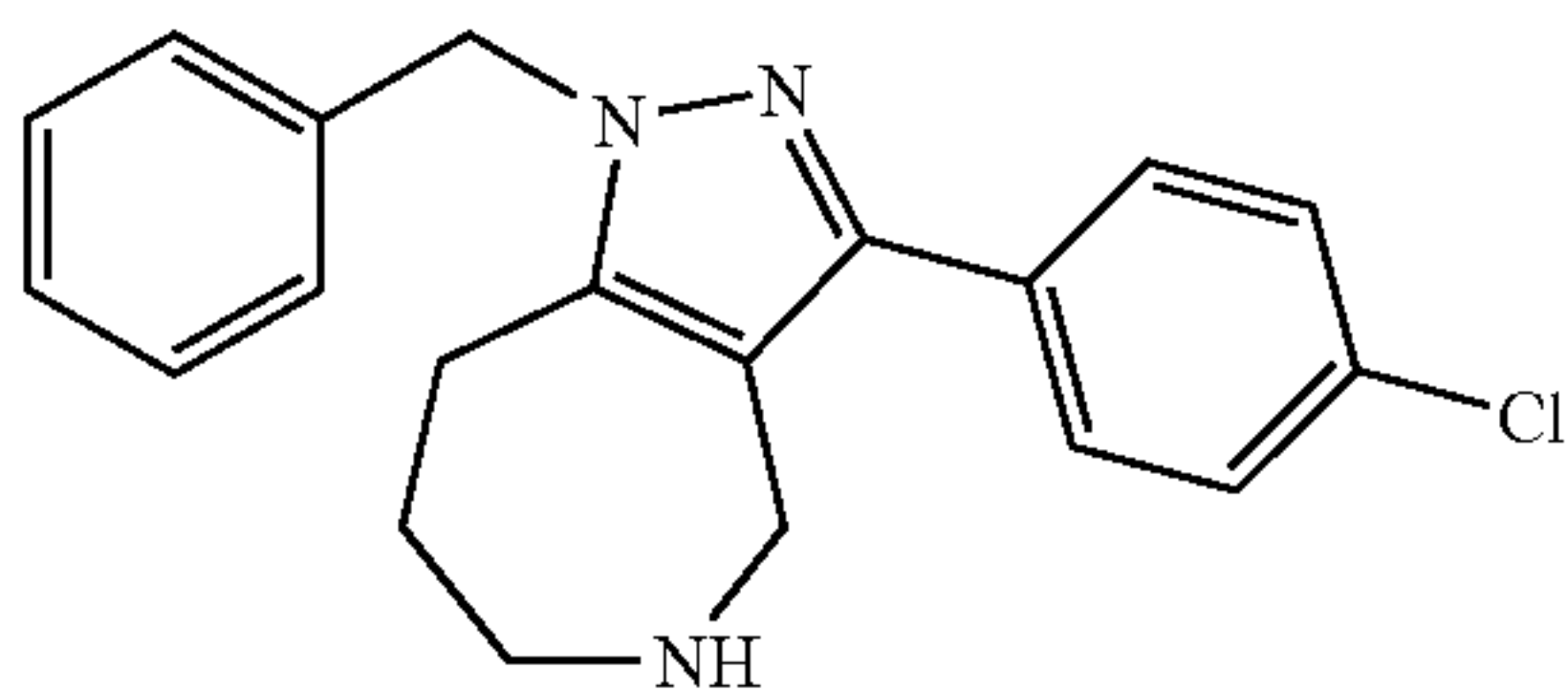
1-Benzyl-3-(4-chloro-phenyl)-1,4,5,6,7,8-hexahydro-1,2,5-triaza-azulene
