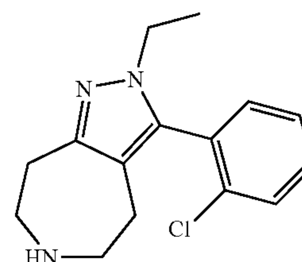
3-(2-Chloro-phenyl)-2-ethyl-2,4,5,6,7,8-hexahydro-1,2,6-triaza-azulene
