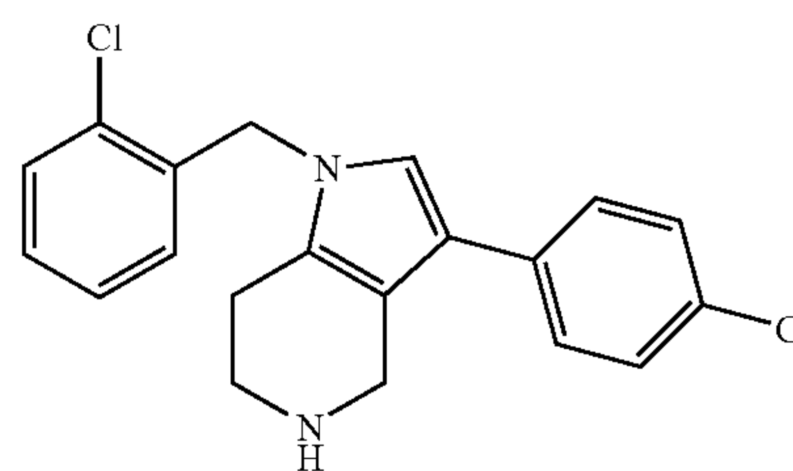
1-(2-Chloro-benzyl)-3-(4-chloro-phenyl)-4,5,6,7-tetrahydro-1H-pyrrolo[3,2-c]pyridine
