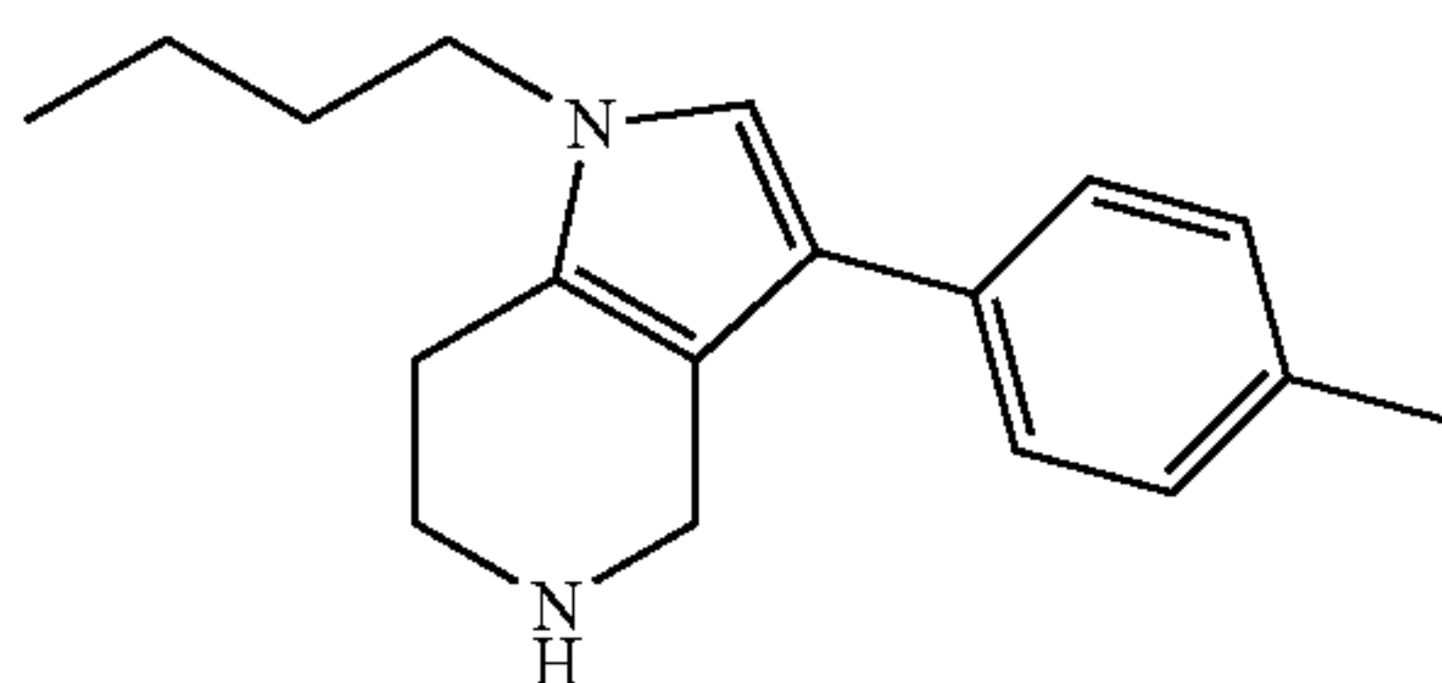
1-Butyl-3-p-tolyl-4,5,6,7-tetrahydro-1H-pyrrolo[3,2-c]pyridine
