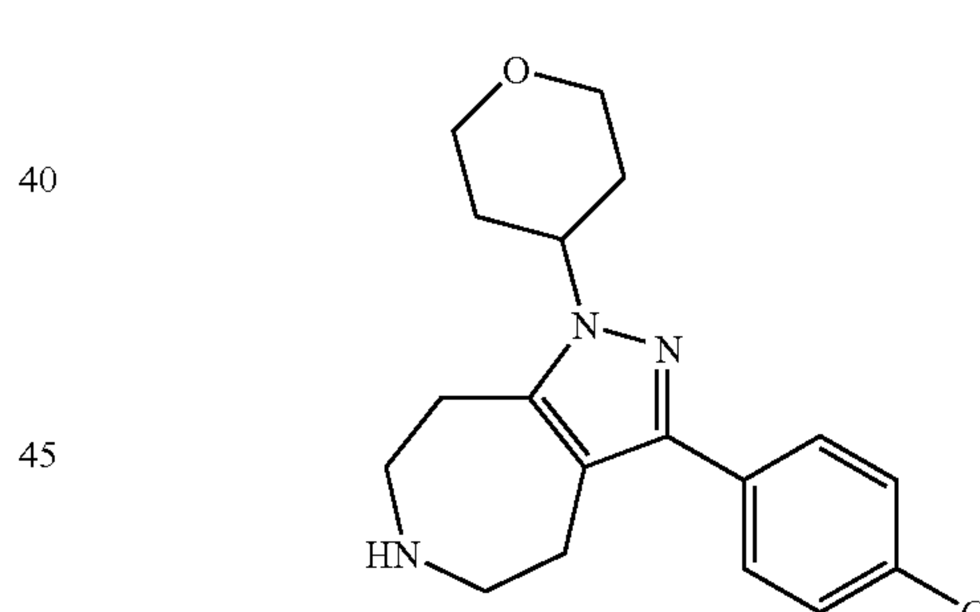
3-(4-Chloro-phenyl)-1-(tetrahydro-pyran-4-yl)-1,4,5, 6,7,8-hexahydro-1,2,6-triaza-azulene
