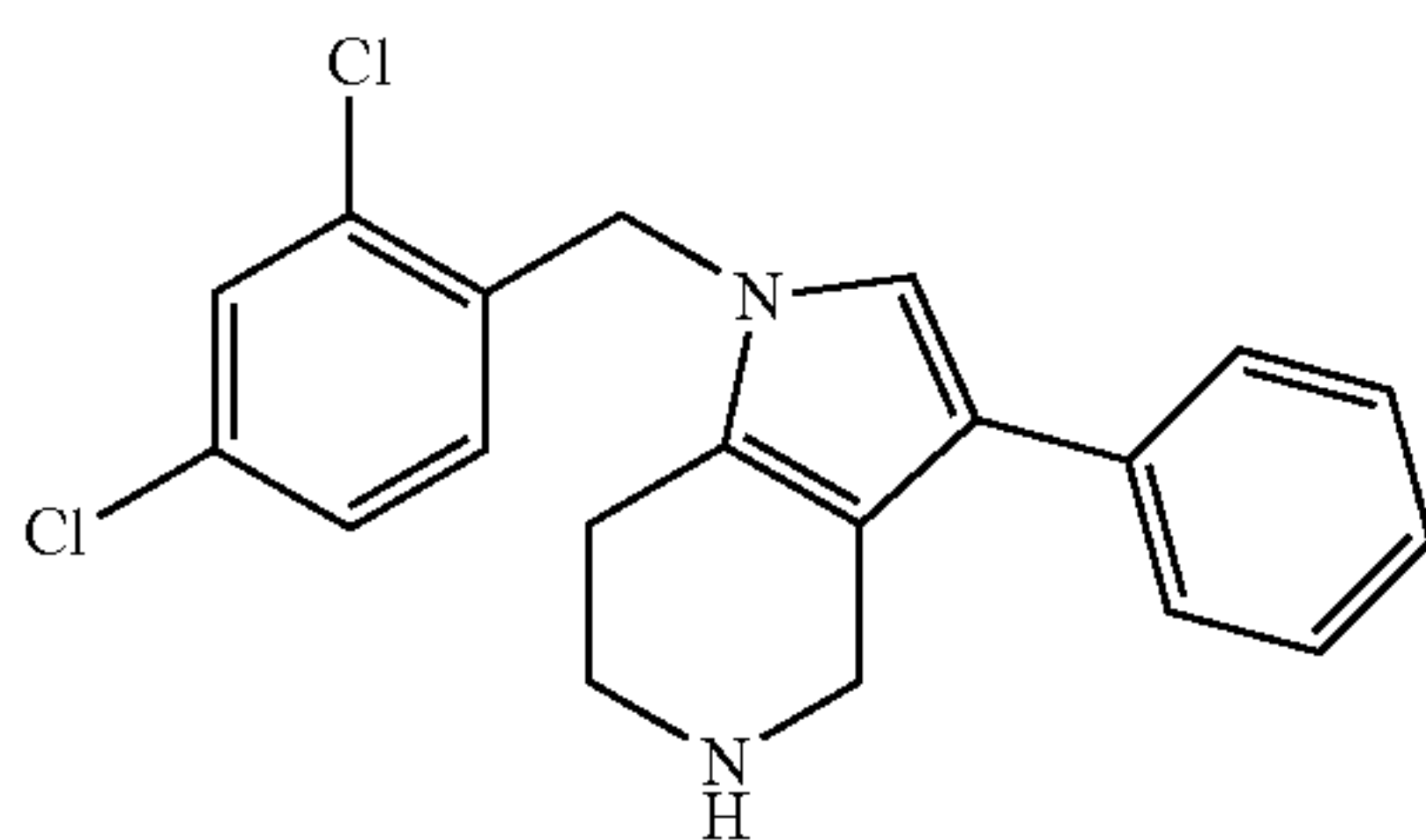
1-(2,4-Dichloro-benzyl)-3-phenyl-4,5,6,7-tetrahydro-1H-pyrrolo[3,2-c]pyridine
