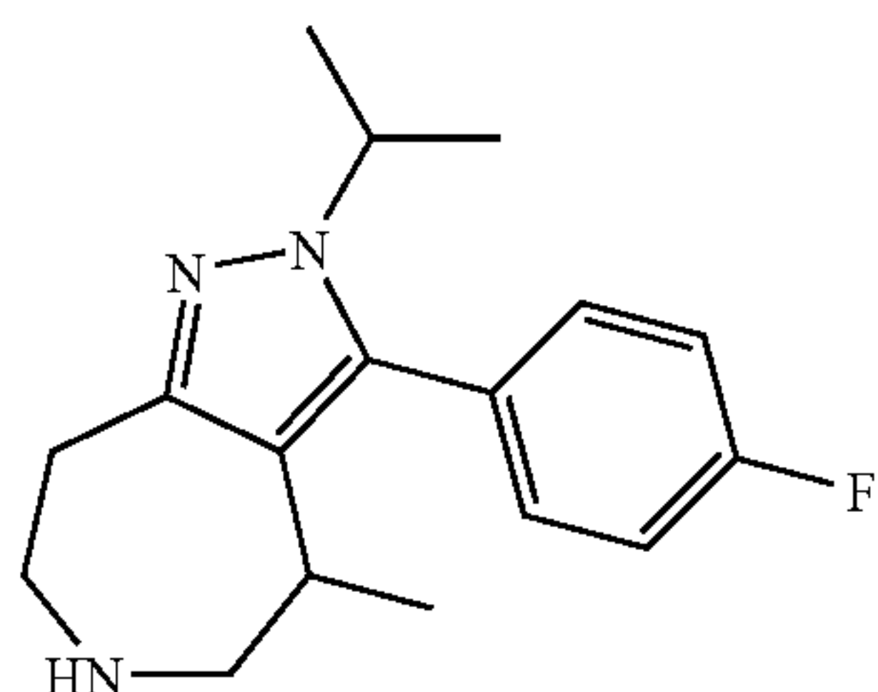
3-(4-Fluoro-phenyl)-2-isopropyl-4-methyl-2,4,5,6,7, 8-hexahydro-1,2,6-triaza-azulene
