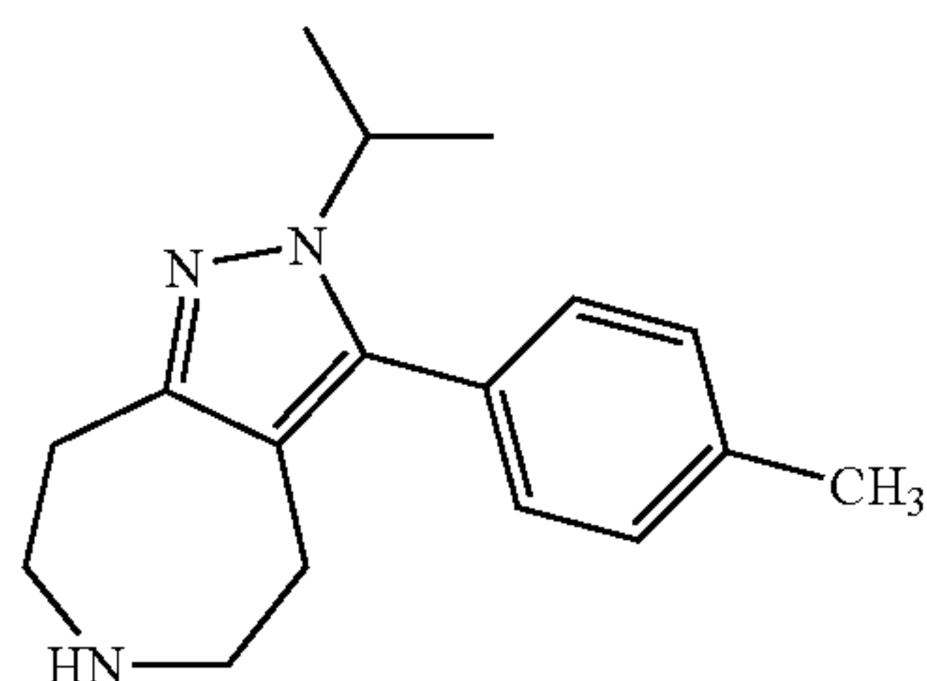
2-Isopropyl-3-p-tolyl-2,4,5,6,7,8-hexahydro-1,2,6-triaza-azulene
