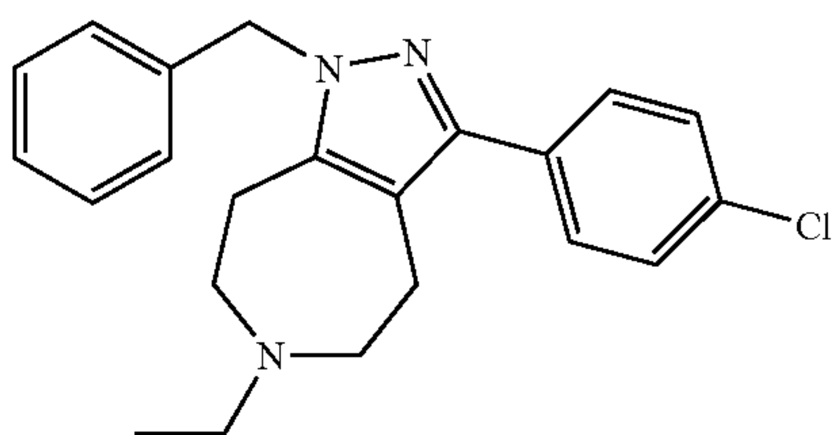
1-Benzyl-3-(4-chloro-phenyl)-6-ethyl-1,4,5,6,7,8-hexahydro-1,2,6-triaza-azulene
