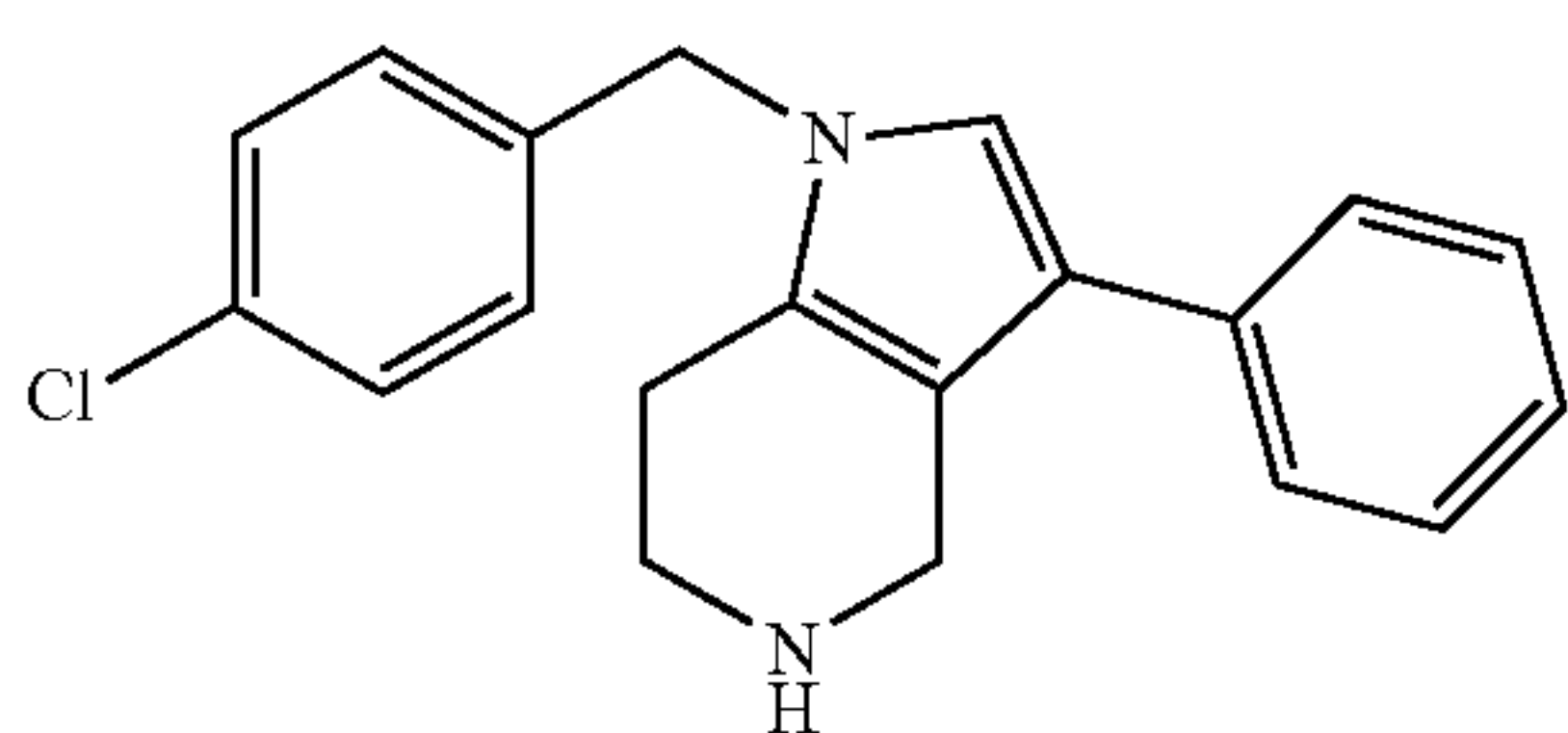
1-(4-Chloro-benzyl)-3-phenyl-4,5,6,7-tetrahydro-1H-pyrrolo[3,2-c]pyridine
