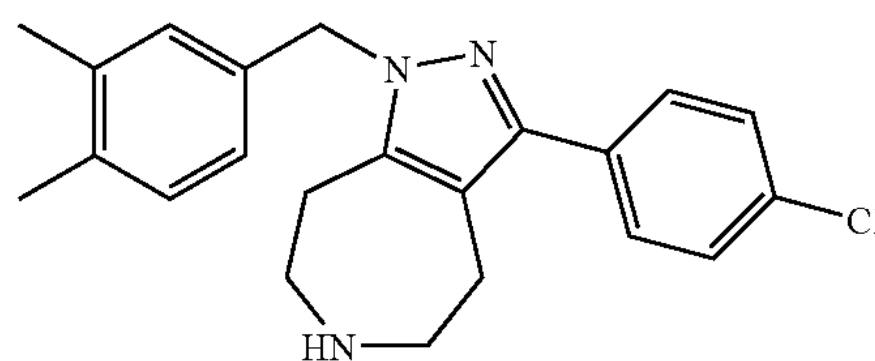
3-(4-Chloro-phenyl)-1-(3,4-dimethyl-benzyl)-1,4,5, 6,7,8-hexahydro-1,2,6-triaza-azulene
