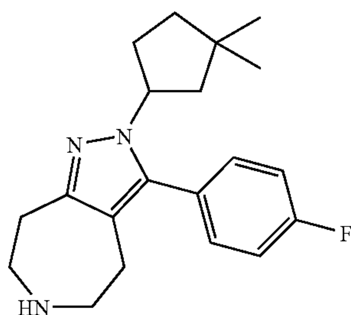
2-(3,3-Dimethyl-cyclopentyl)-3-(4-fluoro-phenyl)-2,4,5,6,7,8-hexahydro-1,2,6-triaza-azulene
