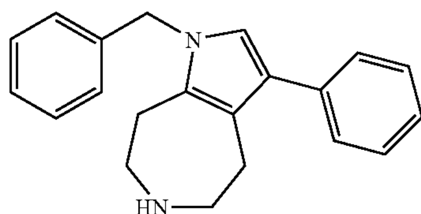
1-Benzyl-3-phenyl-1,4,5,6,7,8-hexahydro-pyrrolo[2,3-d]azepine
