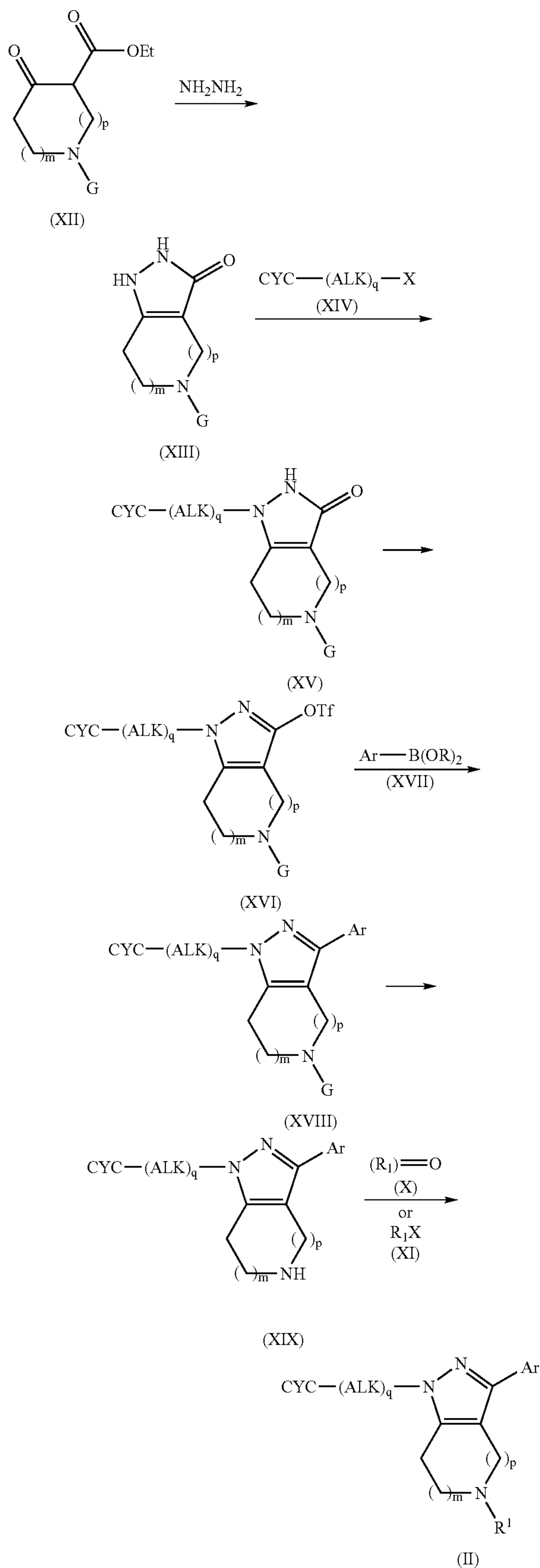
Scheme 2
