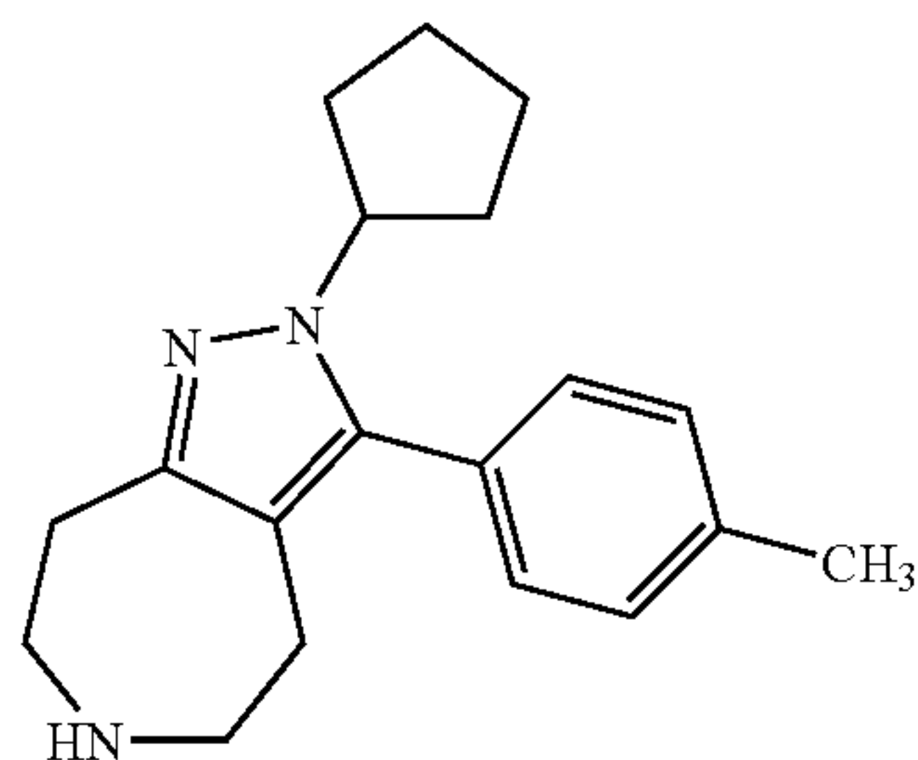
2-Cyclopentyl-3-p-tolyl-2,4,5,6,7,8-hexahydro-1,2,6-triaza-azulene
