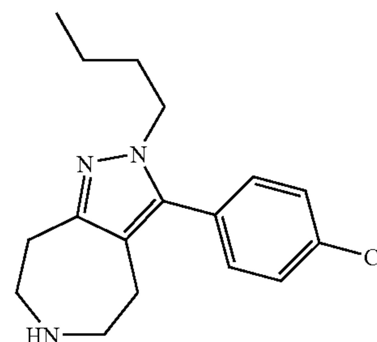
2-Butyl-3-(4-chloro-phenyl)-2,4,5,6,7,8-hexahydro-1,2,6-triaza-azulene
