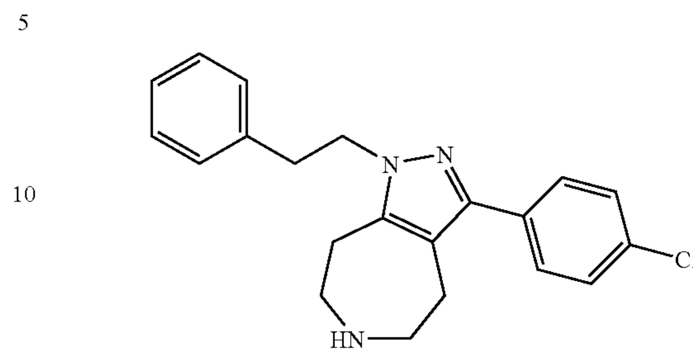
3-(4-Chloro-phenyl)-1-phenethyl-1,4,5,6,7,8-hexahydro-1,2,6-triaza-azulene
