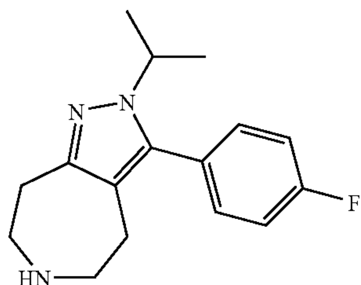
3-(4-Fluoro-phenyl)-2-isopropyl-2,4,5,6,7,8-hexahydro-1,2,6-triaza-azulene
