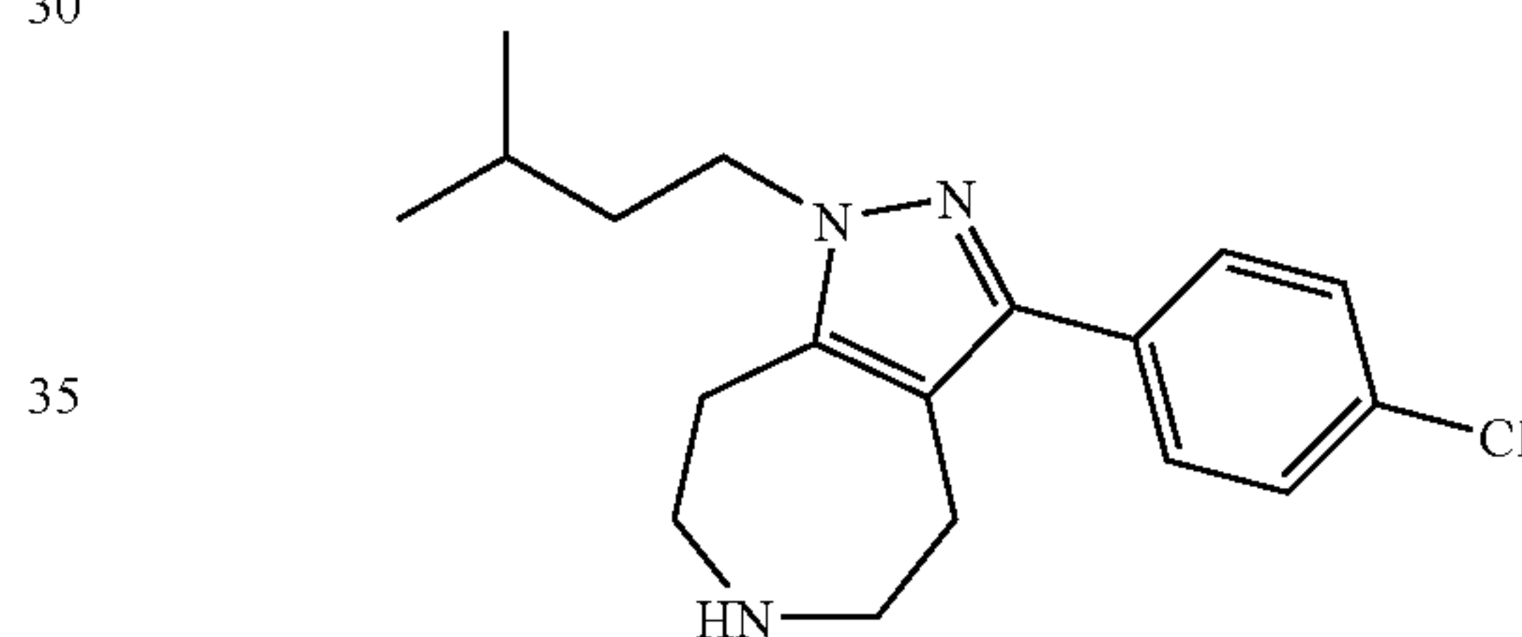
3-(4-Chloro-phenyl)-1-(3-methyl-butyl)-1,4,5,6,7,8-hexahydro-1,2,6-triaza-azulene
