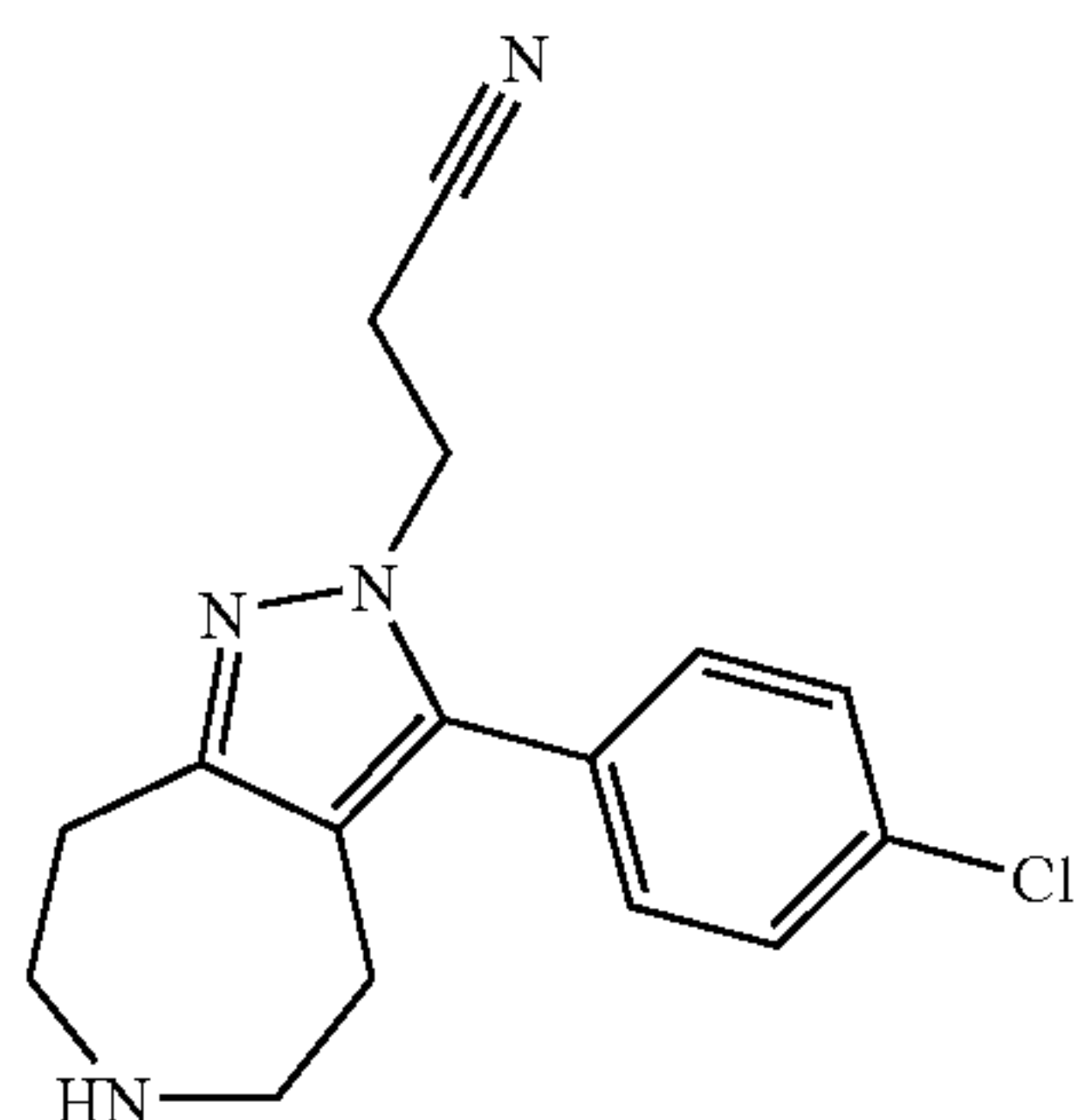
3-[3-(4-Chloro-phenyl)-5,6,7,8-tetrahydro-4H-1,2,6-triaza-azulen-2-yl]-propionitrile
