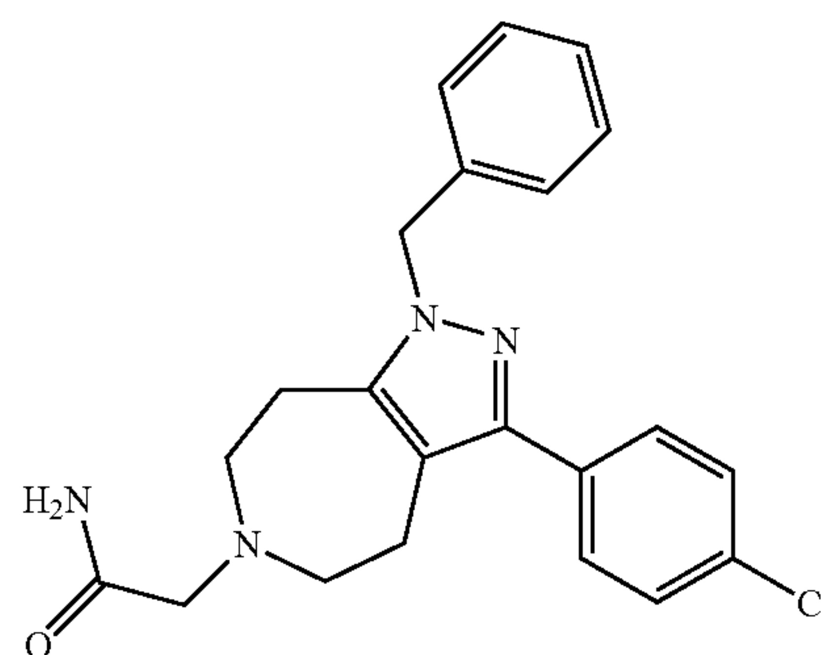
2-[1-Benzyl-3-(4-chloro-phenyl)-4,5,7,8-tetrahydro-1H-1,2,6-triaza-azulen-6-yl]-acetamide
