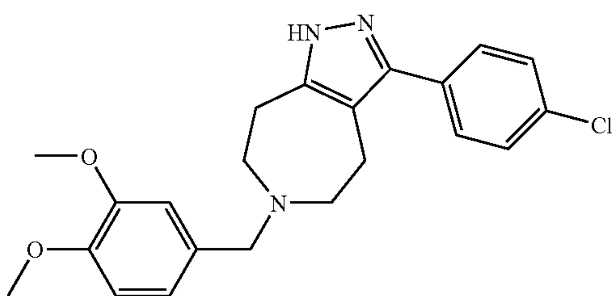
3-(4-Chloro-phenyl)-6-(3,4-dimethoxy-benzyl)-1,4,5,6,7,8-hexahydro-1,2,6-triaza-azulene
