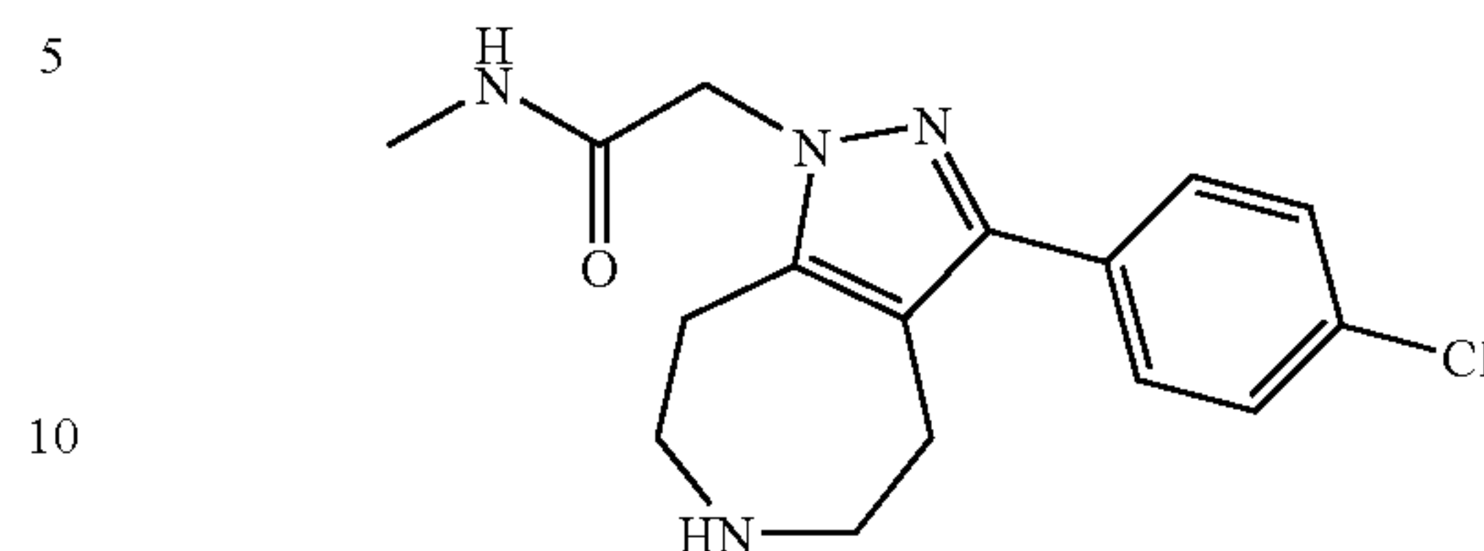
2-[3-(4-Chloro-phenyl)-5,6,7,8-tetrahydro-4H-1,2,6- triaza-azulen-1-yl]-N-methyl-acetamide
