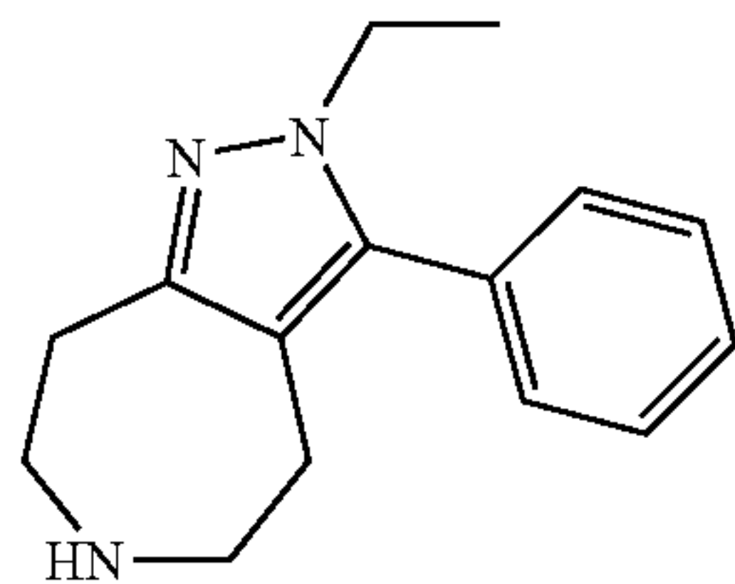
2-Ethyl-3-phenyl-2,4,5,6,7,8-hexahydro-1,2,6-triaza-azulene
