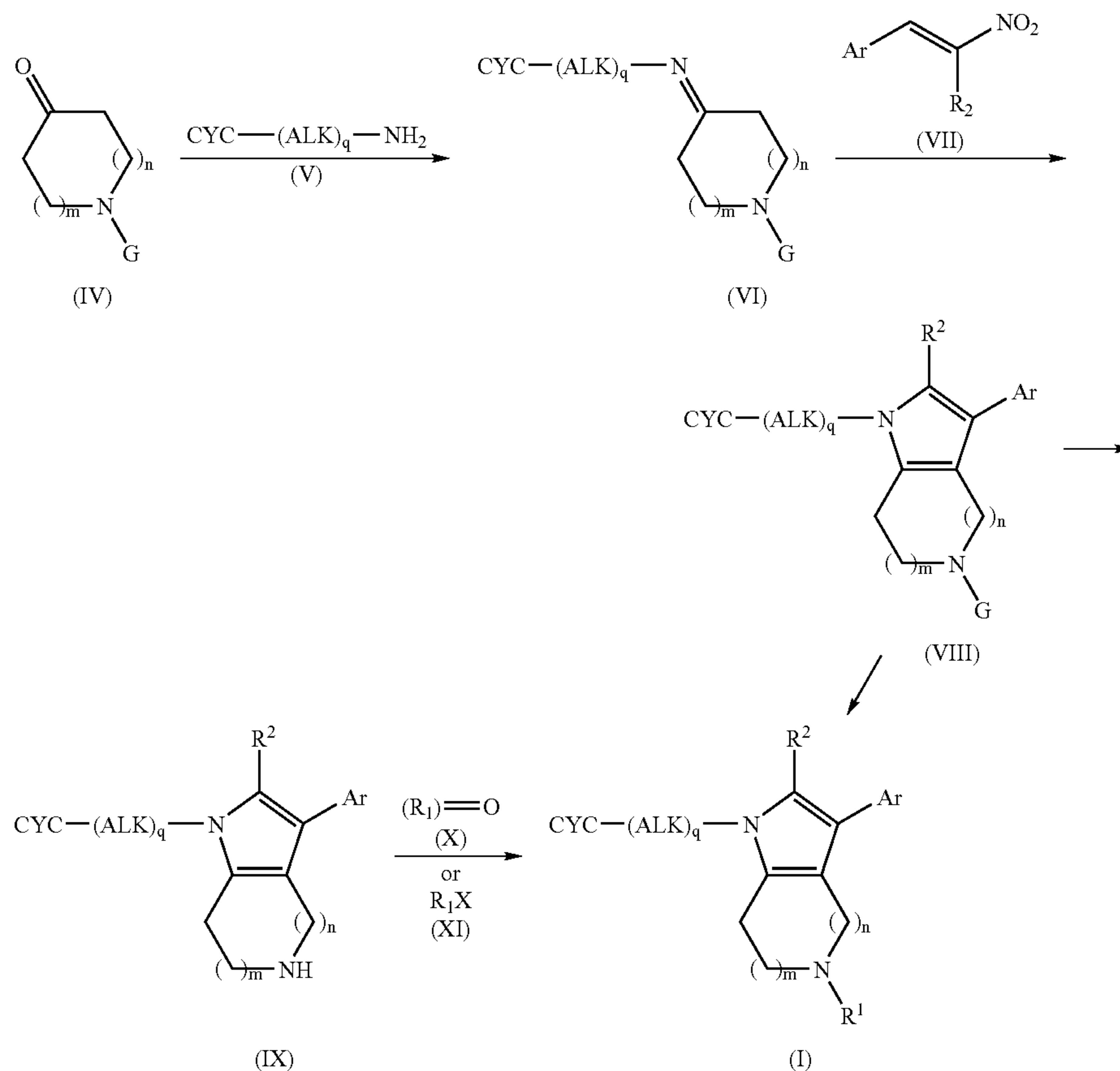
Scheme 1
