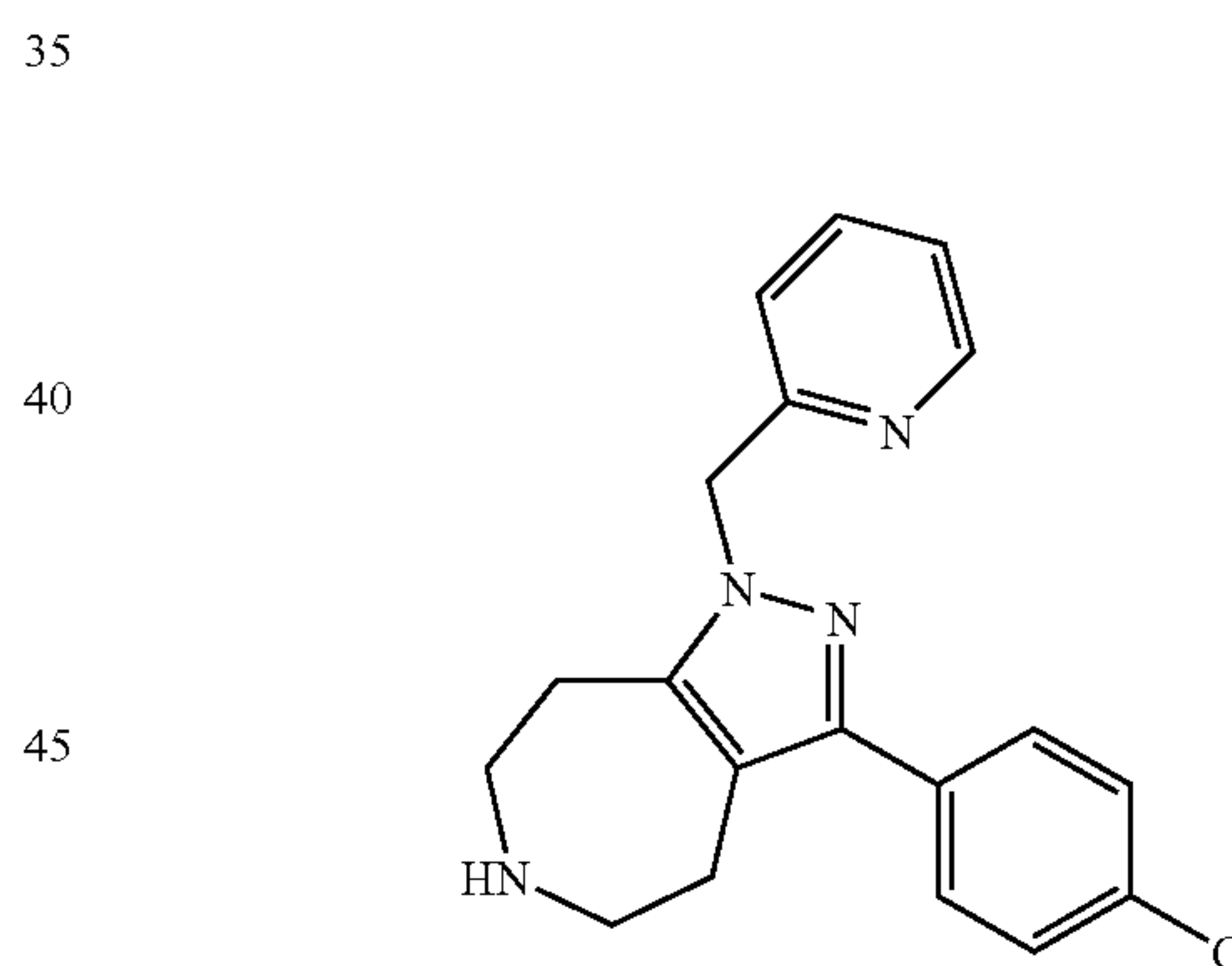
2-Isopropyl-7-methyl-3-p-tolyl-2,4,5,6,7,8-hexahy- dro-1,2,6-triaza-azulene
