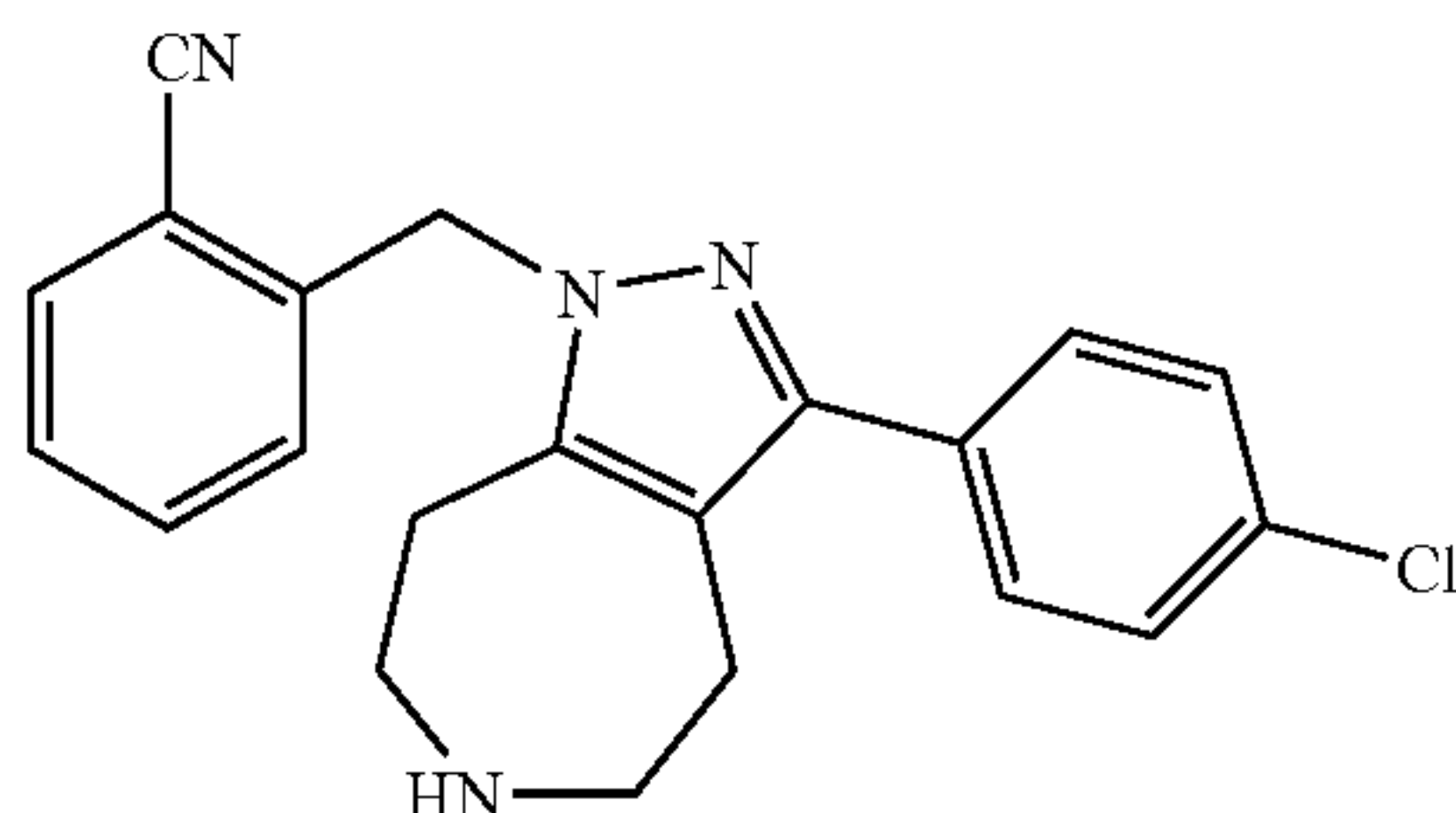
2-[3-(4-Chloro-phenyl)-5,6,7,8-tetrahydro-4H-1,2,6-triaza-azulen-1-ylmethyl]-benzonitrile
