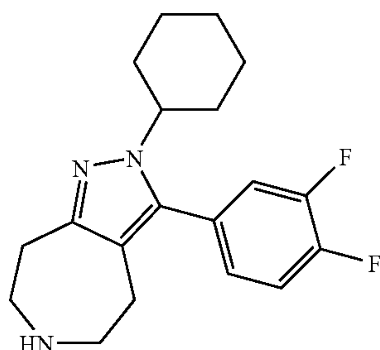
2-Cyclohexyl-3-(3,4-difluoro-phenyl)-2,4,5,6,7,8-hexahydro-1,2,6-triaza-azulene
