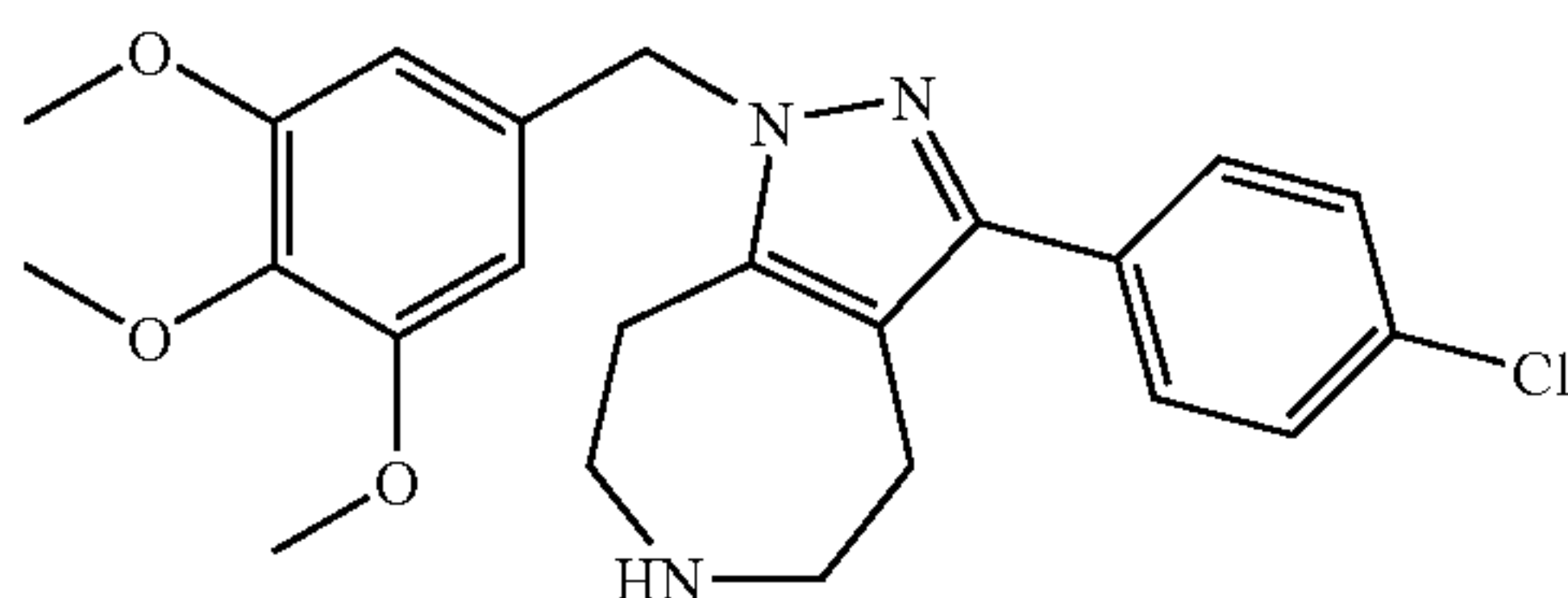
3-(4-Chloro-phenyl)-1-(3,4,5-trimethoxy-benzyl)-4,5,6,7,8-hexahydro-1,2,6-triaza-azulene
