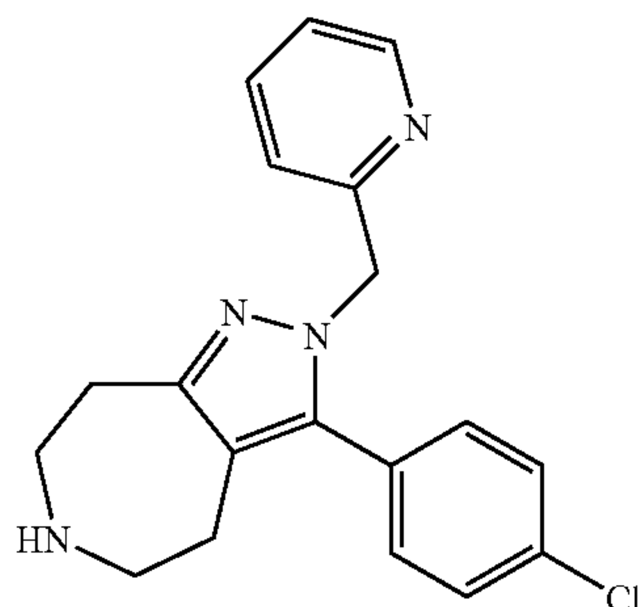
3-(4-Chloro-phenyl)-2-pyridin-2-ylmethyl-1,4,5,6,7, 8-hexahydro-1,2,6-triaza-azulene
