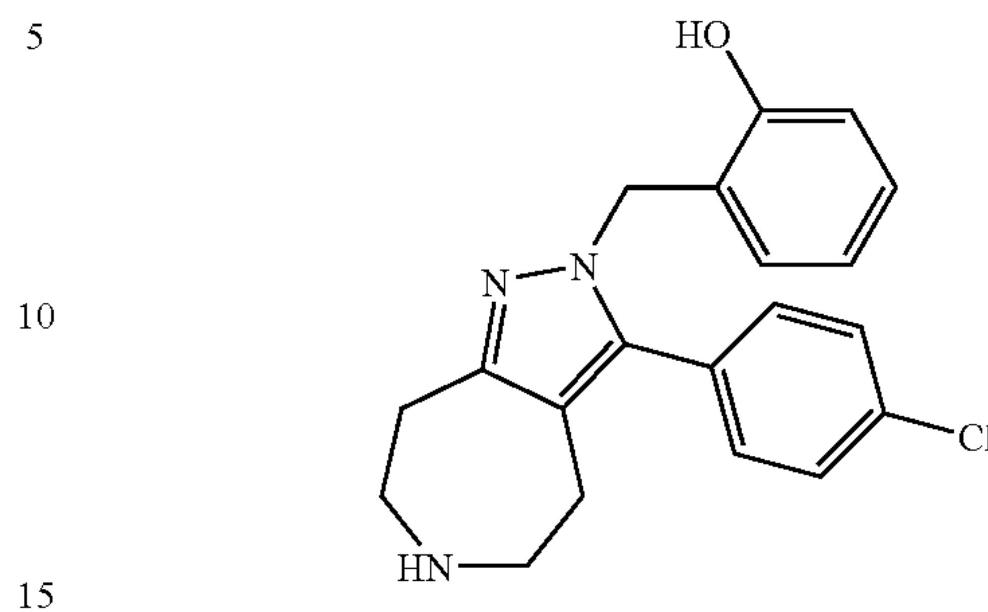
2-[3-(4-Chloro-phenyl)-5,6,7,8-tetrahydro-4H-1,2,6-triaza-azulen-2-ylmethyl]-phenol
