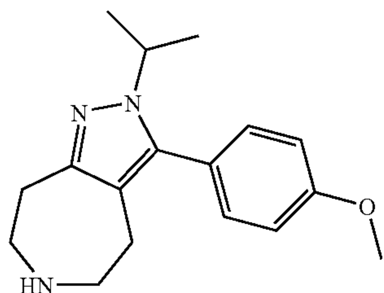
2-Isopropyl-3-(4-methoxy-phenyl)-2,4,5,6,7,8- hexahydro-1,2,6-triaza-azulene
