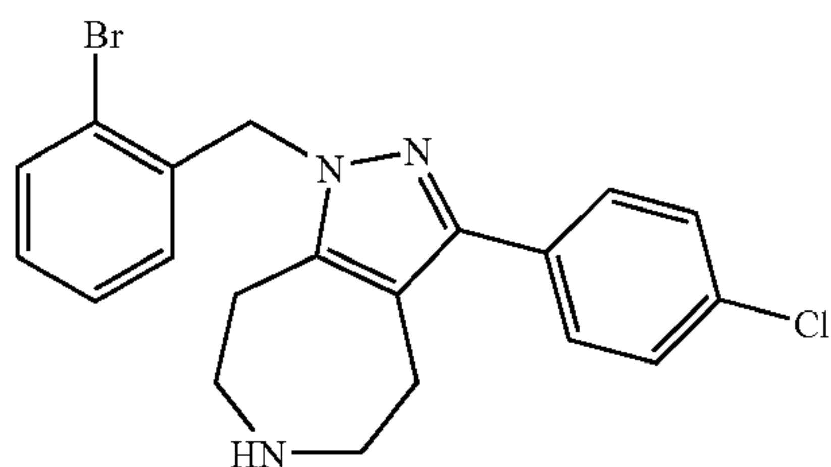
1-(2-Bromo-benzyl)-3-(4-chloro-phenyl)-1,4,5,6,7,8-hexahydro-1,2,6-triaza-azulene
