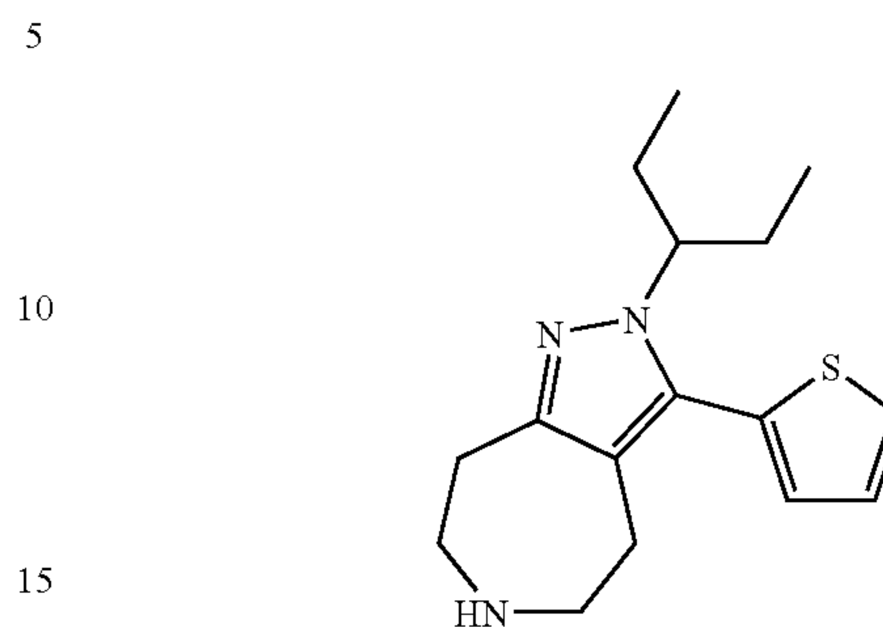
2-(1-Ethyl-propyl)-3-thiophen-2-yl-2,4,5,6,7,8-hexahydro-1,2,6-triaza-azulene
