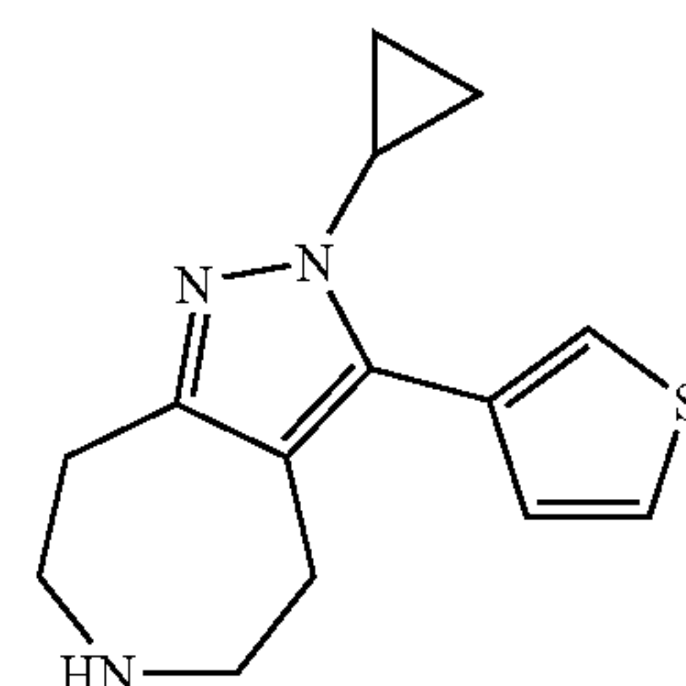
2-Cyclopropyl-3-thiophen-3-yl-2,4,5,6,7,8-hexahydro-1,2,6-triaza-azulene
