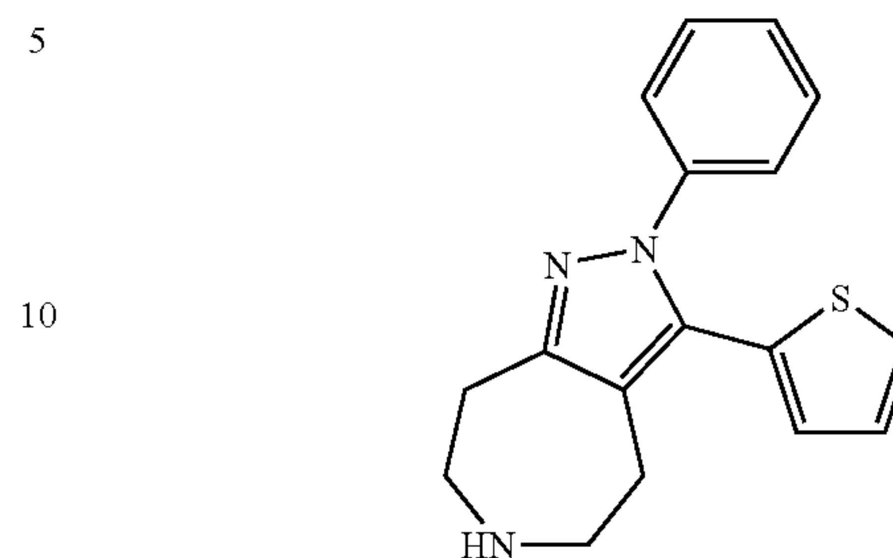
2-Phenyl-3-thiophen-2-yl-2,4,5,6,7,8-hexahydro-1,2,6-triaza-azulene
