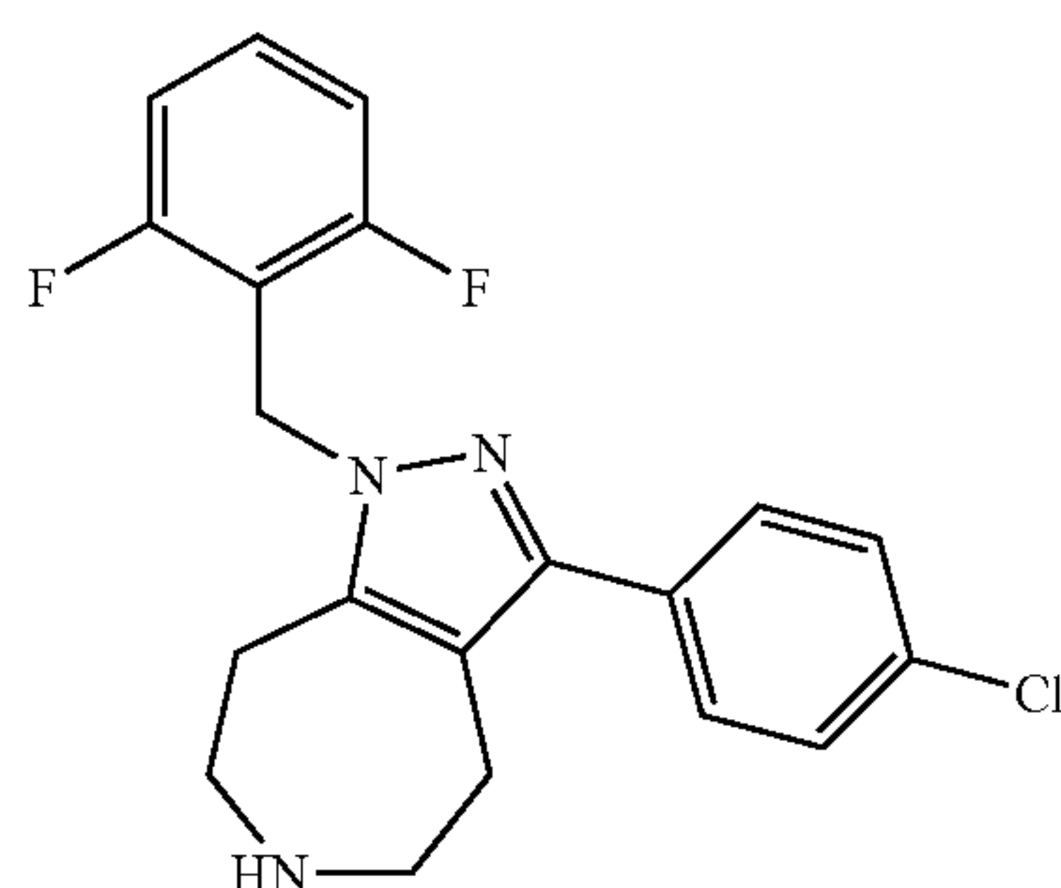
3-(4-Chloro-phenyl)-1-(2,6-difluoro-benzyl)-1,4,5,6,7,8-hexahydro-1,2,6-triaza-azulene
