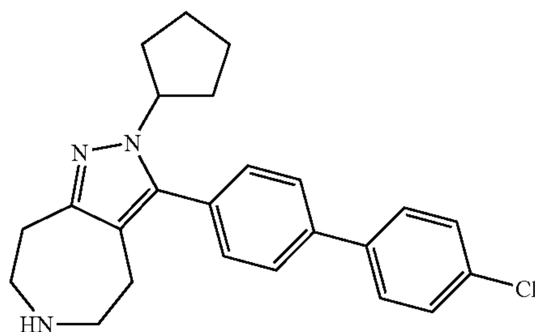
3-(4'-Chloro-biphenyl-4-yl)-2-cyclopentyl-2,4,5,6,7,8-hexahydro-1,2,6-triaza-azulene
