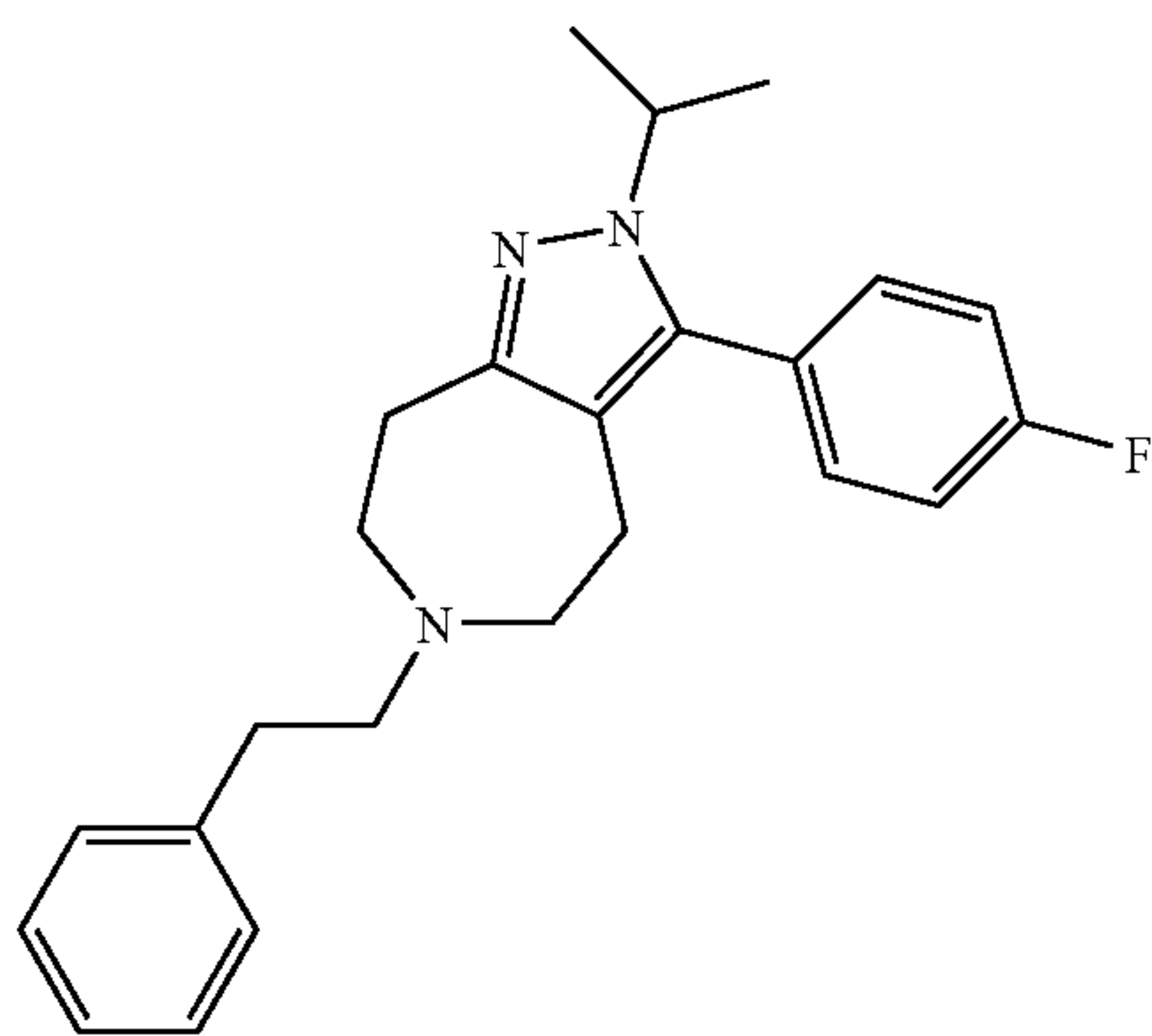
3-(4-Fluoro-phenyl)-2-isopropyl-6-phenethyl-2,4,5,6,7,8-hexahydro-1,2,6-triaza-azulene
