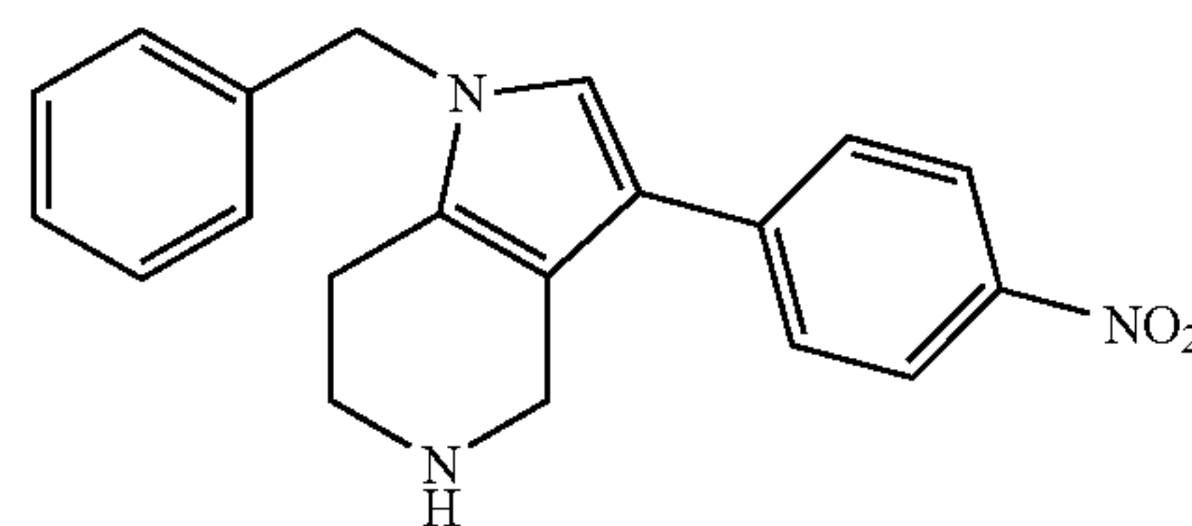
1-Benzyl-3-(4-nitro-phenyl)-4,5,6,7-tetrahydro-1H-pyrrolo[3,2-c]pyridine
