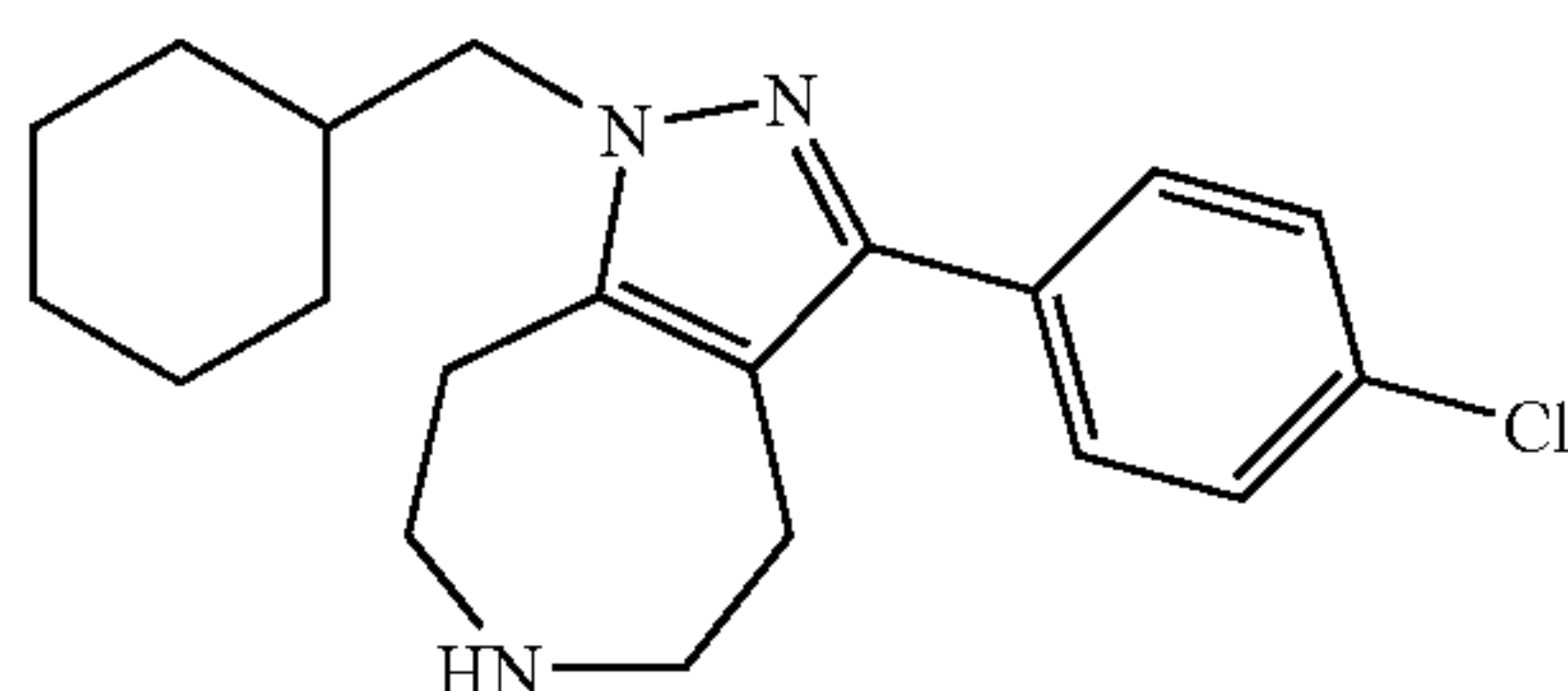
3-(4-Chloro-phenyl)-1-cyclohexylmethyl-1,4,5,6,7,8-hexahydro-1,2,6-triaza-azulene
