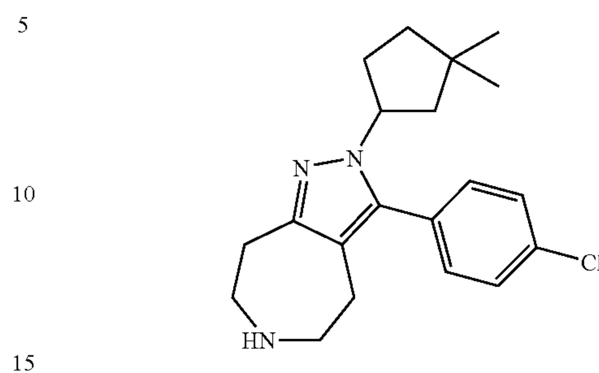
3-(4-Chloro-phenyl)-2-(3,3-dimethyl-cyclopentyl)-2,4,5,6,7,8-hexahydro-1,2,6-triaza-azulene
