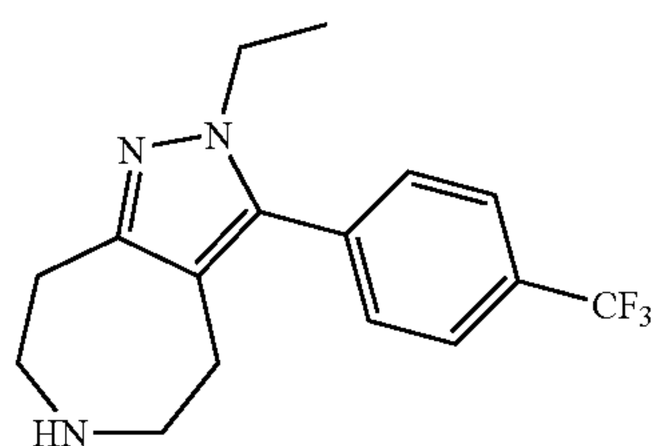
2-Ethyl-3-(4-trifluoromethyl-phenyl)-2,4,5,6,7,8-hexahydro-1,2,6-triaza-azulene
