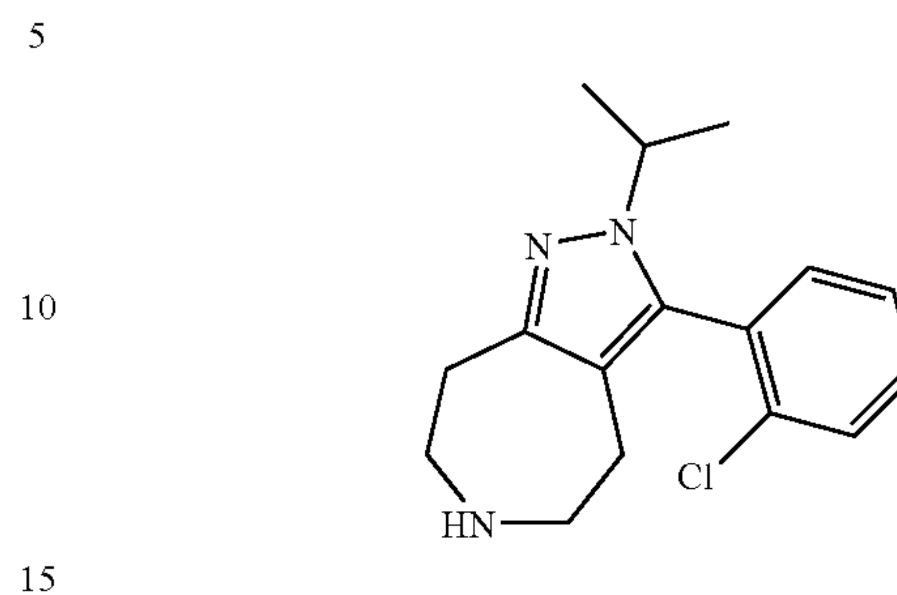
3-(2-Chloro-phenyl)-2-isopropyl-2,4,5,6,7,8-hexahydro-1,2,6-triaza-azulene
