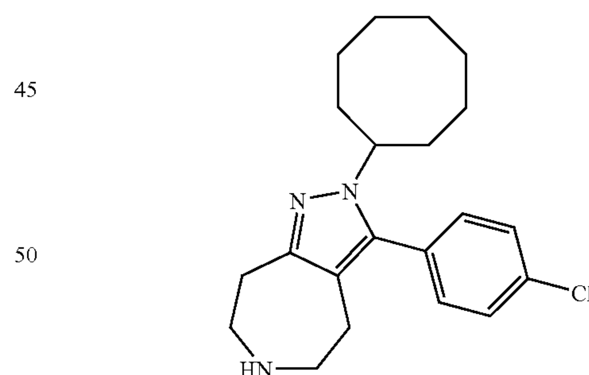
3-(4-Chloro-phenyl)-2-cyclooctyl-2,4,5,6,7,8-hexahydro-1,2,6-triaza-azulene
