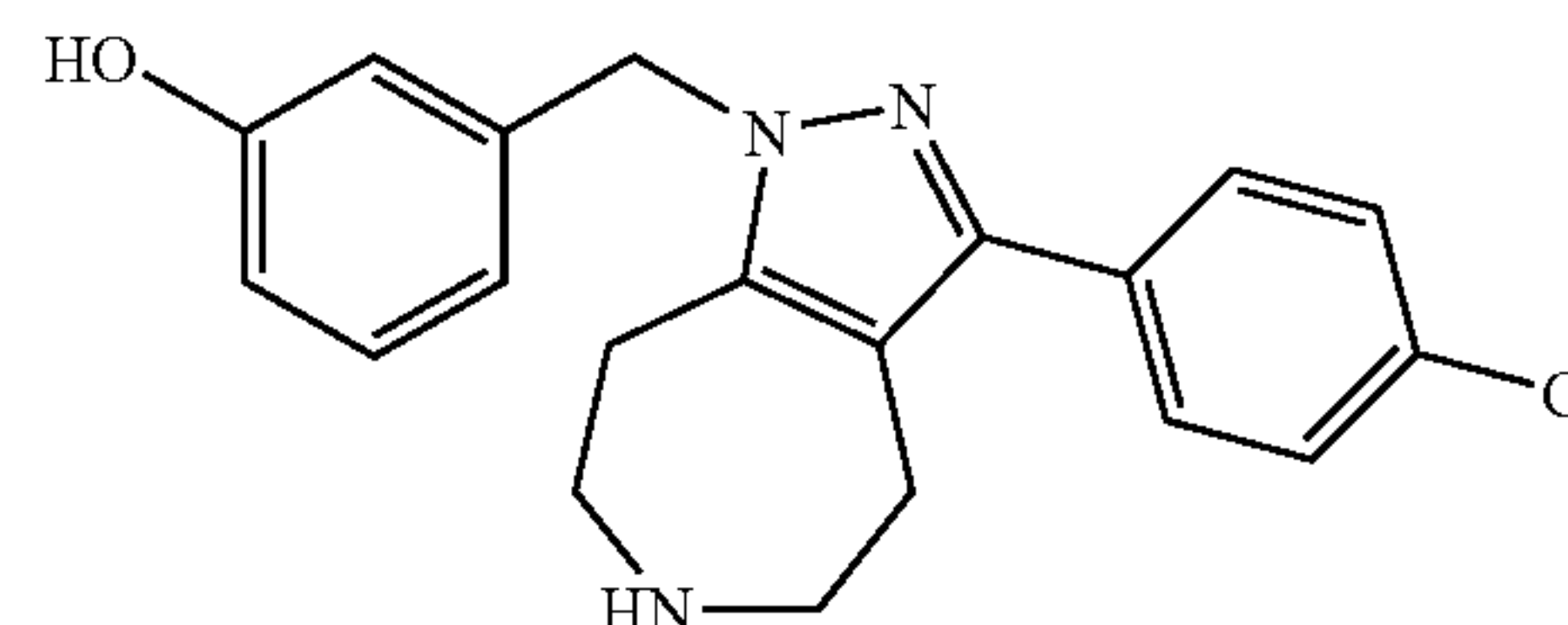
3-[3-(4-Chloro-phenyl)-5,6,7,8-tetrahydro-4H-1,2,6-triaza-azulen-1-ylmethyl]-phenol
