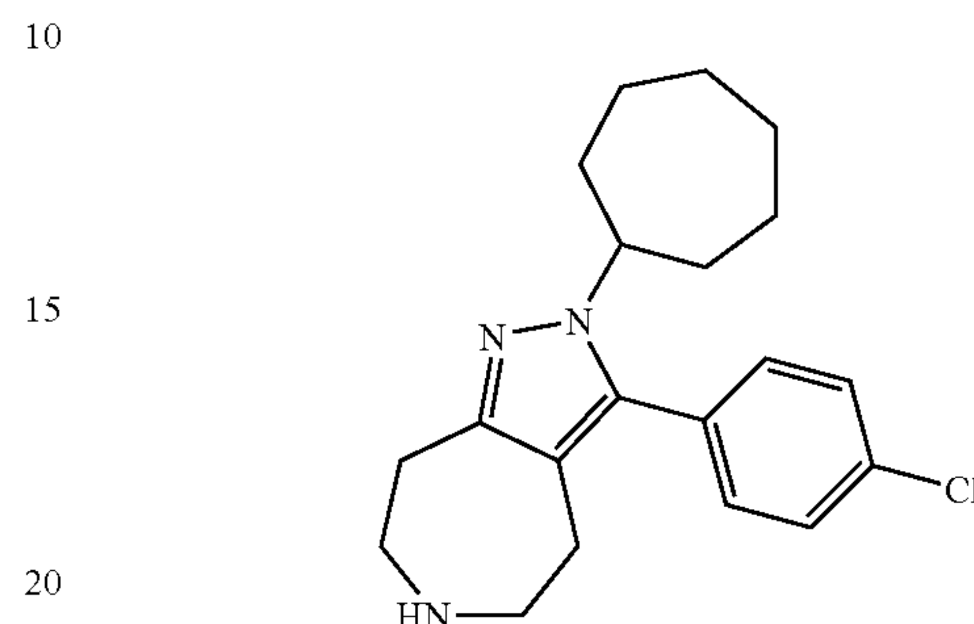
3-(4-Chloro-phenyl)-2-cycloheptyl-2,4,5,6,7,8-hexahydro-1,2,6-triaza-azulene
