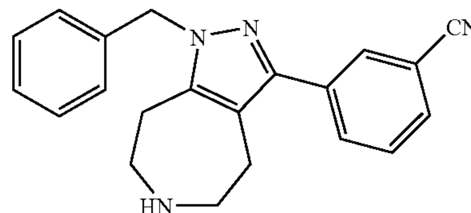
3-(1-Benzyl-1,4,5,6,7,8-hexahydro-1,2,6-triaza-azulen-3-yl)-benzonitrile
