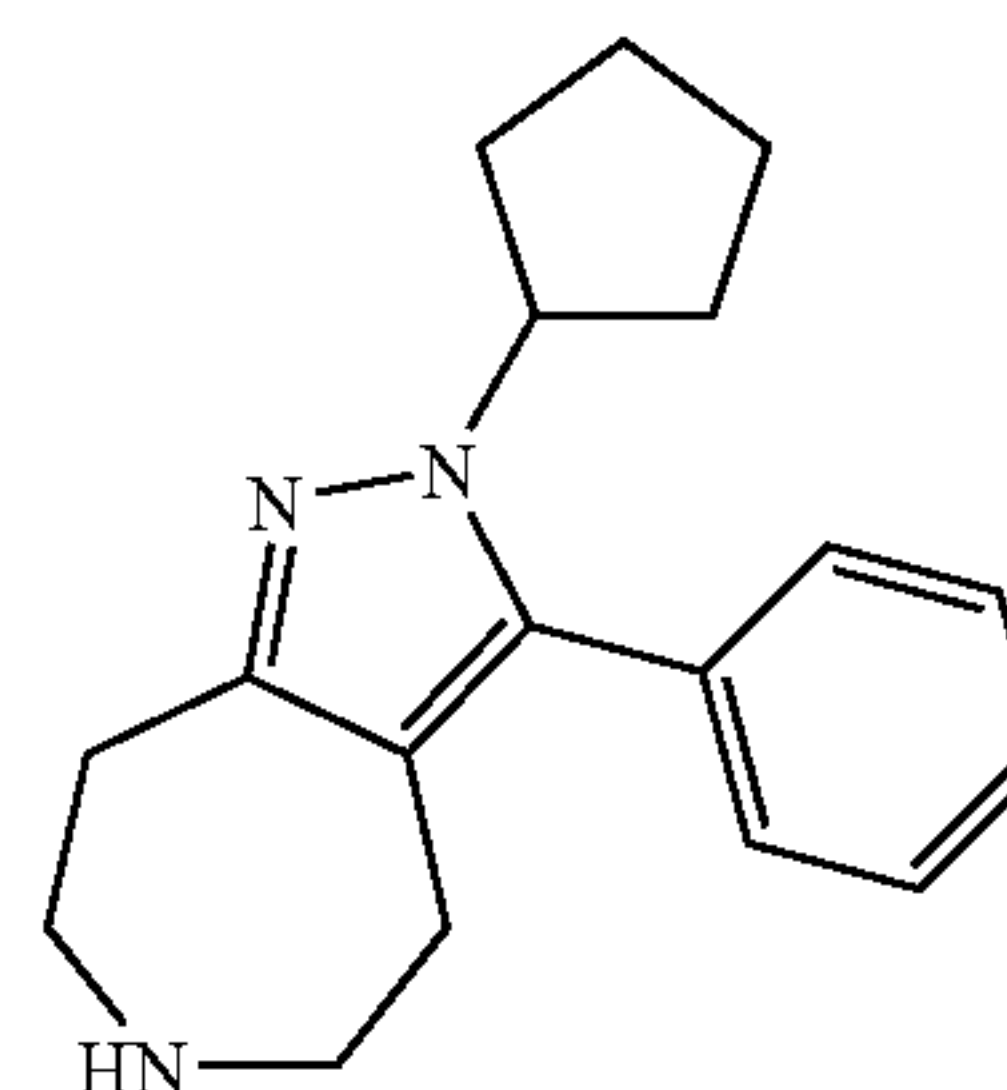
2-Cyclopentyl-3-phenyl-2,4,5,6,7,8-hexahydro-1,2,6-triaza-azulene
