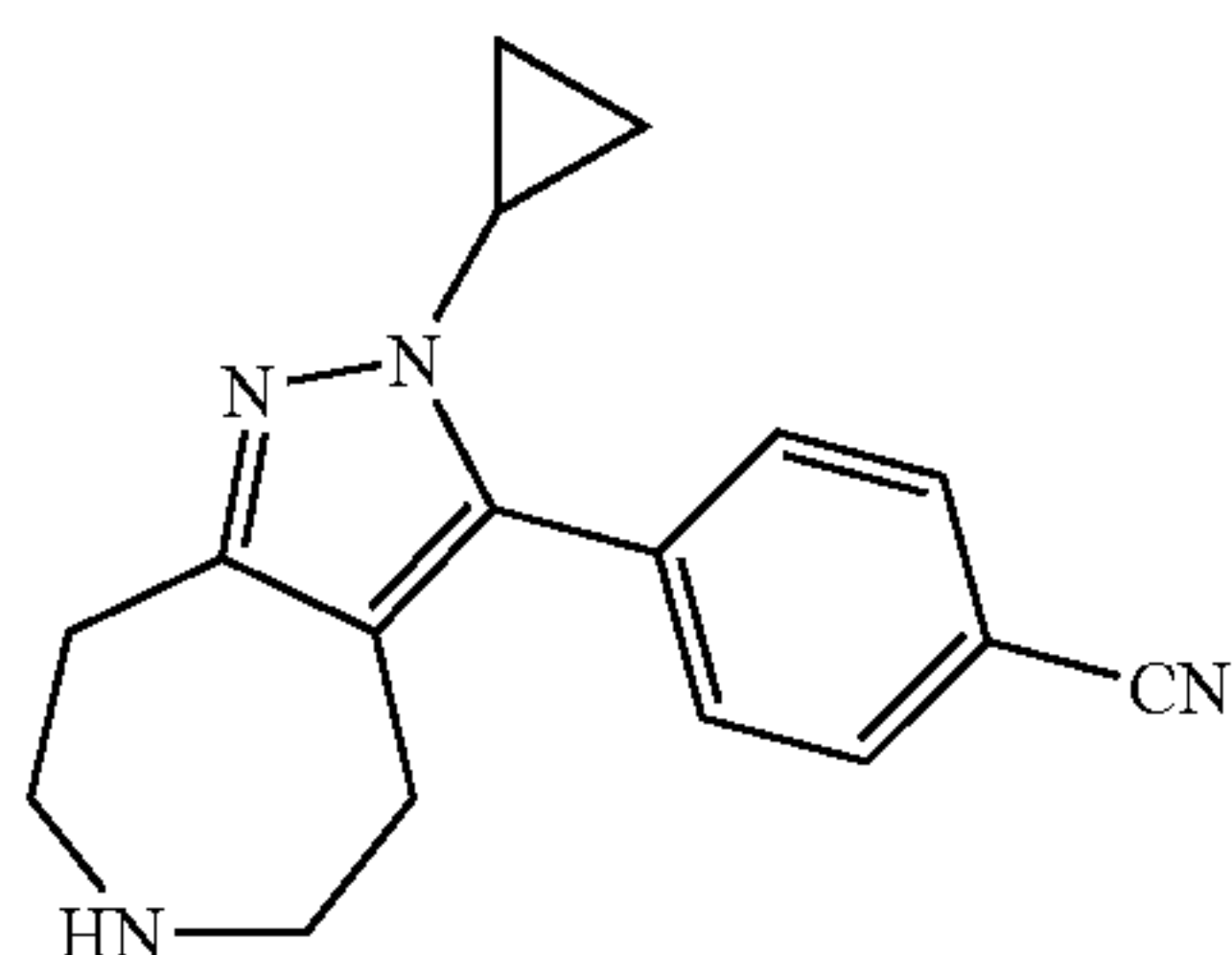
4-(2-Cyclopropyl-2,4,5,6,7,8-hexahydro-1,2,6-triazazulen-3-yl)-benzonitrile
