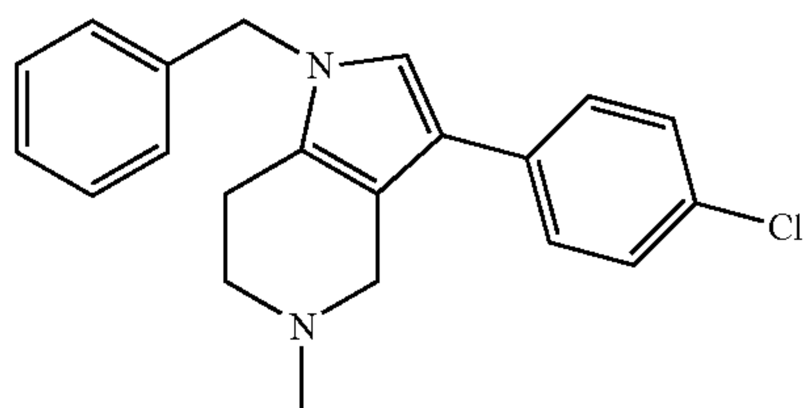
1-Benzyl-3-(4-chloro-phenyl)-5-methyl-4,5,6,7-tetrahydro-1H-pyrrolo[3,2-c]pyridine
