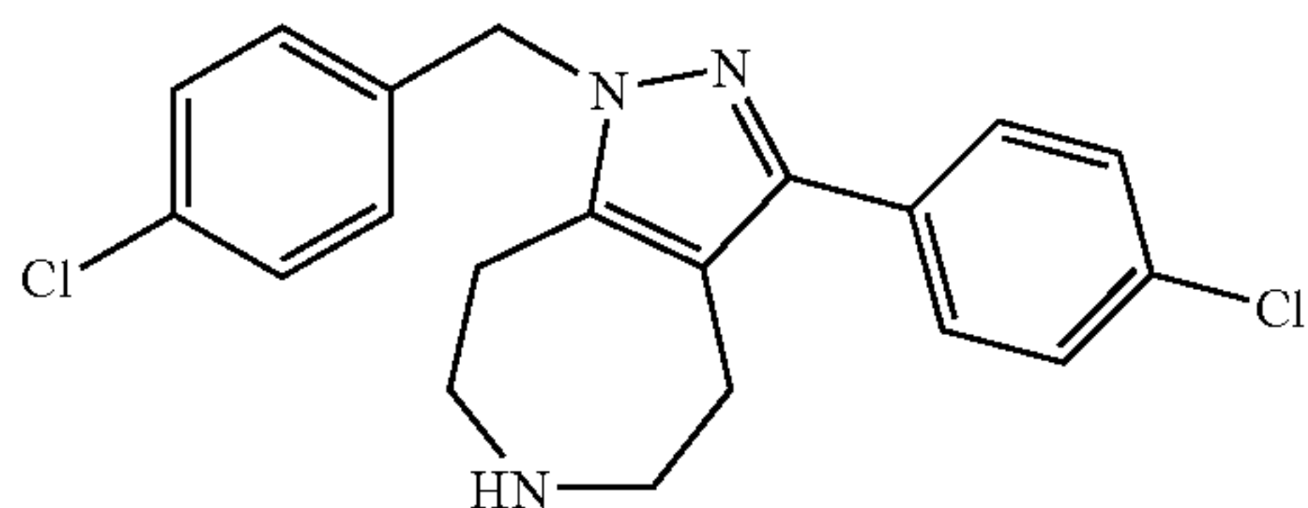
1-(4-Chloro-benzyl)-3-(4-chloro-phenyl)-1,4,5,6,7,8-hexahydro-1,2,6-triaza-azulene
