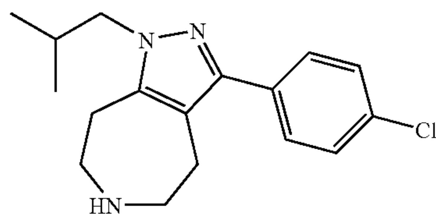
3-(4-Chloro-phenyl)-1-isobutyl-1,4,5,6,7,8-hexahydro-1,2,6-triaza-azulene
