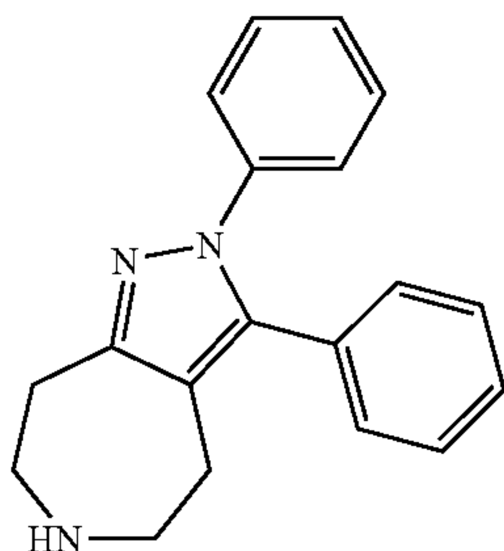
2,3-Diphenyl-2,4,5,6,7,8-hexahydro-1,2,6-triaza-azulene
