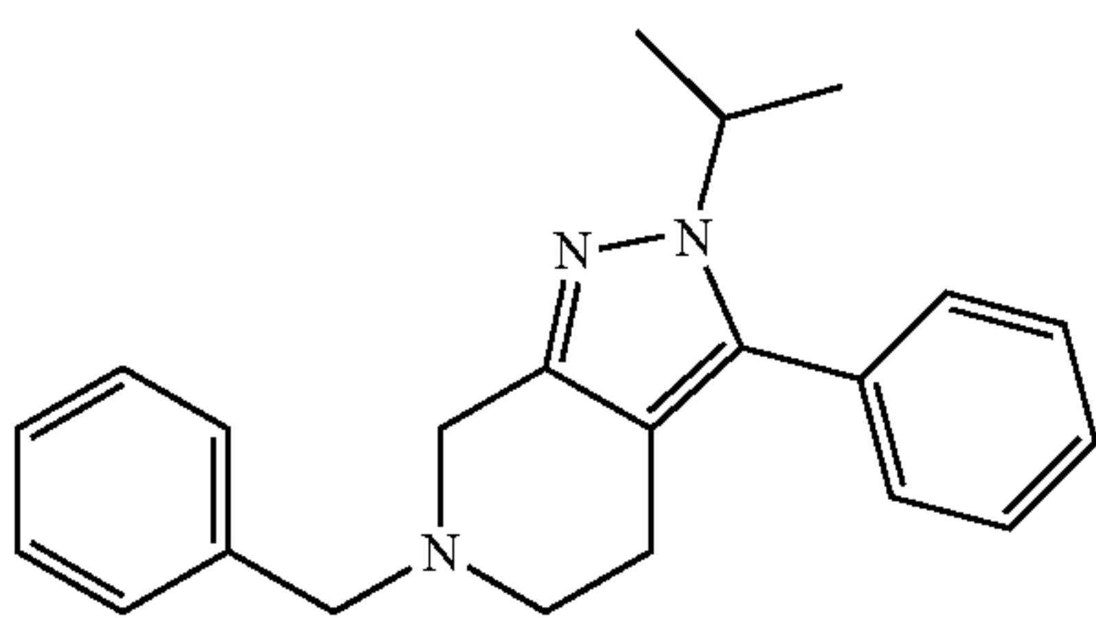
6-Benzyl-2-isopropyl-3-phenyl-4,5,6,7-tetrahydro-2H-pyrazolo[3,4-c]pyridine
