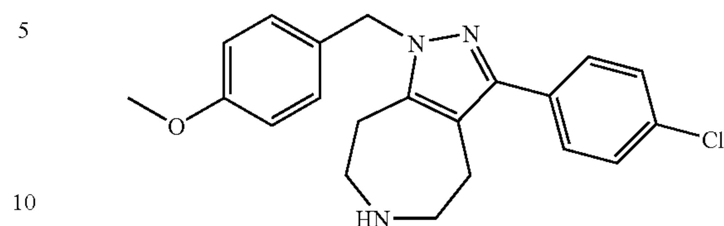
3-(4-Chloro-phenyl)-1-(4-methoxy-benzyl)-1,4,5,6,7,8-hexahydro-1,2,6-triaza-azulene
