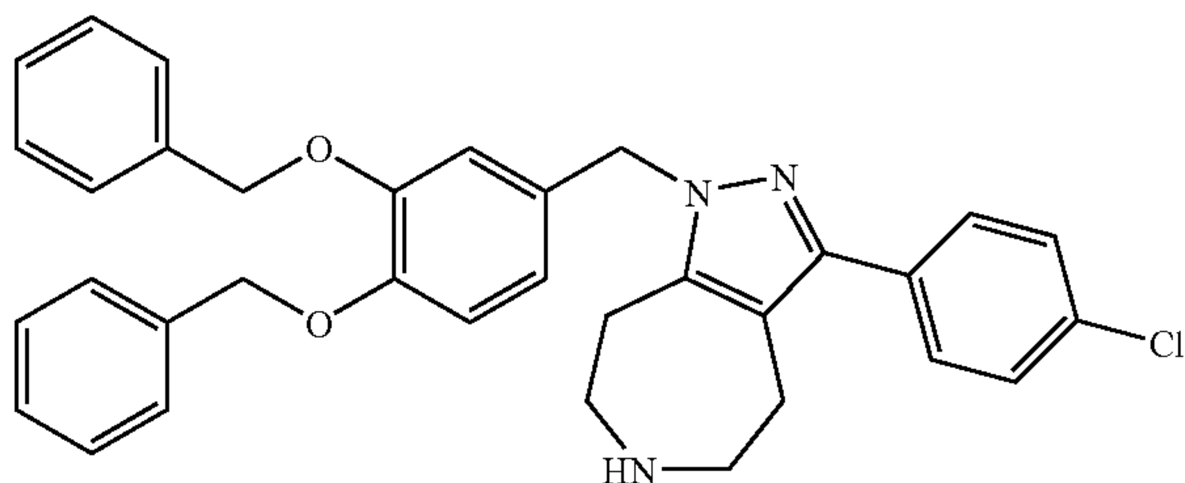
1-(3,4-Bis-benzyloxy-benzyl)-3-(4-chloro-phenyl)-1,4,5,6,7,8-hexahydro-1,2,6-triaza-azulene
