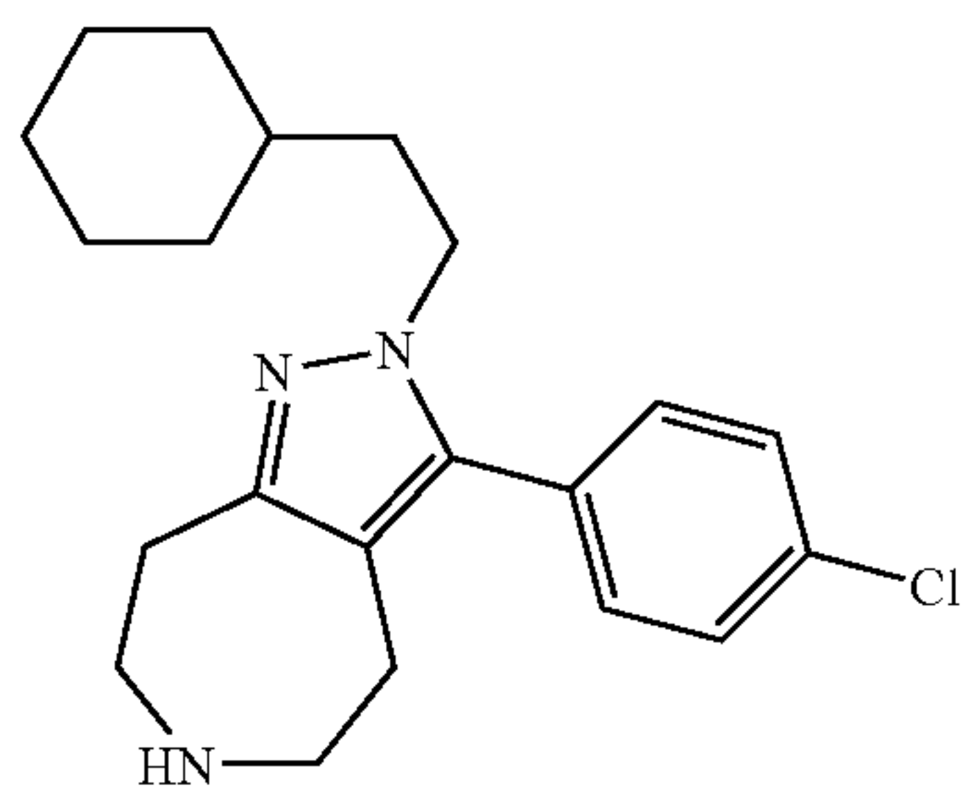
3-(4-Chloro-phenyl)-2-(2-cyclohexyl-ethyl)-2,4,5,6,7,8-hexahydro-1,2,6-triaza-azulene
