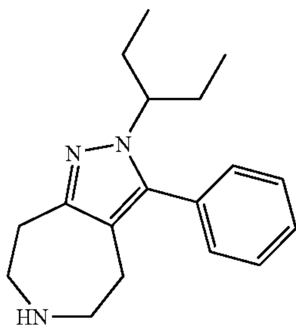
2-(1-Ethyl-propyl)-3-phenyl-2,4,5,6,7,8-hexahydro-1,2,6-triaza-azulene
