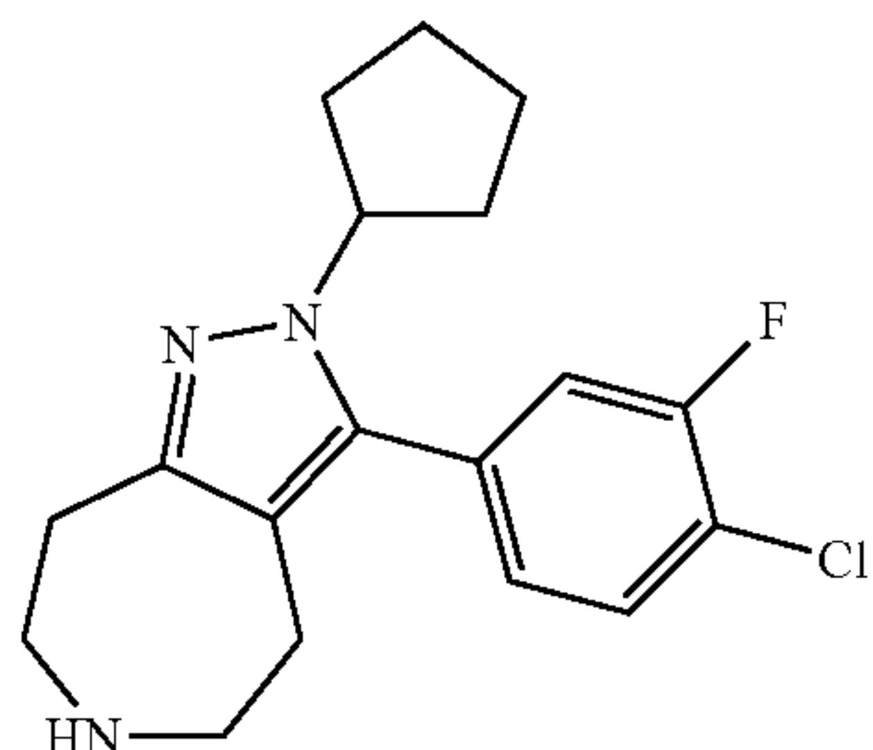
3-(4-Chloro-3-fluoro-phenyl)-2-cyclopentyl-2,4,5,6, 7,8-hexahydro-1,2,6-triaza-azulene
