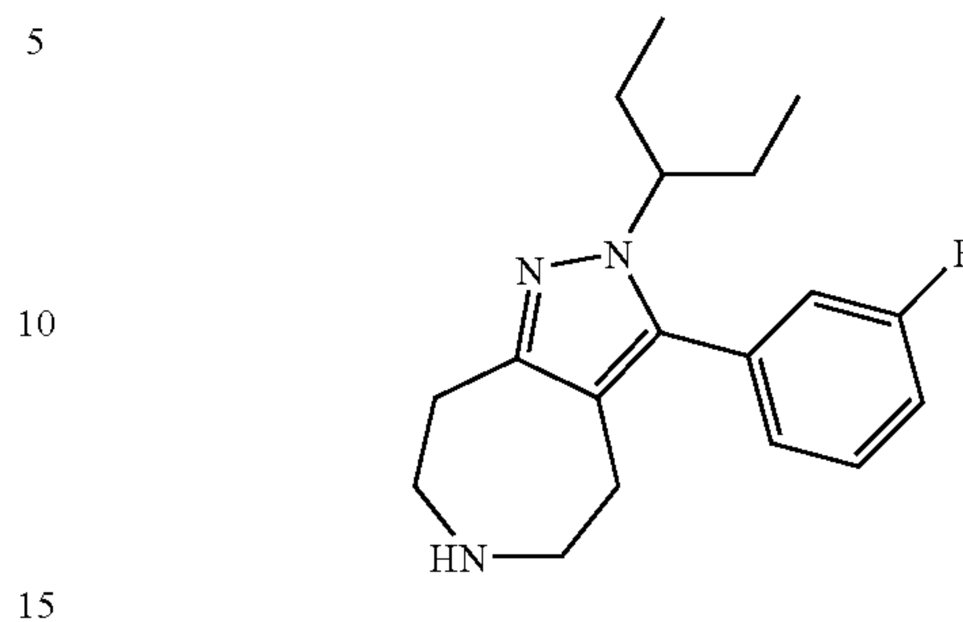
2-(1-Ethyl-propyl)-3-(3-fluoro-phenyl)-2,4,5,6,7,8-hexahydro-1,2,6-triaza-azulene
