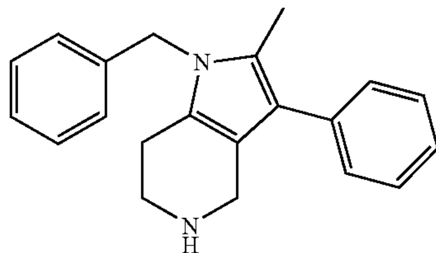
1-Benzyl-2-methyl-3-phenyl-4,5,6,7-tetrahydro-1H-pyrrolo[3,2-c]pyridine
