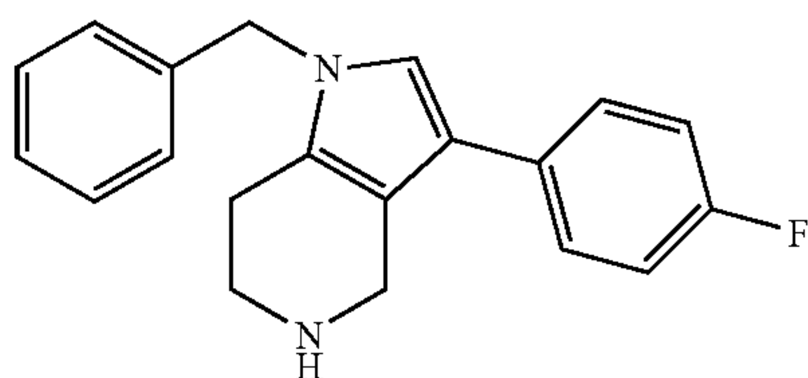
1-Benzyl-3-(4-fluoro-phenyl)-4,5,6,7-tetrahydro-1H-pyrrolo[3,2-c]pyridine
