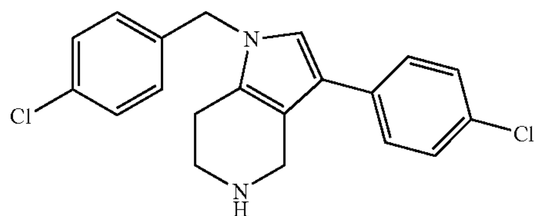
1-(4-Chloro-benzyl)-3-(4-chloro-phenyl)-4,5,6,7-tetrahydro-1H-pyrrolo[3,2-c]pyridine
