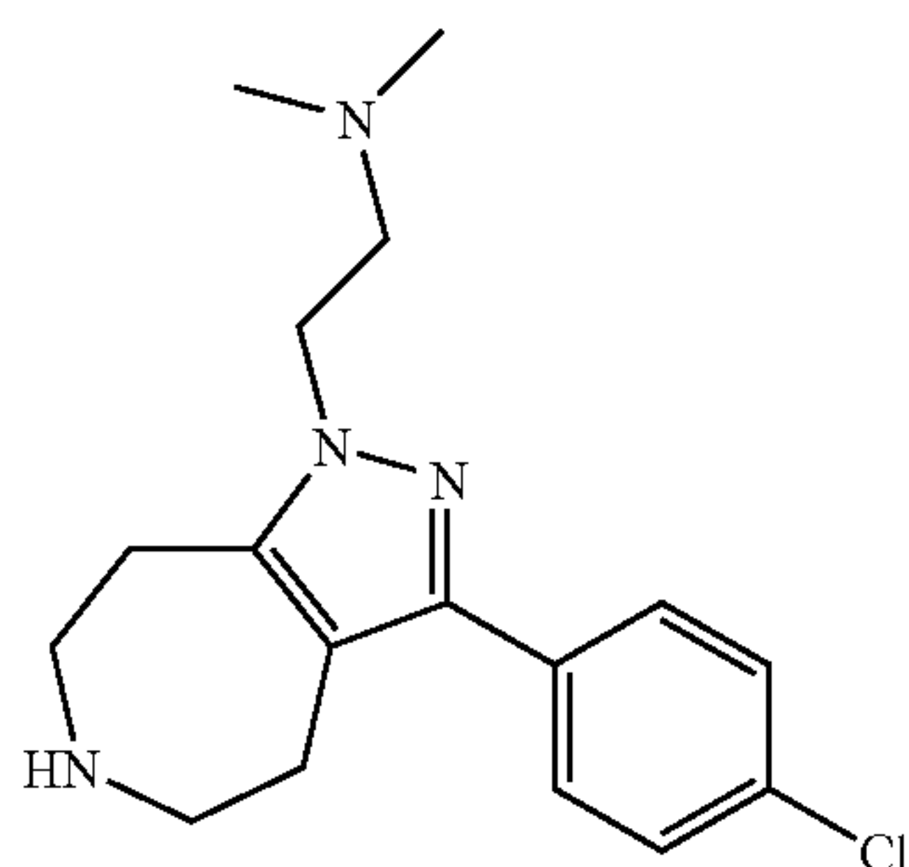
{2-[3-(4-Chloro-phenyl)-5,6,7,8-tetrahydro-4H-1,2,6-triaza-azulen-1-yl]-ethyl}-dimethyl-amine
