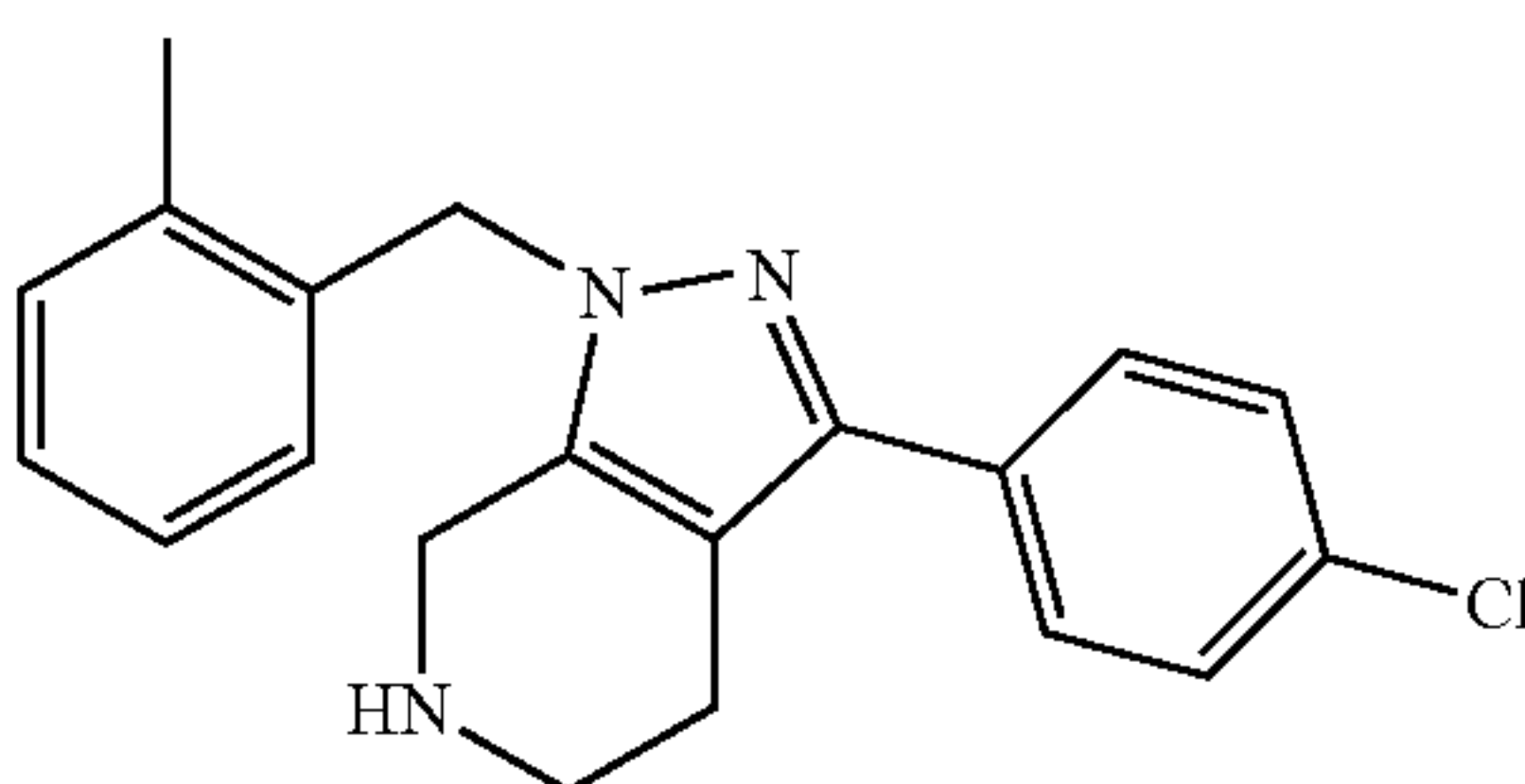
3-(4-Chloro-phenyl)-1-(2-methyl-benzyl)-4,5,6,7-tetrahydro-1H-pyrazolo[3,4-c]pyridine
