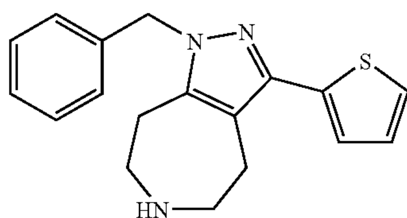
1-Benzyl-3-thiophen-2-yl-1,4,5,6,7,8-hexahydro-1,2,6-triaza-azulene
