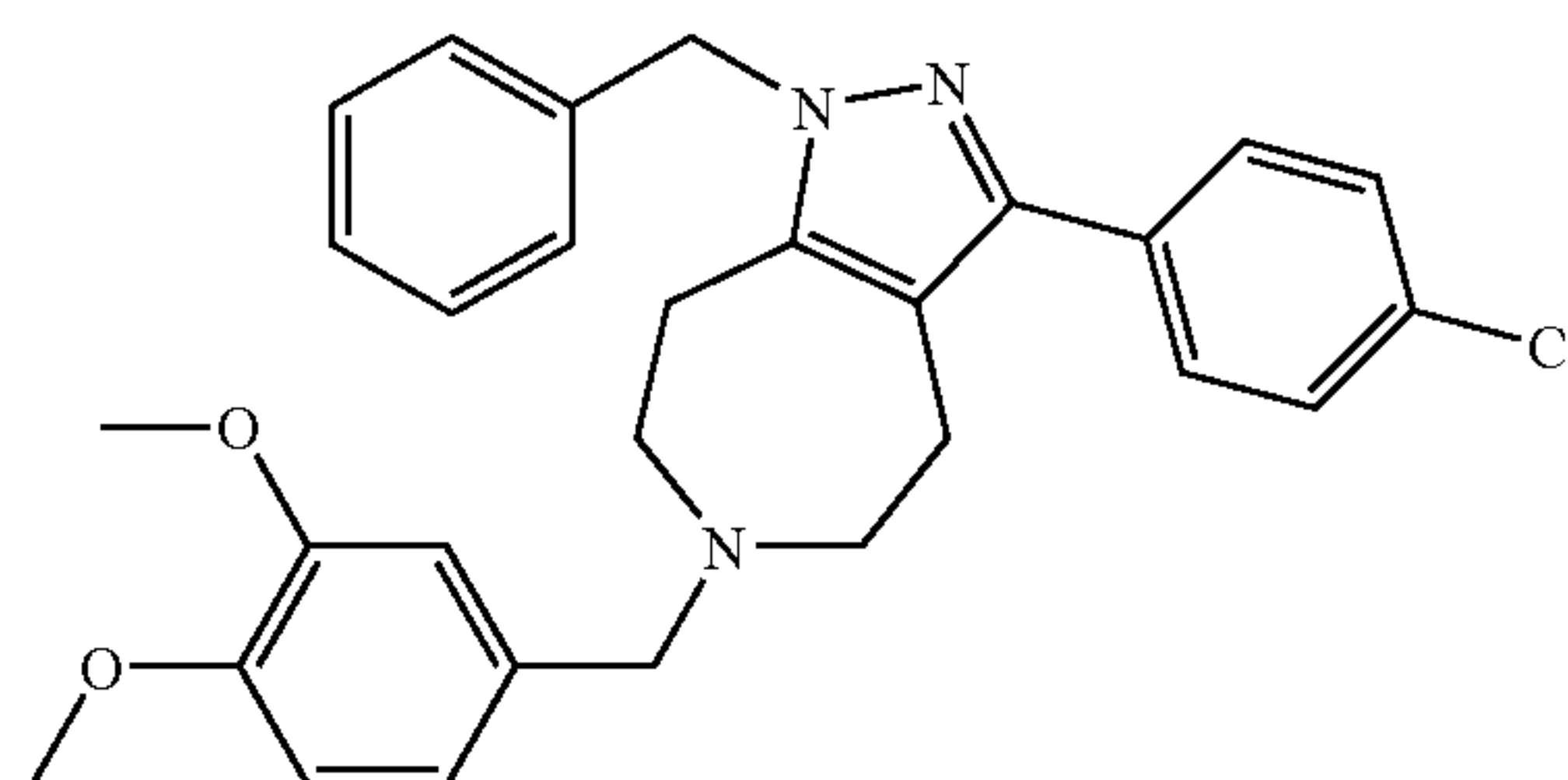
1-Benzyl-3-(4-chloro-phenyl)-6-(3,4-dimethoxy-benzyl)-1,4,5,6,7,8-hexahydro-1,2,6-triaza-azulene
