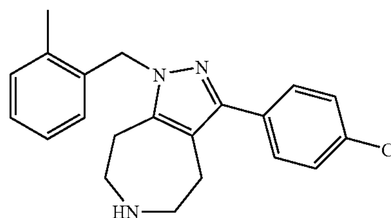
3-(4-Chloro-phenyl)-1-(2-methyl-benzyl)-1,4,5,6,7,8-hexahydro-1,2,6-triaza-azulene
