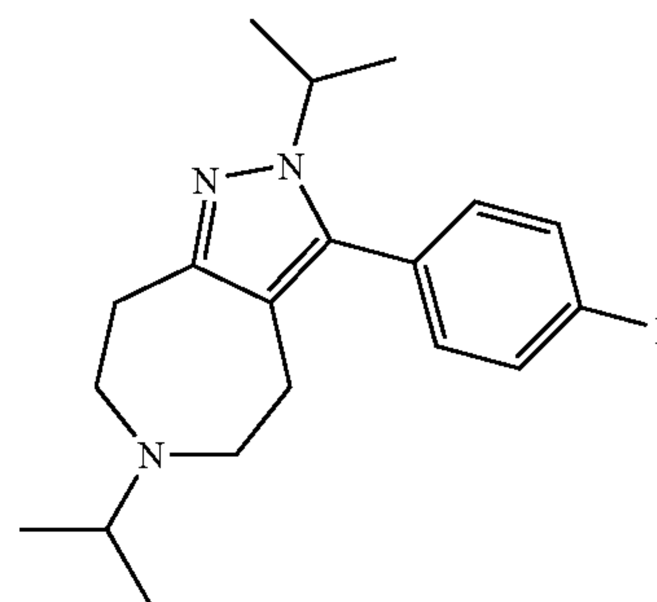
3-(4-Fluoro-phenyl)-2,6-diisopropyl-2,4,5,6,7,8-hexahydro-1,2,6-triaza-azulene
