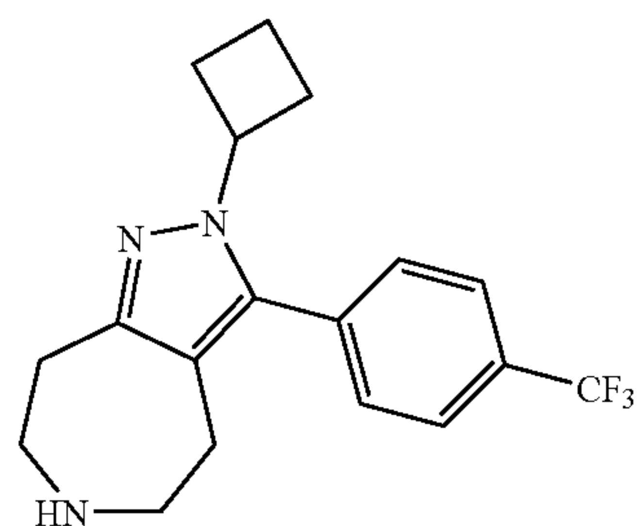
2-Cyclobutyl-3-(4-trifluoromethyl-phenyl)-2,4,5,6,7,8-hexahydro-1,2,6-triaza-azulene
