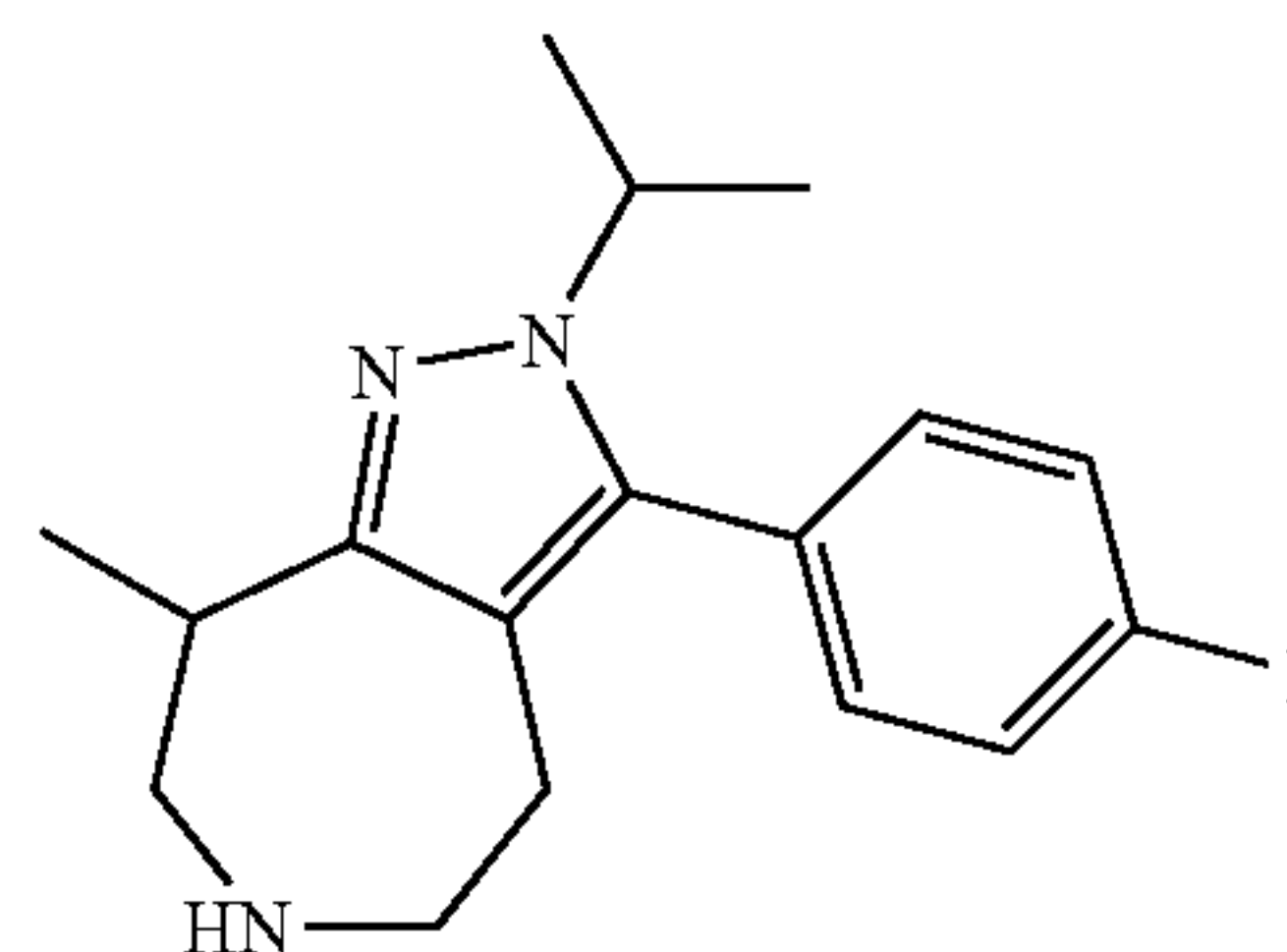
3-(4-Fluoro-phenyl)-2-isopropyl-8-methyl-2,4,5,6,7, 8-hexahydro-1,2,6-triaza-azulene
