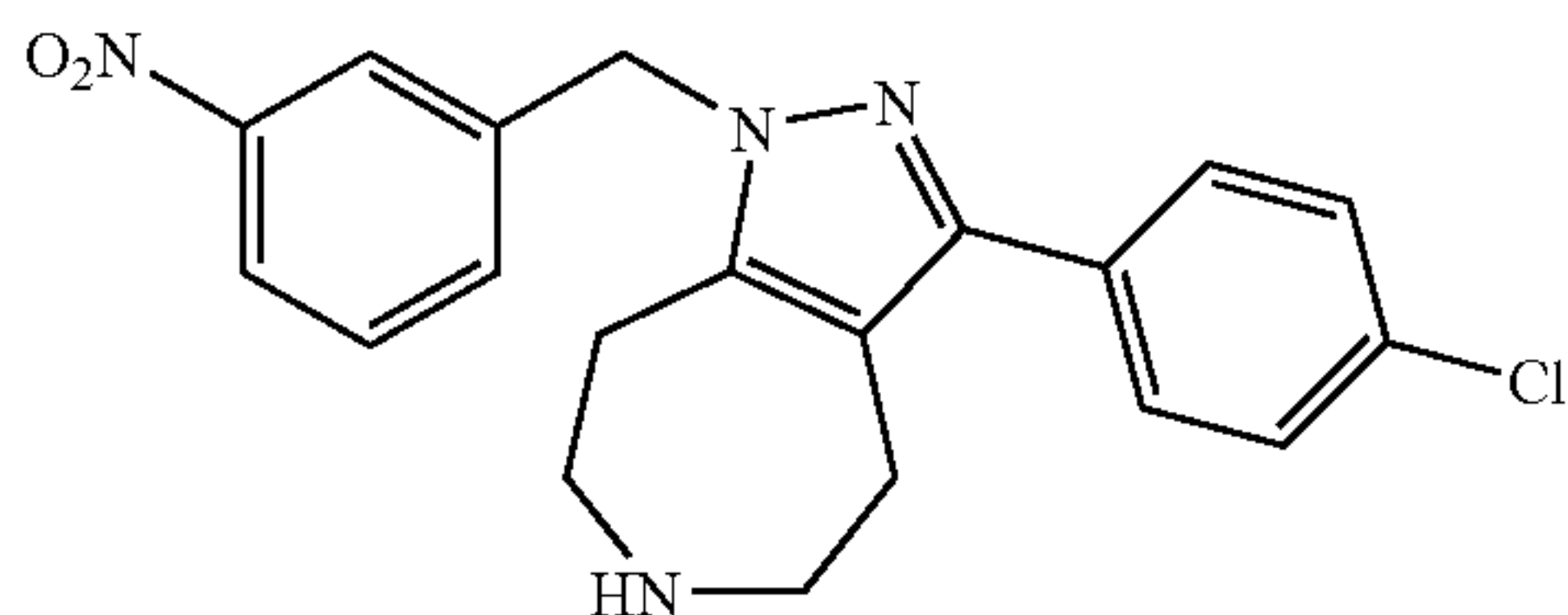
3-(4-Chloro-phenyl)-1-(3-nitro-benzyl)-1,4,5,6,7,8- hexahydro-1,2,6-triaza-azulene
