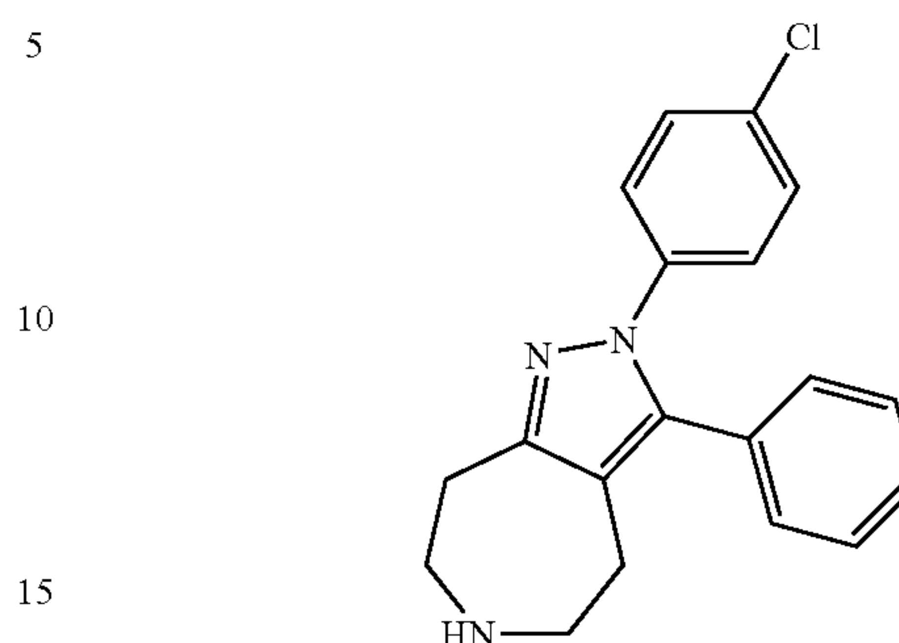
2-(4-Chloro-phenyl)-3-phenyl-2,4,5,6,7,8-hexahydro-1,2,6-triaza-azulene
