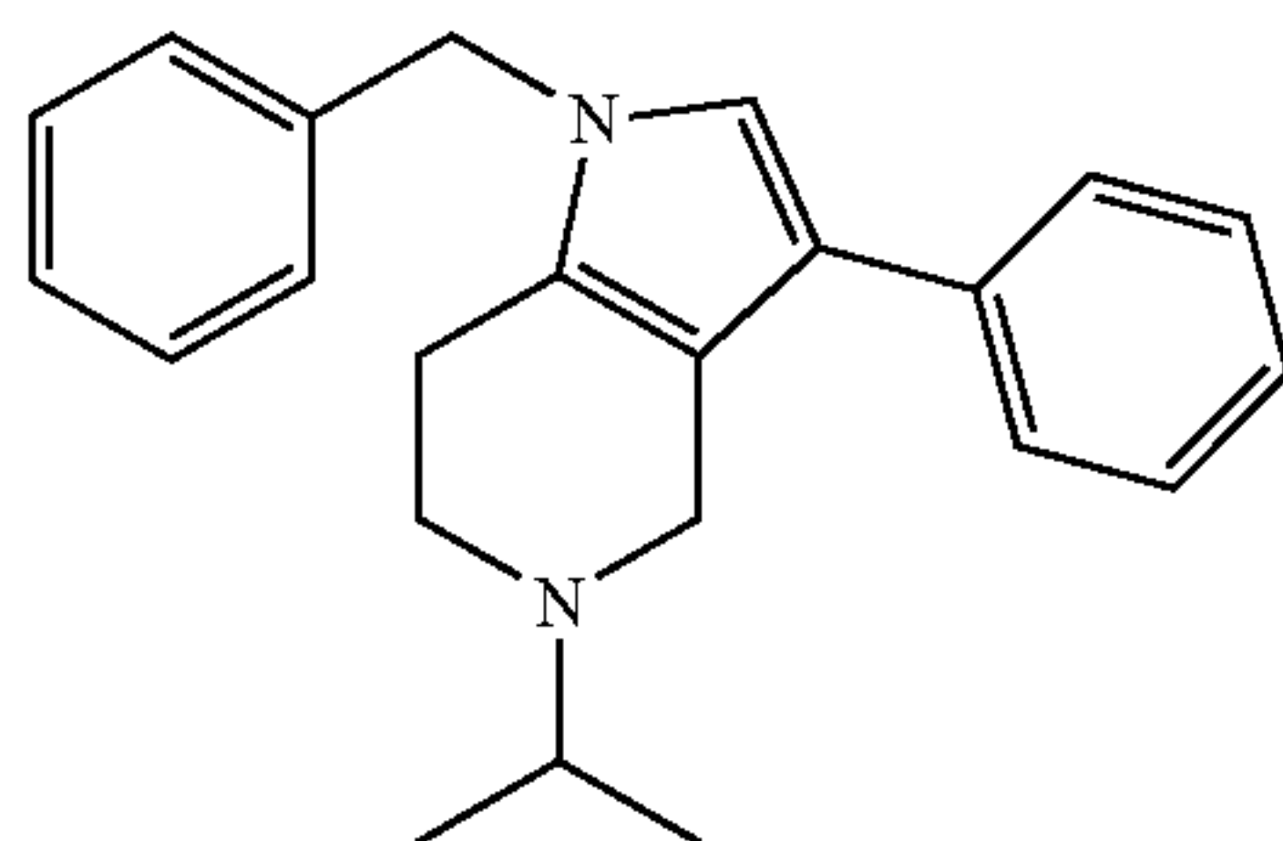
1-Benzyl-5-isopropyl-3-phenyl-4,5,6,7-tetrahydro-1H-pyrrolo[3,2-c]pyridine
