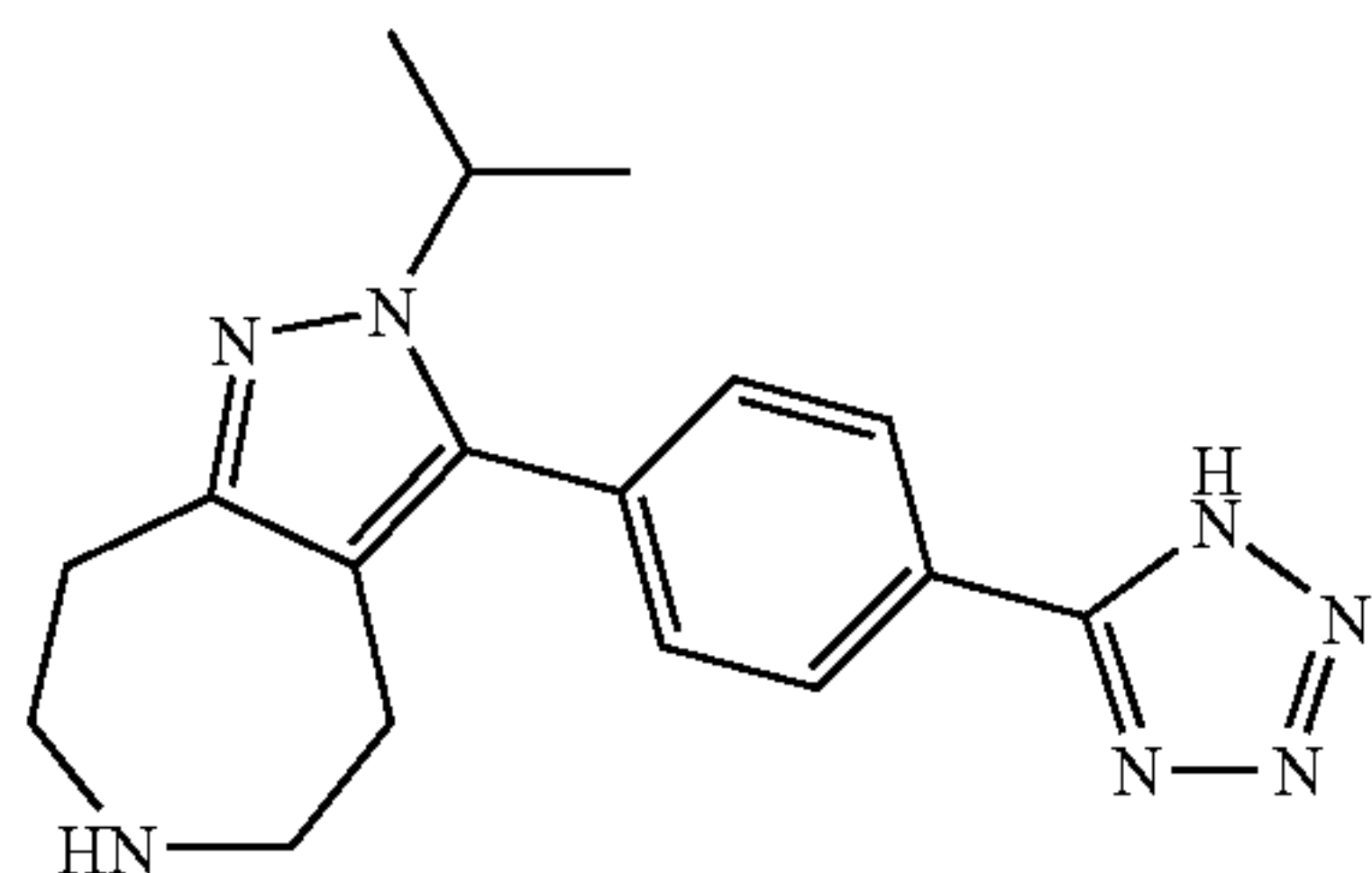
2-Isopropyl-3-[4-(1H-tetrazol-5-yl)-phenyl]-2,4,5,6, 7,8-hexahydro-1,2,6-triaza-azulene
