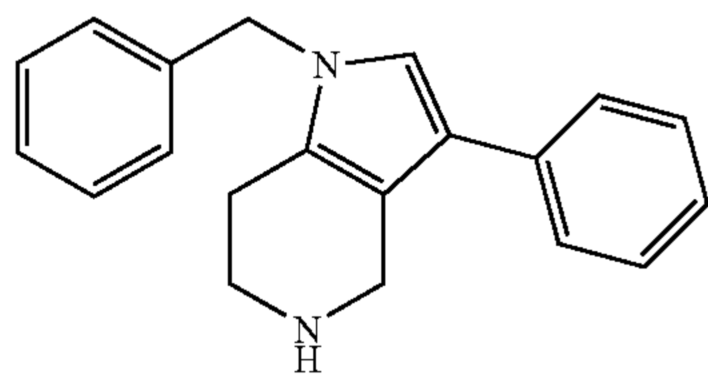
1-Benzyl-3-phenyl-4,5,6,7-tetrahydro-1H-pyrrolo[3,2-c]pyridine
