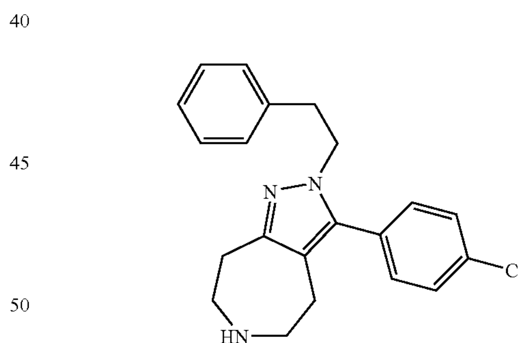
3-(4-Chloro-phenyl)-2-phenethyl-2,4,5,6,7,8-hexahydro-1,2,6-triaza-azulene
