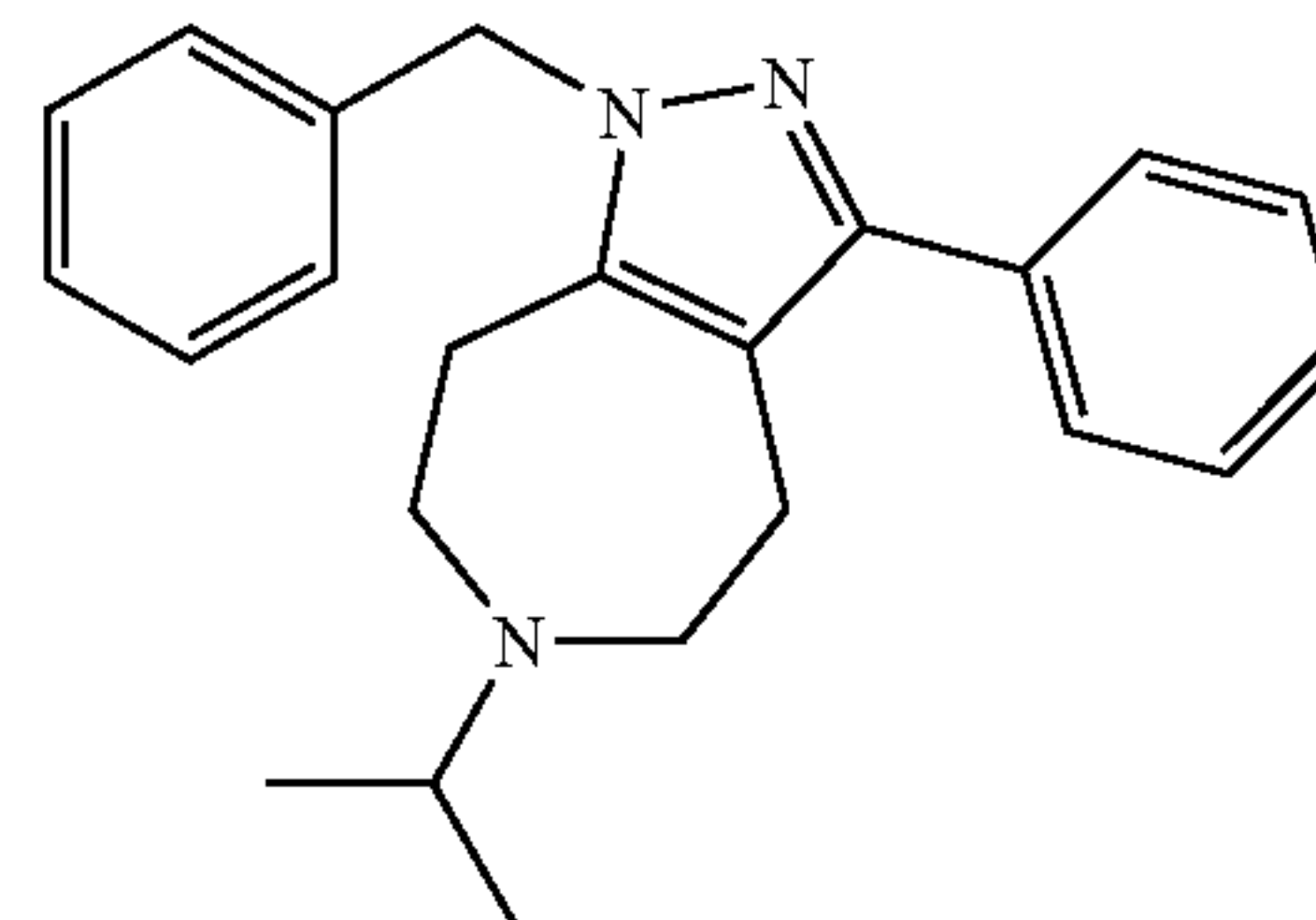
1-Benzyl-6-isopropyl-3-phenyl-1,4,5,6,7,8-hexahydro-1,2,6-triaza-azulene
