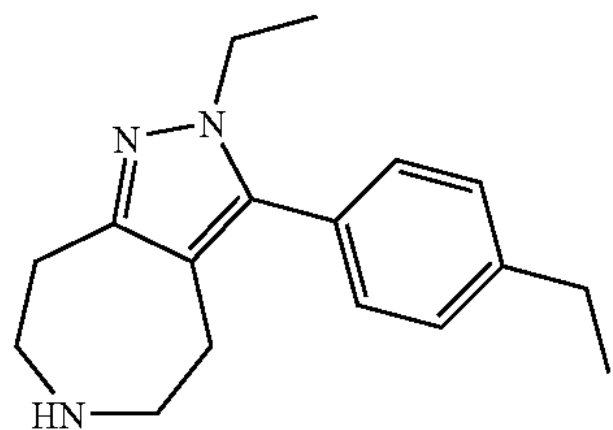
2-Ethyl-3-(4-ethyl-phenyl)-2,4,5,6,7,8-hexahydro-1,2,6-triaza-azulene
