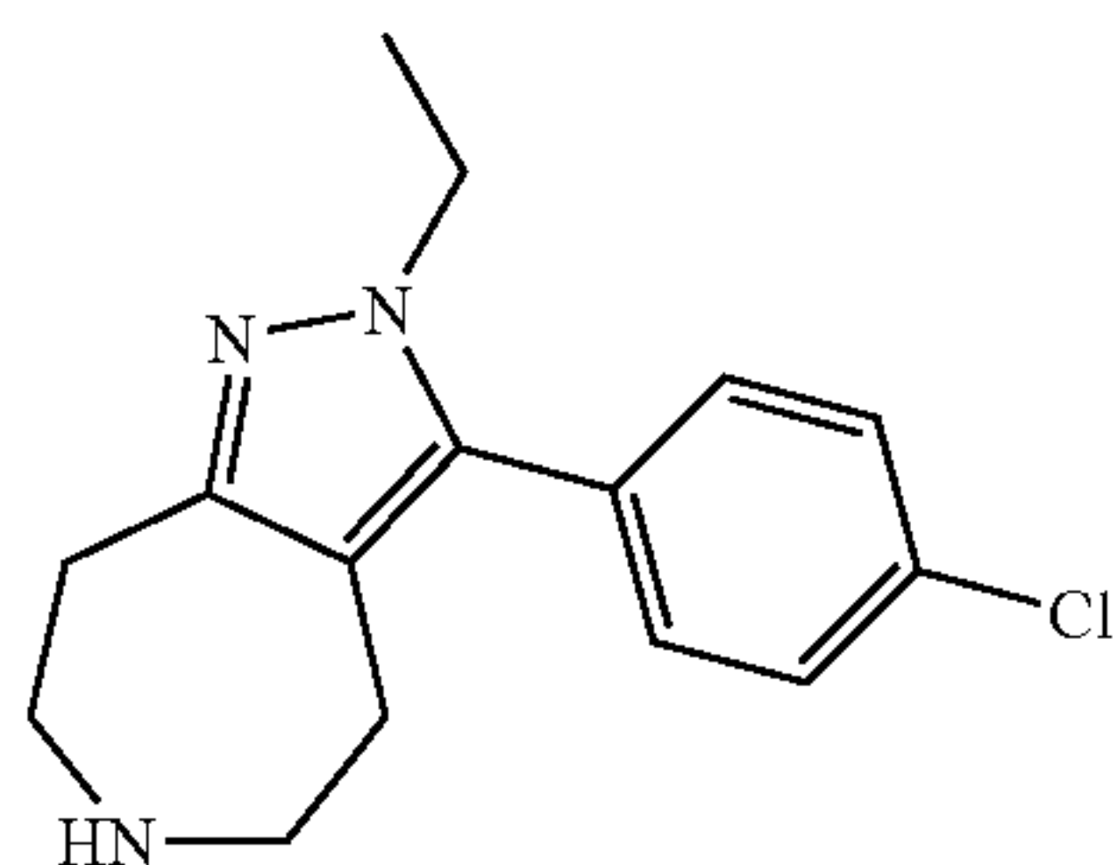
3-(4-Chloro-phenyl)-2-ethyl-2,4,5,6,7,8-hexahydro-1,2,6-triaza-azulene
