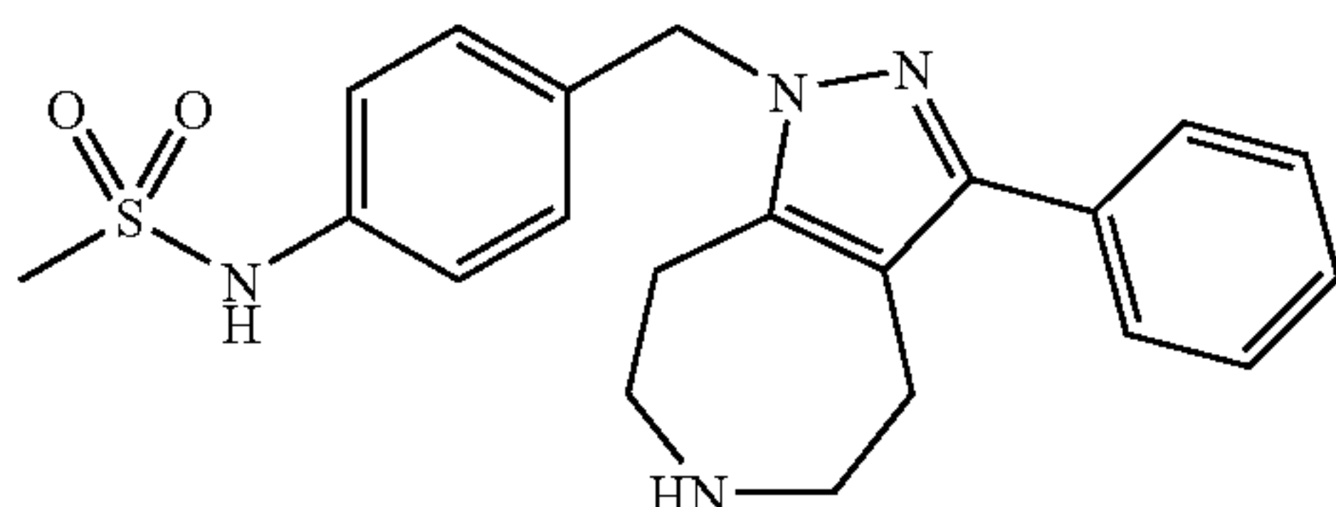
N-[4-(3-Phenyl-5,6,7,8-tetrahydro-4H-1,2,6-triaza-azulen-1-ylmethyl)-phenyl]-methanesulfonamide
