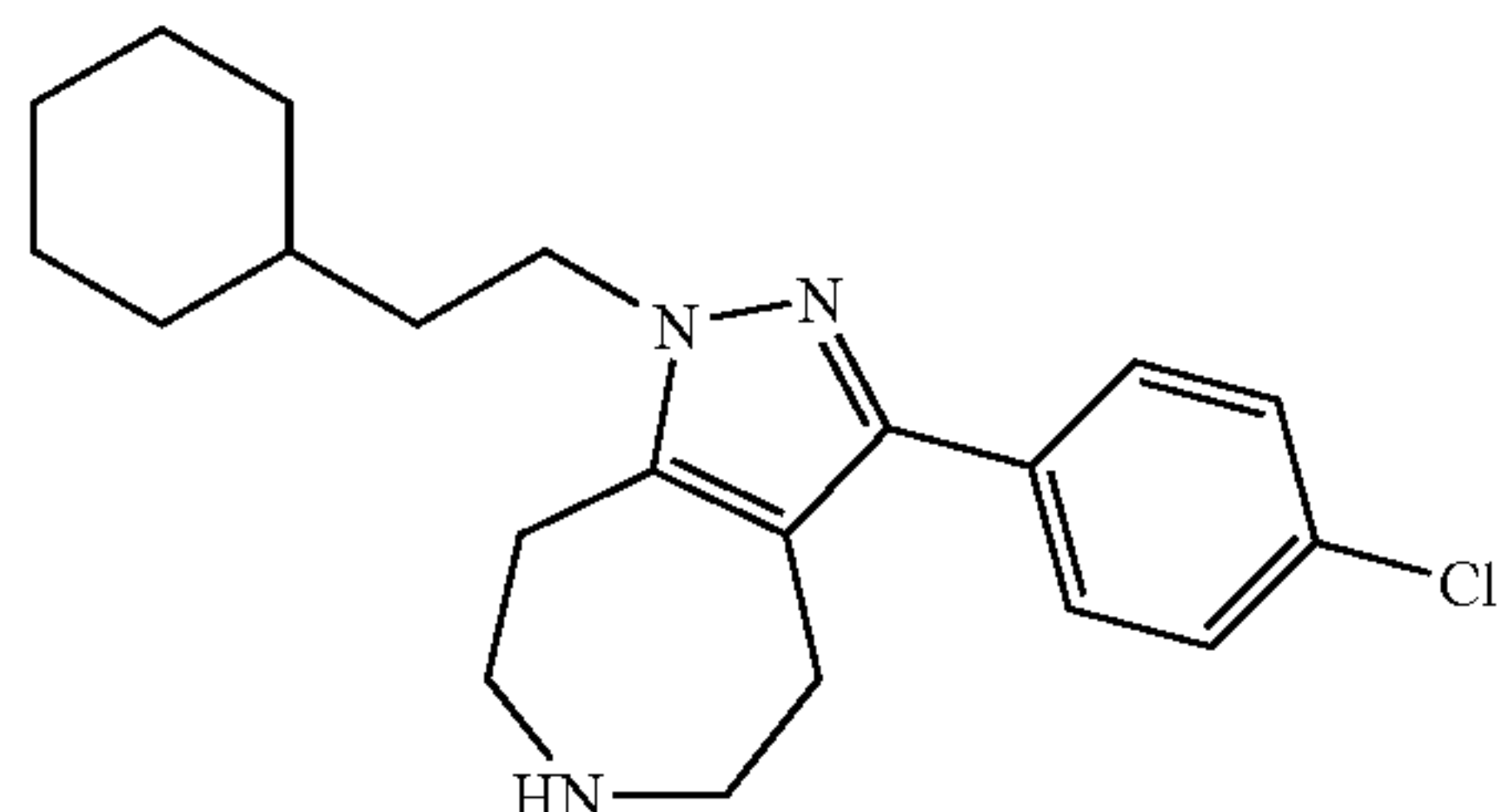
3-(4-Chloro-phenyl)-1-(2-cyclohexyl-ethyl)-1,4,5,6,7,8-hexahydro-1,2,6-triaza-azulene
