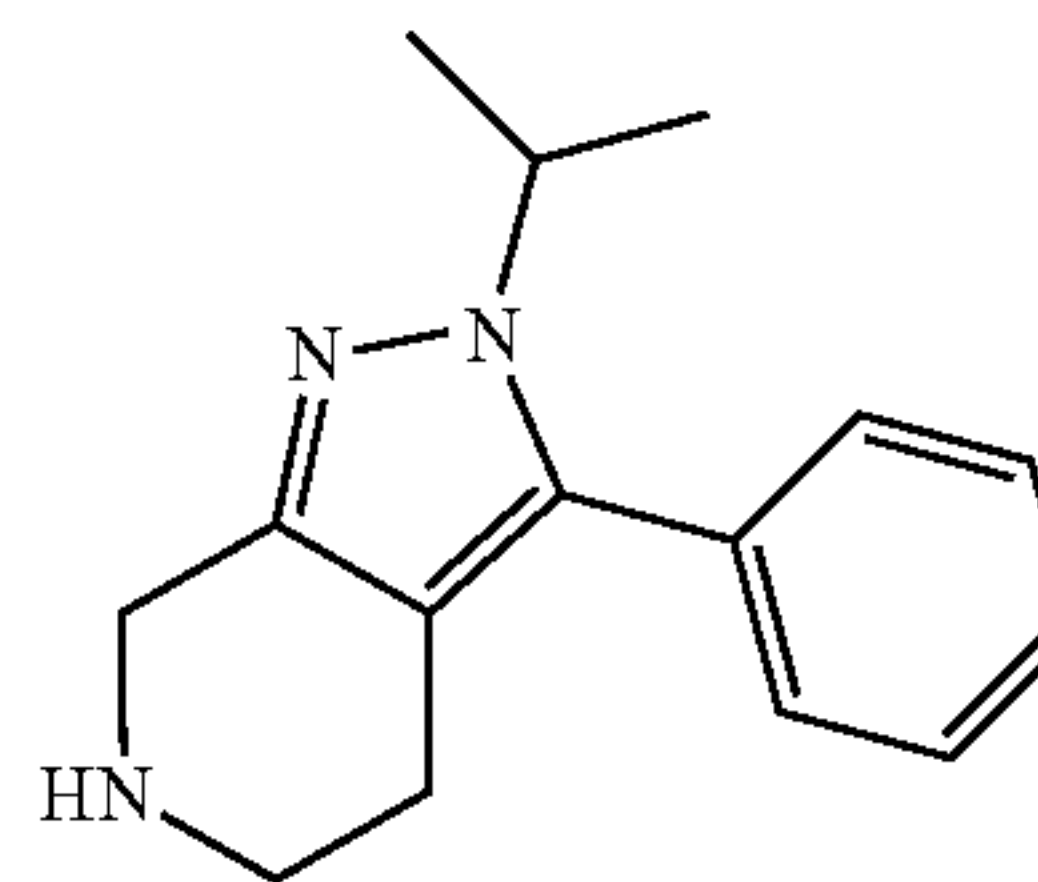
2-Isopropyl-3-phenyl-4,5,6,7-tetrahydro-2H-pyrazolo[3,4-c]pyridine
