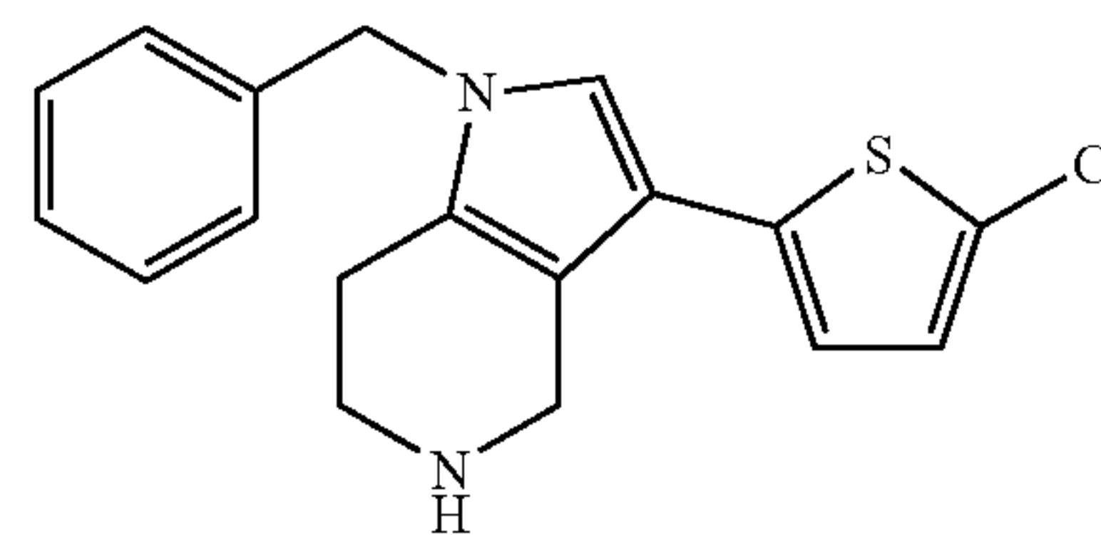
1-Benzyl-3-(5-chloro-thiophen-2-yl)-4,5,6,7-tetrahydro-1H-pyrrolo[3,2-c]pyridine
