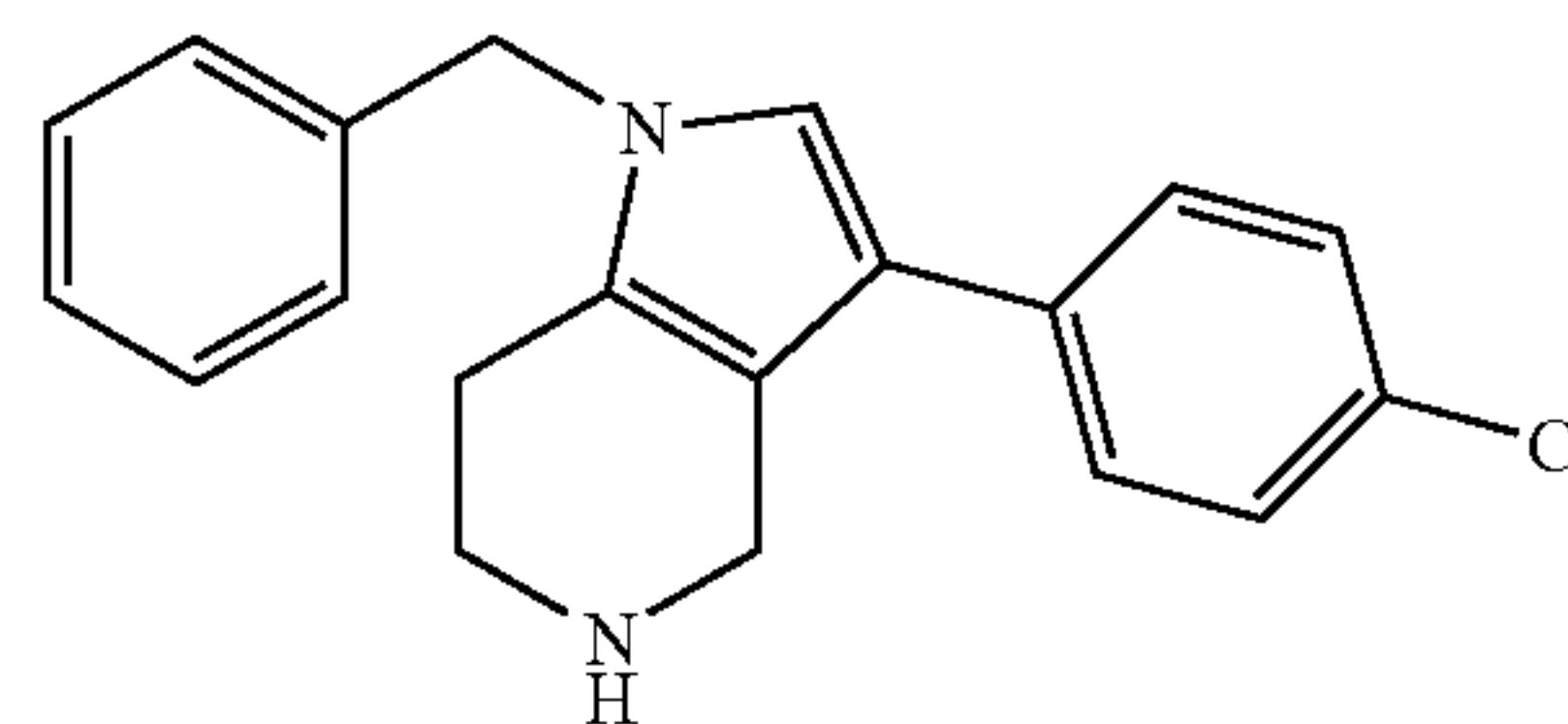
1-Benzyl-3-(4-chloro-phenyl)-4,5,6,7-tetrahydro-1H-pyrrolo[3,2-c]pyridine
