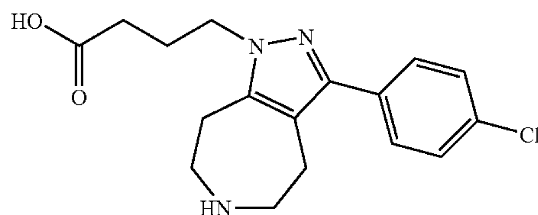
4-[3-(4-Chloro-phenyl)-5,6,7,8-tetrahydro-4H-1,2,6-triaza-azulen-1-yl]-butyric Acid
