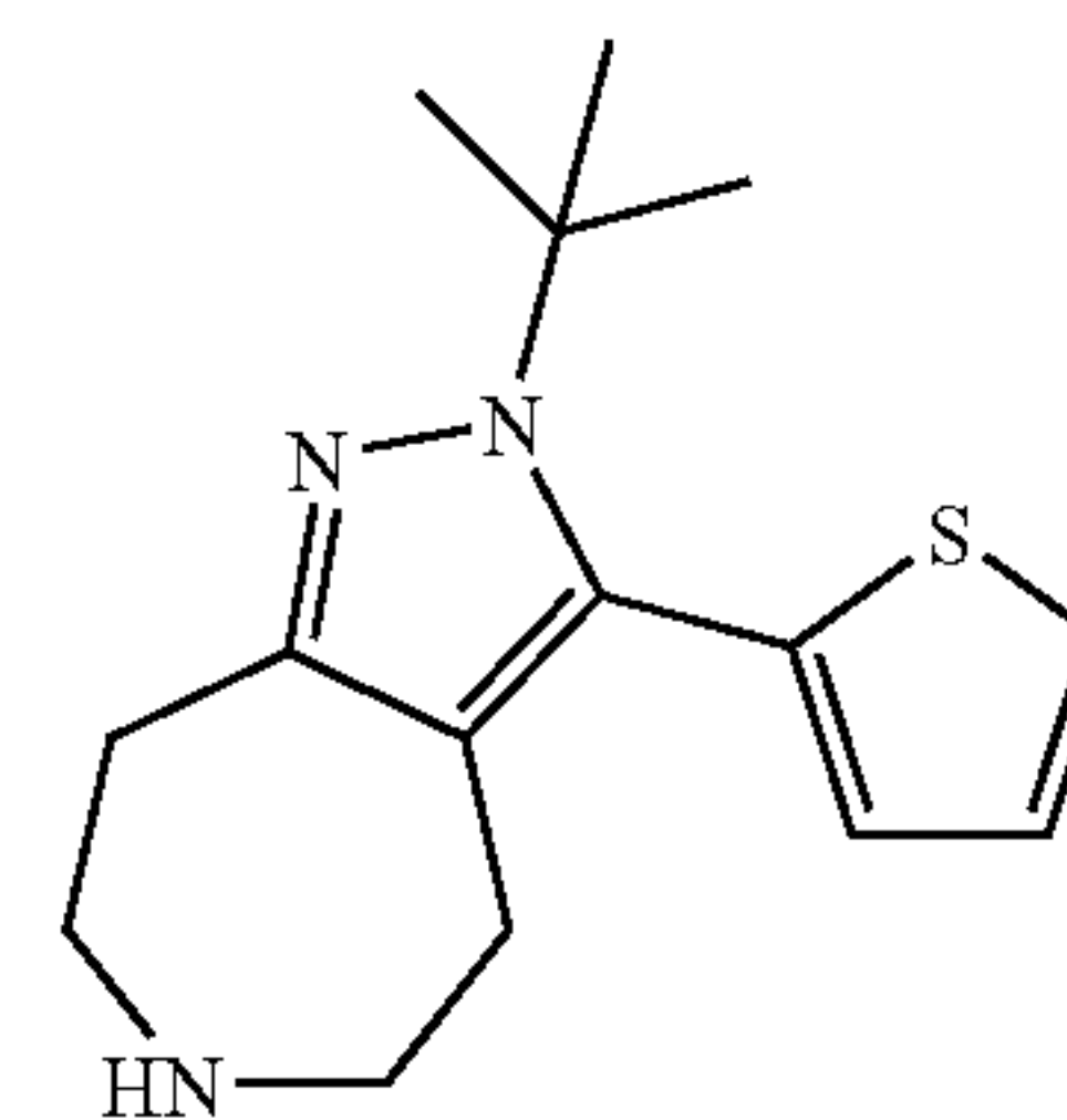
2-tert-Butyl-3-thiophen-2-yl-2,4,5,6,7,8-hexahydro-1,2,6-triaza-azulene
