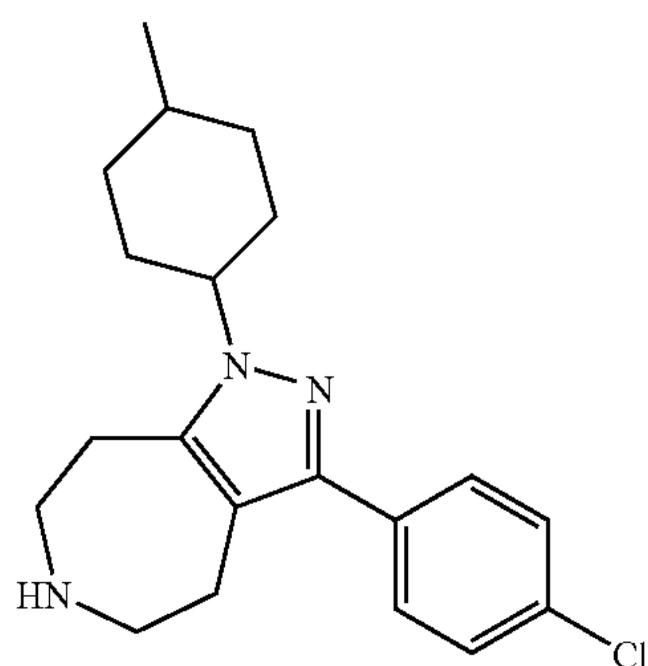
3-(4-Chloro-phenyl)-1-(4-methyl-cyclohexyl)-1,4,5,6,7,8-hexahydro-1,2,6-triaza-azulene
