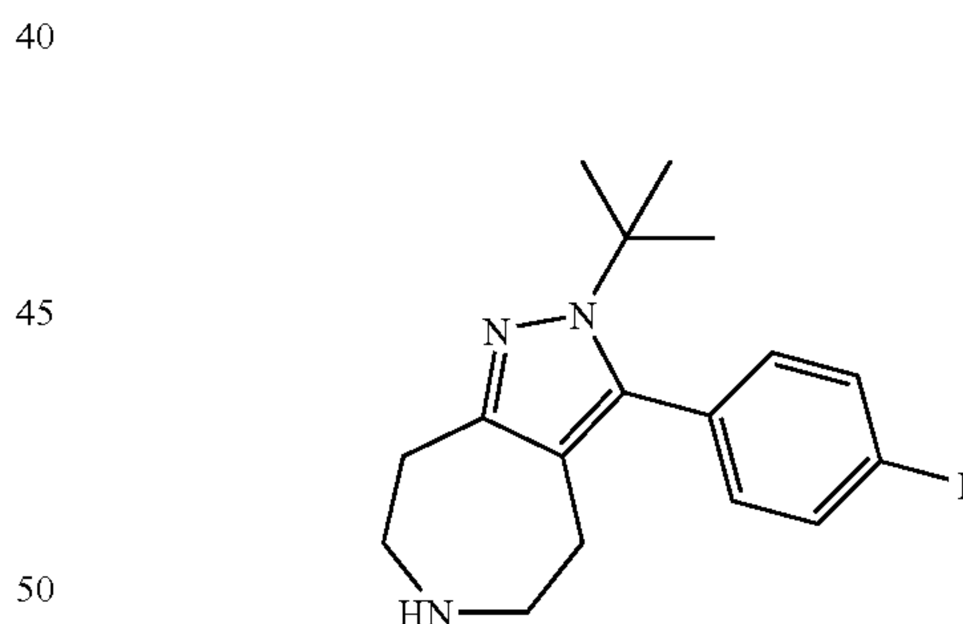
2-tert-Butyl-3-(4-fluorophenyl)-2,4,5,6,7,8-hexahydro-1,2,6-triaza-azulene
