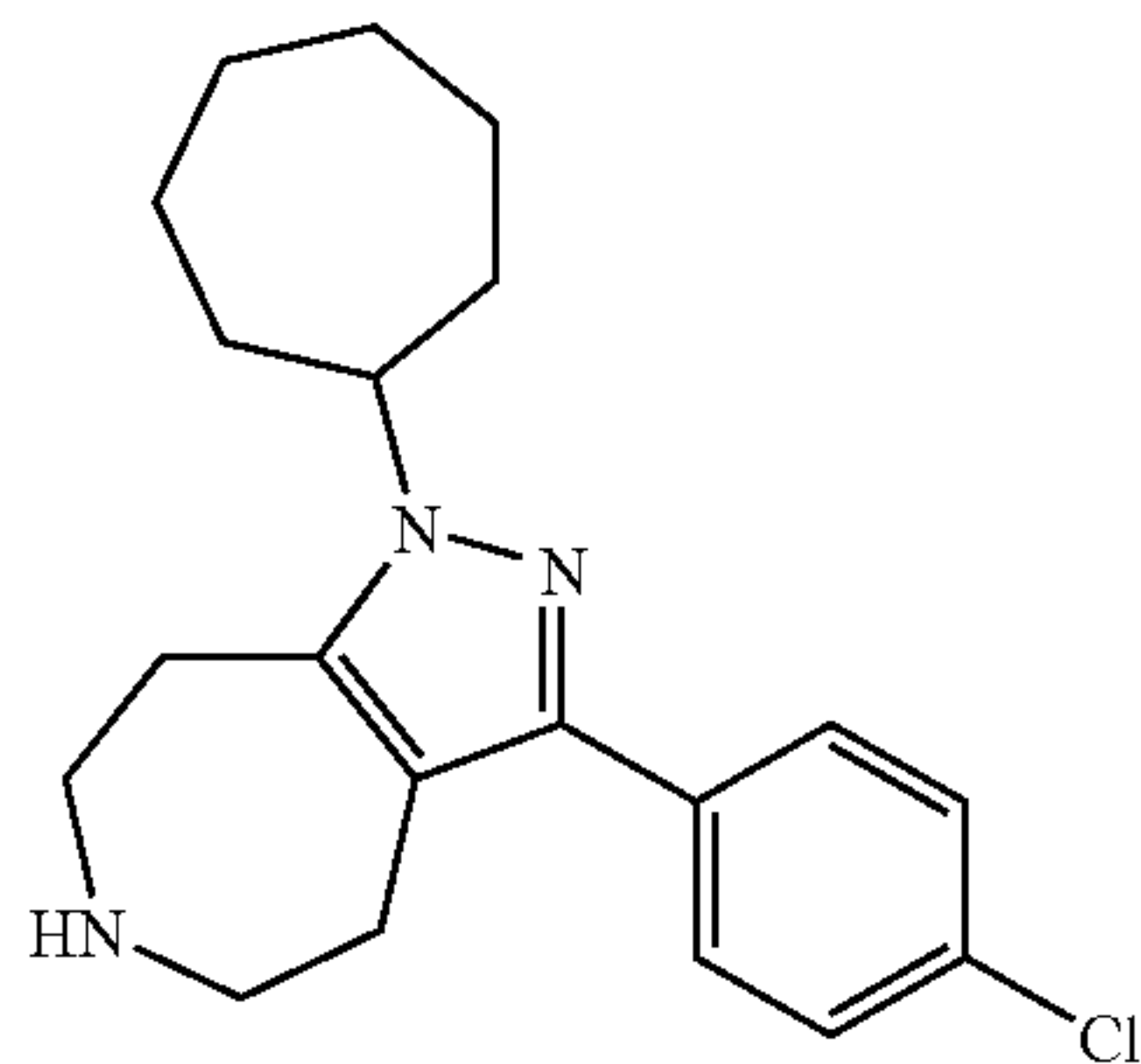
3-(4-Chloro-phenyl)-1-cycloheptyl-1,4,5,6,7,8-hexahydro-1,2,6-triaza-azulene
