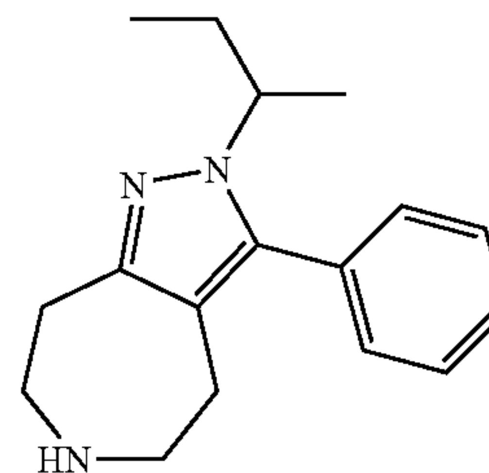
2-sec-Butyl-3-phenyl-2,4,5,6,7,8-hexahydro-1,2,6-triaza-azulene
