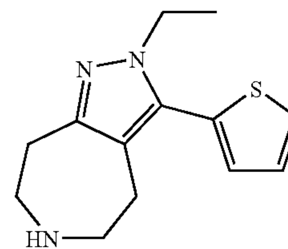
2-Ethyl-3-thiophen-2-yl-2,4,5,6,7,8-hexahydro-1,2,6-triaza-azulene
