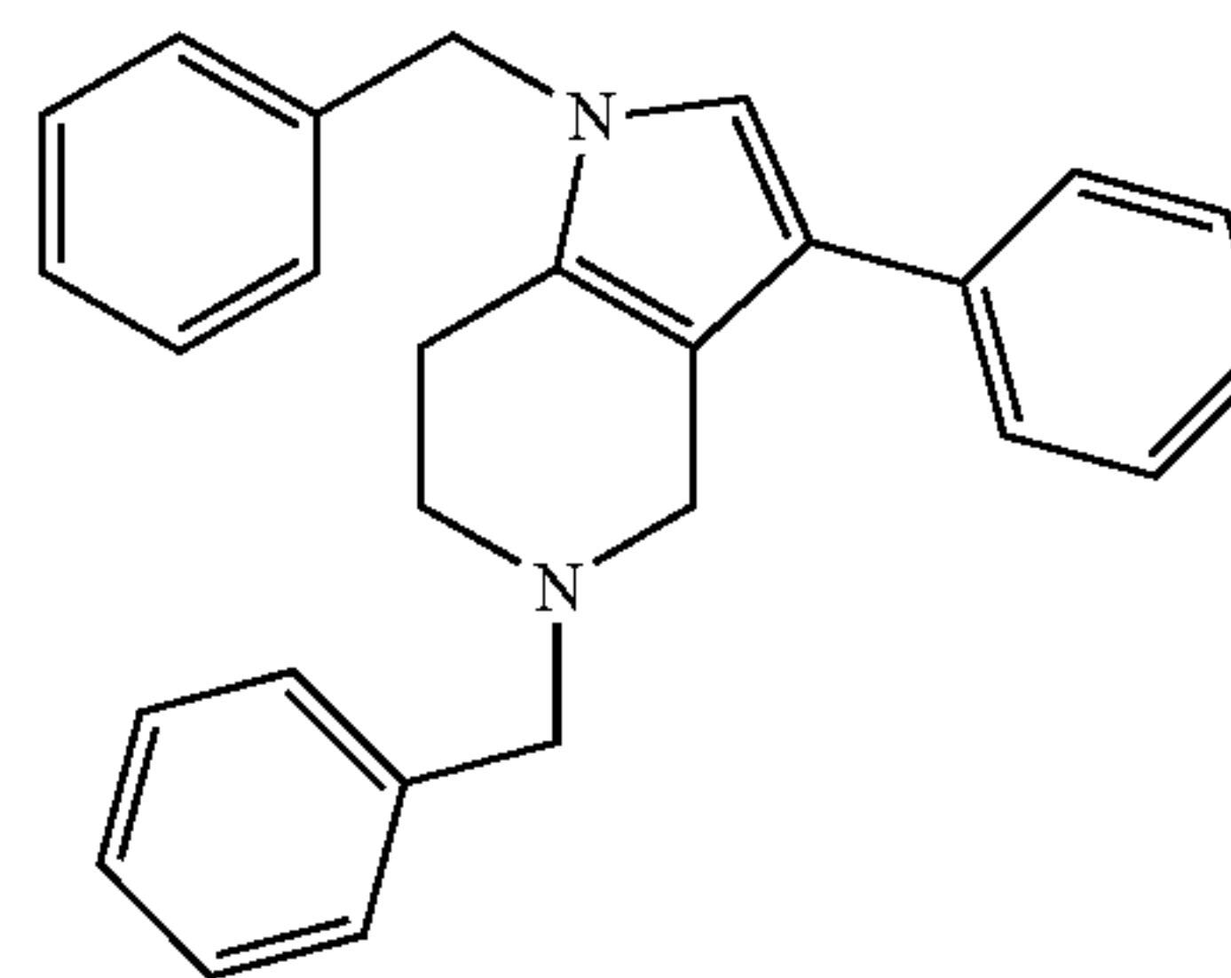
1,5-Dibenzyl-3-phenyl-4,5,6,7-tetrahydro-1H-pyrrolo[3,2-c]pyridine
