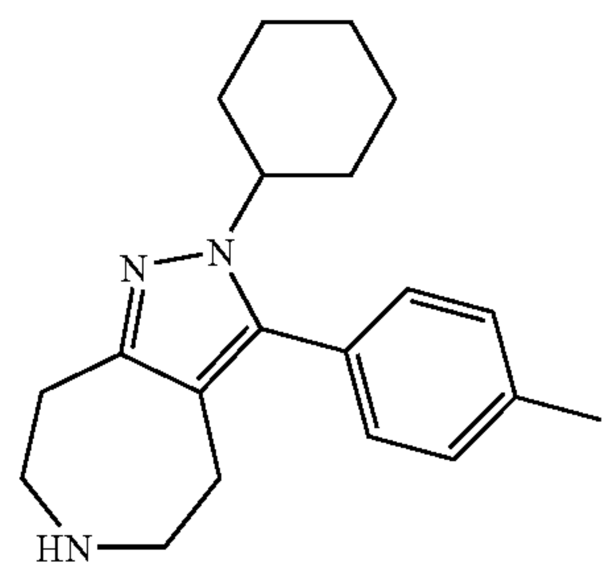
2-Cyclohexyl-3-p-tolyl-2,4,5,6,7,8-hexahydro-1,2,6-triaza-azulene
