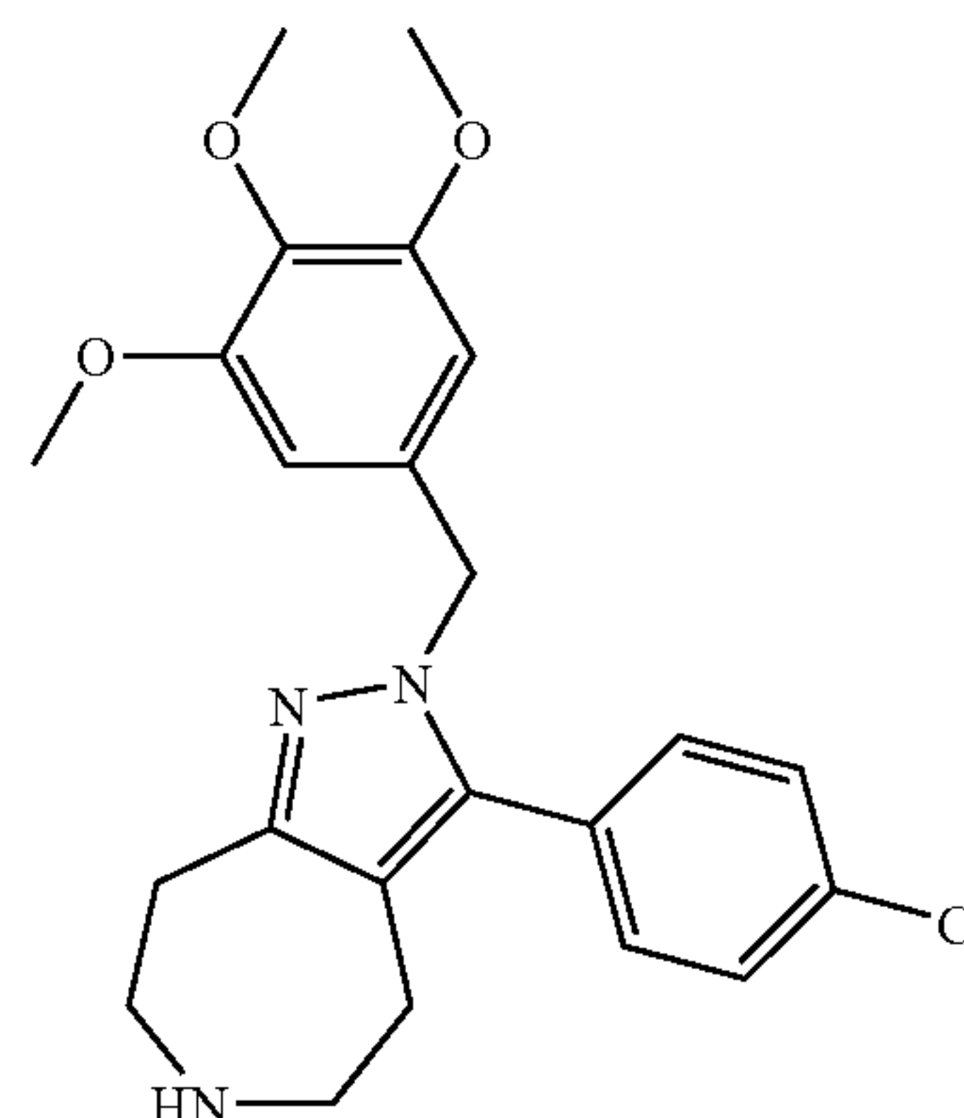
3-(4-Chloro-phenyl)-2-(3,4,5-trimethoxy-benzyl)-4,5,6,7,8-hexahydro-1,2,6-triaza-azulene
