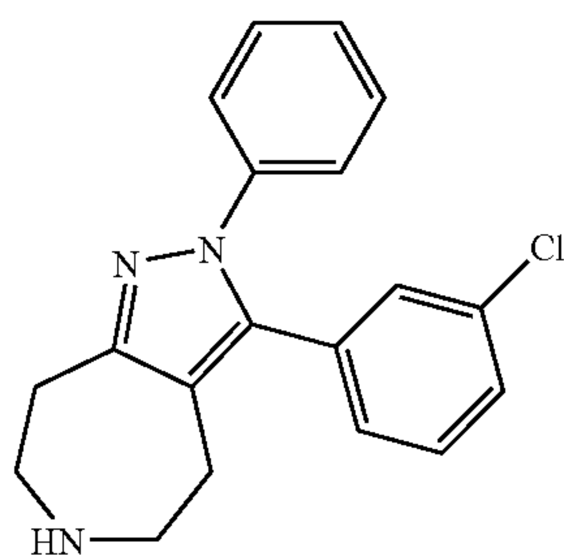
3-(3-Chloro-phenyl)-2-phenyl-2,4,5,6,7,8-hexahydro-1,2,6-triaza-azulene
