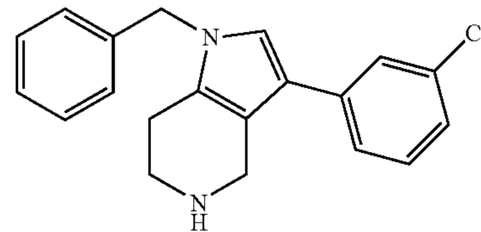
1-Benzyl-3-(3-chloro-phenyl)-4,5,6,7-tetrahydro-1H-pyrrolo[3,2-c]pyridine
