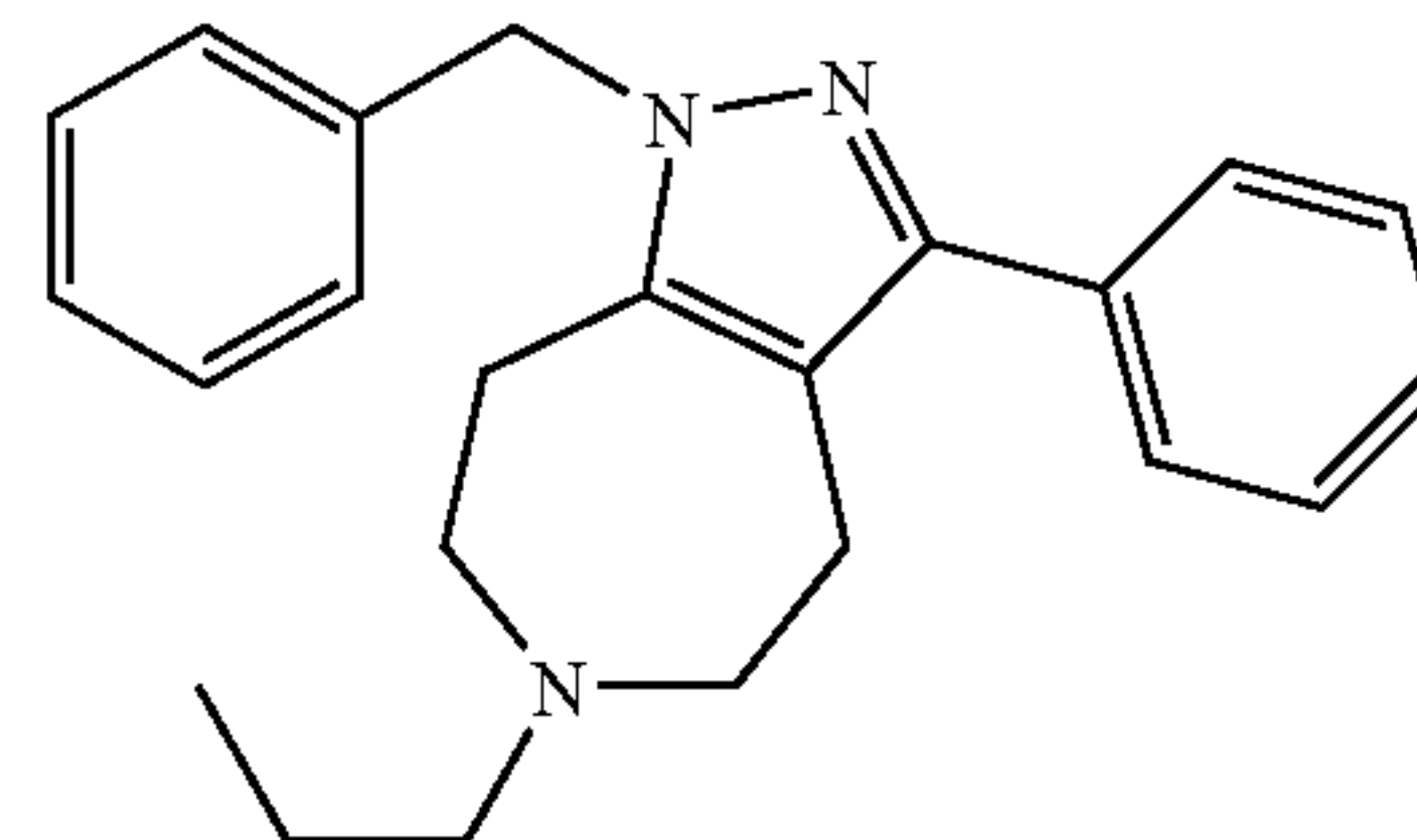
1-Benzyl-3-phenyl-6-propyl-1,4,5,6,7,8-hexahydro-1,2,6-triaza-azulene
