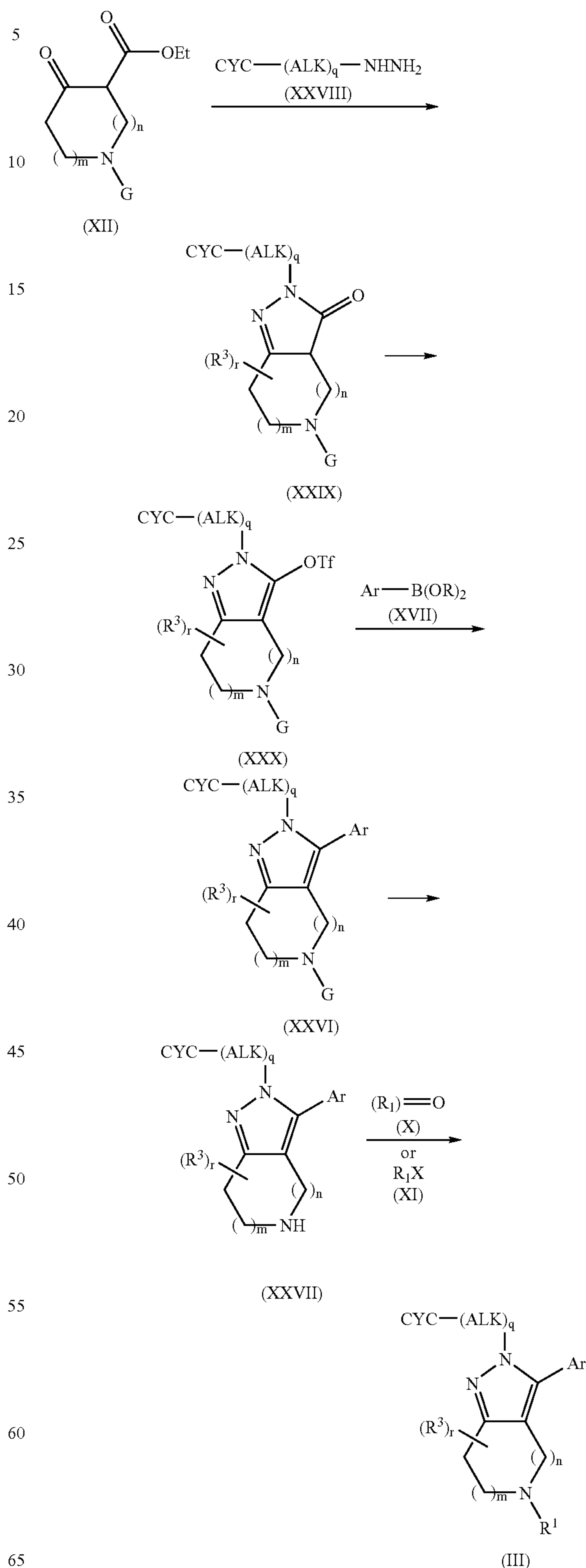
Scheme 4
