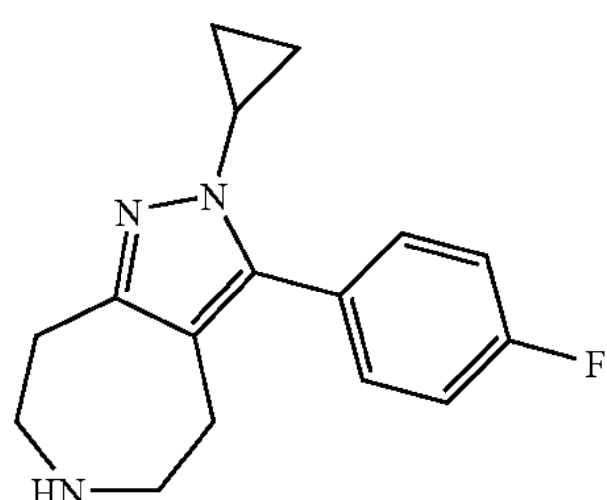
2-Cyclopropyl-3-(4-fluoro-phenyl)-2,4,5,6,7,8-hexahydro-1,2,6-triaza-azulene
