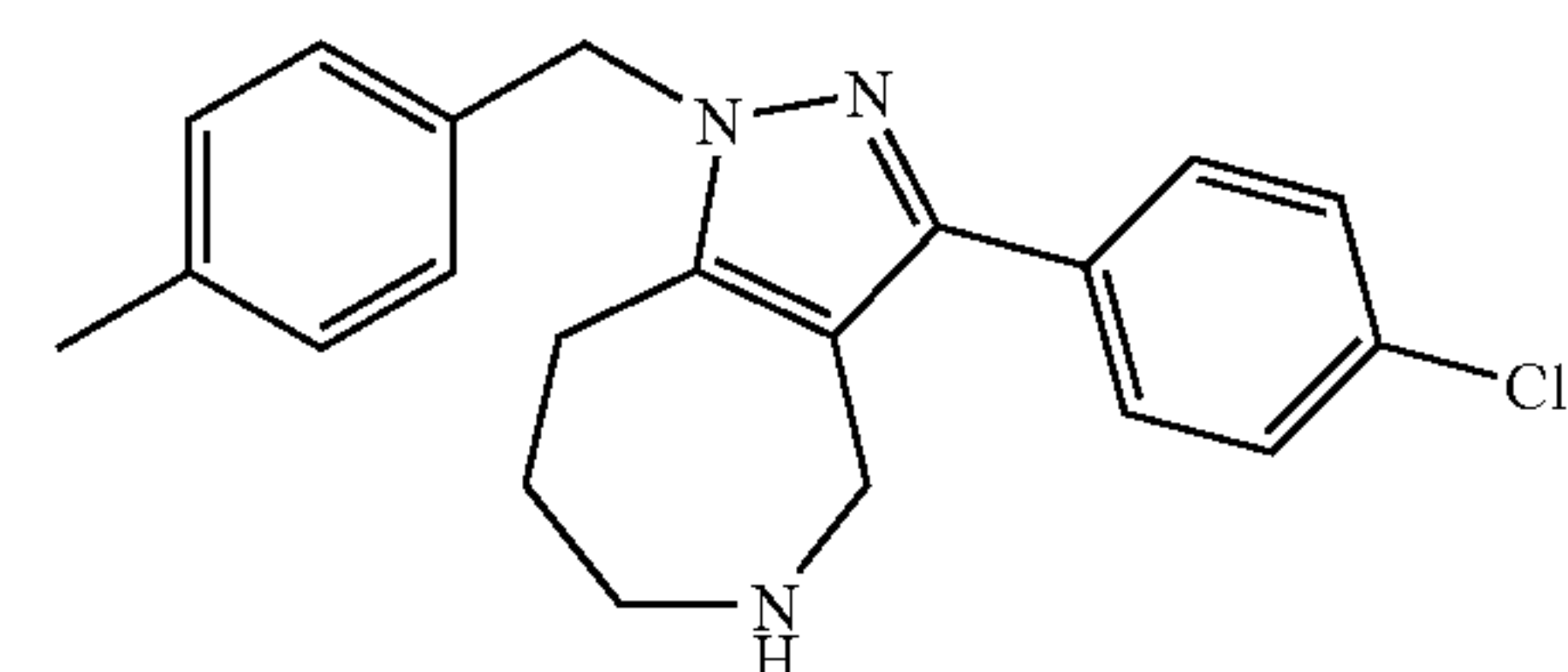
3-(4-Chloro-phenyl)-1-(4-methyl-benzyl)-1,4,5,6,7,8-hexahydro-1,2,5-triaza-azulene
