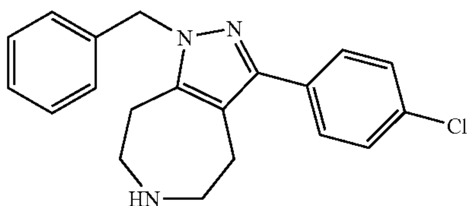
1-Benzyl-3-(4-chloro-phenyl)-1,4,5,6,7,8-hexahydro-1,2,6-triaza-azulene
