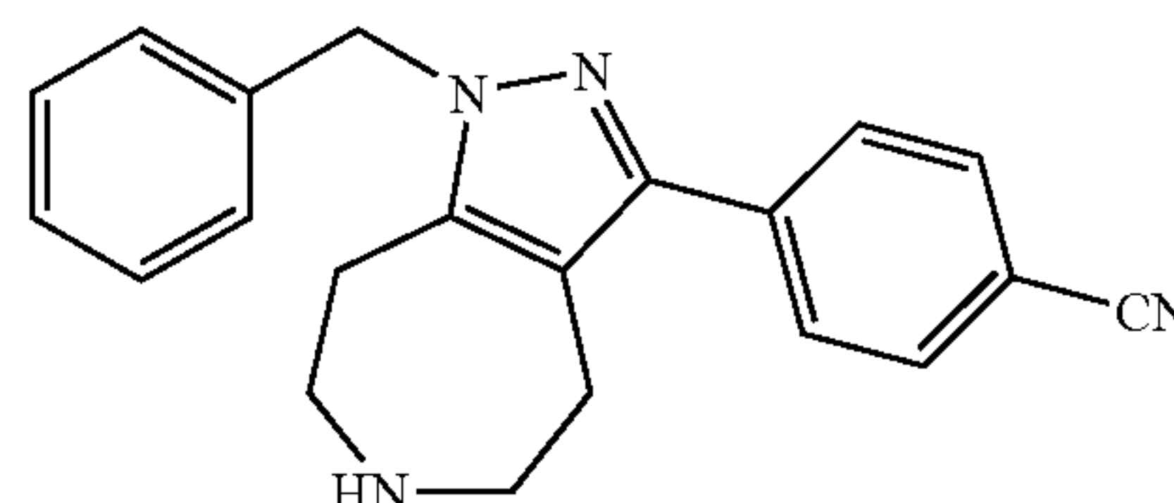
4-(1-Benzyl-1,4,5,6,7,8-hexahydro-1,2,6-triaza-azulen-3-yl)-benzonitrile
