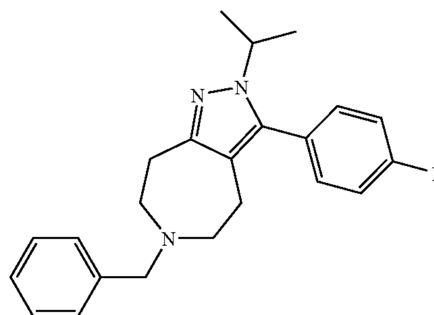
6-Benzyl-3-(4-fluoro-phenyl)-2-isopropyl-2,4,5,6,7,8-hexahydro-1,2,6-triaza-azulene
