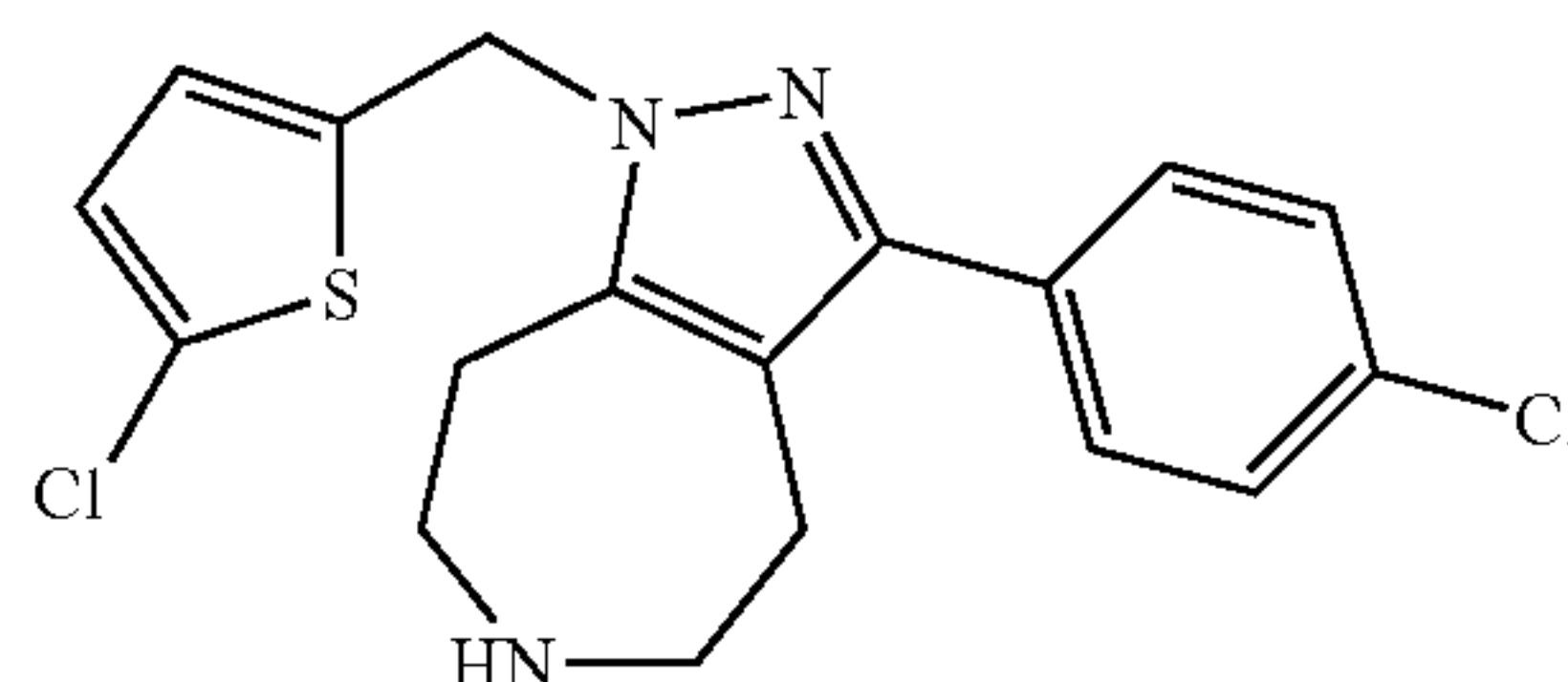
3-(4-Chloro-phenyl)-1-(5-chloro-thiophen-2-ylmethyl)-1,4,5,6,7,8-hexahydro-1,2,6-triaza-azulene
