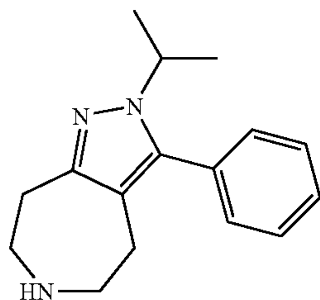
2-Isopropyl-3-phenyl-2,4,5,6,7,8-hexahydro-1,2,6-triaza-azulene
