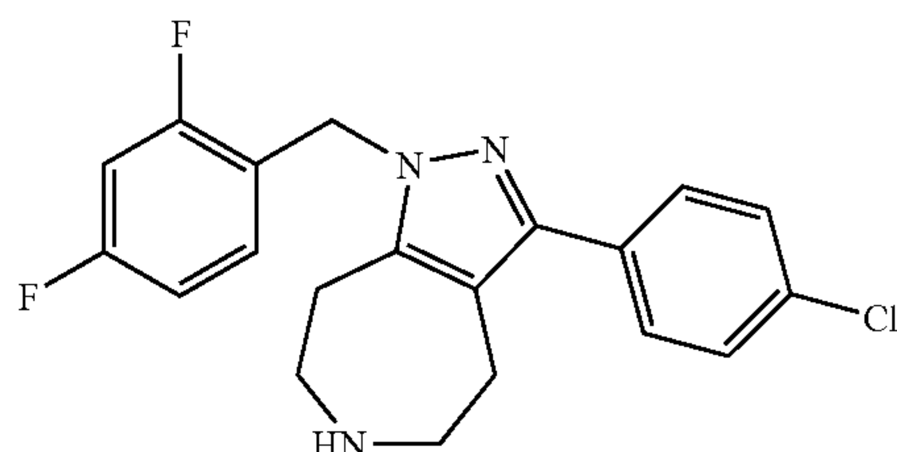
3-(4-Chloro-phenyl)-1-(2,4-difluoro-benzyl)-1,4,5,6,7,8-hexahydro-1,2,6-triaza-azulene
