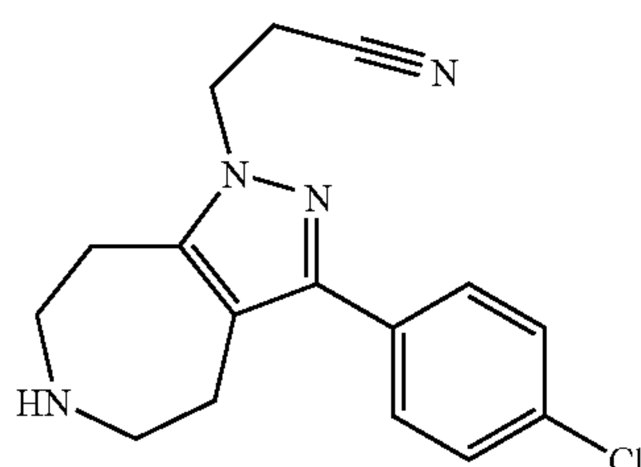
3-[3-(4-Chloro-phenyl)-5,6,7,8-tetrahydro-4H-1,2,6-triaza-azulen-1-yl]-propionitrile
