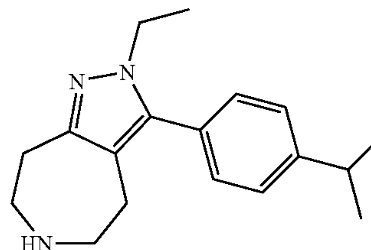
2-Ethyl-3-(4-isopropyl-phenyl)-2,4,5,6,7,8-hexahydro-1,2,6-triaza-azulene
