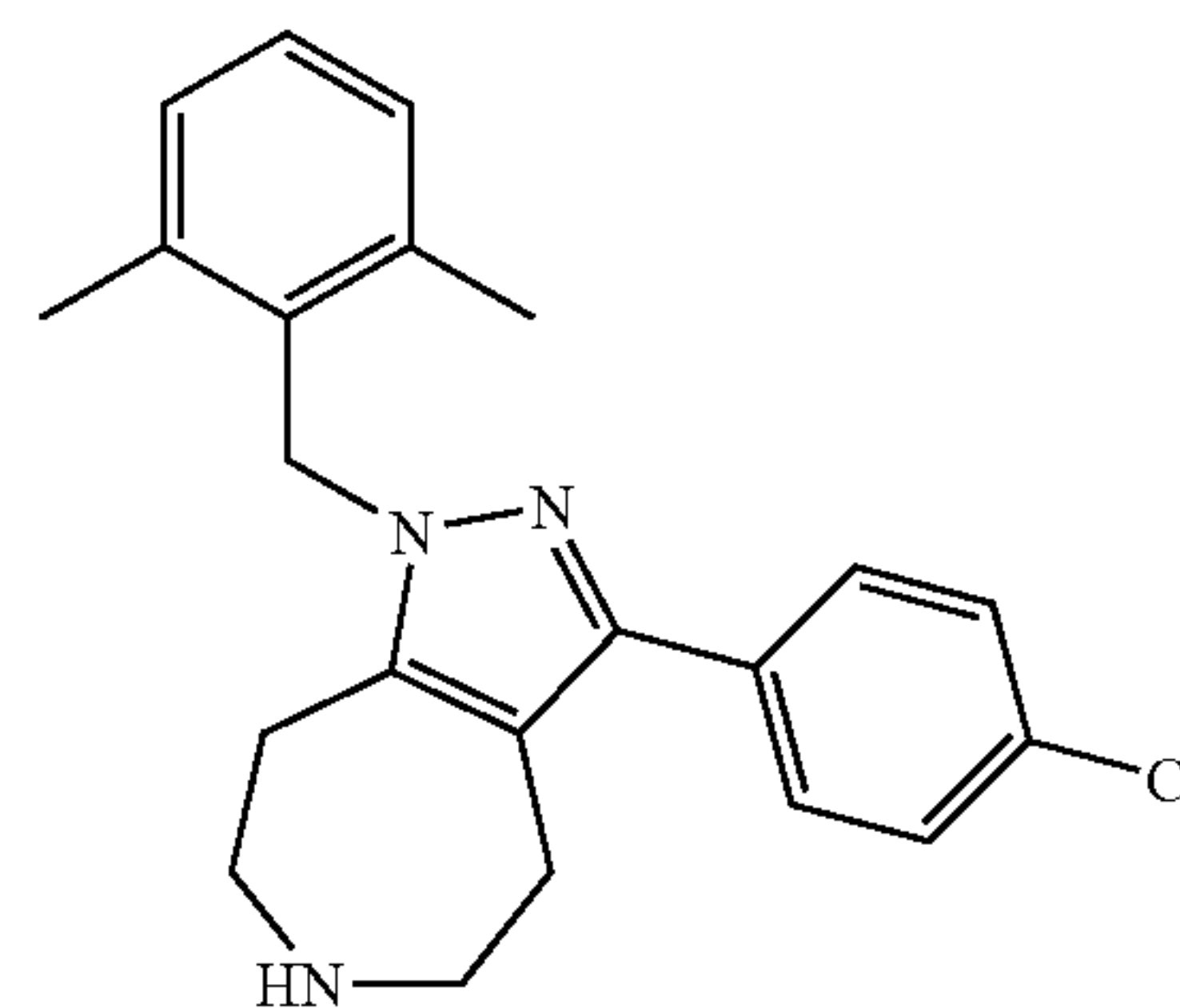
3-(4-Chloro-phenyl)-1-(2,6-dimethyl-benzyl)-4,5,6,7,8-hexahydro-1,2,6-triaza-azulene
