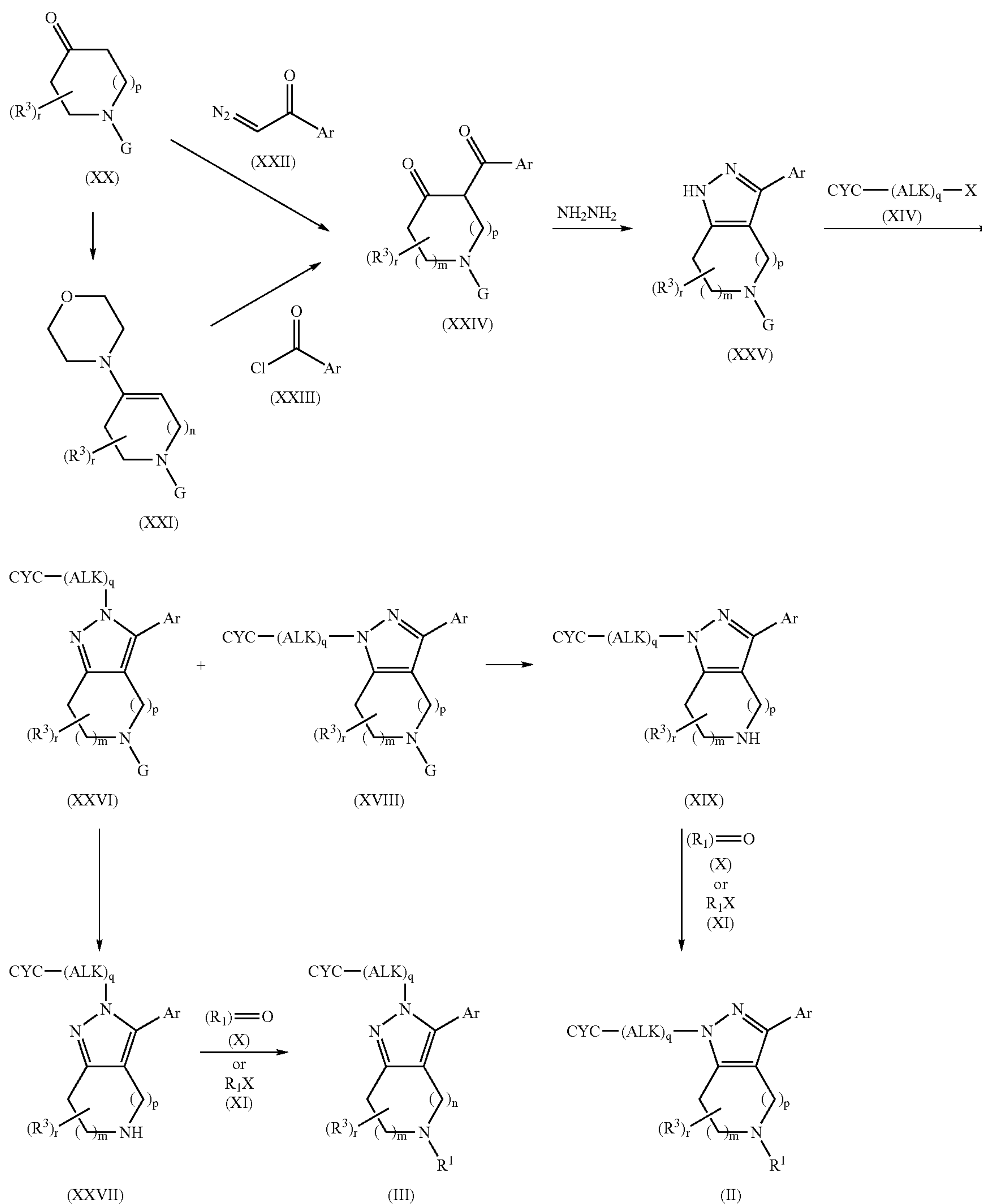
Scheme 3
