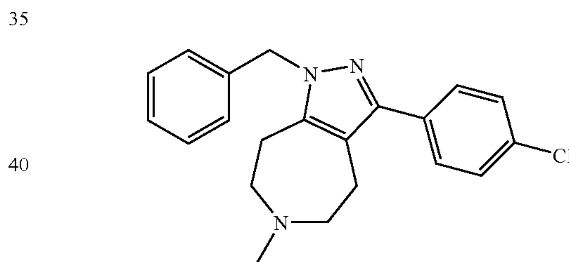
1-Benzyl-3-(4-chloro-phenyl)-6-methyl-1,4,5,6,7,8-hexahydro-1,2,6-triaza-azulene
