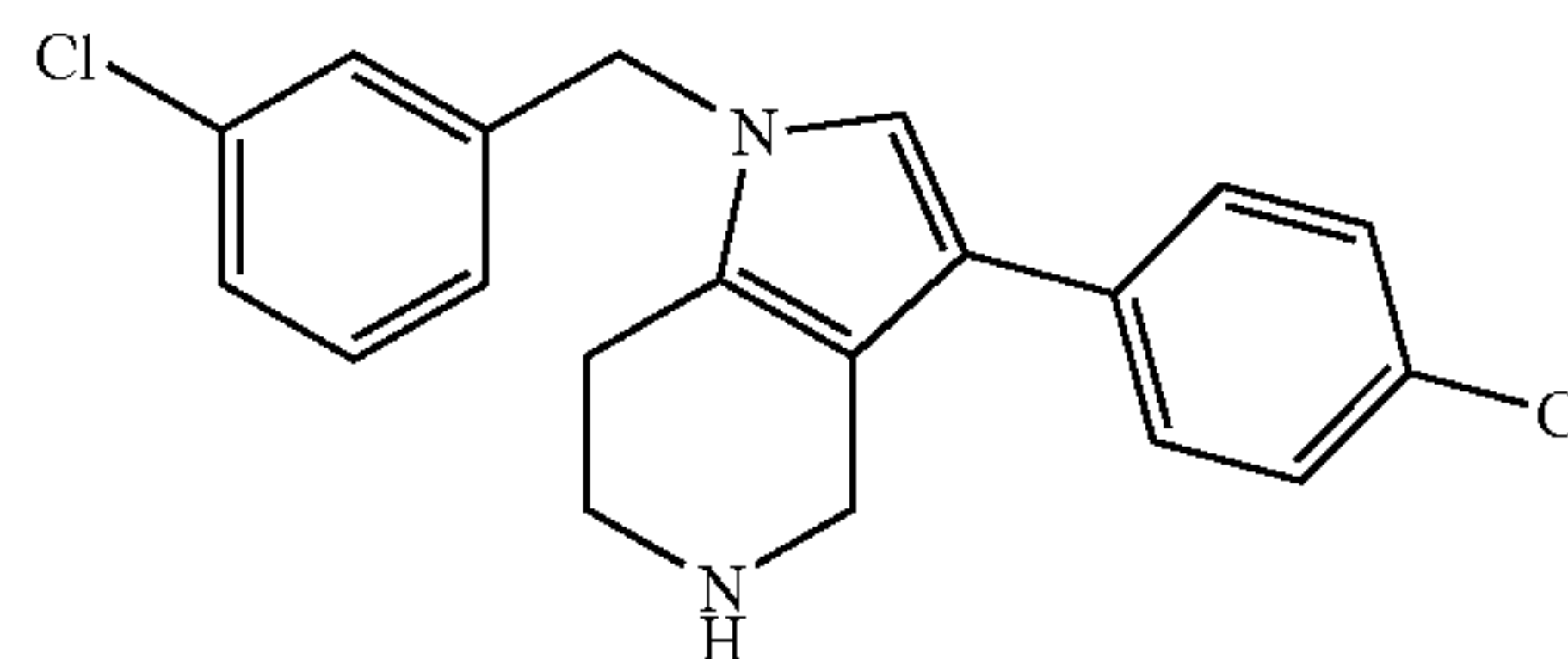
1-(3-Chloro-benzyl)-3-(4-chloro-phenyl)-4,5,6,7-tetrahydro-1H-pyrrolo[3,2-c]pyridine
