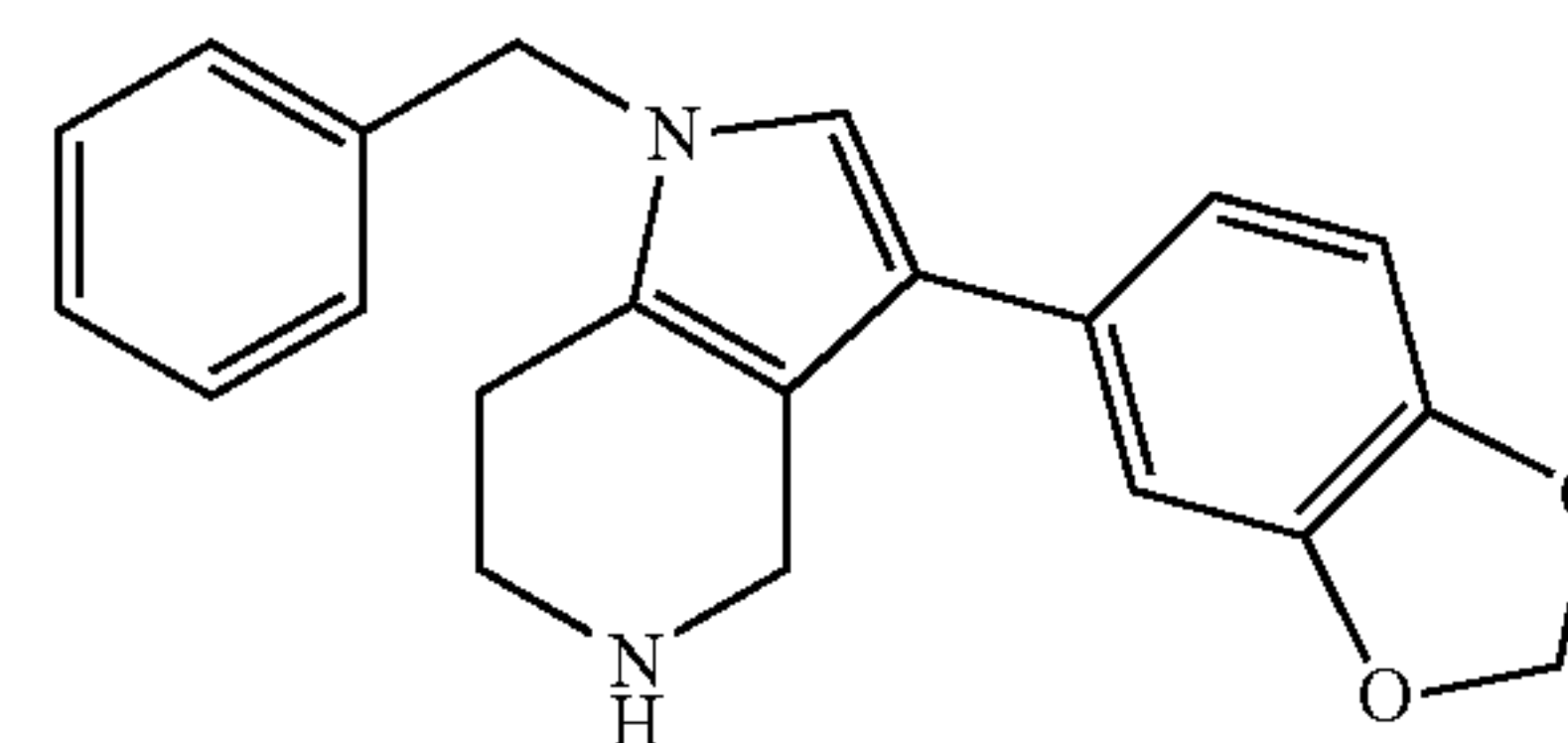
3-Benzo[1,3]dioxol-5-yl-1-benzyl-4,5,6,7-tetrahydro-1H-pyrrolo[3,2-c]pyridine
