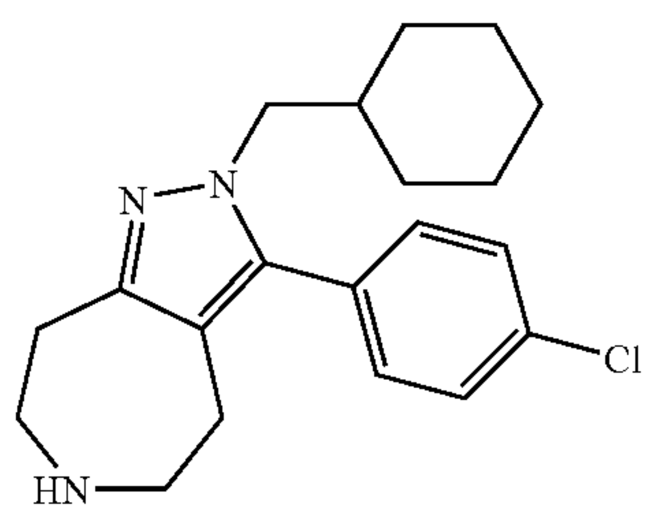
3-(4-Chloro-phenyl)-2-cyclohexylmethyl-2,4,5,6,7,8-hexahydro-1,2,6-triaza-azulene
