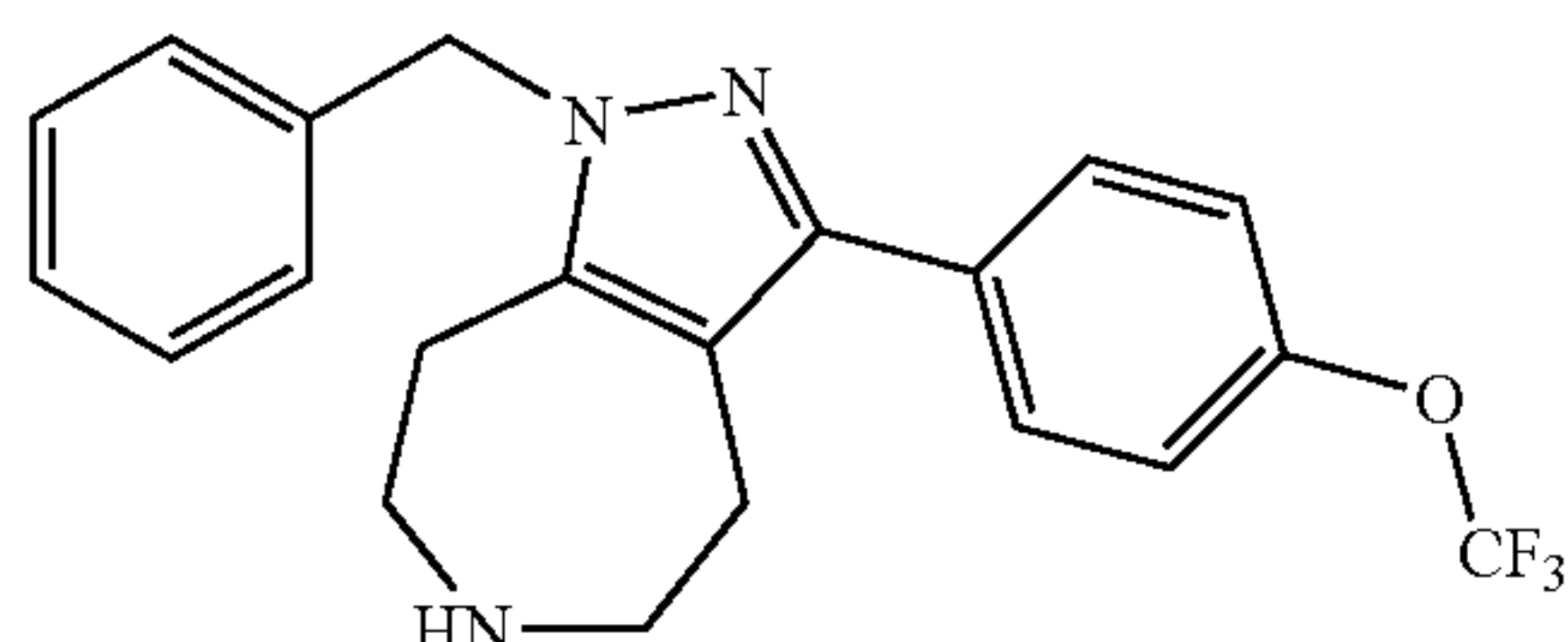
1-Benzyl-3-(4-trifluoromethoxy-phenyl)-1,4,5,6,7,8-hexahydro-1,2,6-triaza-azulene
