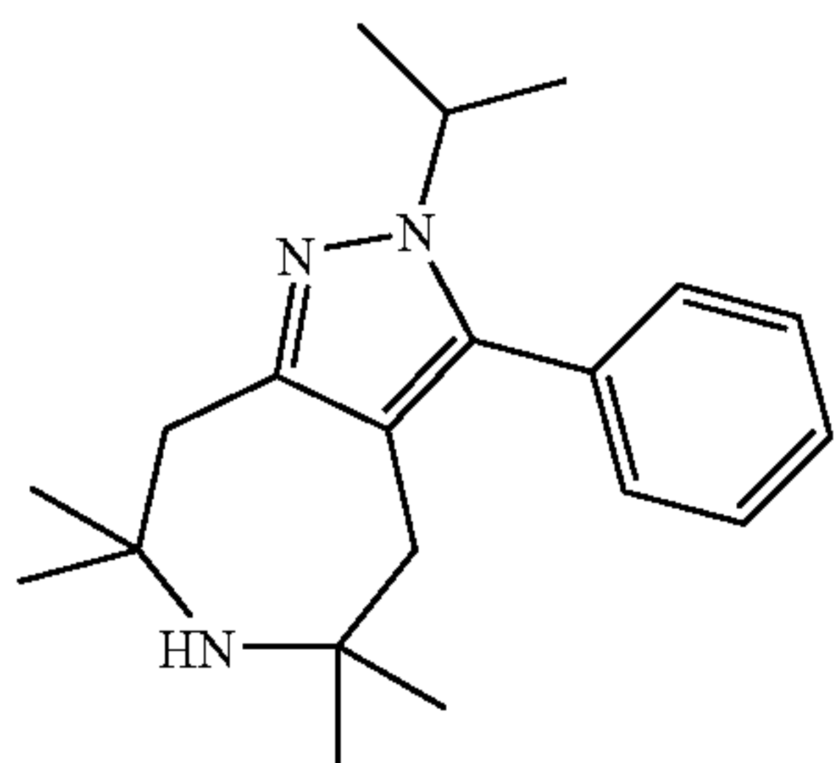
2-Isopropyl-5,5,7,7-tetramethyl-3-phenyl-2,4,5,6,7,8-hexahydro-1,2,6-triaza-azulene
