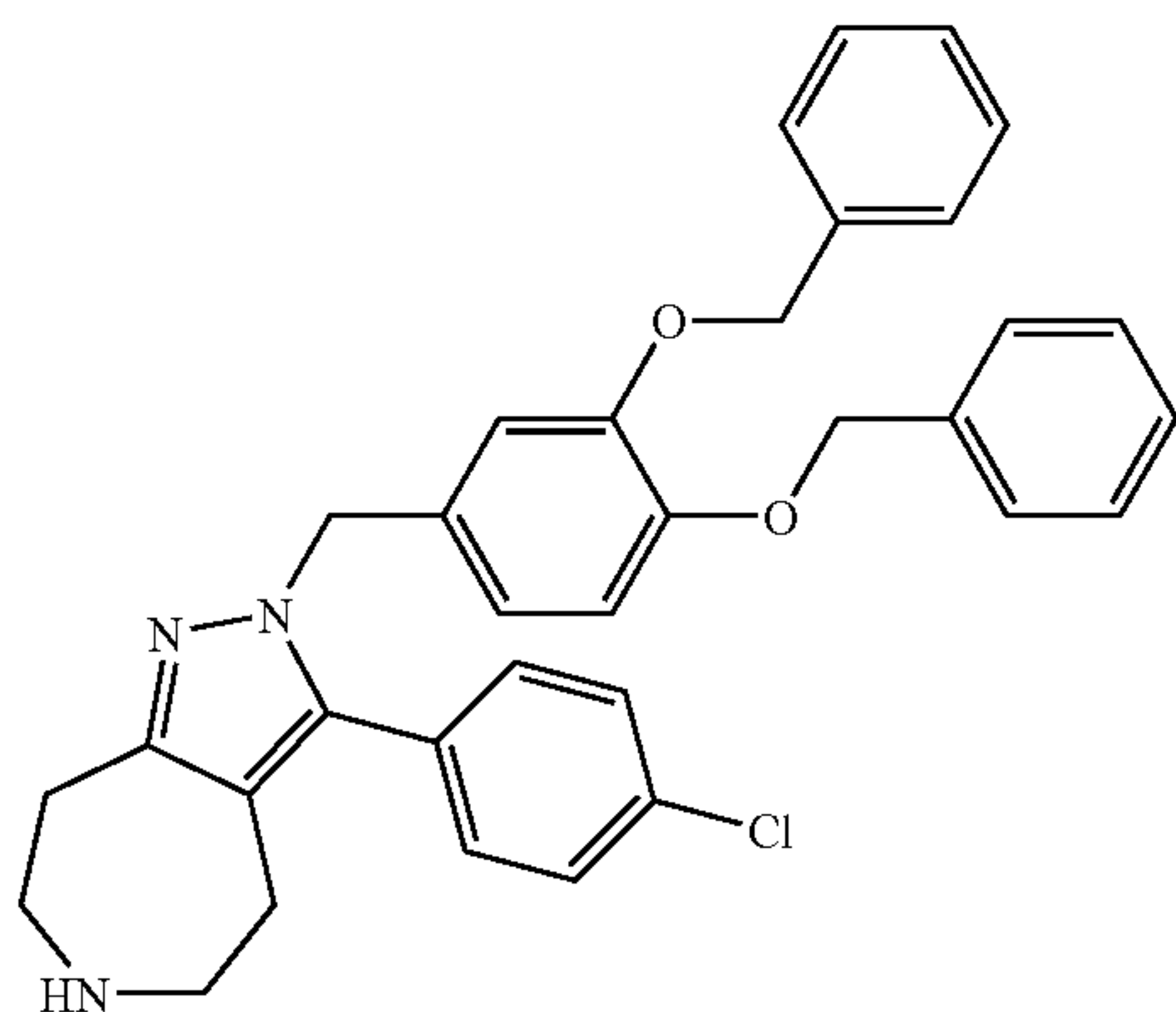
2-(3,4-Bis-benzyloxy-benzyl)-3-(4-chloro-phenyl)-2,4,5,6,7,8-hexahydro-1,2,6-triaza-azulene
