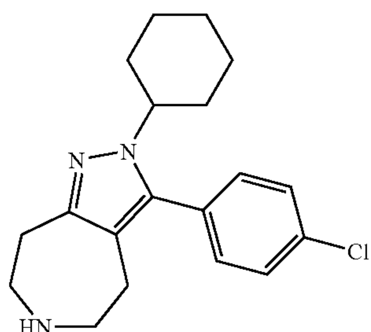
3-(4-Chloro-phenyl)-2-cyclohexyl-2,4,5,6,7,8-hexahydro-1,2,6-triaza-azulene
