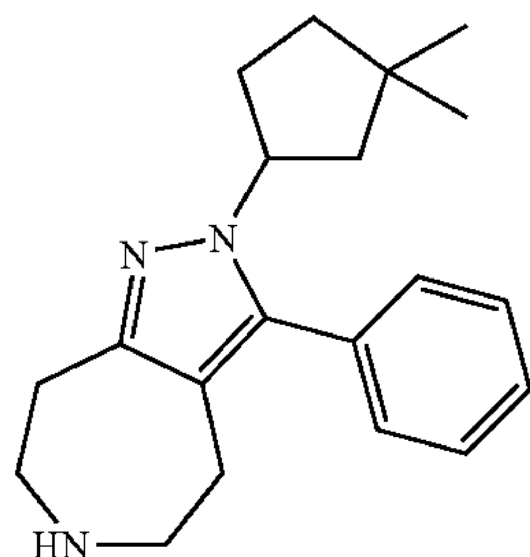
2-(3,3-Dimethyl-cyclopentyl)-3-phenyl-2,4,5,6,7,8-hexahydro-1,2,6-triaza-azulene
