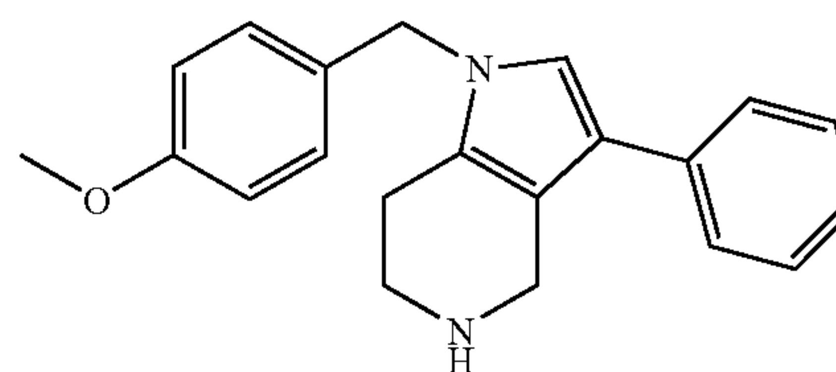
1-(4-Methoxy-benzyl)-3-phenyl-4,5,6,7-tetrahydro-1H-pyrrolo[3,2-c]pyridine
