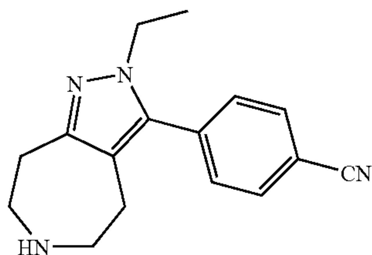
4-(2-Ethyl-2,4,5,6,7,8-hexahydro-1,2,6-triaza-azulen-3-yl)-benzonitrile
