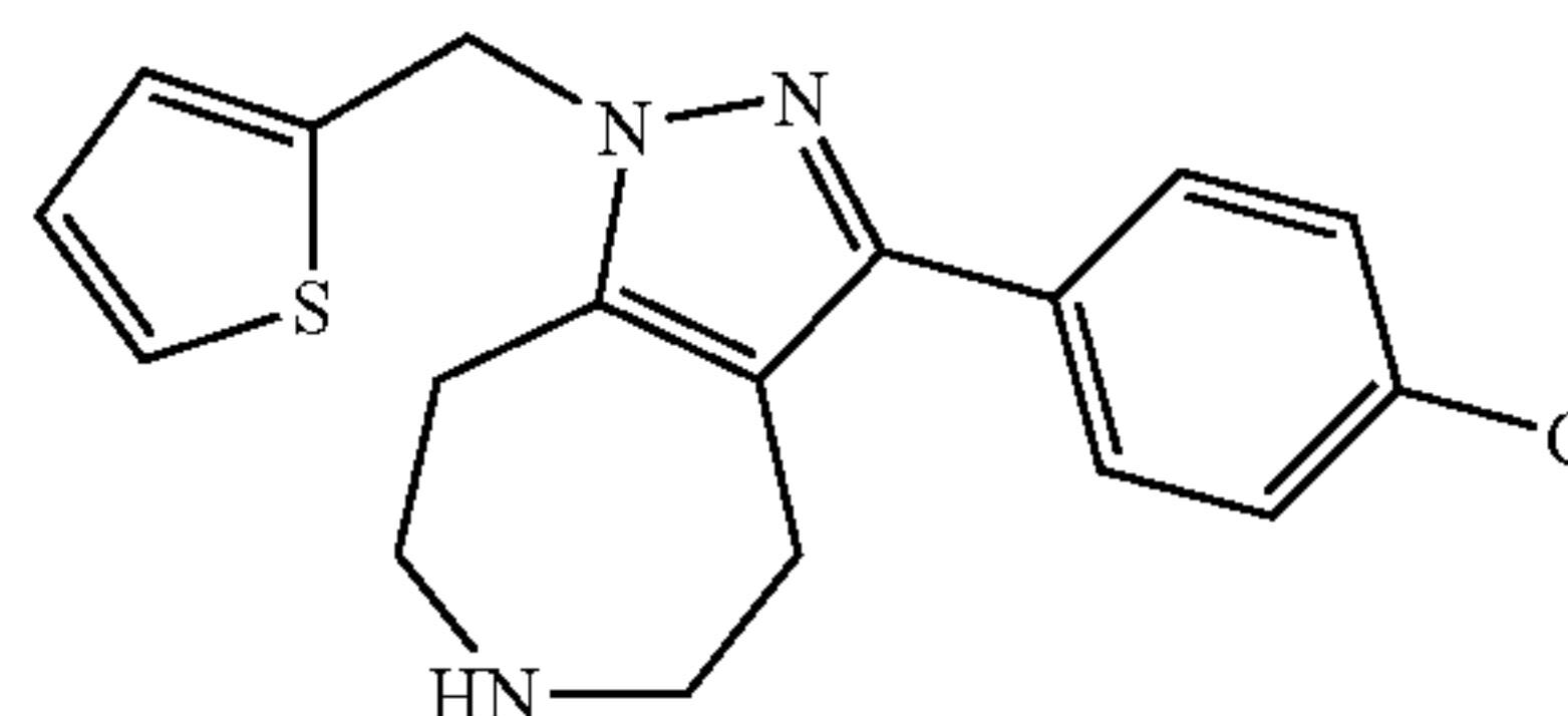
3-(4-Chloro-phenyl)-1-thiophen-2-ylmethyl-1,4,5,6,7,8-hexahydro-1,2,6-triaza-azulene
