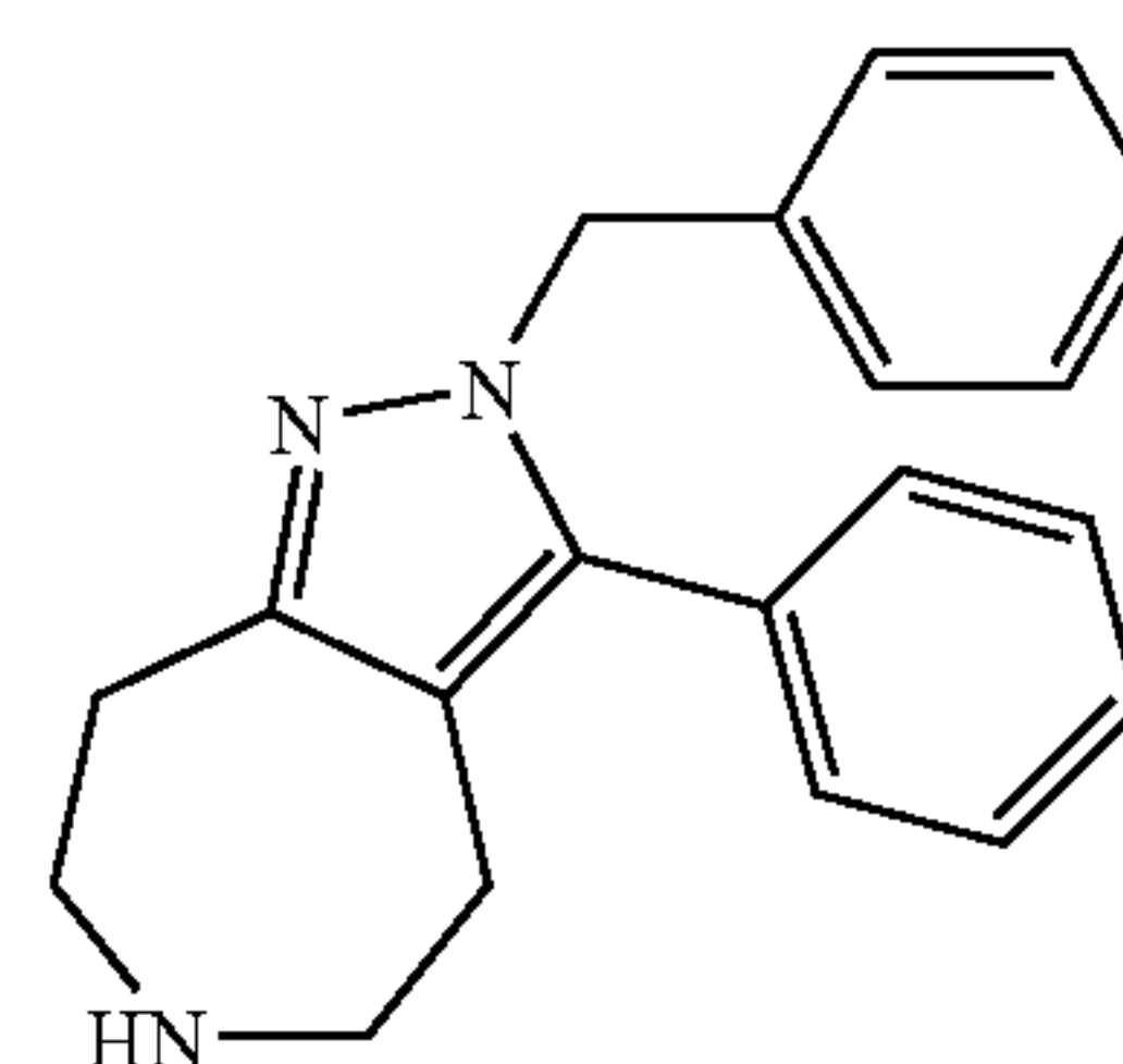
2-Benzyl-3-phenyl-2,4,5,6,7,8-hexahydro-1,2,6-triaza-azulene
