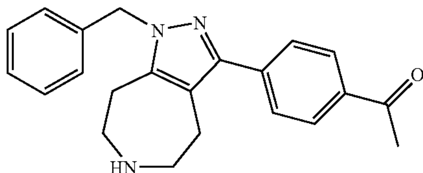
1-[4-(1-Benzyl-1,4,5,6,7,8-hexahydro-1,2,6-triaza-azulen-3-yl)-phenyl]-ethanone
