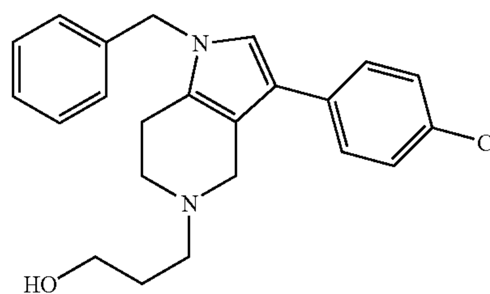
3-[1-Benzyl-3-(4-chloro-phenyl)-1,4,6,7-tetrahydro-pyrrolo[3,2-c]pyridin-5-yl]-propan-1-ol
