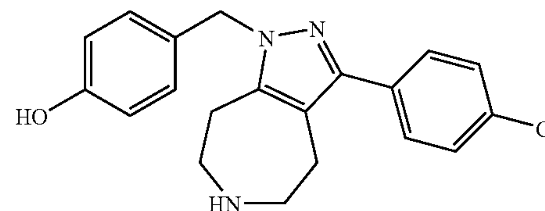
4-[3-(4-Chloro-phenyl)-5,6,7,8-tetrahydro-4H-1,2,6-triaza-azulen-1-ylmethyl]-phenol
