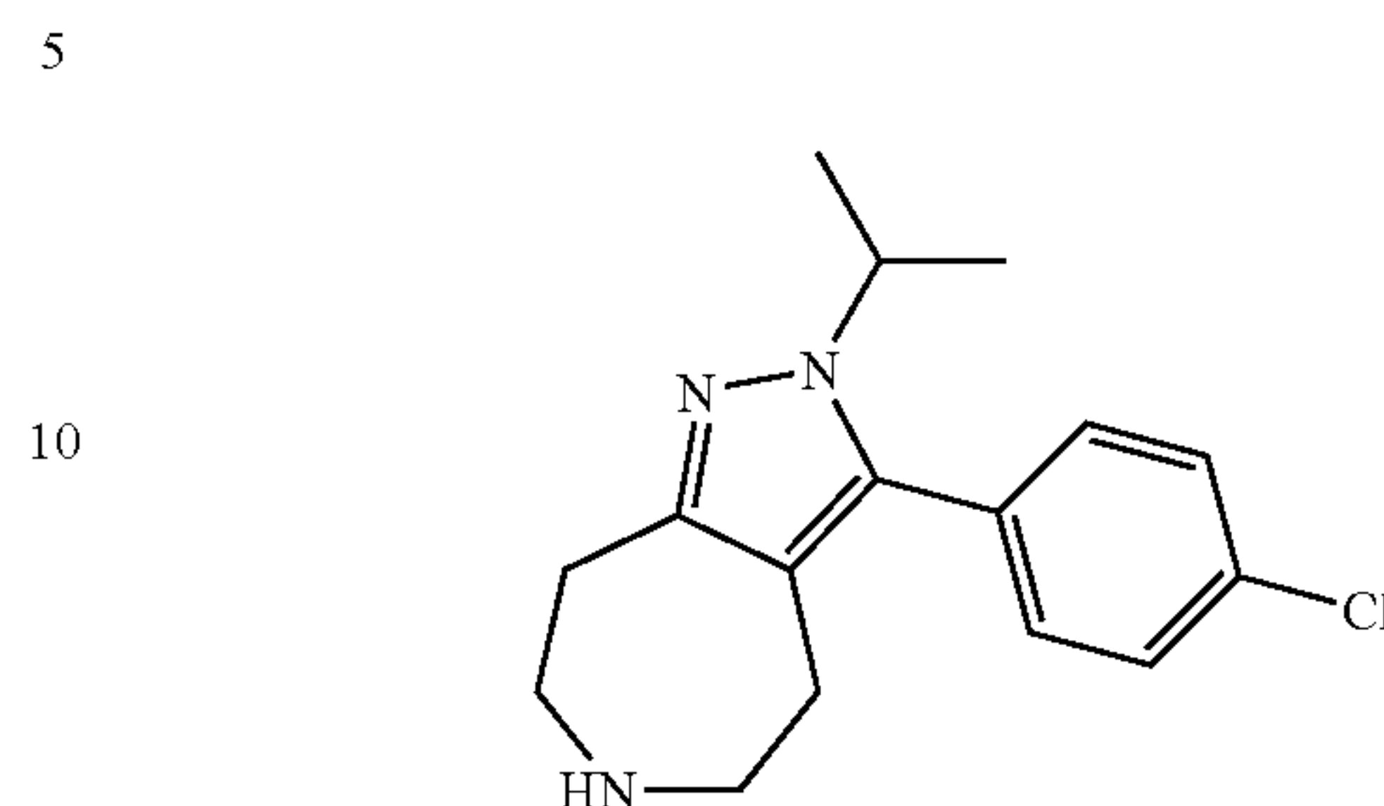
3-(4-Chloro-phenyl)-2-isopropyl-2,4,5,6,7,8-hexahydro-1,2,6-triaza-azulene
