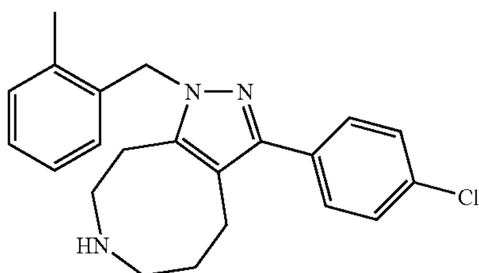
3-(4-Chloro-phenyl)-1-(2-methyl-benzyl)-4,5,6,7,8,9-hexahydro-1H-1,2,7-triaza-cyclopentacycloocte
