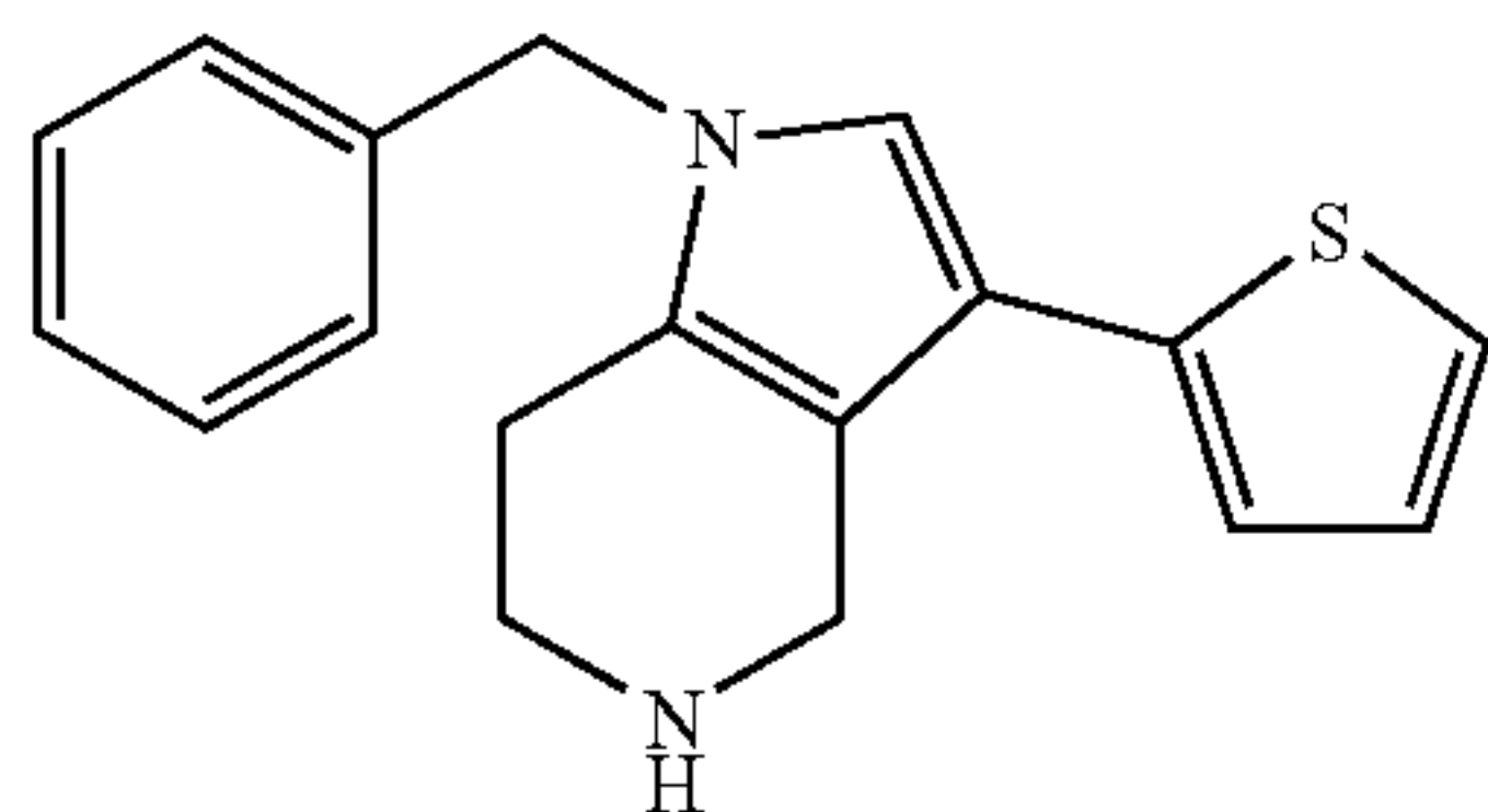
1-Benzyl-3-thiophen-2-yl-4,5,6,7-tetrahydro-1H-pyrrolo[3,2-c]pyridine
