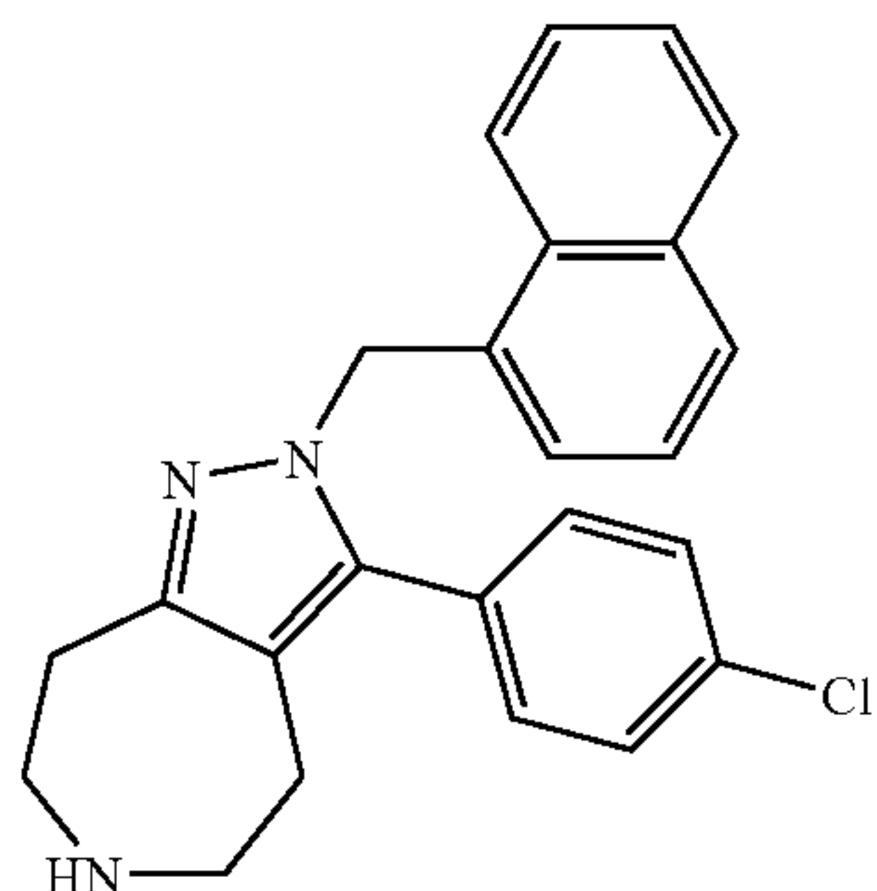
3-(4-Chloro-phenyl)-2-naphthalen-1-ylmethyl-4,5,6,7,8-hexahydro-1,2,6-triaza-azulene
