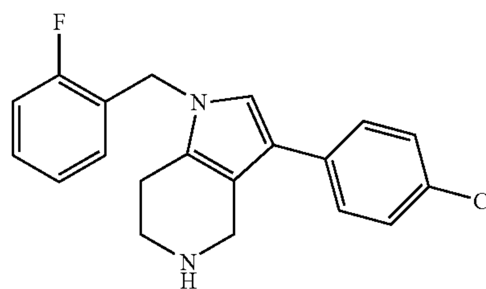
3-(4-Chloro-phenyl)-1-(2-fluoro-benzyl)-4,5,6,7-tetrahydro-1H-pyrrolo[3,2-c]pyridine
