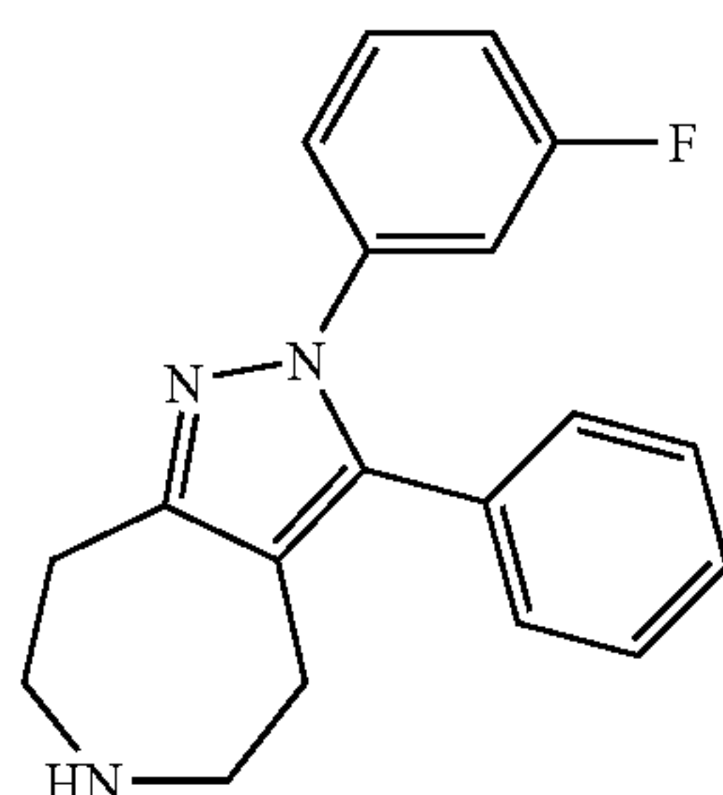
2-(3-Fluoro-phenyl)-3-phenyl-2,4,5,6,7,8-hexahydro-1,2,6-triaza-azulene
