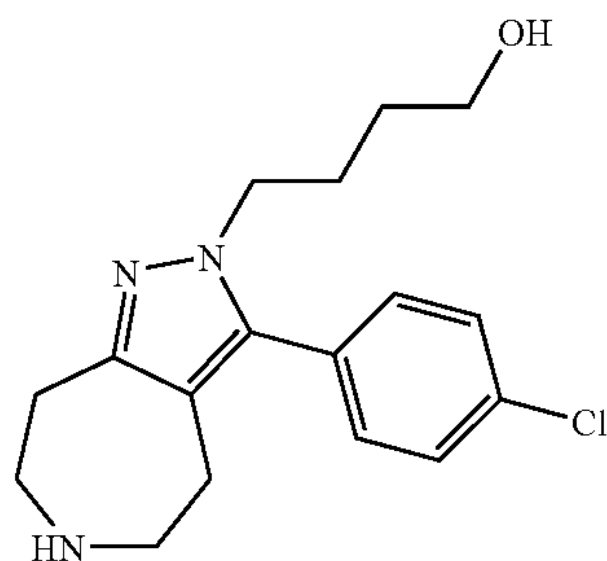
4-[3-(4-Chloro-phenyl)-5,6,7,8-tetrahydro-4H-1,2,6-triaza-azulen-2-yl]-butan-1-ol
