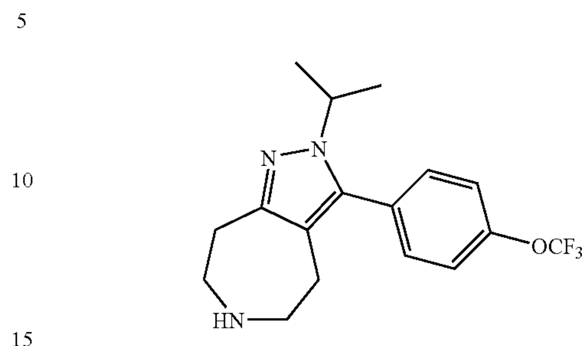
2-Isopropyl-3-(4-trifluoromethoxy-phenyl)-2,4,5,6,7, 8-hexahydro-1,2,6-triaza-azulene
