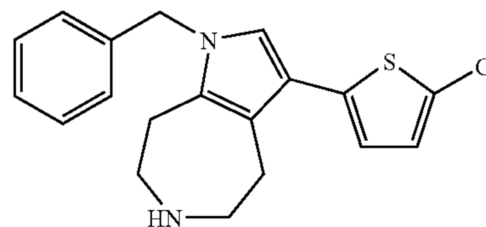
1-Benzyl-3-(5-chloro-thiophen-2-yl)-1,4,5,6,7,8-hexahydro-pyrrolo[2,3-d]azepine
