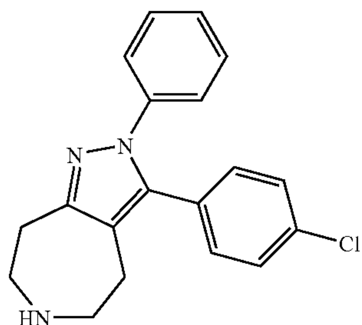
3-(4-Chloro-phenyl)-2-phenyl-2,4,5,6,7,8-hexahydro-1,2,6-triaza-azulene
