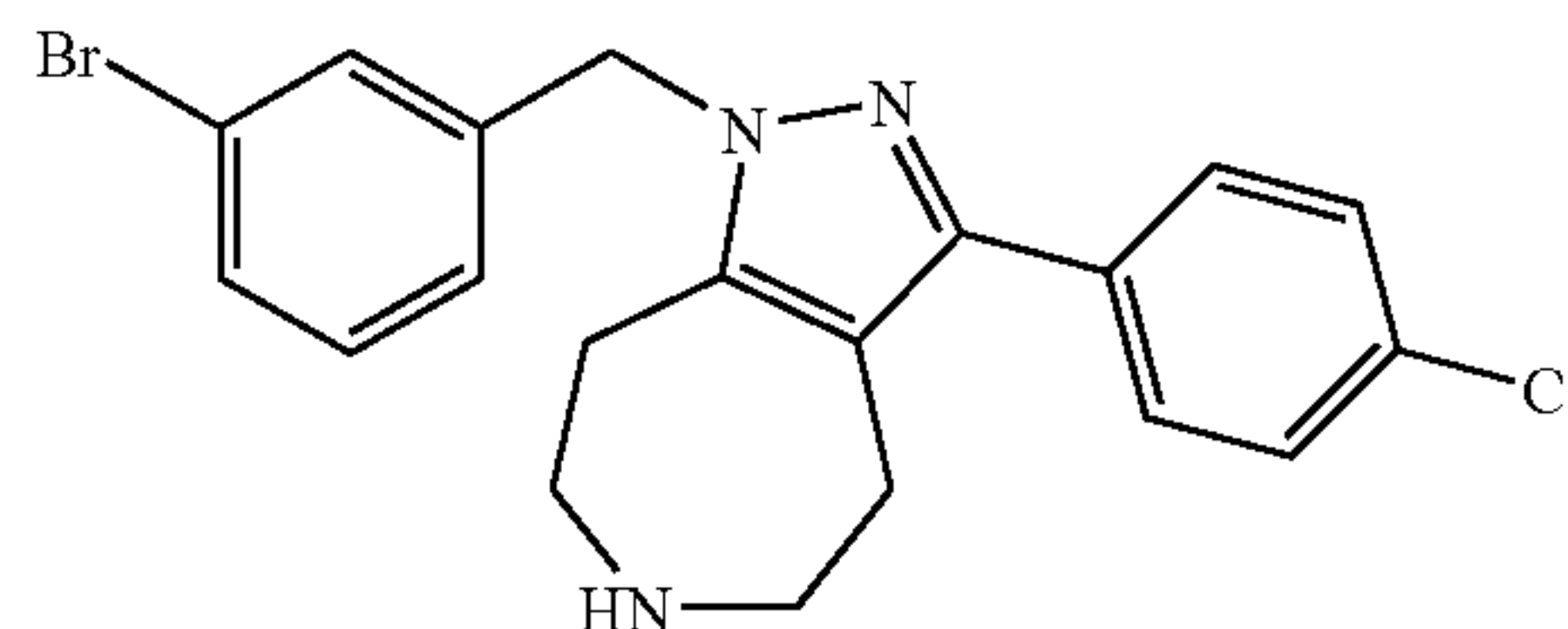
1-(3-Bromo-benzyl)-3-(4-chloro-phenyl)-1,4,5,6,7,8-hexahydro-1,2,6-triaza-azulene
