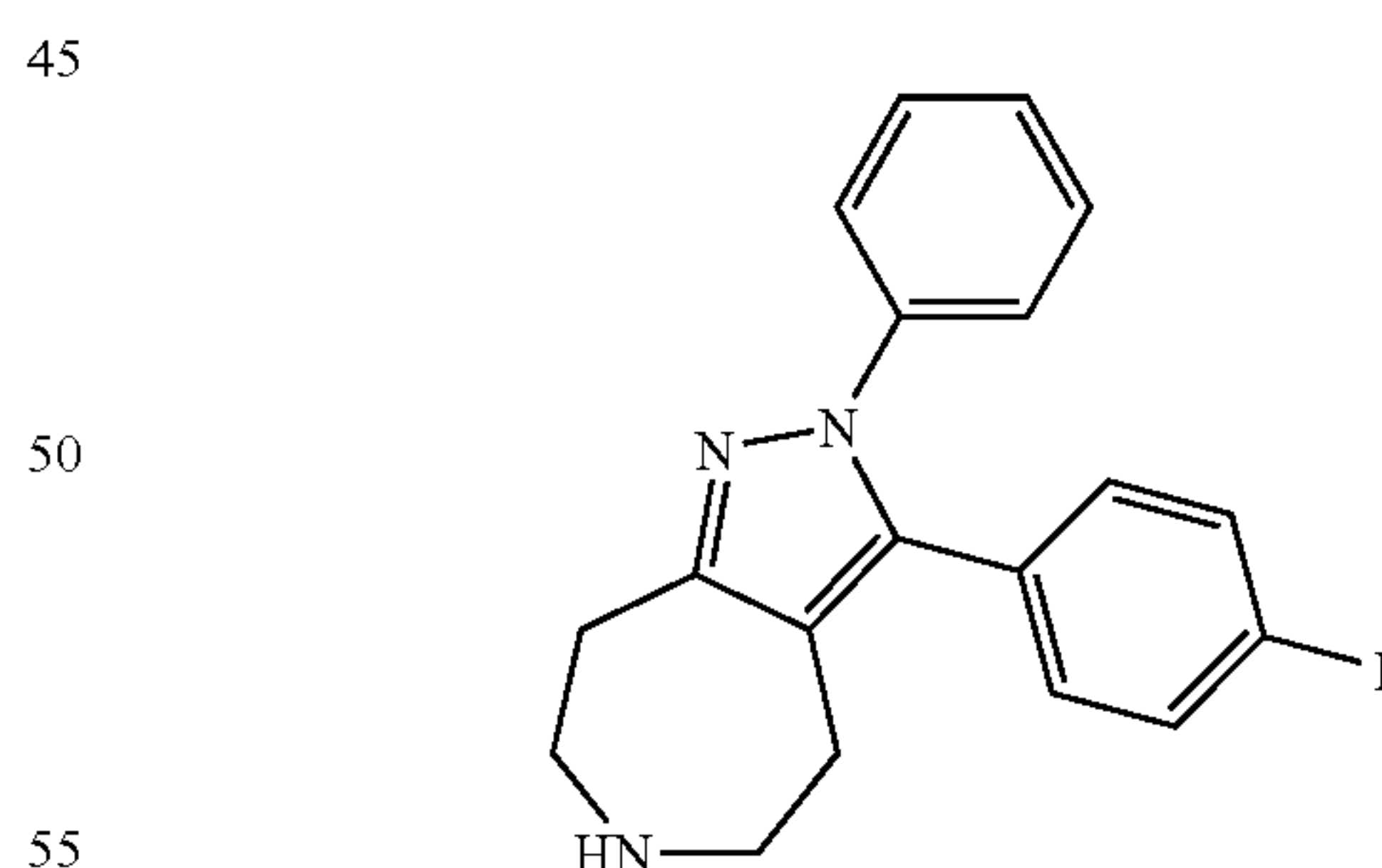
3-(4-Fluoro-phenyl)-2-phenyl-2,4,5,6,7,8-hexahydro-1,2,6-triaza-azulene
