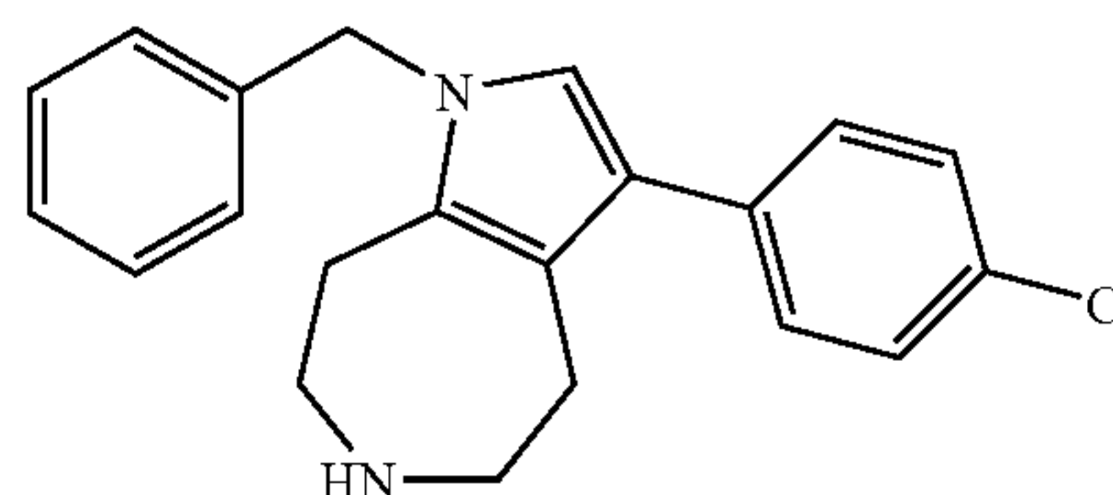
1-Benzyl-3-(4-chloro-phenyl)-1,4,5,6,7,8-hexahydro-pyrrolo[2,3-d]azepine
