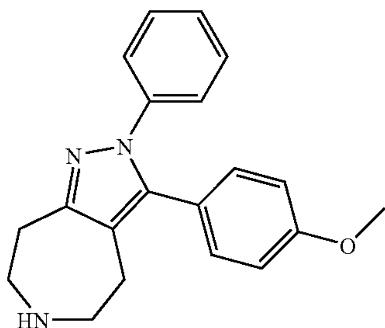
3-(4-Methoxy-phenyl)-2-phenyl-2,4,5,6,7,8-hexahydro-1,2,6-triaza-azulene
