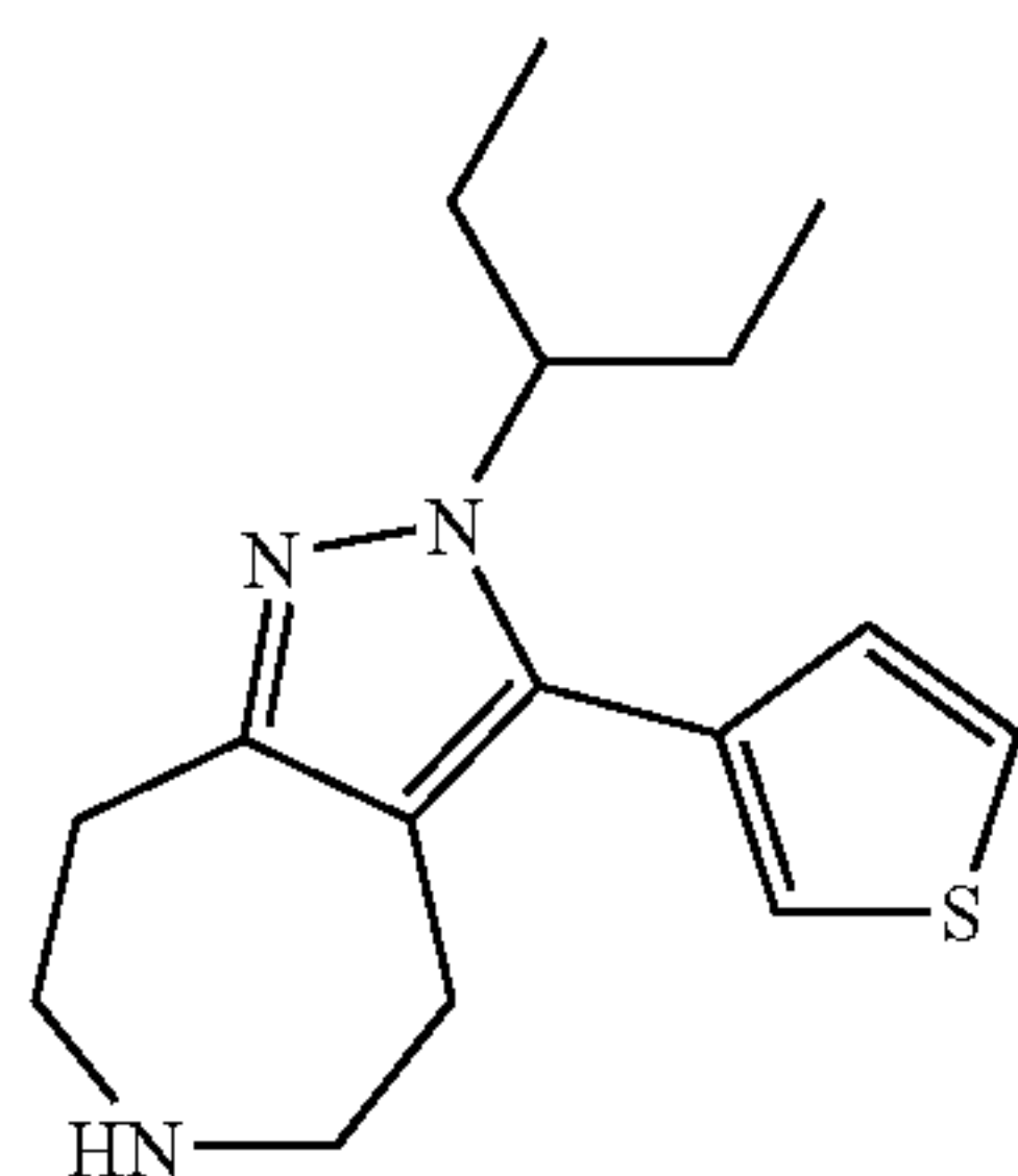
2-(1-Ethyl-propyl)-3-thiophen-3-yl-2,4,5,6,7,8-hexahydro-1,2,6-triaza-azulene
