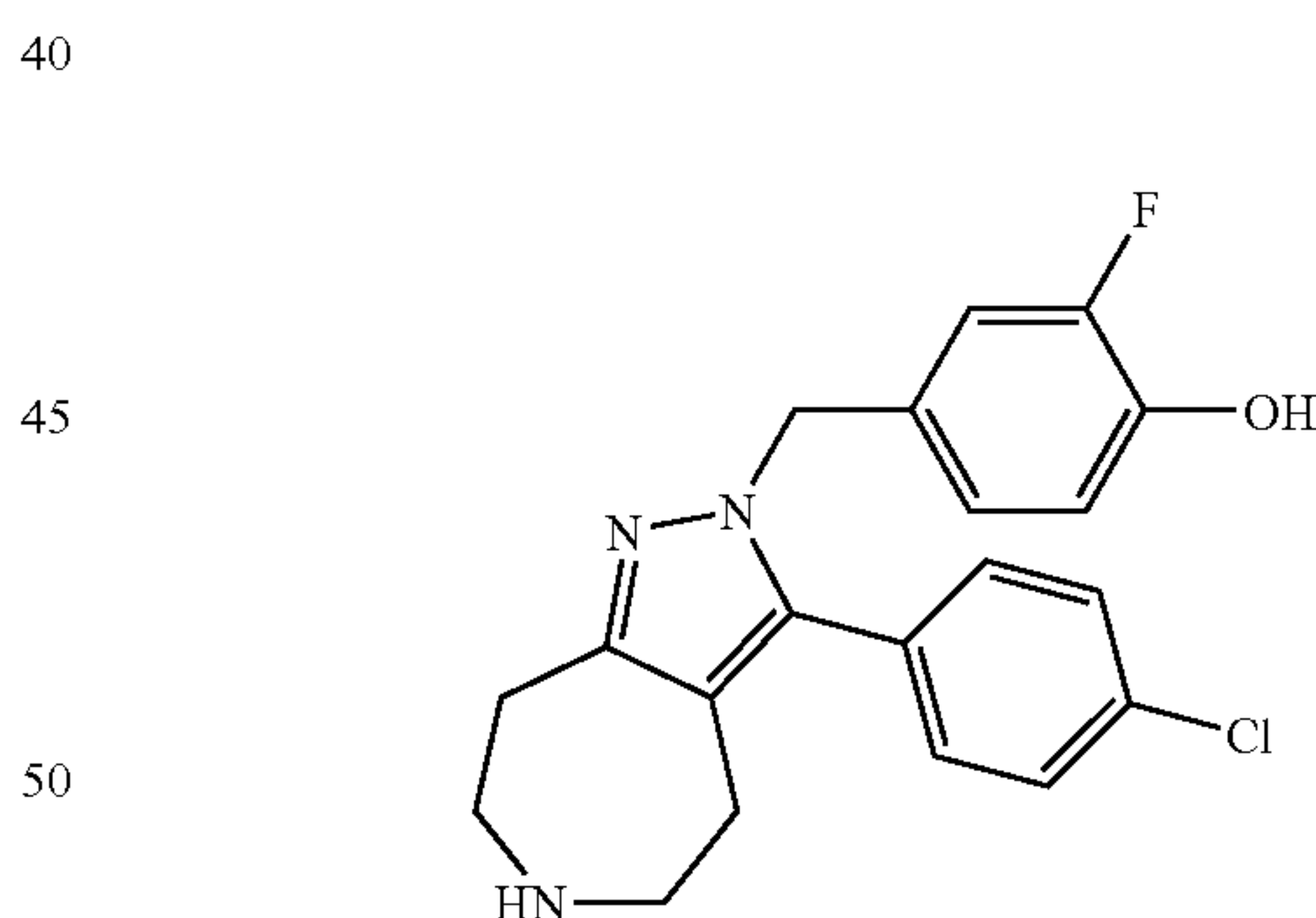
4-[3-(4-Chloro-phenyl)-5,6,7,8-tetrahydro-4H-1,2,6-triaza-azulen-2-ylmethyl]-2-fluoro-phenol
