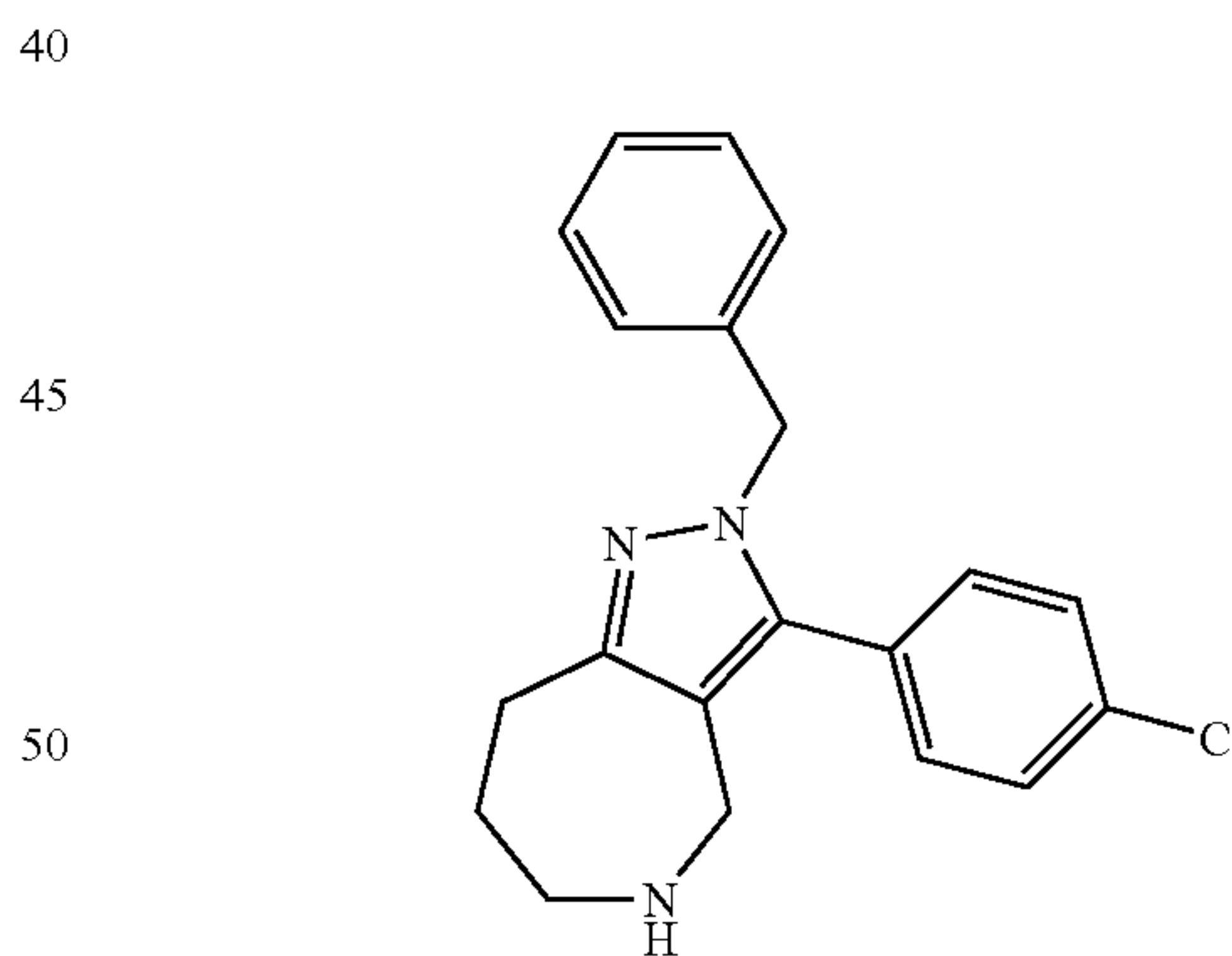
2-Benzyl-3-(4-chloro-phenyl)-2,4,5,6,7,8-hexahydro-1,2,5-triaza-azulene
