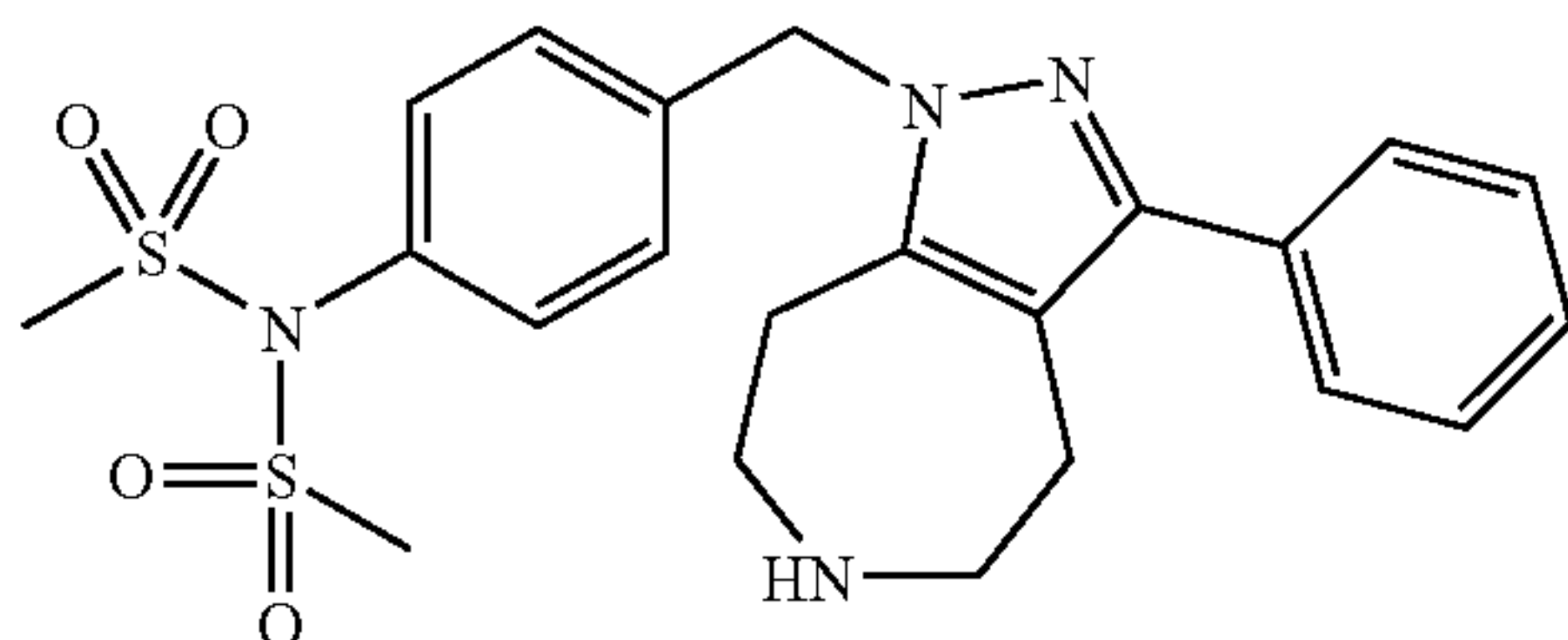
N,N-[4-(3-phenyl-5,6,7,8-tetrahydro-4H-1,2,6-triaza-azulen-1-ylmethyl)-phenyl]-dimethanesulfonamide
