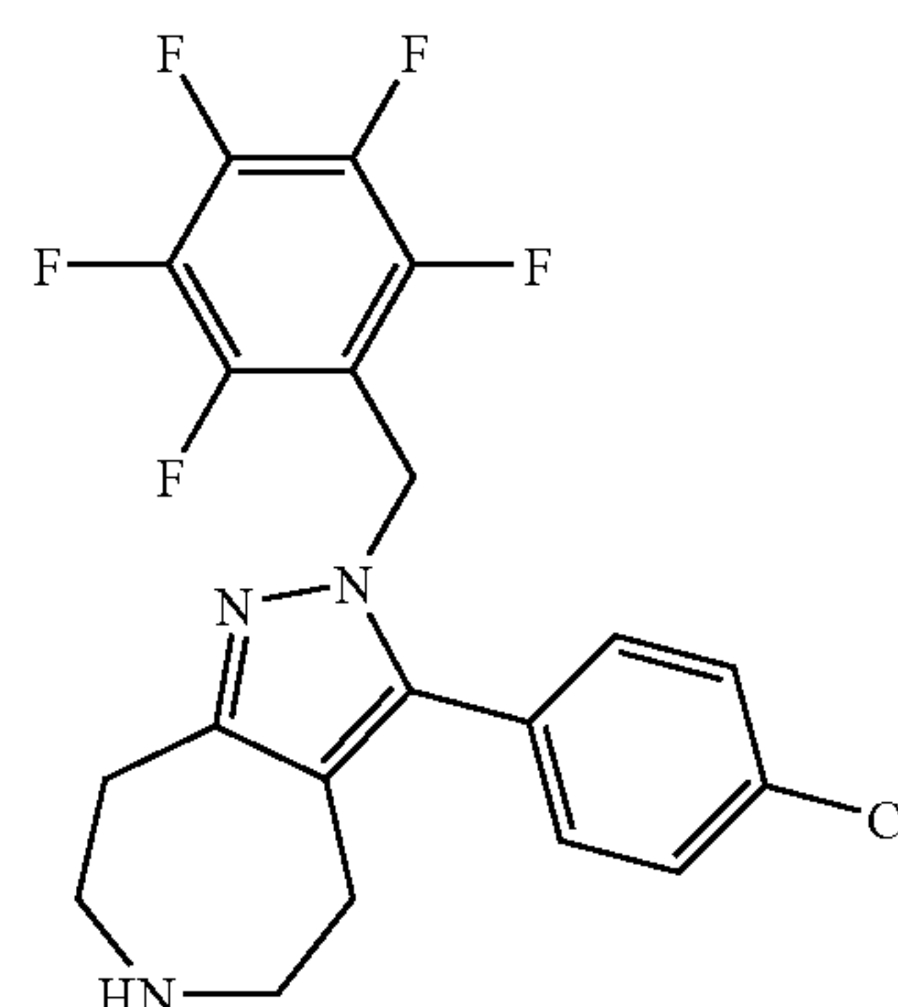
3-(4-Chloro-phenyl)-2-pentafluorophenylmethyl-2,4, 5,6,7,8-hexahydro-1,2,6-triaza-azulene
