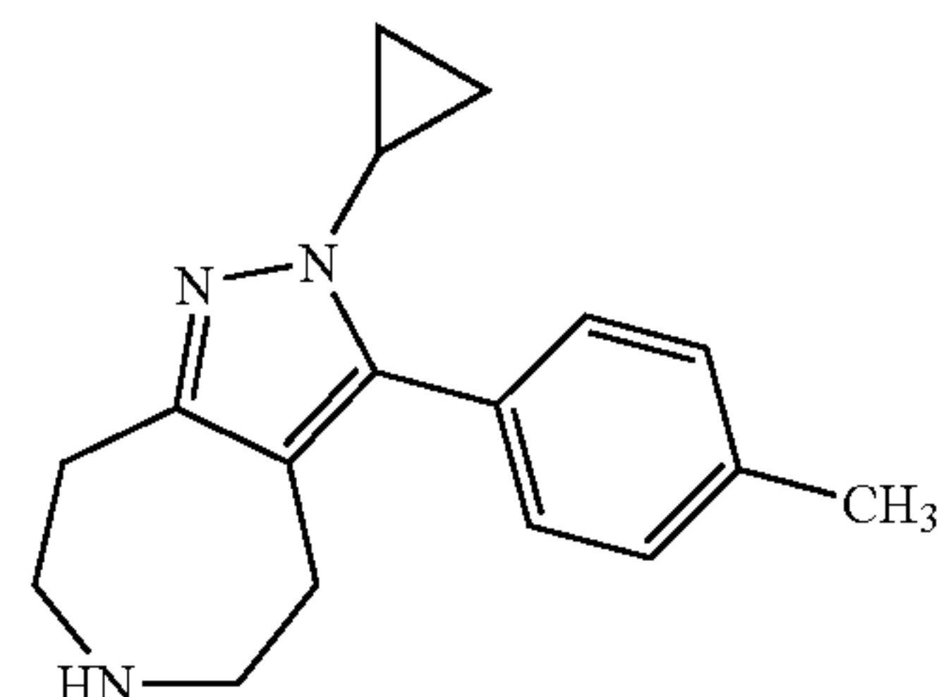
2-Cyclopropyl-3-p-tolyl-2,4,5,6,7,8-hexahydro-1,2,6-triaza-azulene
