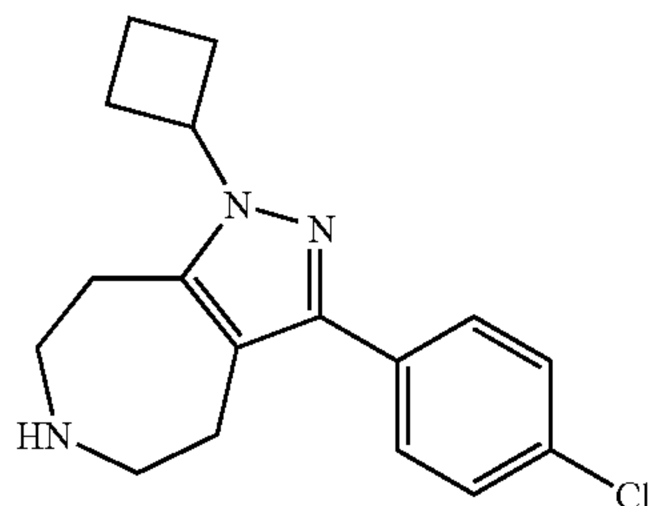
3-(4-Chloro-phenyl)-1-cyclobutyl-1,4,5,6,7,8-hexahydro-1,2,6-triaza-azulene
