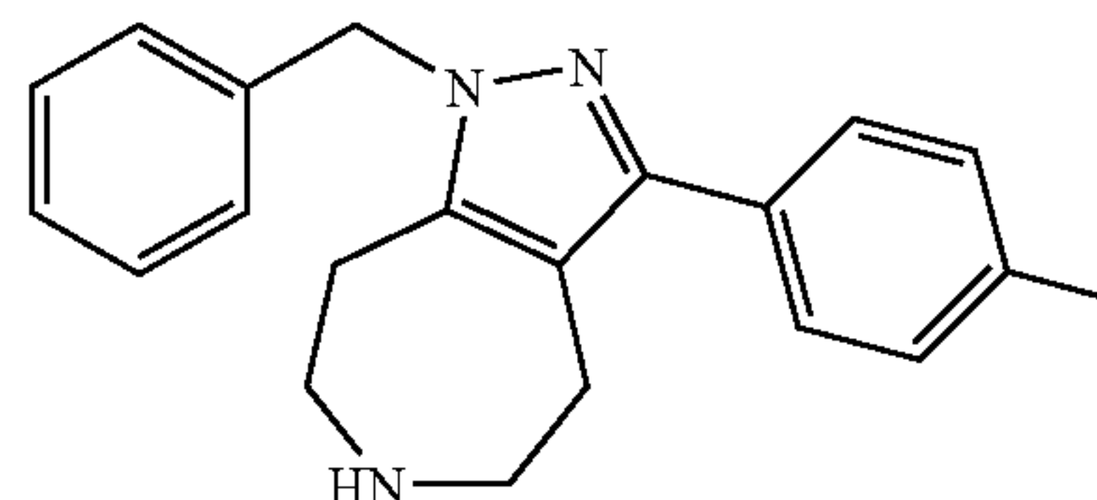
1-Benzyl-3-p-tolyl-1,4,5,6,7,8-hexahydro-1,2,6-triaza-azulene
