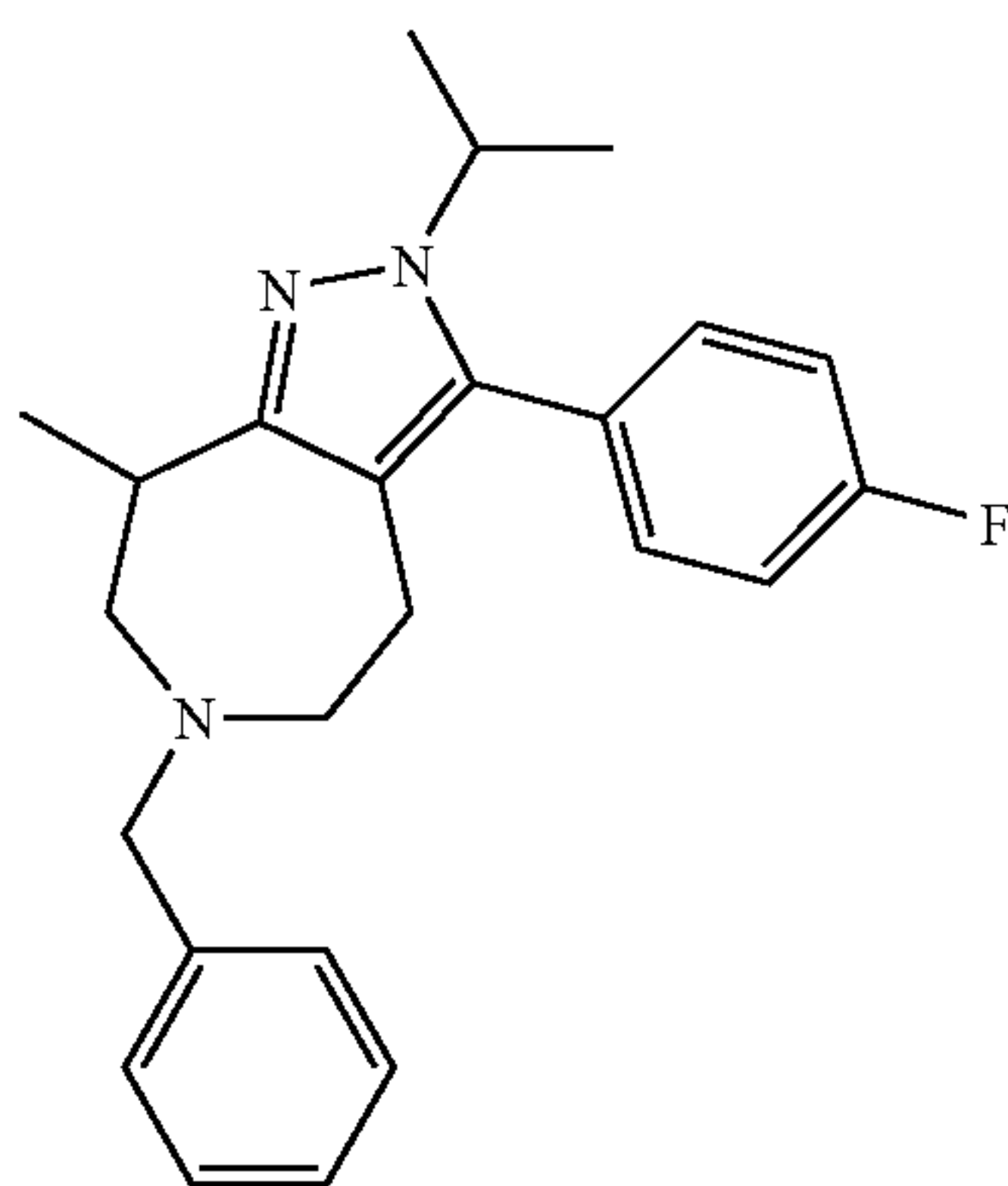
6-Benzyl-3-(4-fluoro-phenyl)-2-isopropyl-8-methyl- 2,4,5,6,7,8-hexahydro-2,2,6-triaza-azulene
