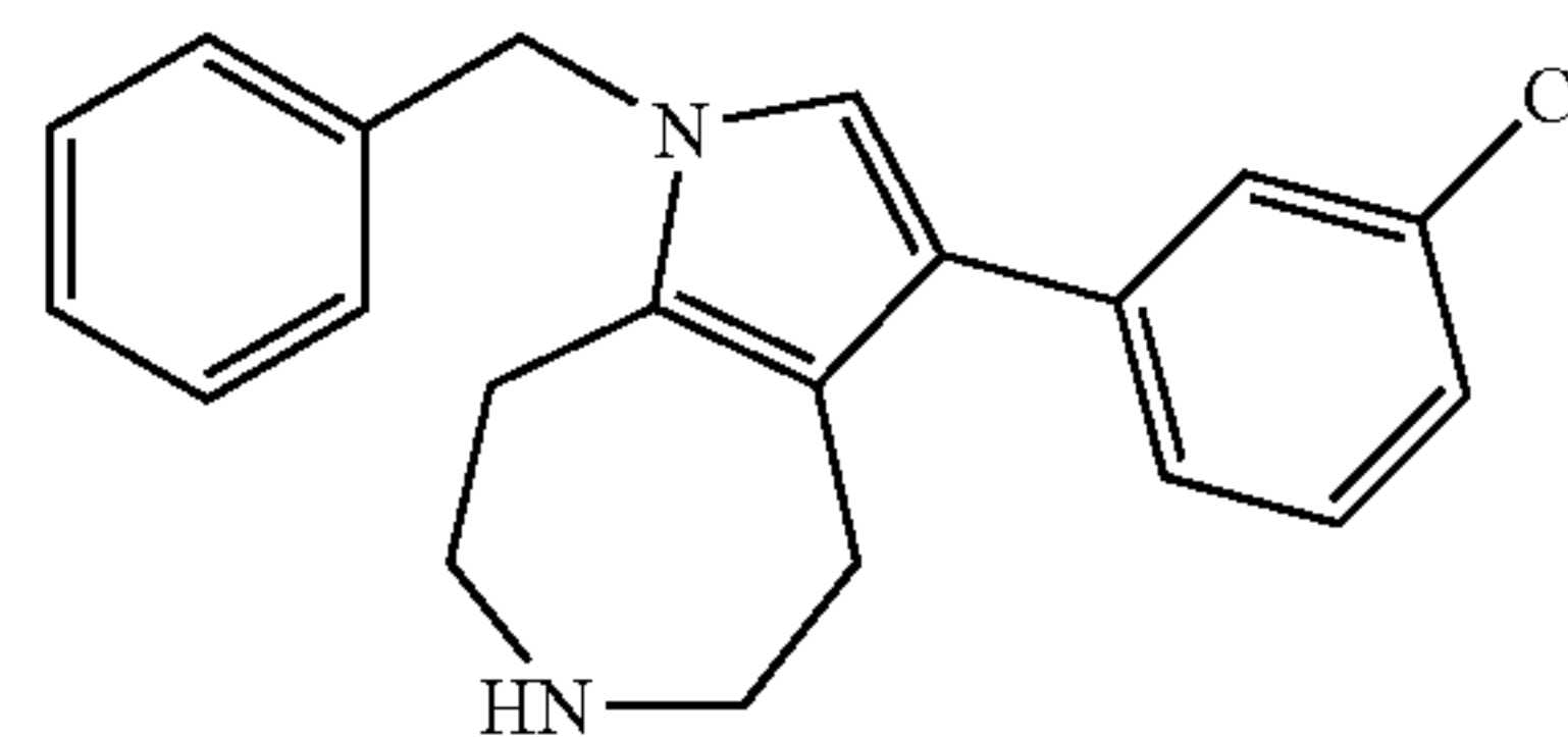
1-Benzyl-3-(3-chloro-phenyl)-1,4,5,6,7,8-hexahydro-pyrrolo[2,3-d]azepine
