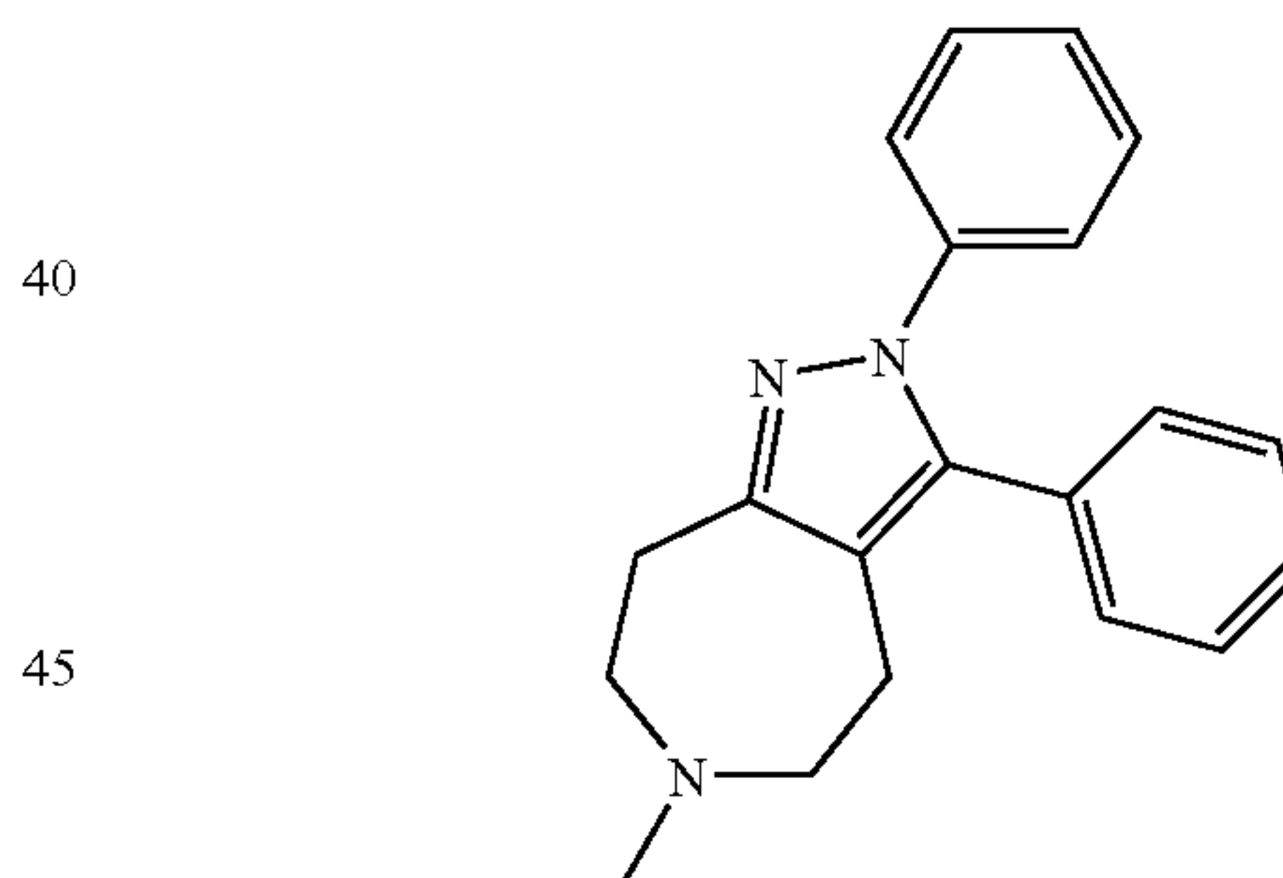
6-Methyl-2,3-diphenyl-2,4,5,6,7,8-hexahydro-1,2,6-triaza-azulene
