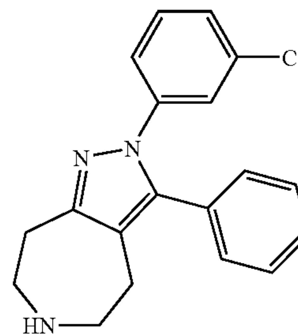
2-(3-Chlorophenyl)-3-phenyl-2,4,5,6,7,8-hexahydro-1,2,6-triaza-azulene
