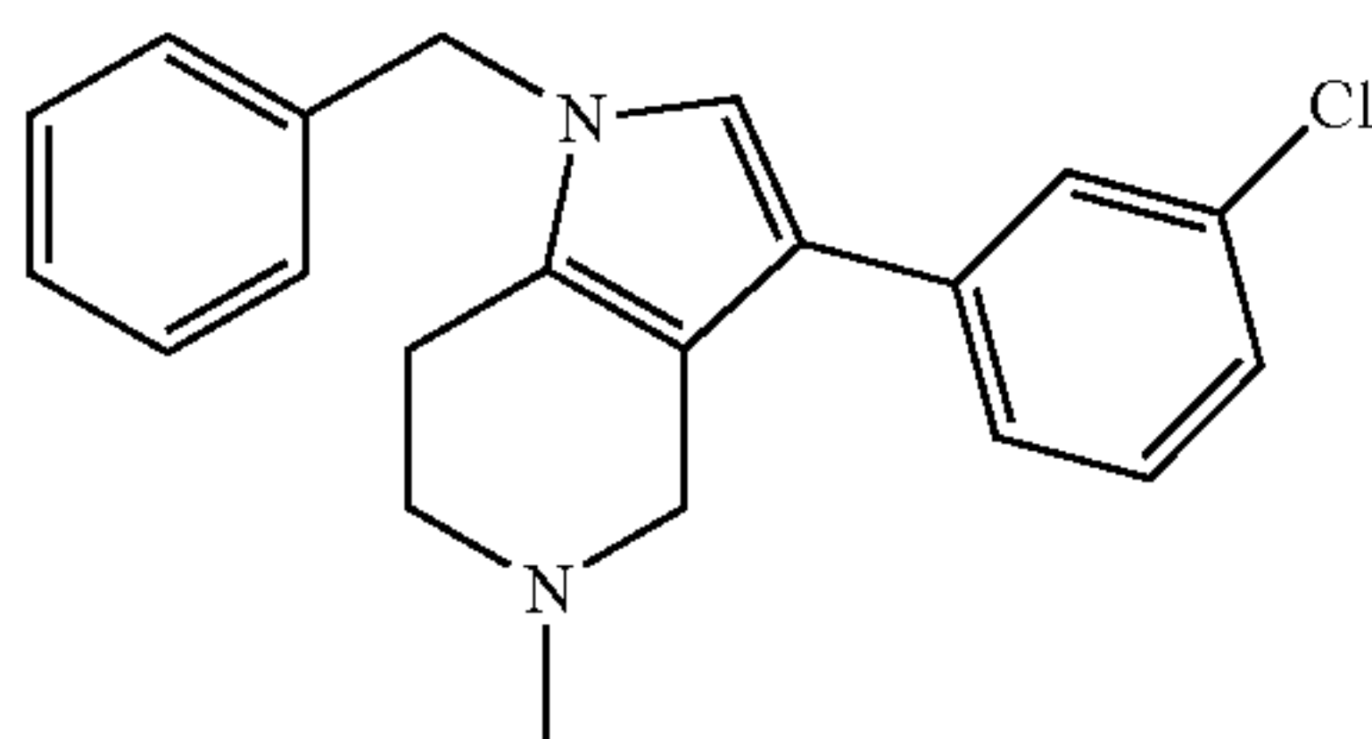
1-Benzyl-3-(3-chloro-phenyl)-5-methyl-4,5,6,7-tetrahydro-1H-pyrrolo[3,2-c]pyridine
