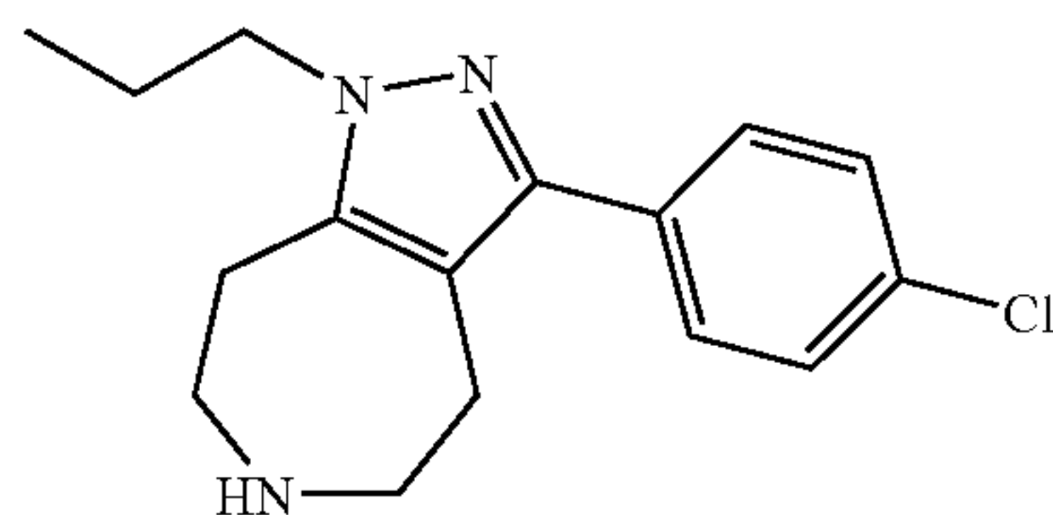
3-(4-Chloro-phenyl)-1-propyl-1,4,5,6,7,8-hexahydro-1,2,6-triaza-azulene
