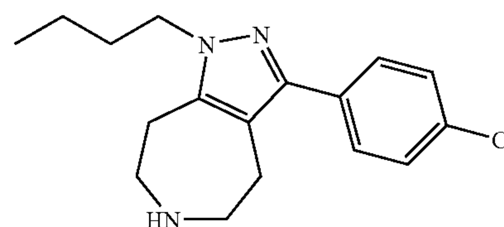
1-Butyl-3-(4-chloro-phenyl)-1,4,5,6,7,8-hexahydro-1,2,6-triaza-azulene
