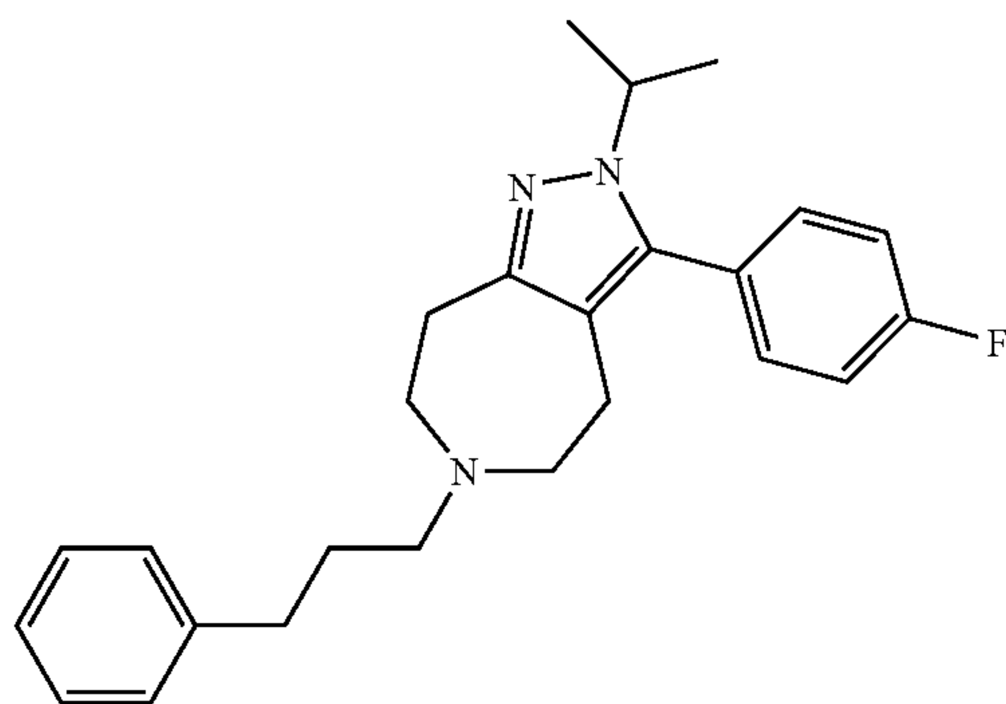
3-(4-Fluoro-phenyl)-2-isopropyl-6-(3-phenyl-propyl)-2,4,5,6,7,8-hexahydro-1,2,6-triaza-azulene
