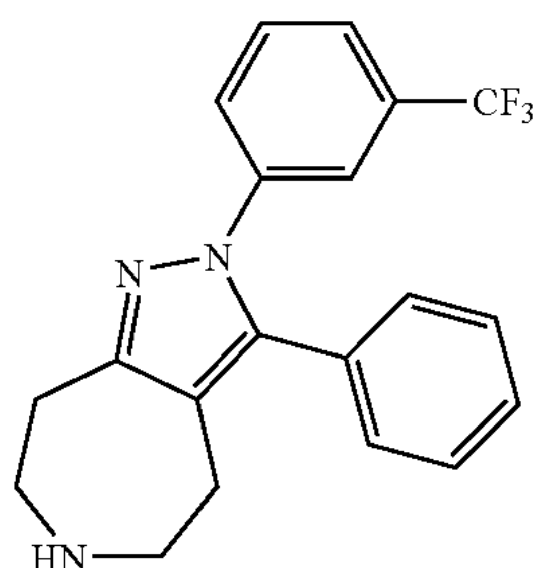
3-Phenyl-2-(3-trifluoromethyl-phenyl)-2,4,5,6,7,8-hexahydro-1,2,6-triaza-azulene
