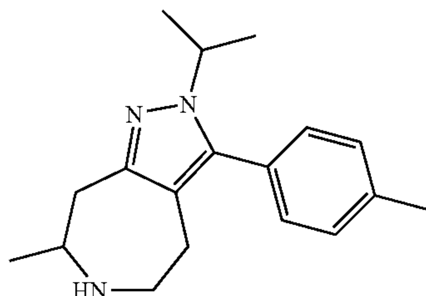
2-Isopropyl-7-methyl-3-p-tolyl-2,4,5,6,7,8-hexahy- dro-1,2,6-triaza-azulene
