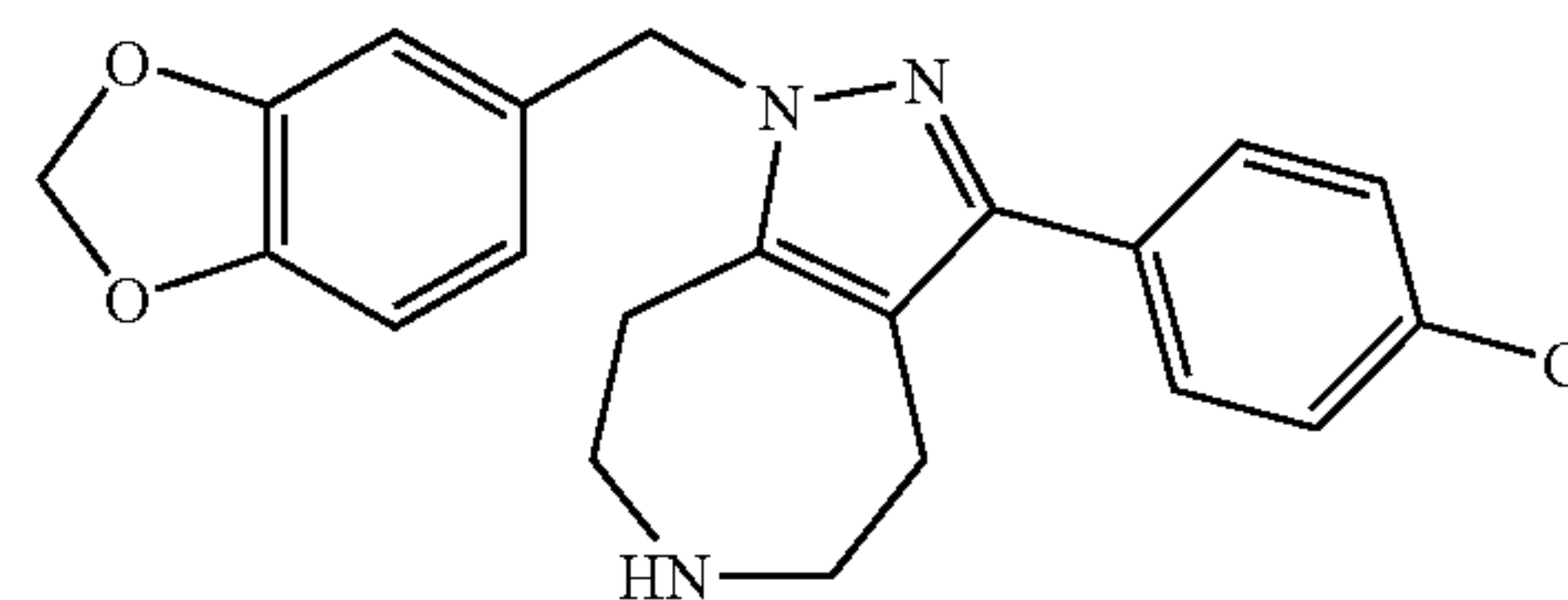
1-Benzo[1,3]dioxol-5-ylmethyl-3-(4-chloro-phenyl)-1,4,5,6,7,8-hexahydro-1,2,6-triaza-azulene
