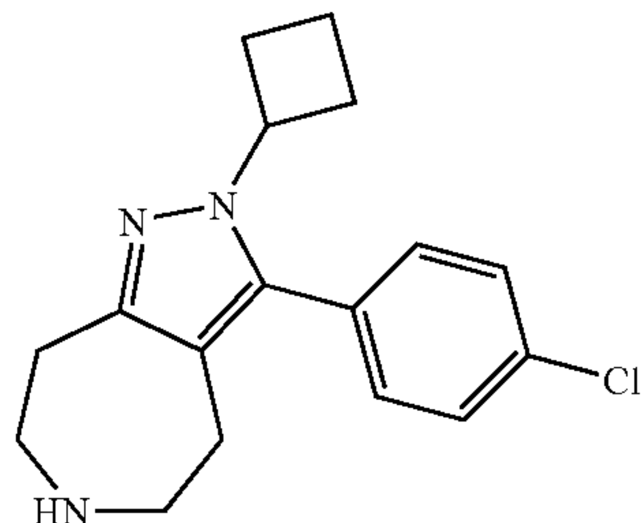
3-(4-Chloro-phenyl)-2-cyclobutyl-2,4,5,6,7,8-hexahydro-1,2,6-triaza-azulene
