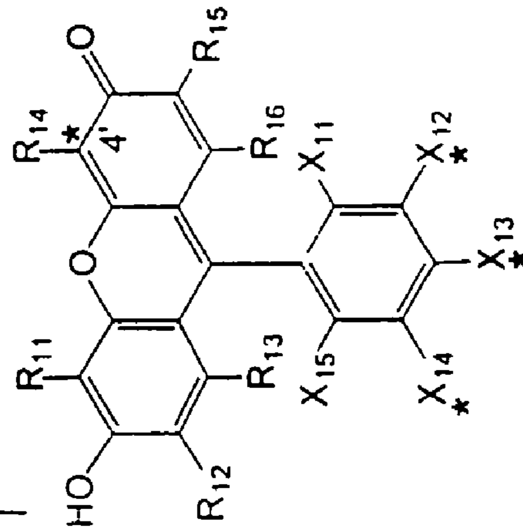
FLUORESCIEIN
