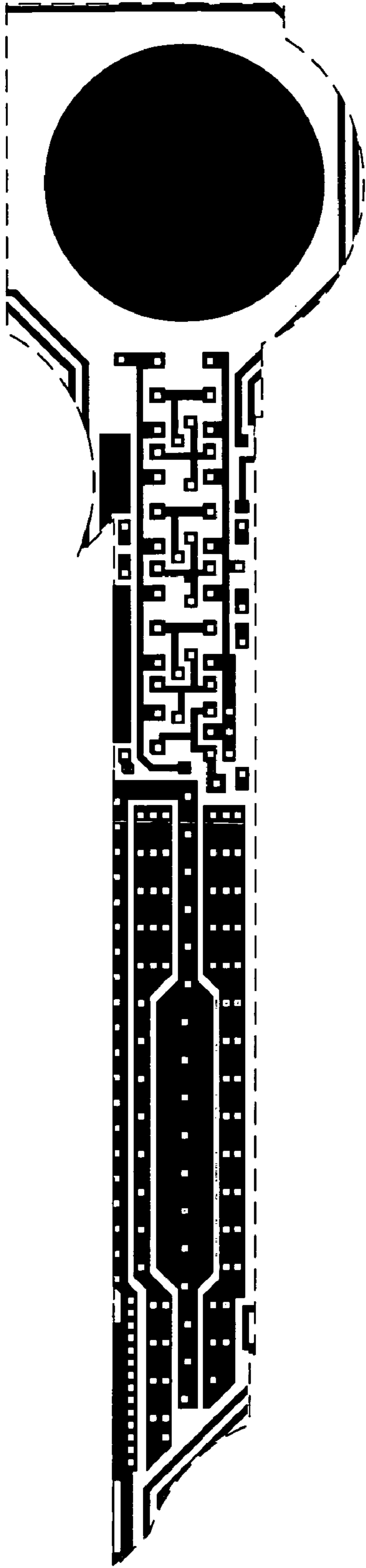
Metal 1 mask
