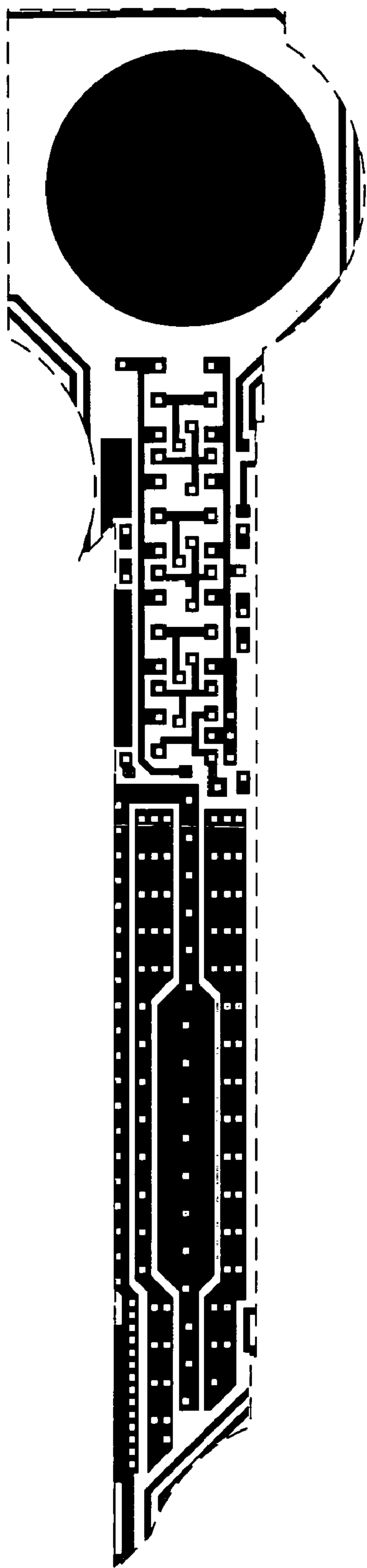
Metal 1 mask
