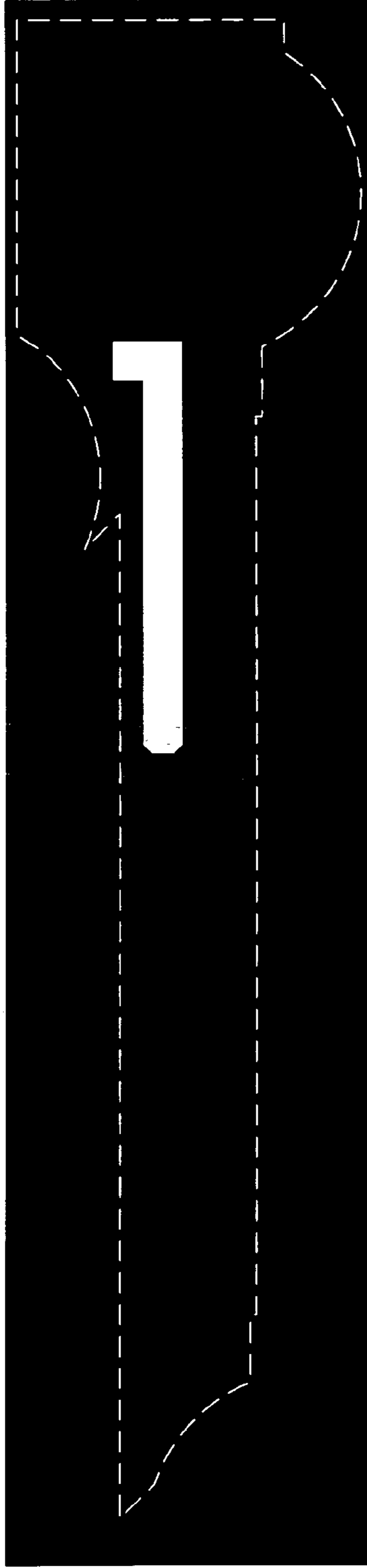
N-Well mask
