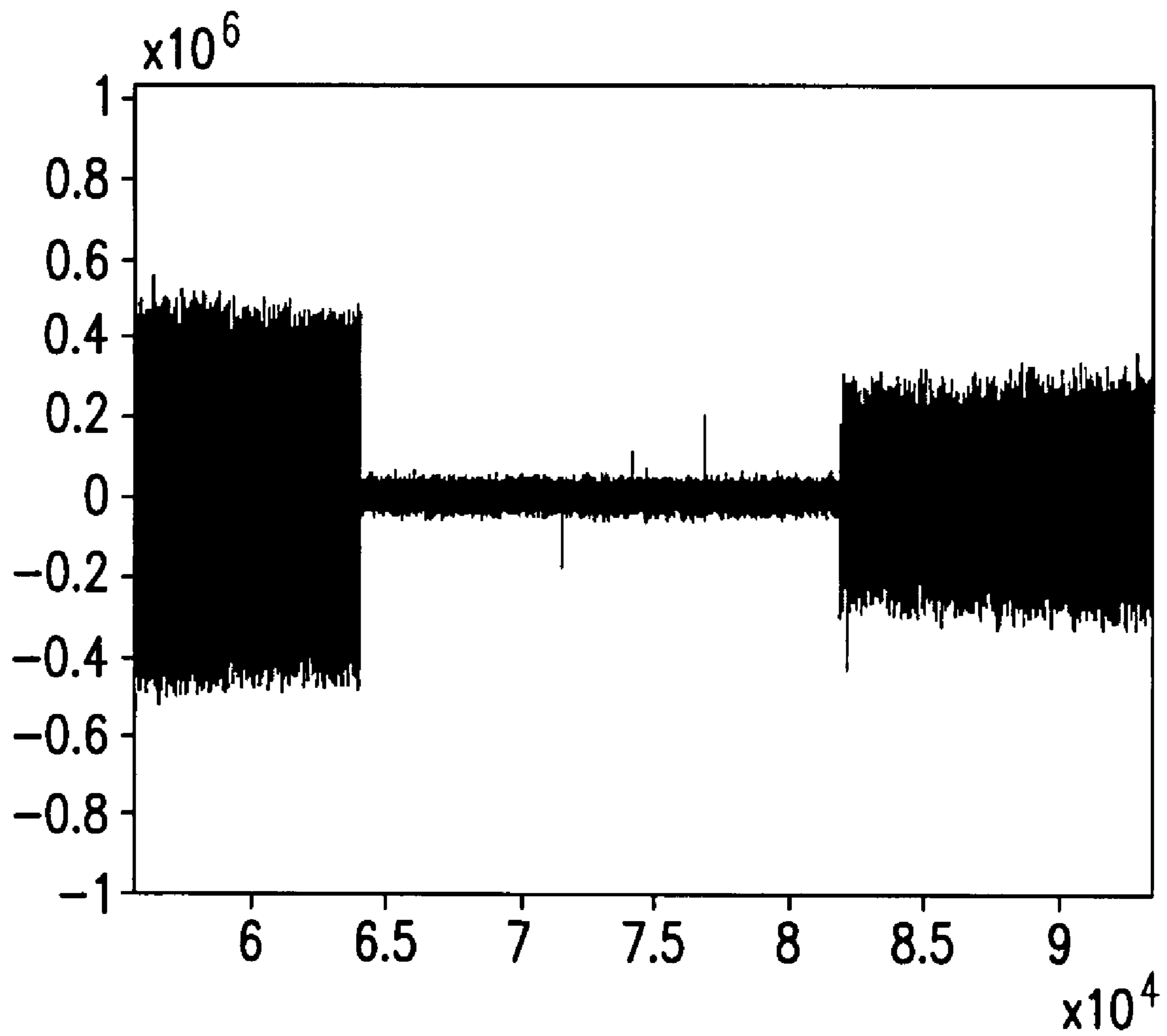
TIME DOMAIN DISPLAY OF RAW DATA
