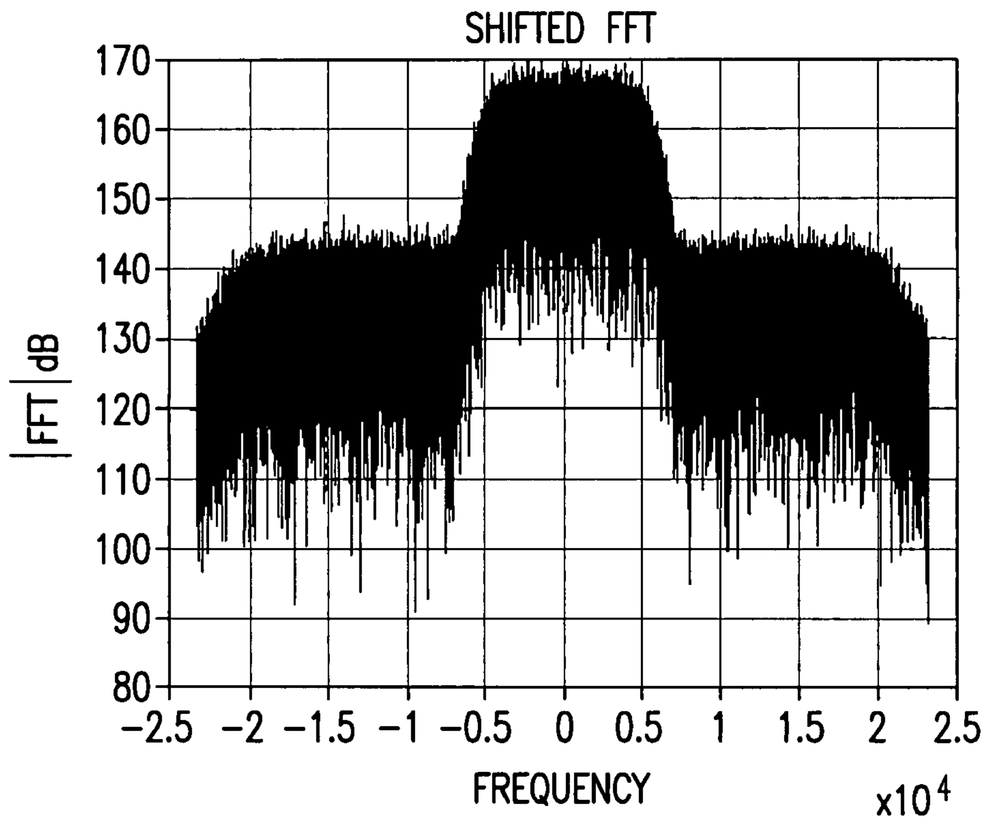
FREQUENCY DOMAIN DISPLAY OF DESIRED SIGNAL
