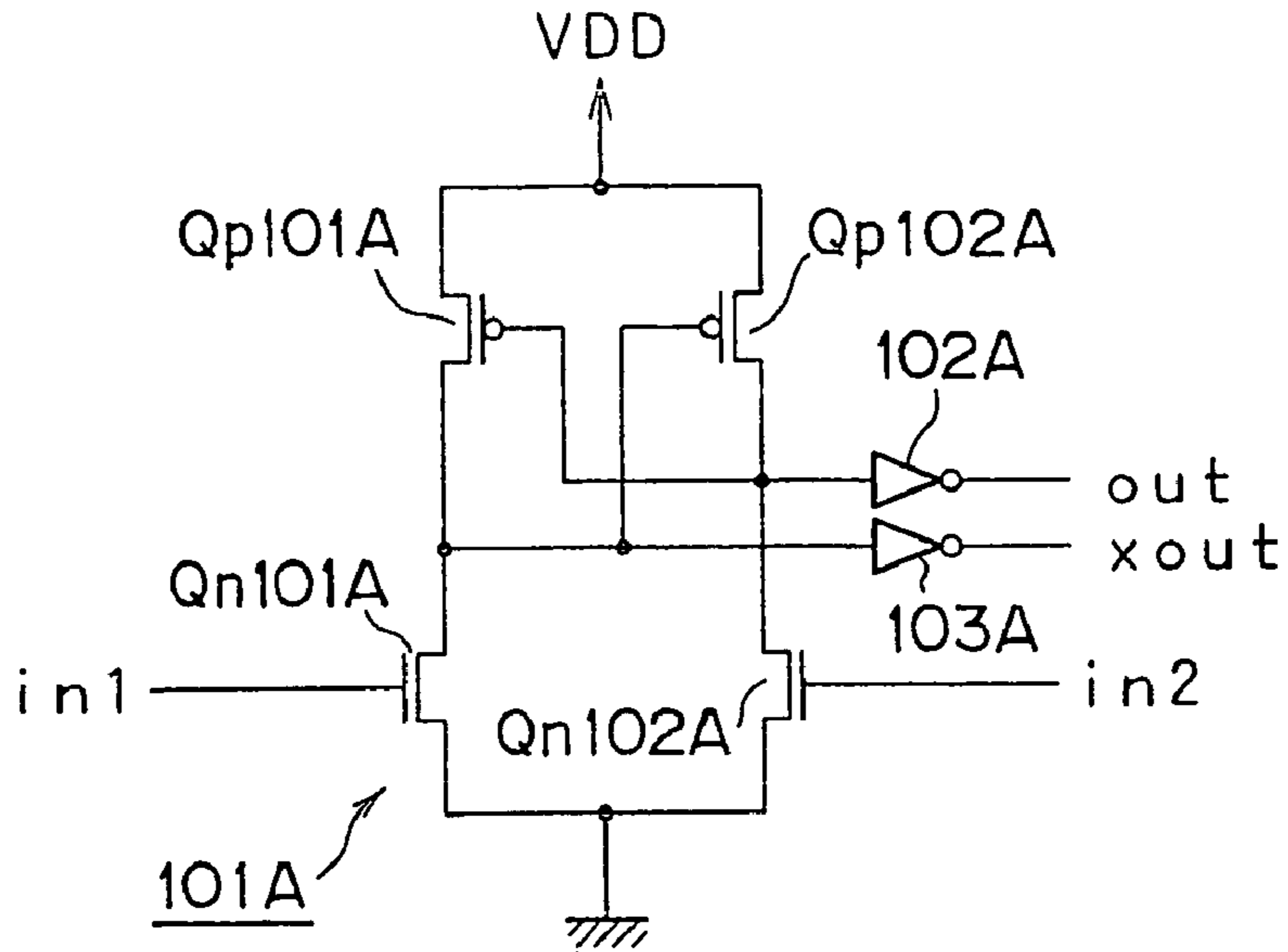
FIG. 13A RELATED ART 1
