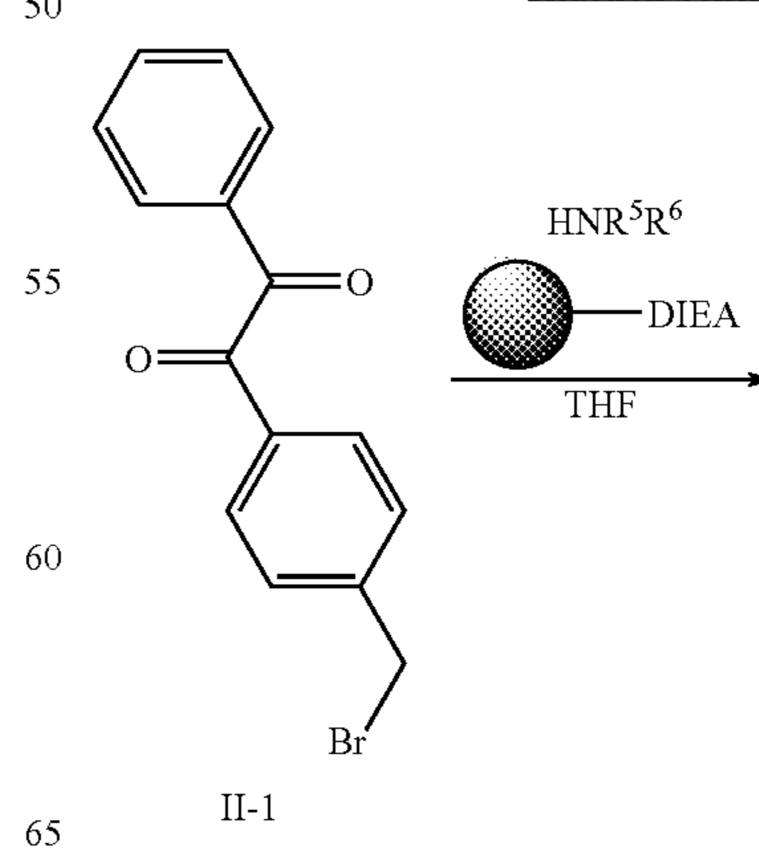
Reaction Scheme III
