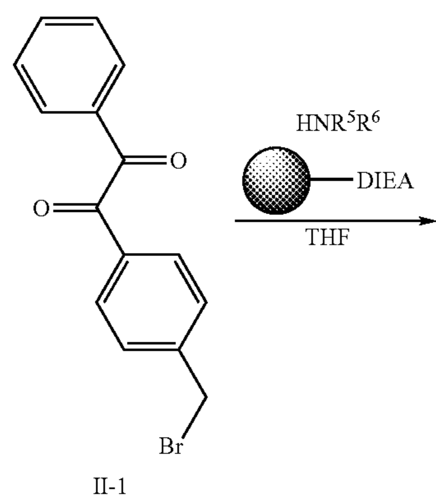
Reaction Scheme II
