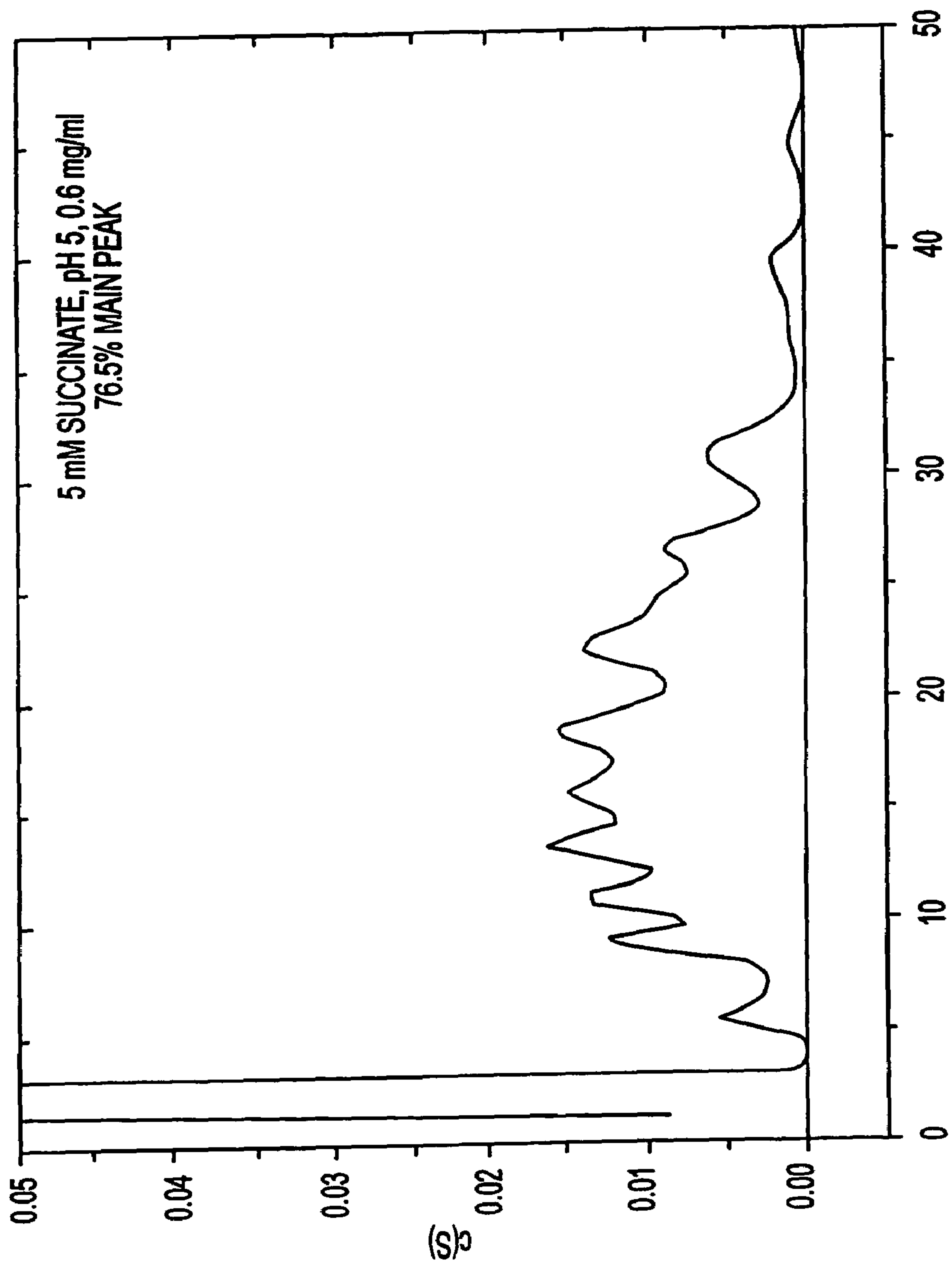
SEDIMENTATION COEFFICIENT (SVEDBERGS) FIG. 5
