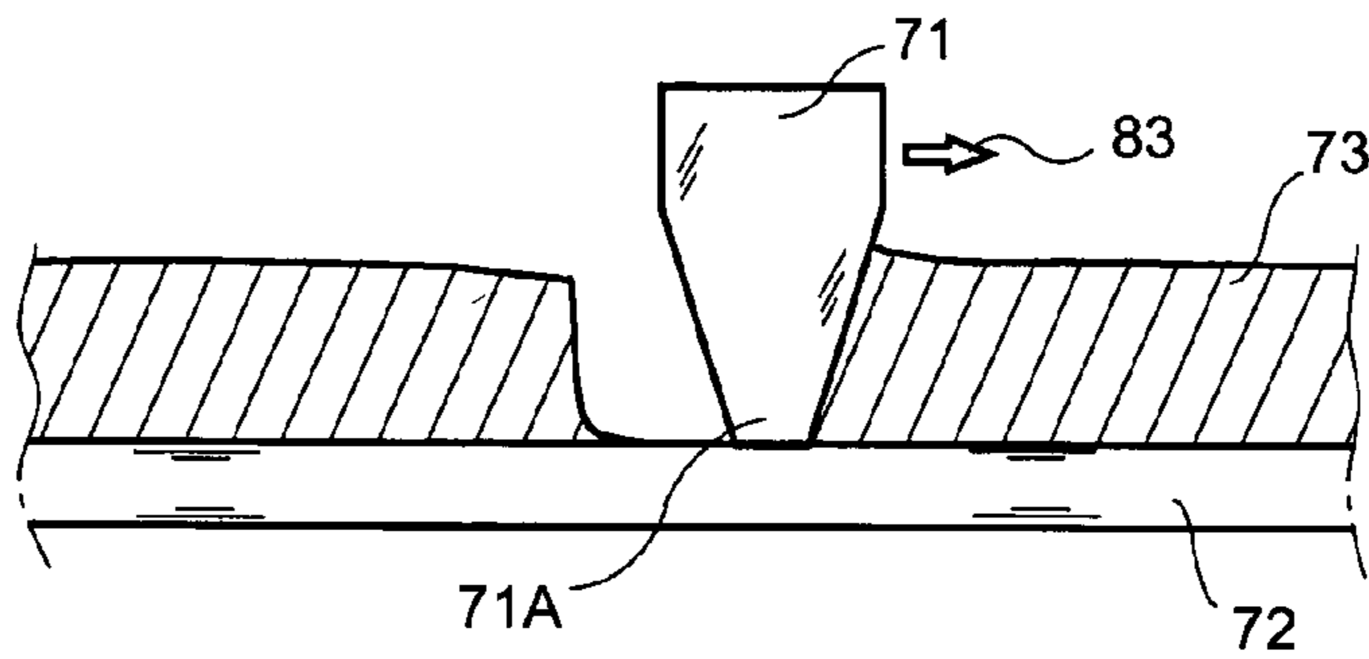
FIG22 [PRIOR ART]
