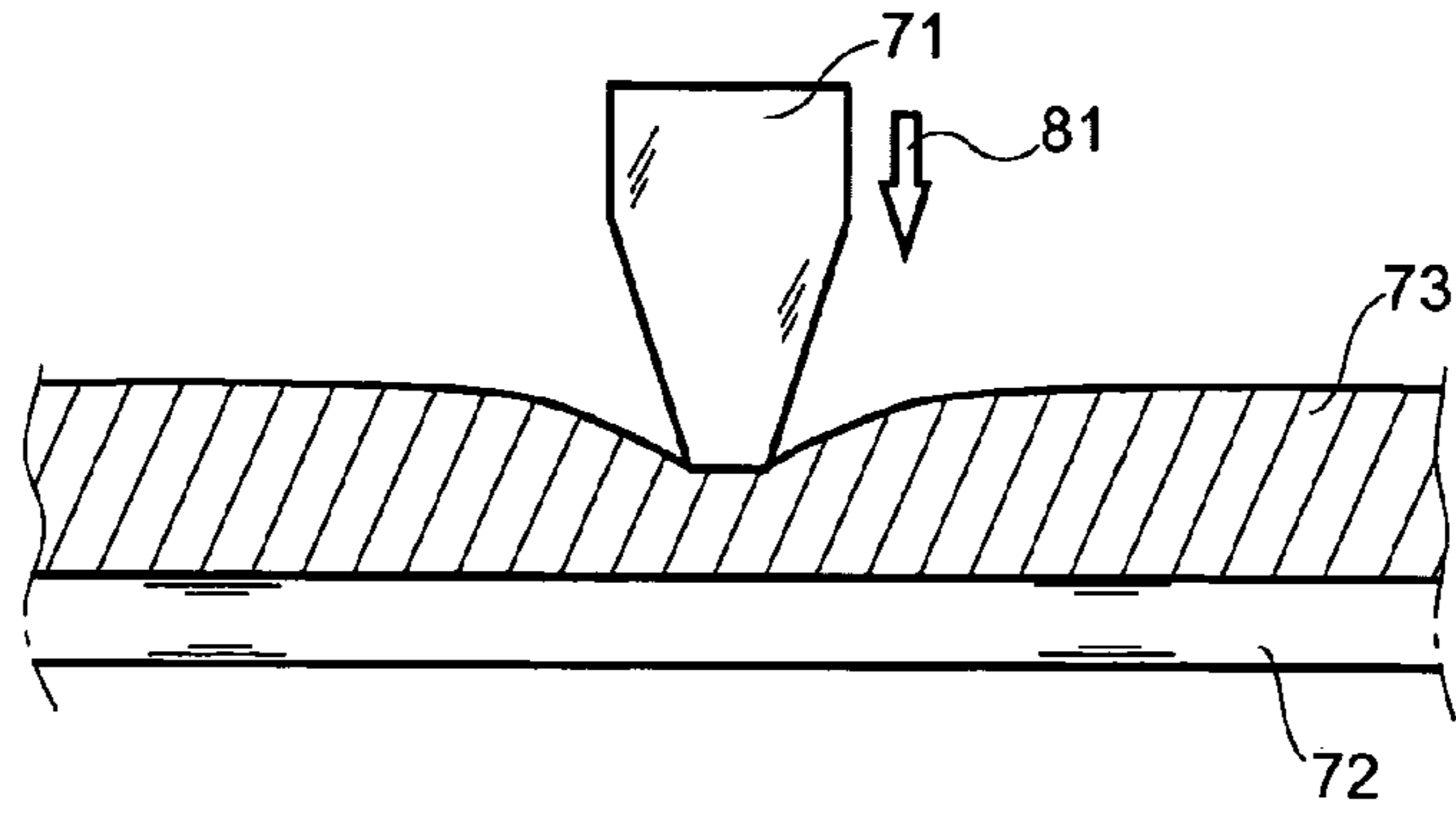
FIG20 [PRIOR ART]
