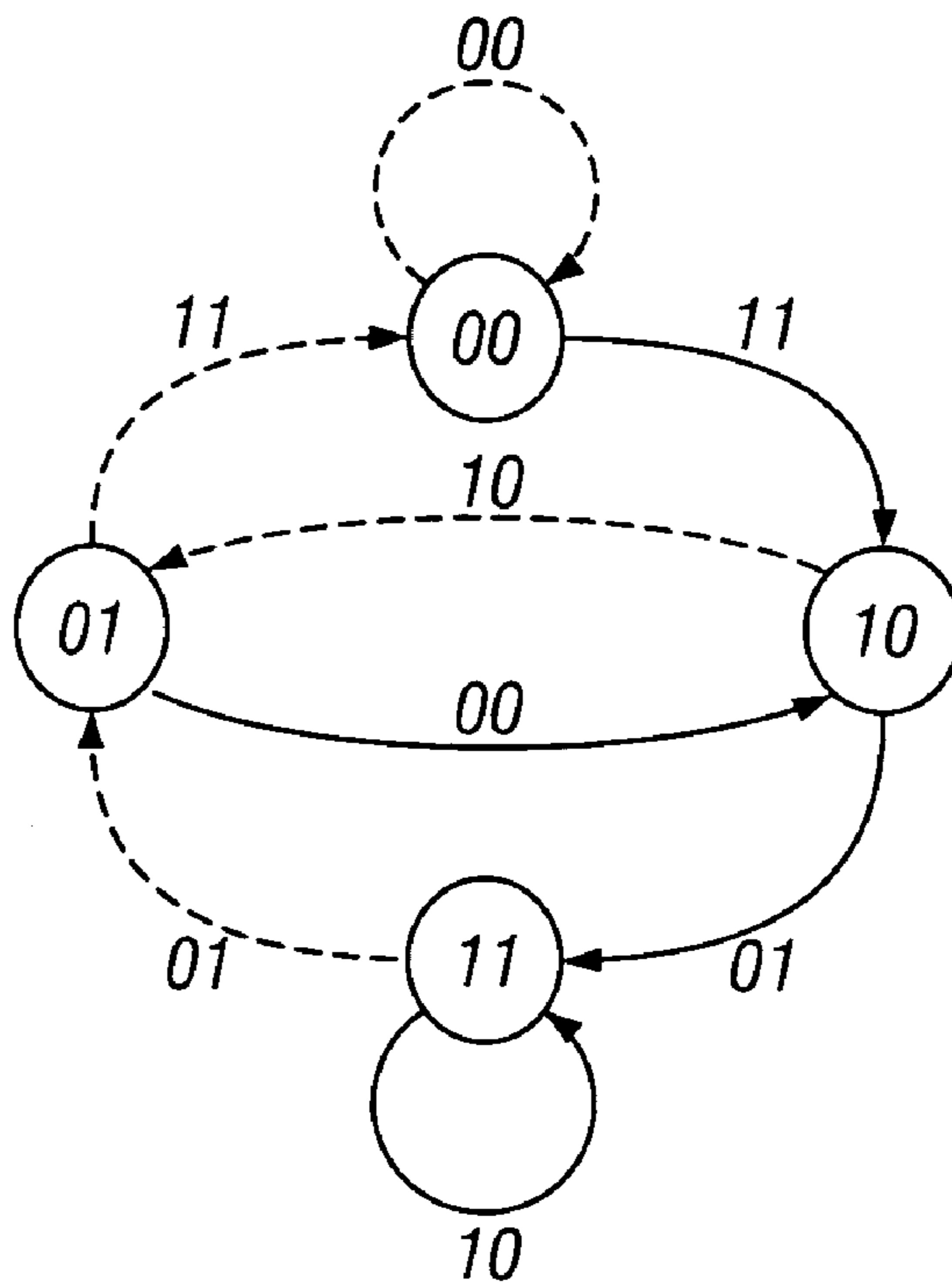
FIG. 3 (Prior Art)
