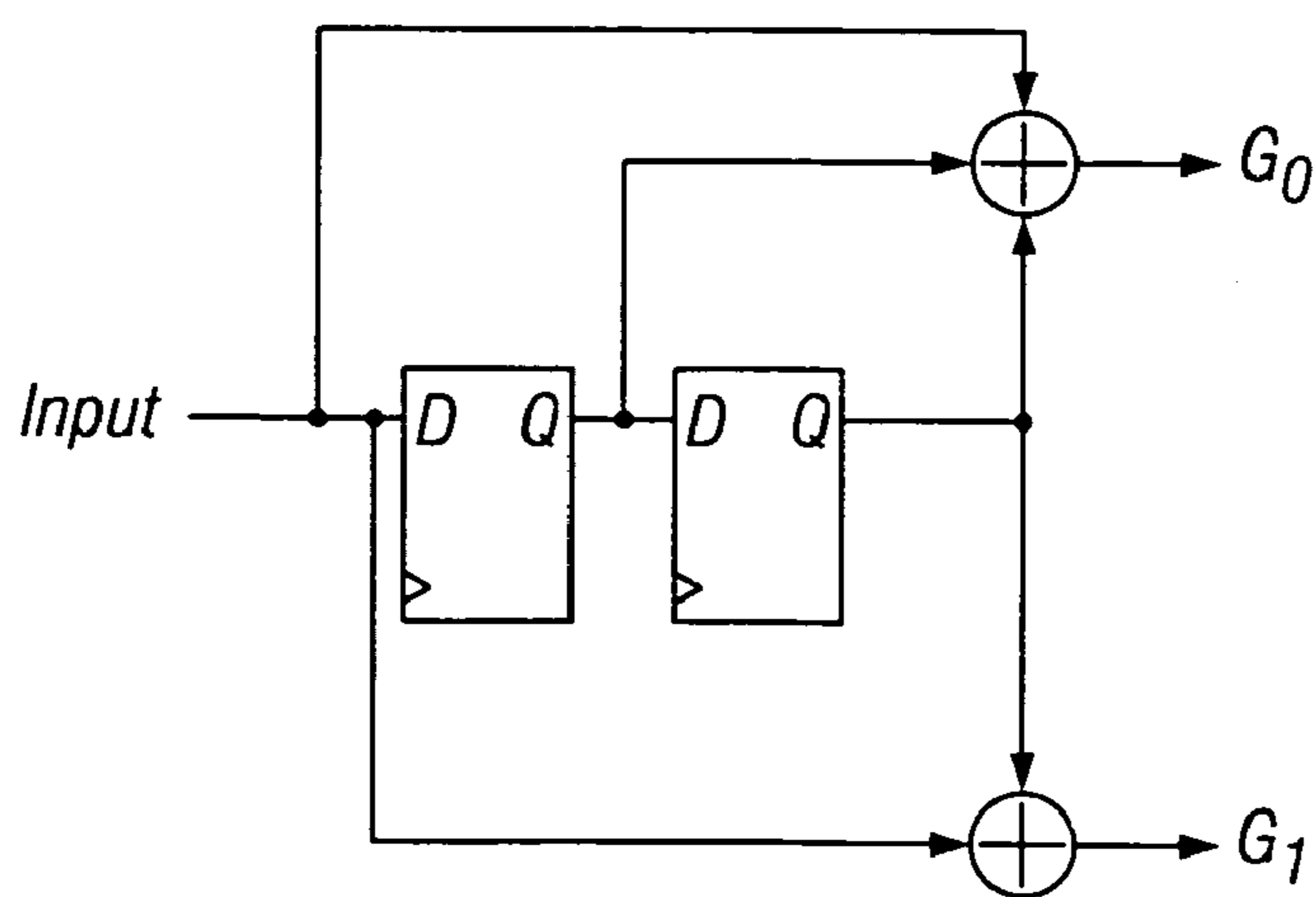
FIG. 2 (Prior Art)
