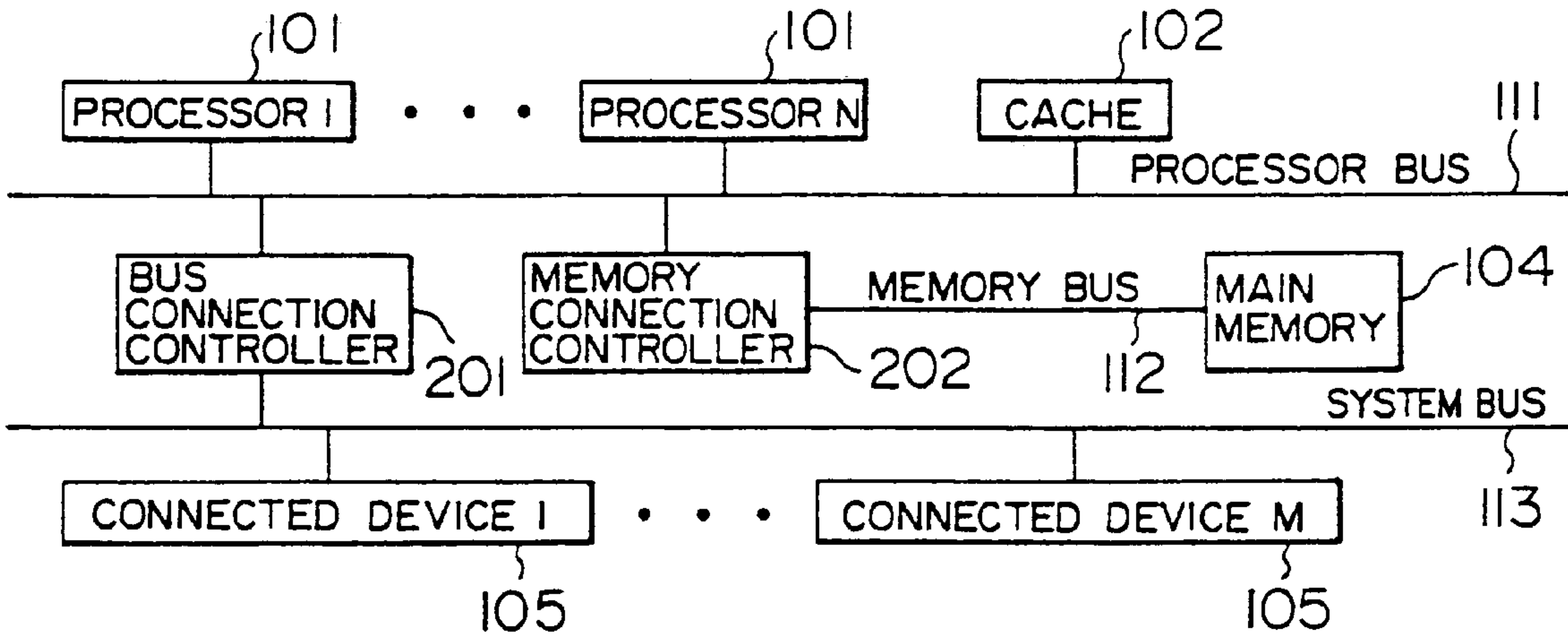
FIG. 3 PRIOR ART
