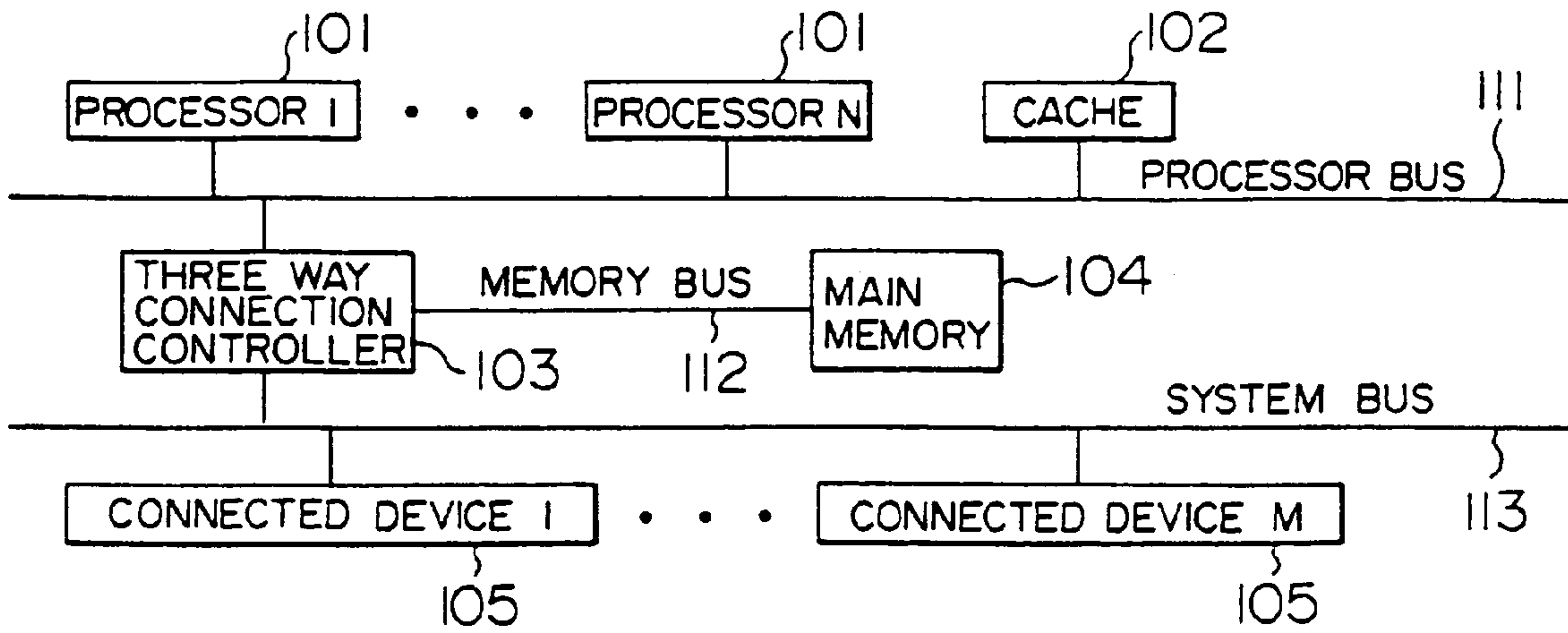
FIG. 2 PRIOR ART
