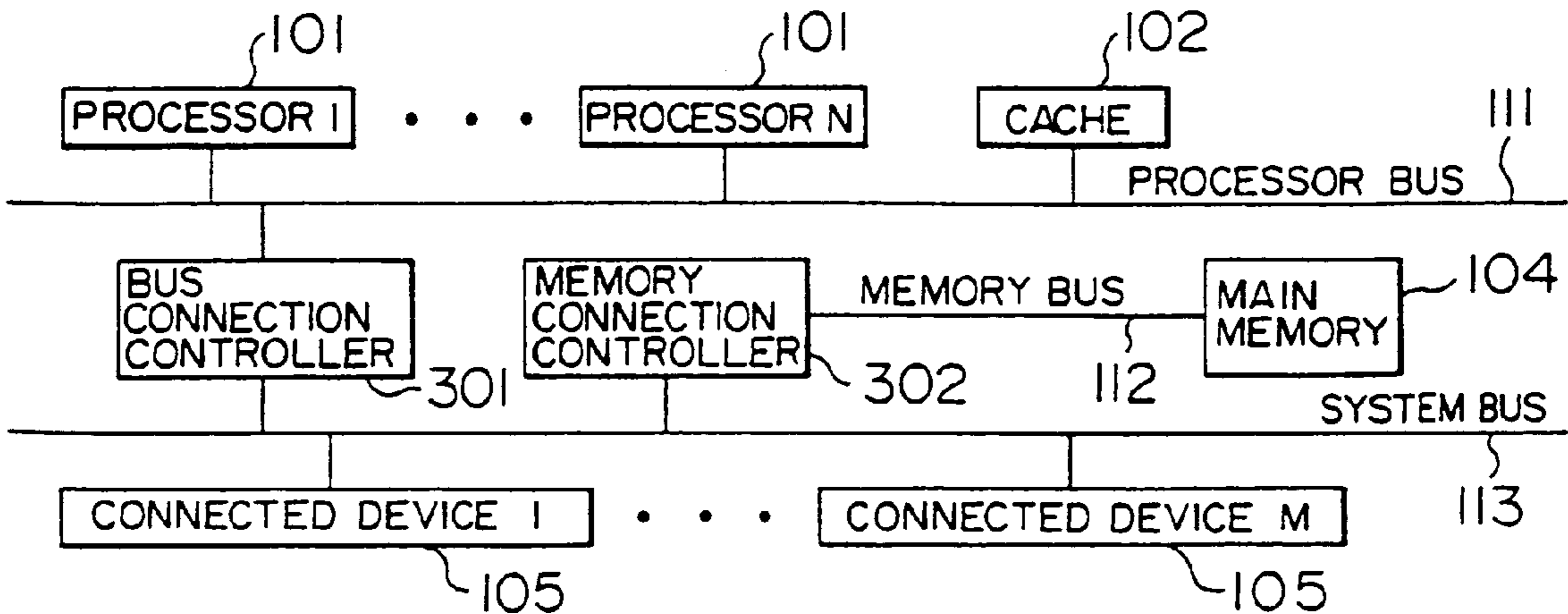
FIG. 3 PRIOR ART
