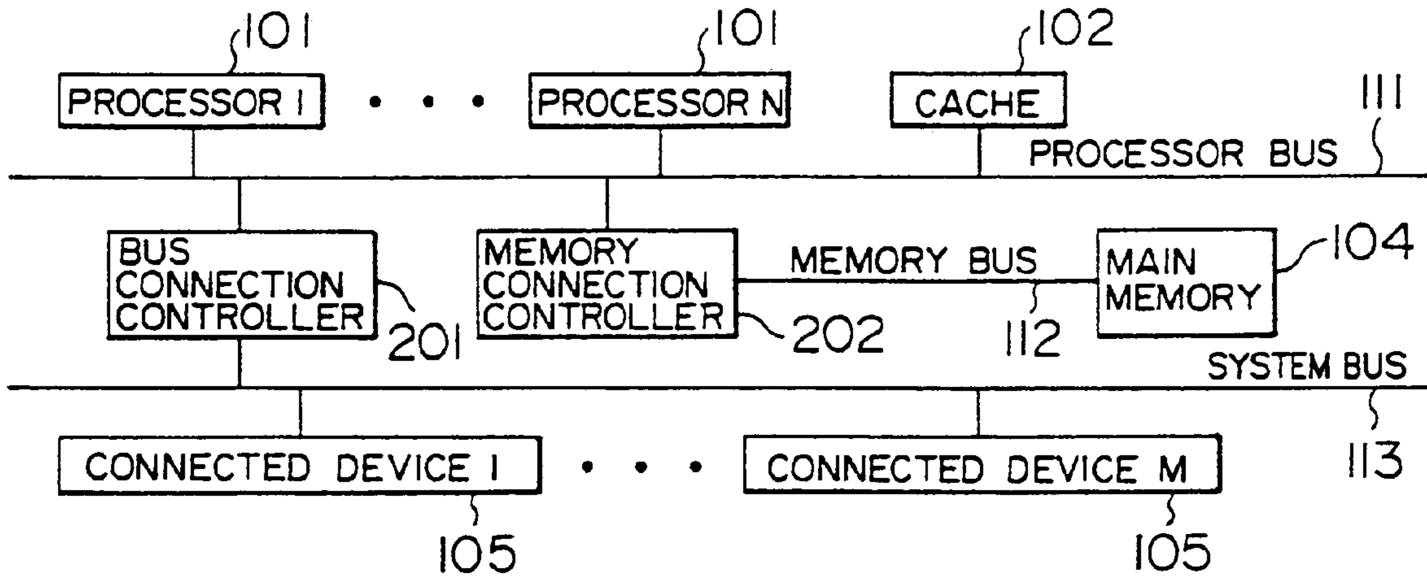
FIG. 3 PRIOR ART
