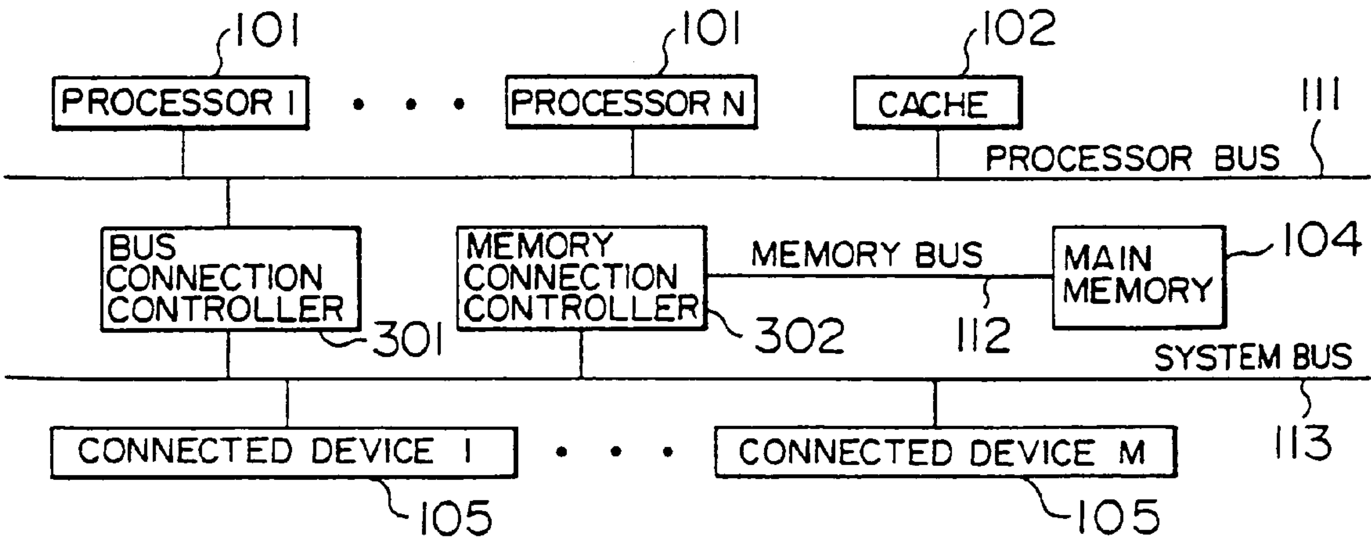
FIG. 3 PRIOR ART
